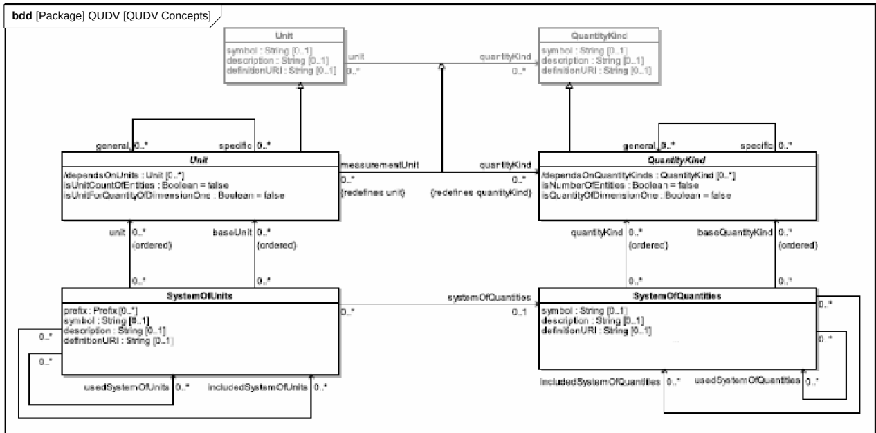
Figure E.5: QUDV Concepts Diagram
