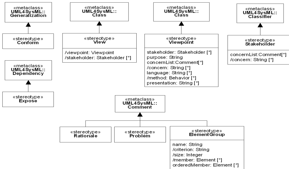
Figure 7.1: Stereotypes defined in package ModelElements
