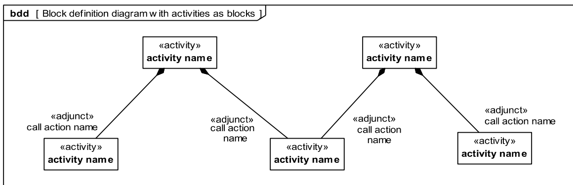
Figure 11.1 - Block definition diagram with activities as blocks
