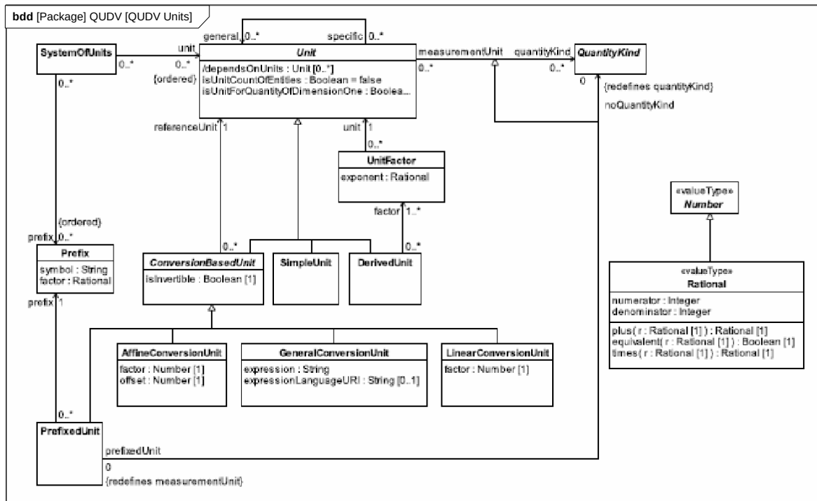
Figure E.6: QUDV Units Diagram
