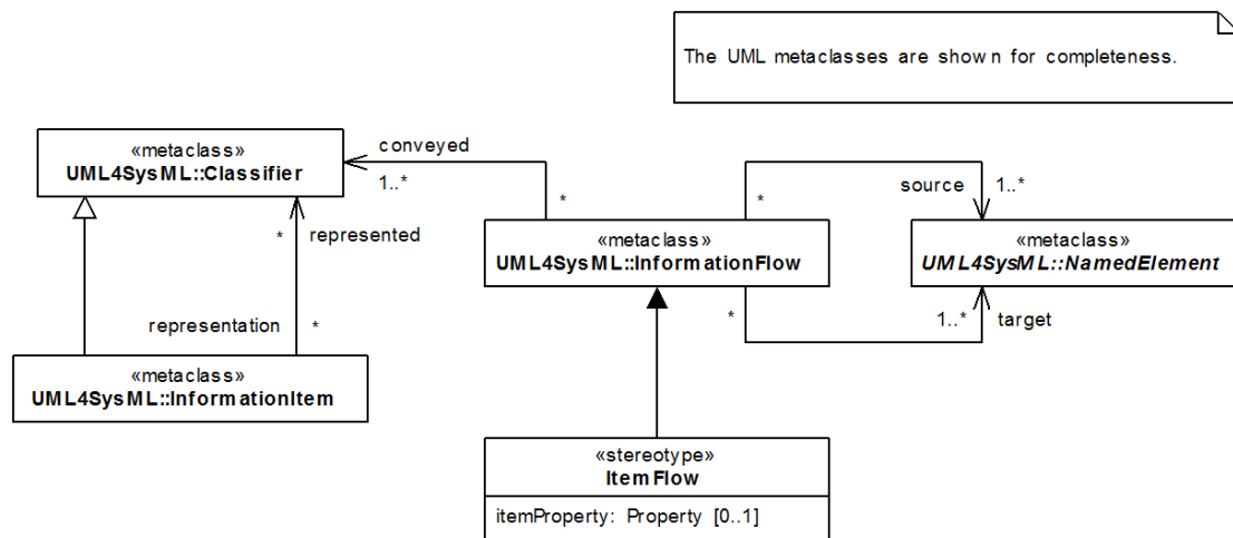
Figure 9.5 - Item Flow Stereotype
