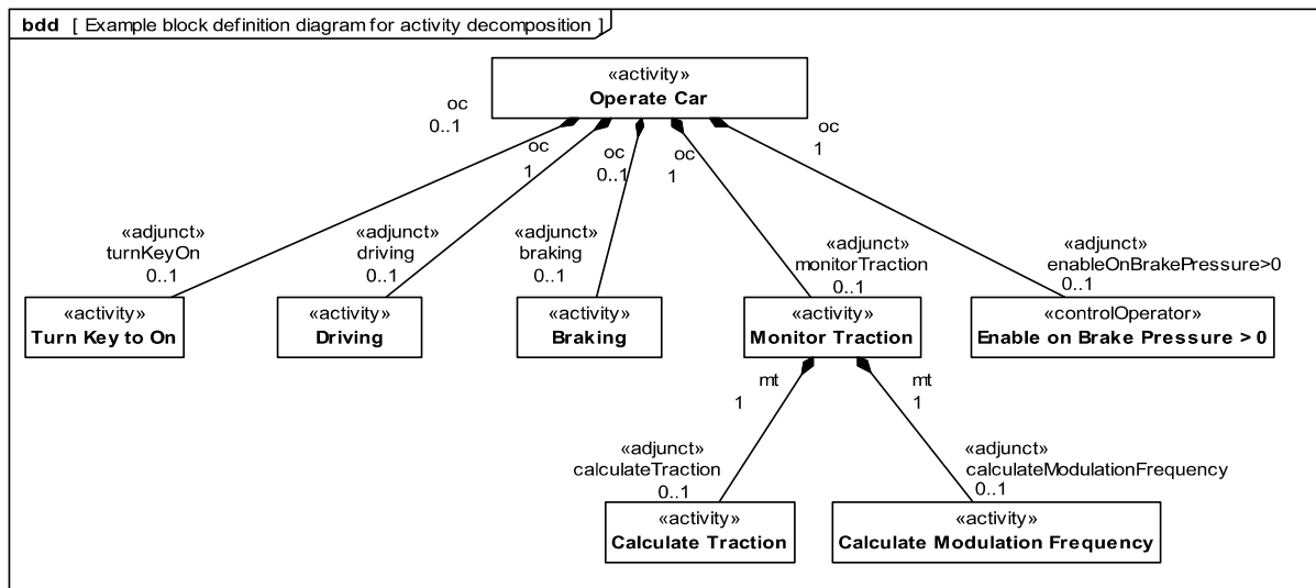
Figure 11.13 - Example block definition diagram for activity decomposition
