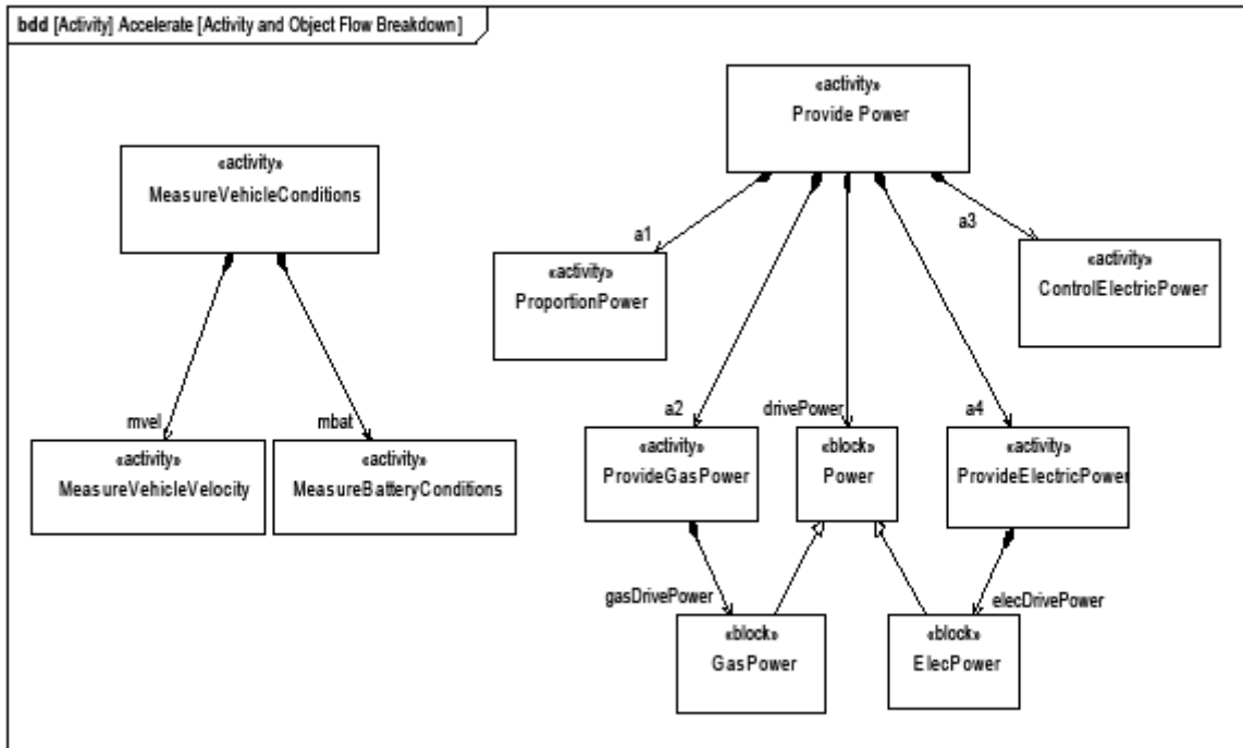
Figure D.37: Decomposition of “Accelerate” Function (Block Definition diagram)
