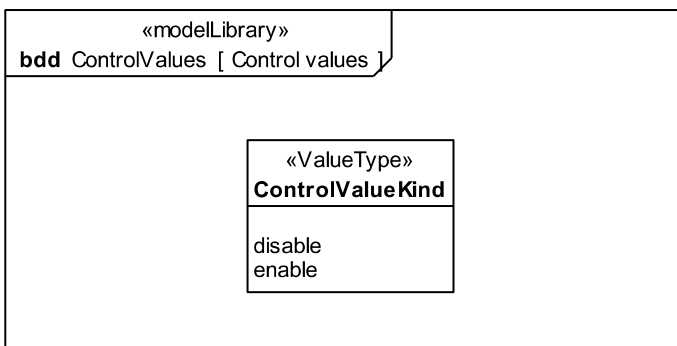
Figure 11.9 - Control values
