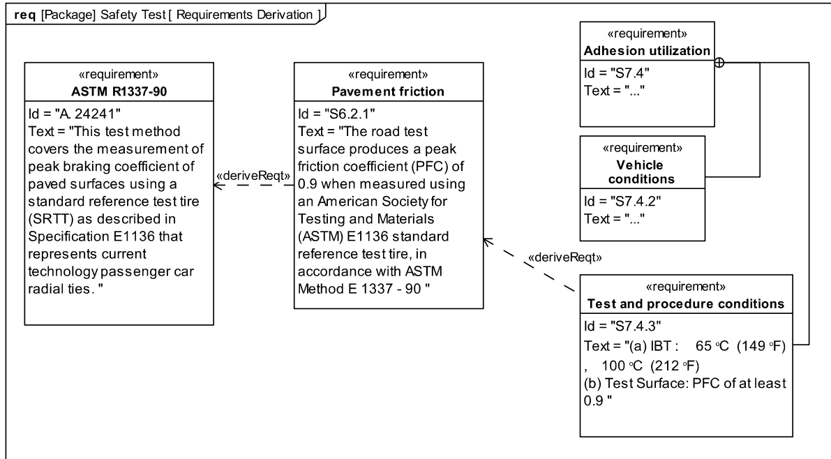
Figure 16.2 - Requirements Derivation
