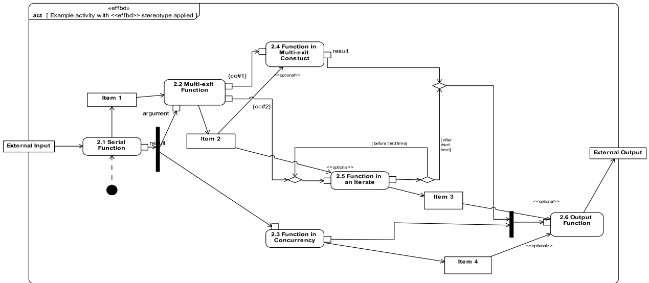
Figure E.1: Example activity with «effbd» stereotype applied
