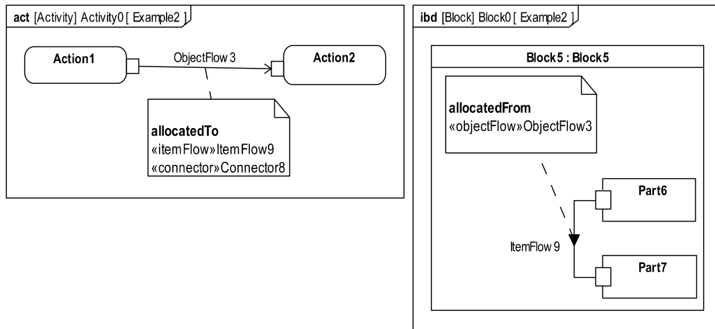
Figure 15.6 - Example of flow allocation from ObjectFlow to ItemFlow
