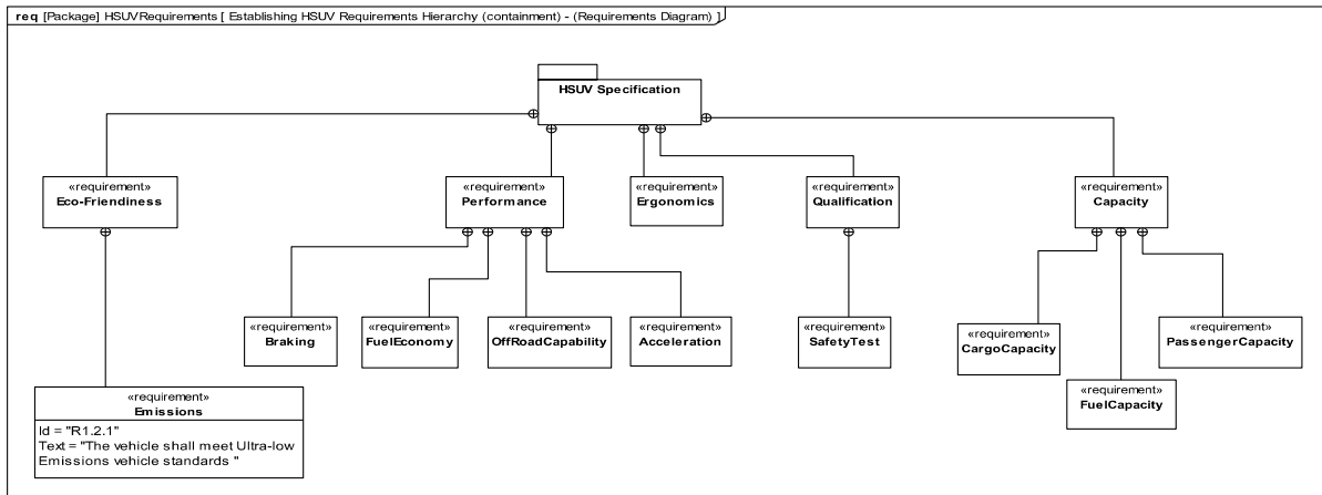
Figure D.11: Establishing HSUV Requirements Hierarchy (containment) - (Requirements Diagram)
