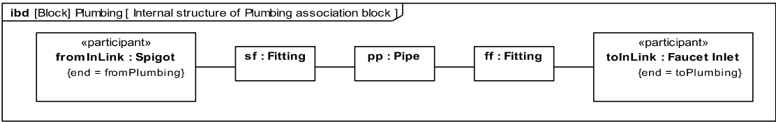
Figure 9.13 - Internal structure of Plumbing association block
