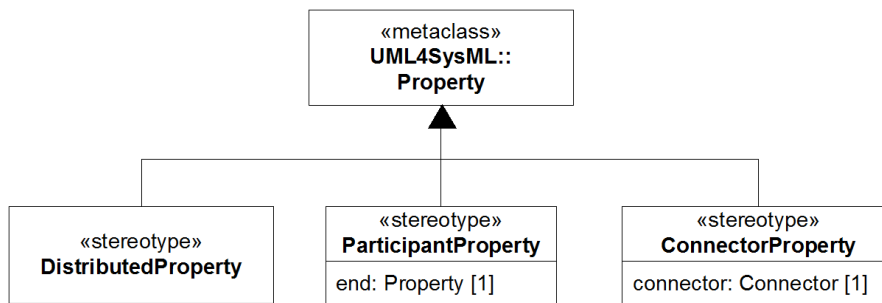
Figure 8.2: Abstract syntax extensions for SysML blocks
