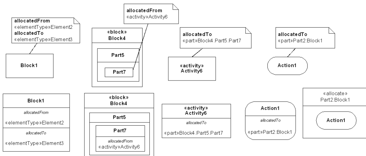
Figure 15.4 - Behavior Allocation
