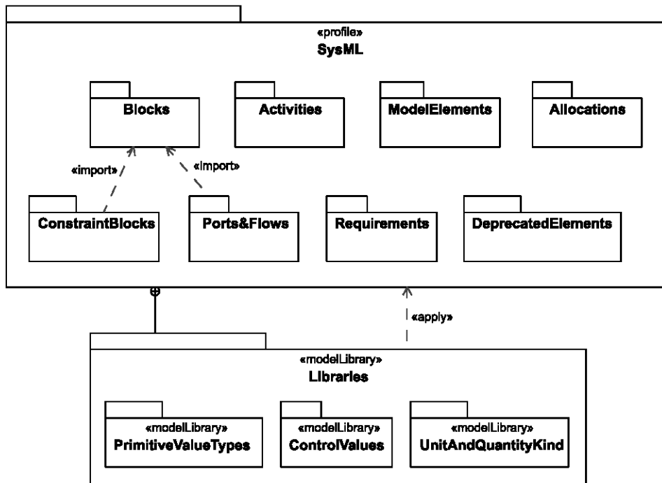
Figure 4.3: SysML Package Structure
