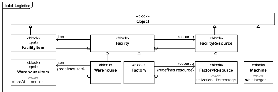
Figure 8.22 Property-specific types in facility example
