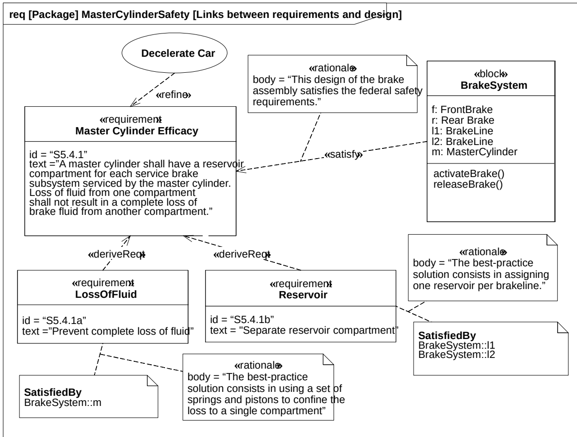
Figure 16.3 - Links between requirements and design
