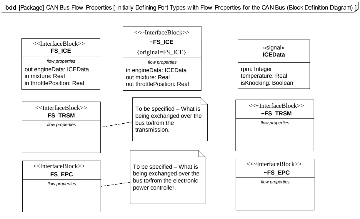
Figure D.21: Initially Defining Port Types with Flow Properties for the CAN Bus (Block Definition Diagram)
