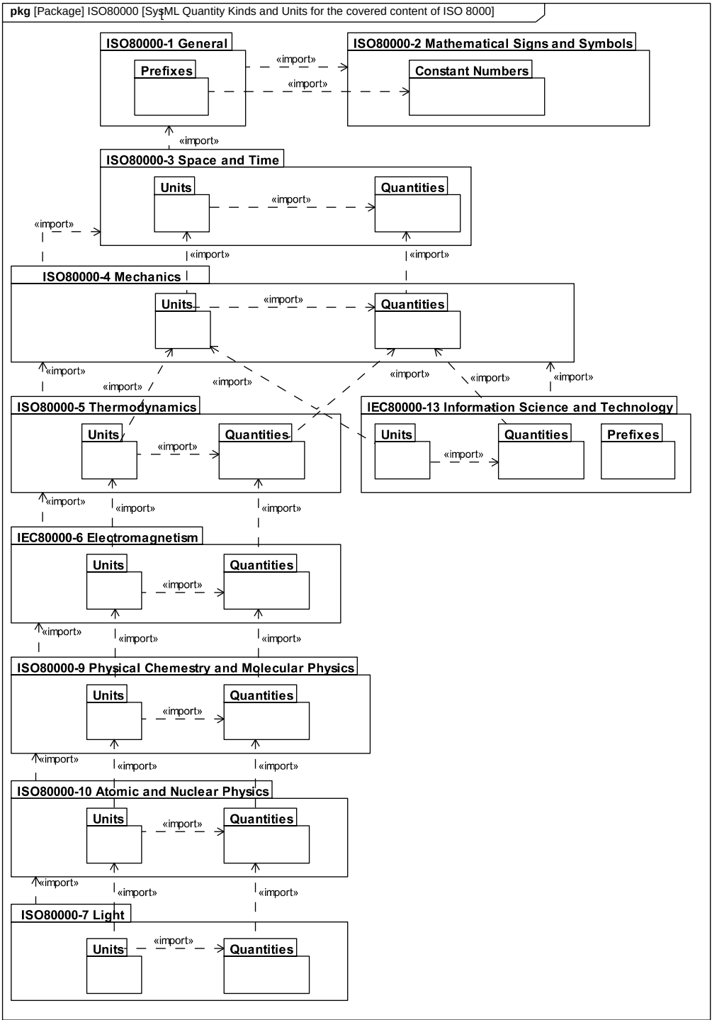
Figure E.12: Organization of the definitions of units and quantities from the normative parts of ISO 80000 covered in SysML 1.4, which includes all the normative content of parts 3,4,5,6; the subset of parts 7,9,10 corresponding to the content from SysML 1.3 and the subset of part 13 pertaining to commonly used units of
