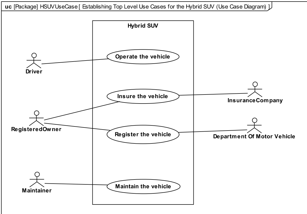
Figure D.5: Establishing Top Level Use Cases for the Hybrid SUV (Use Case Diagram)
