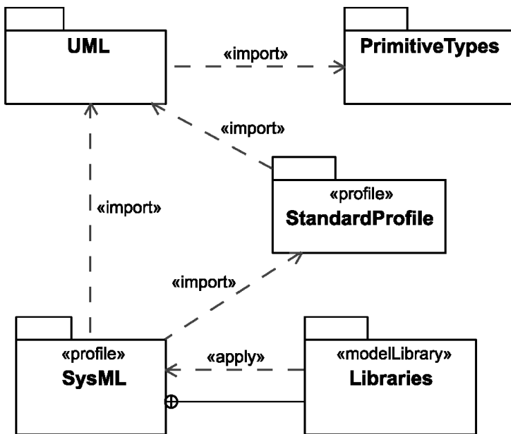
Figure 4.2: SysML Extension of UML
