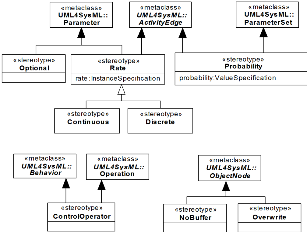
Figure 11.8 - Abstract Syntax for SysML Activity Extensions
