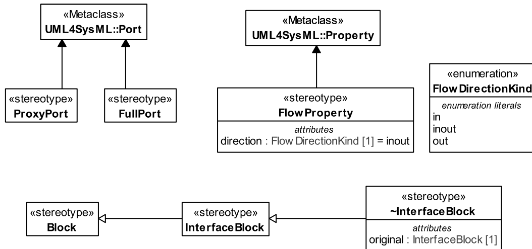
Figure 9.1 - Port Stereotypes
