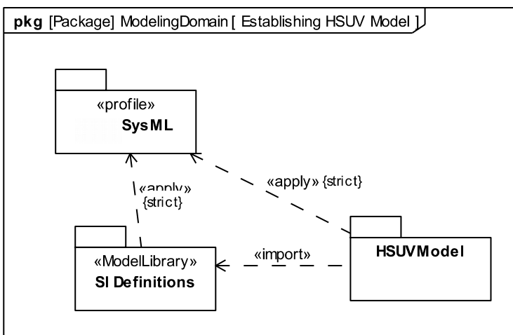
Figure 17.8 - A model with applied profile and imported model library
