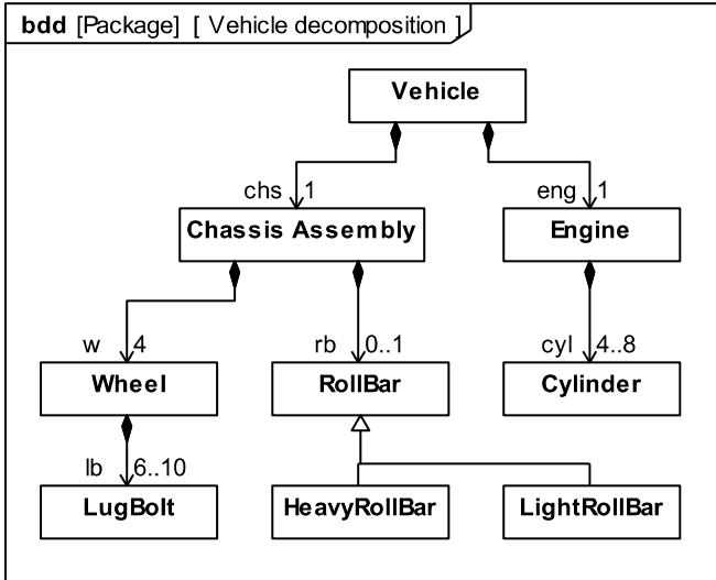
nested connector ends, because they link inside the parts of the vehicle. Figure 8.15: Vehicle Decomposition
