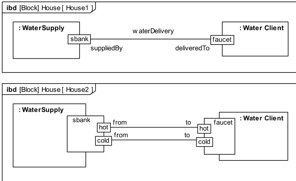
Figure 9.10 - Two views of Water Delivery connector within House block
