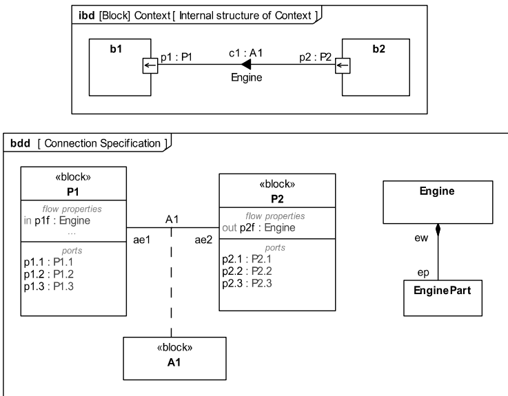
Figure 9.17 - Usage example of item flow decomposition
