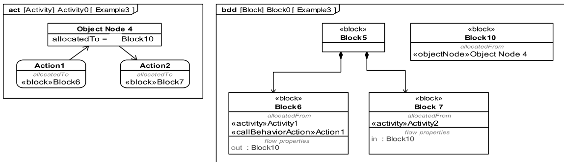
Figure 15.7 - Example of flow allocation from ObjectNode to FlowProperty
