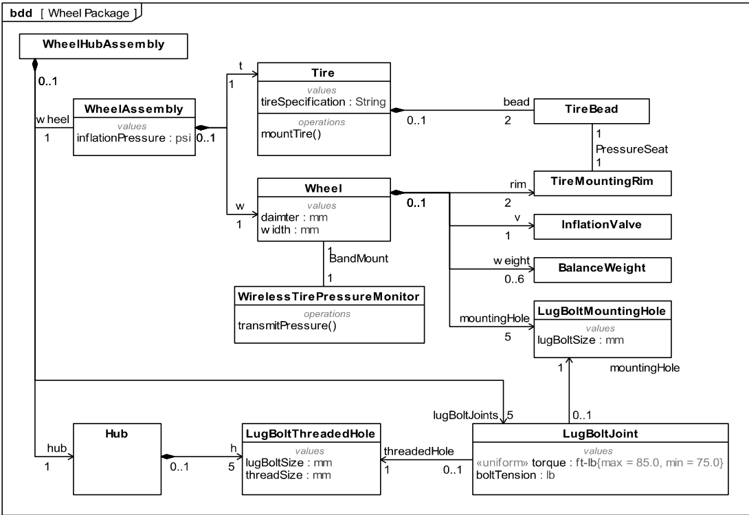
Figure 8.12: Block diagram for the Wheel Package
