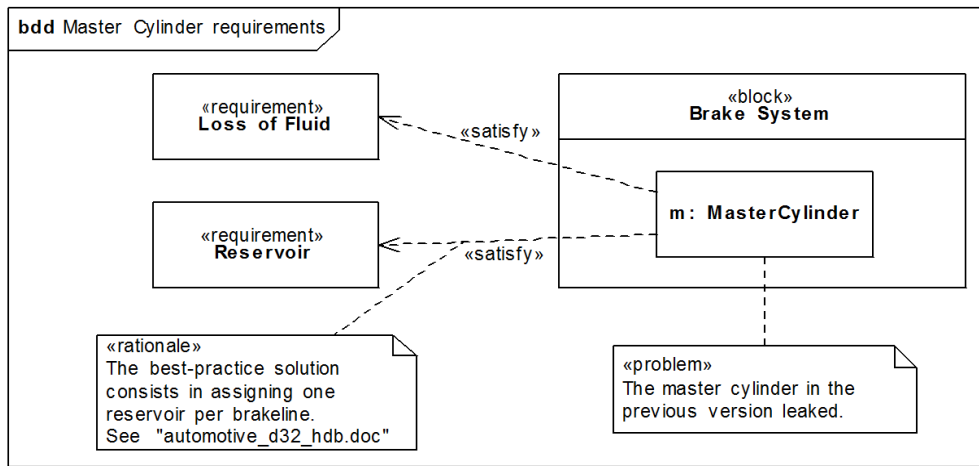
Figure 7.2: Rationale and Problem Example
