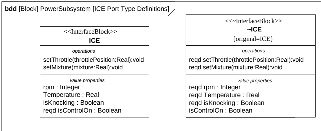
Figure D.20: Blocks Typing Ports in the Power Subsystem (Block Definition Diagram)
