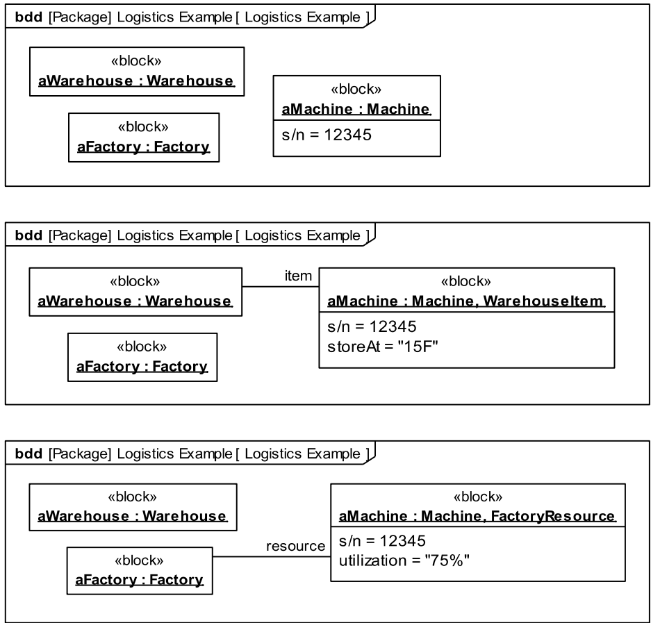
Figure 8.23 Changes in classification over time due to property-specific types
