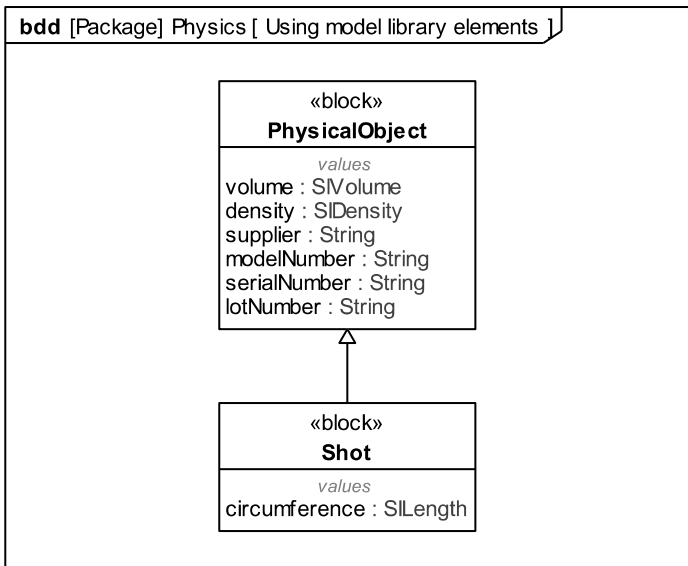
Figure 17.10 - Using model library elements
