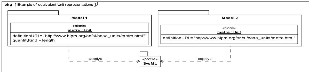
Figure 8.20 - Example of equivalent Unit representations
