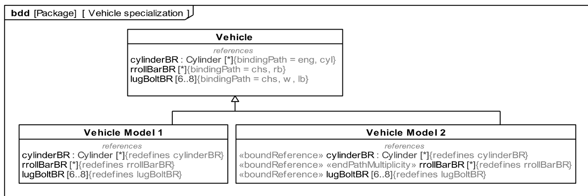
Figure 8.17: Vehicle specialization
