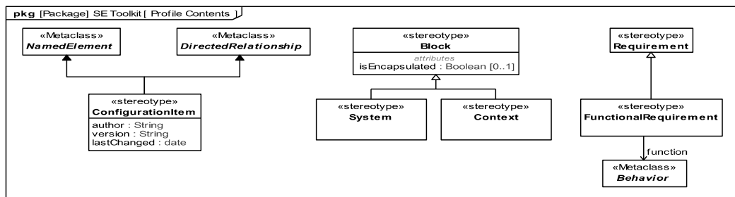
Figure 17.6 - Profile Contents
