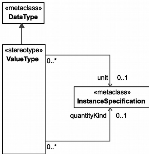
Figure 8.4: Abstract syntax extensions for SysML value types
