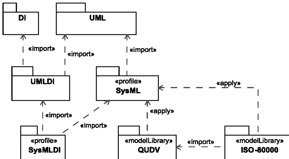
Figure 4.4: Non-normative Package Structure
