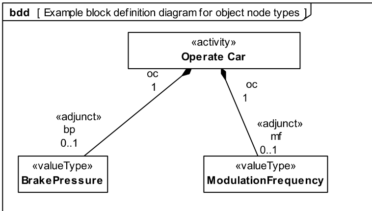
Figure 11.14 - Example block definition diagram for object node types
