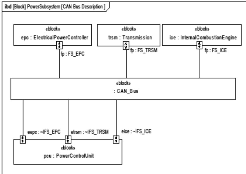
Figure D.22: Consolidating Connectors into the CAN Bus. (Internal Block Diagram)
