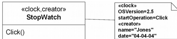
Figure 17.3 - Other notational forms for showing values
