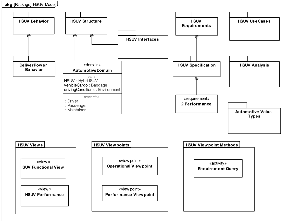
Figure D.3: Establishing Structure of the User Model using Packages and Views (Package Diagram)
