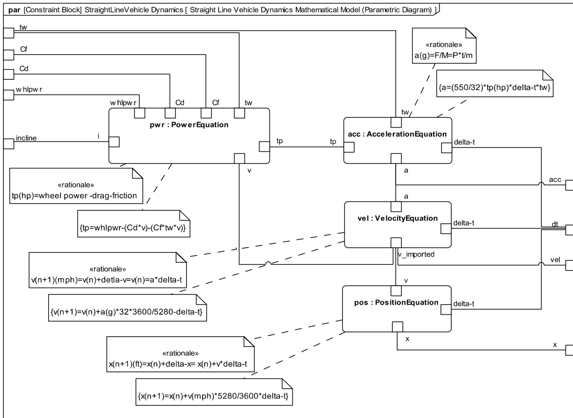
Figure D.33: Straight Line Vehicle Dynamics Mathematical Model (Parametric Diagram)
