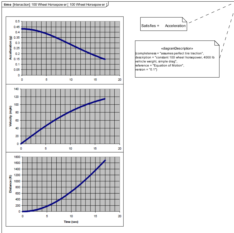
Figure D.35: Results of Maximum Acceleration Analysis (Timing Diagram)
