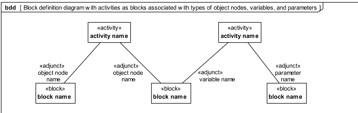
Figure 11.5 - Block definition diagram with activities as blocks associated with types of object nodes, variables, and parameter
