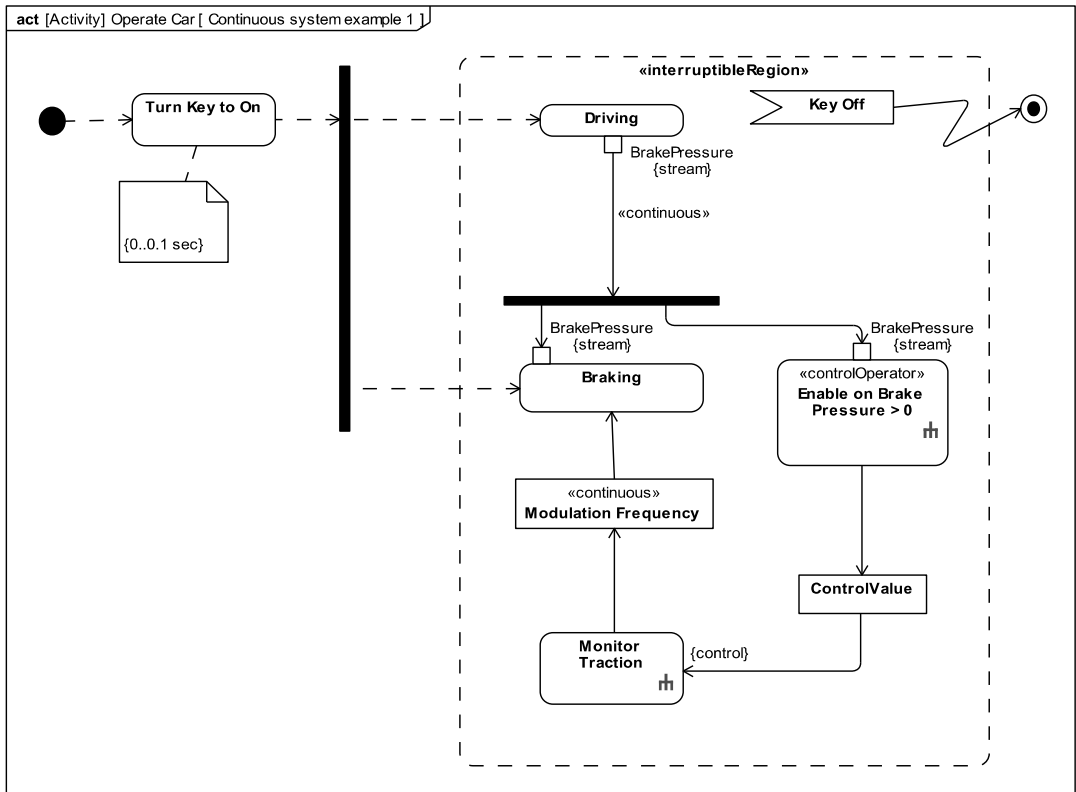
Figure 11.10 - Continuous system example 1
