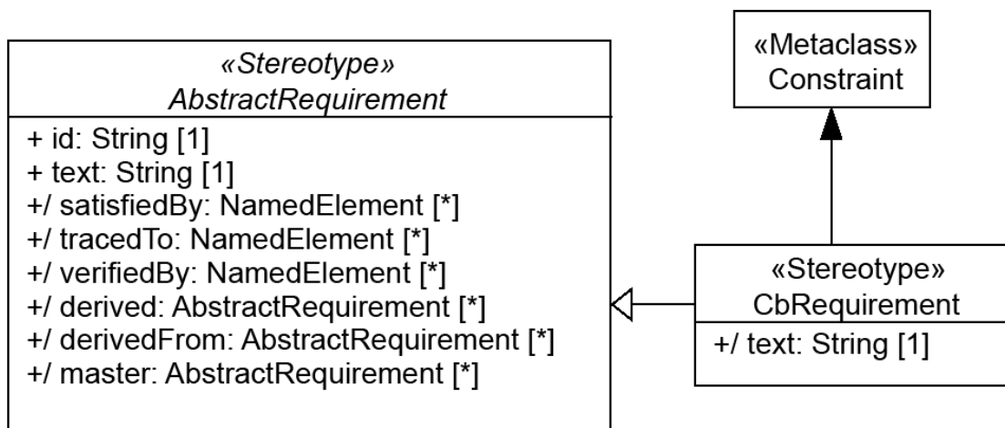
Figure E.27: Example of a PBR profile based on Constraints
