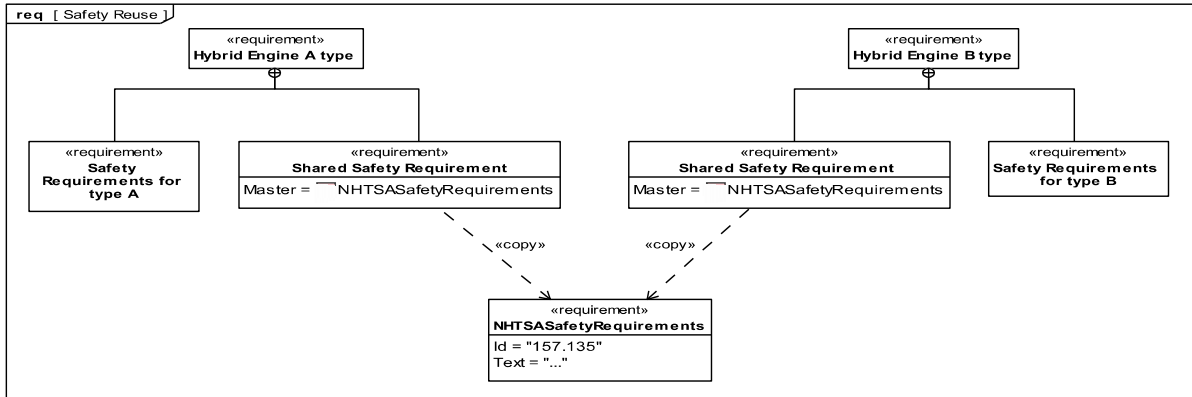
Figure 16.5 - Use of the copy dependency to facilitate reuse
