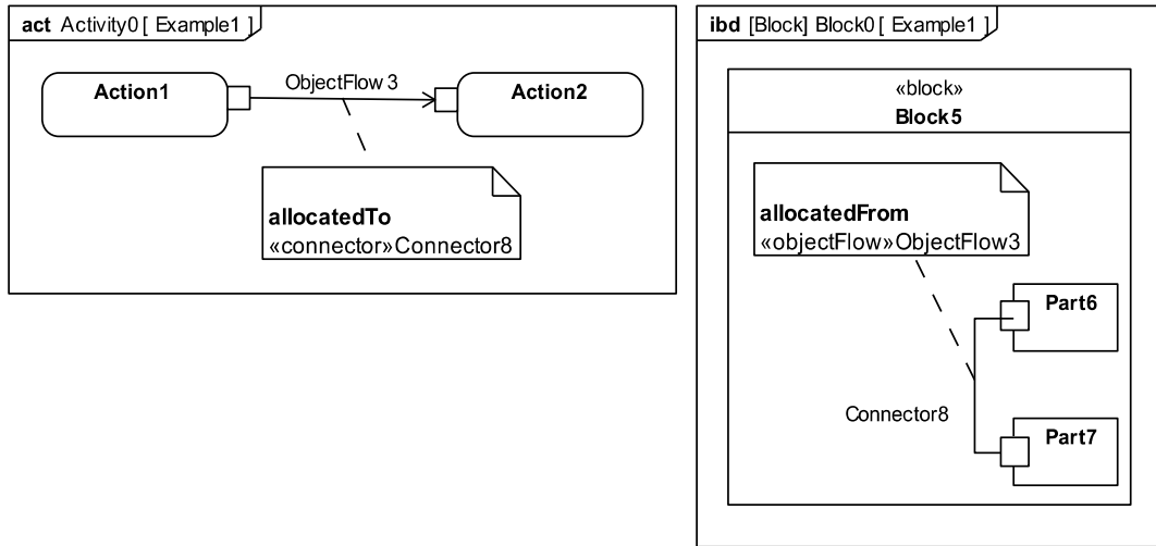
Figure 15.5 - Example of flow allocation from ObjectFlow to Connector
