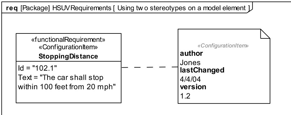
Figure 17.9 - Using two stereotypes on a model element
