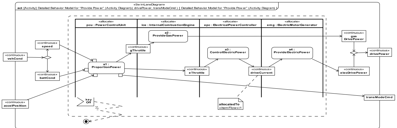
Figure D.38: Detailed Behavior Model for “Provide Power” (Activity Diagram)
