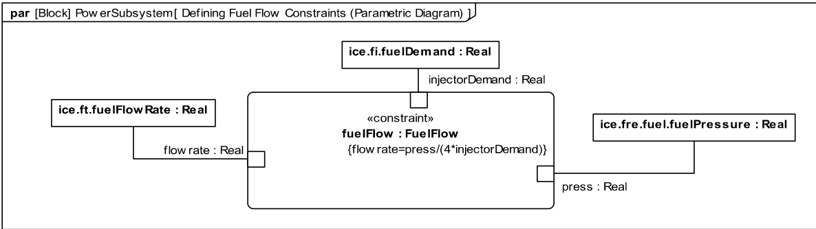
Figure D.24: Defining Fuel Flow Constraints (Parametric Diagram)
