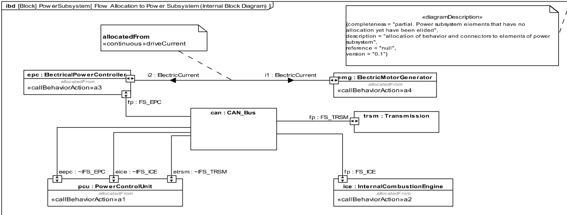
Figure D.39: Flow Allocation to Power Subsystem (Internal Block Diagram)
