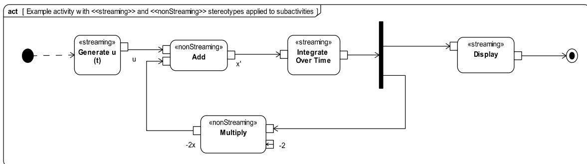
Figure E.2: Example activity with «streaming» and «nonStreaming» stereotypes applied to subactivities
