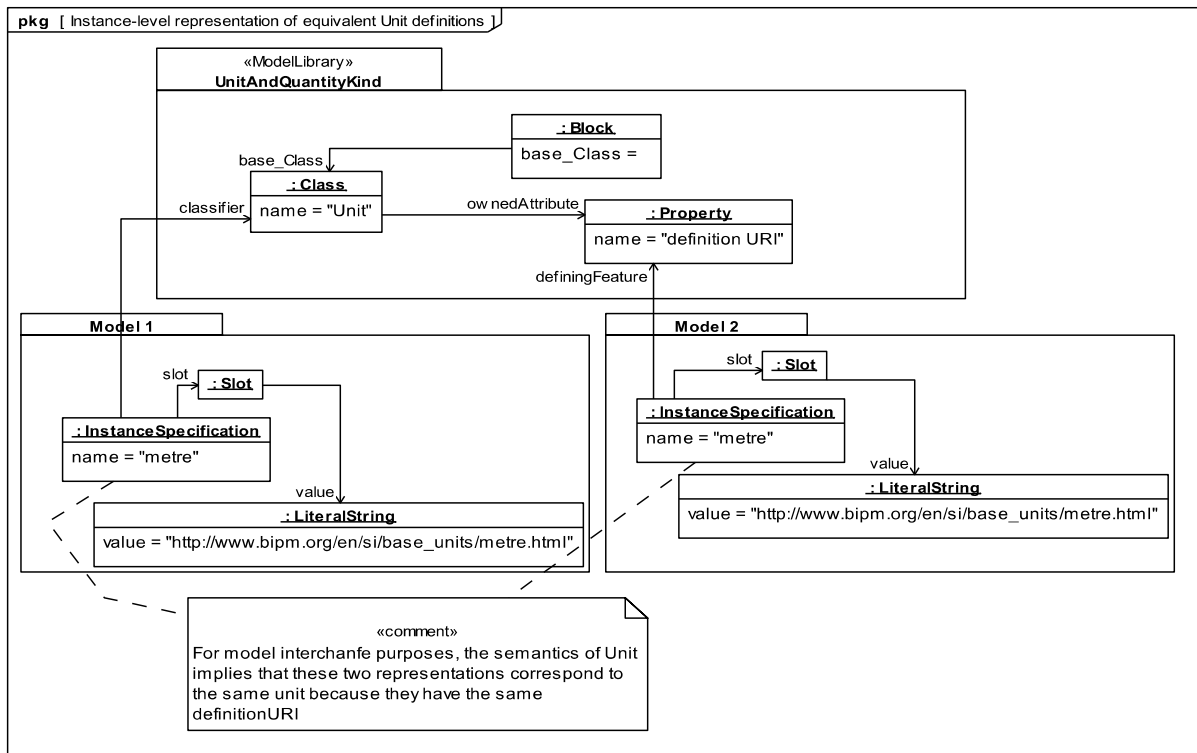
Figure 8.21 - Instance-level representation of equivalent Unit definitions
