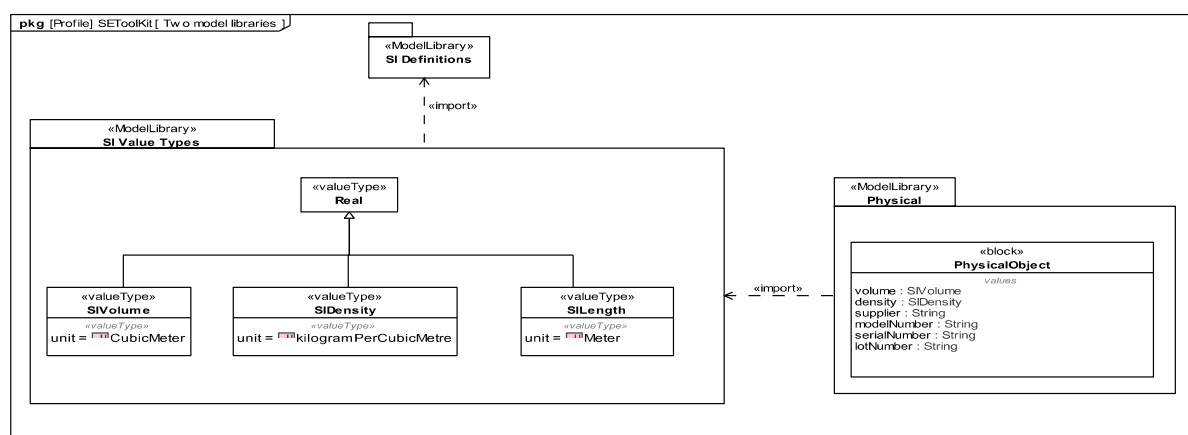
Figure 17.7 - Two model libraries
