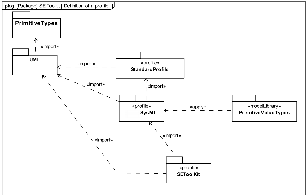
Figure 17.5 - Definition of a profile
