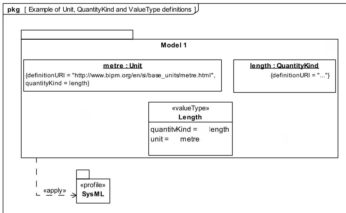
Figure 8.18: Example of Unit, QuantityKind and ValueType definitions
