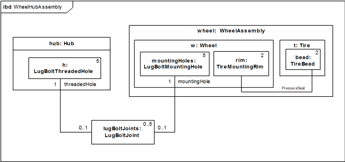
Figure 8.13: Internal Block Diagram for WheelHubAssembly
