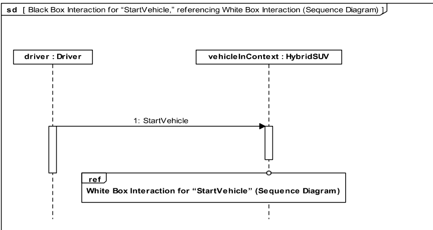
Figure D.9: Black Box Interaction for “StartVehicle,” referencing White Box Interaction (Sequence Diagram)
