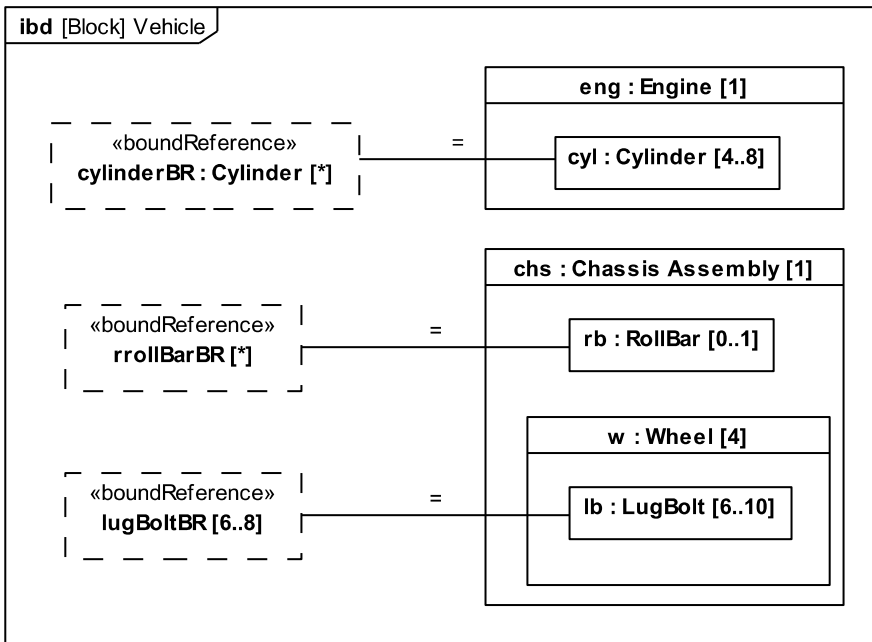
Figure 8.16: Vehicle internal structure
