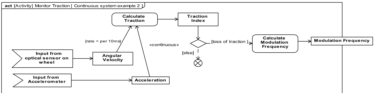
Figure 11.11 - Continuous system example 2
