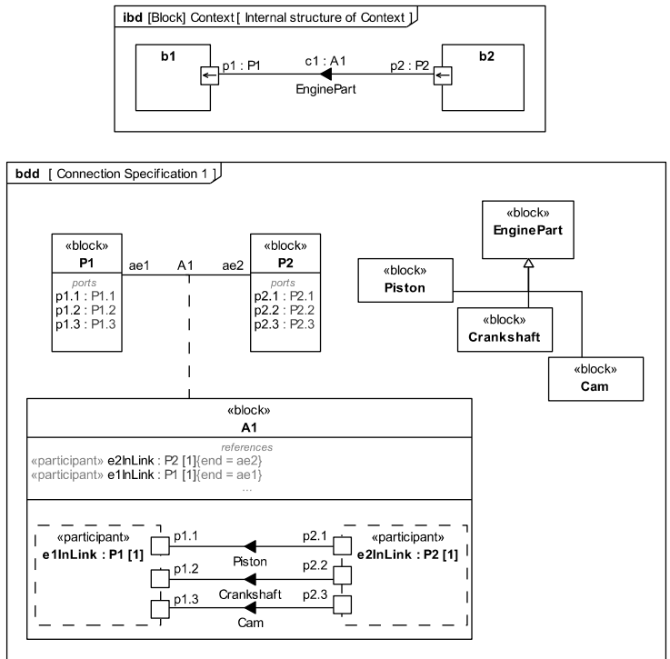
Figure 9.16 - Usage example of item flow decomposition
