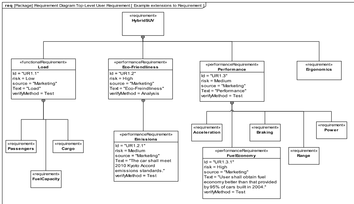
Figure E.3: Example extensions to Requirement
