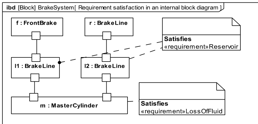
Figure 16.4 - Requirement satisfaction in an internal block diagram
