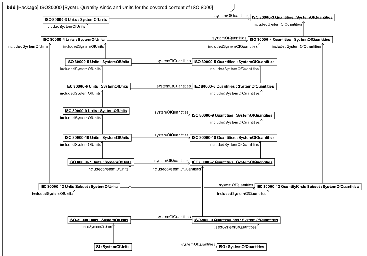
Figure E.13: Content relationships for the systems of units and quantities in from the different parts of ISO 80000 in relation to ISO 80000 as a whole and to the International System of Units (SI) and quantities (ISQ)
