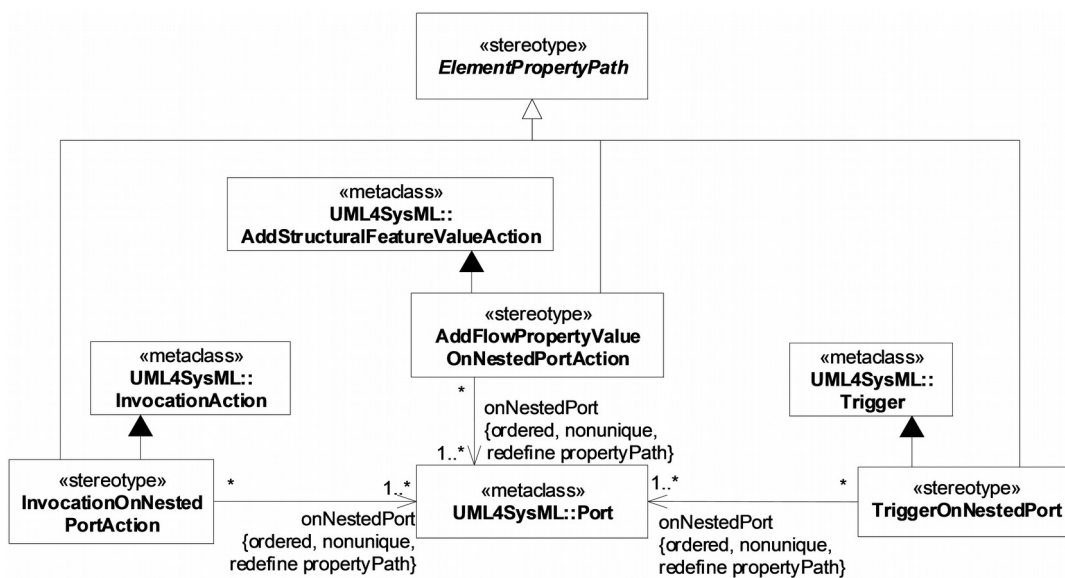
Figure 9.2 - Stereotypes for Actions on Nested Ports
