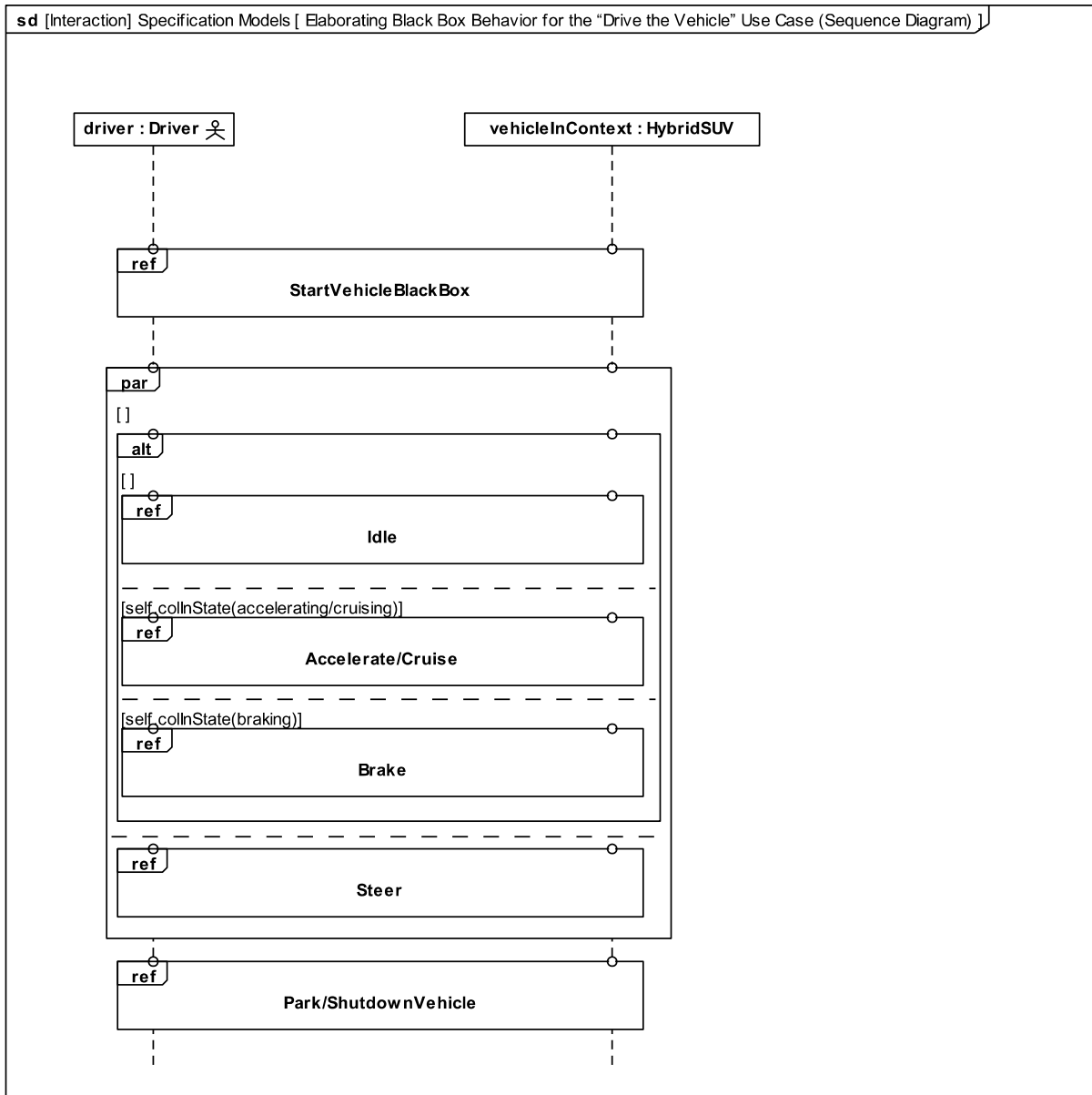
Figure D.7: Elaborating Black Box Behavior for the "Drive the Vehicle" Use Case (Sequence Diagram)
