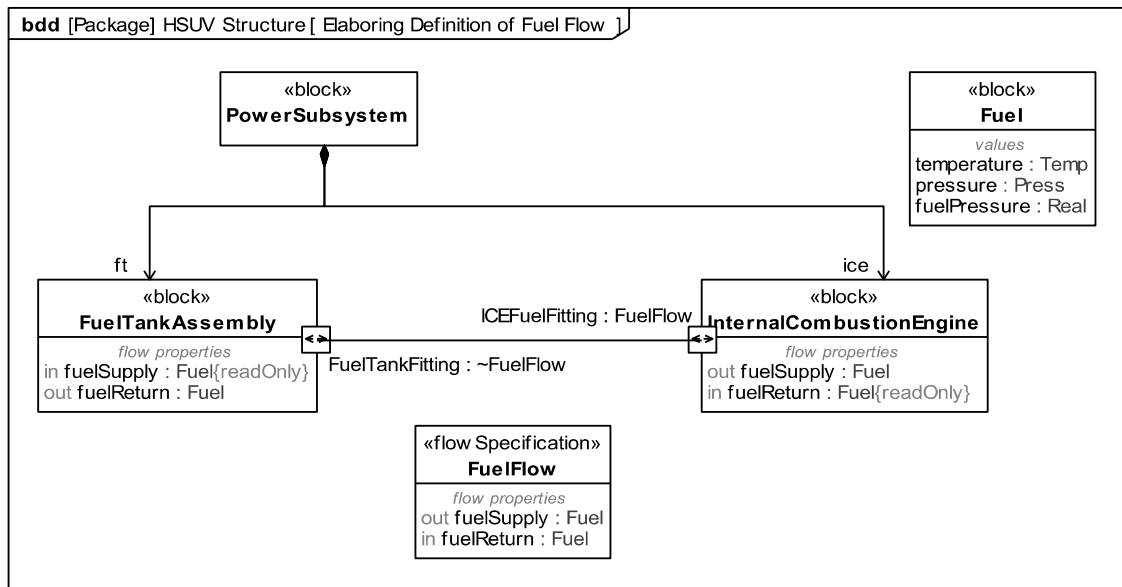
Figure D.23: Elaborating Definition of Fuel Flow. (Block Definition Diagram)
