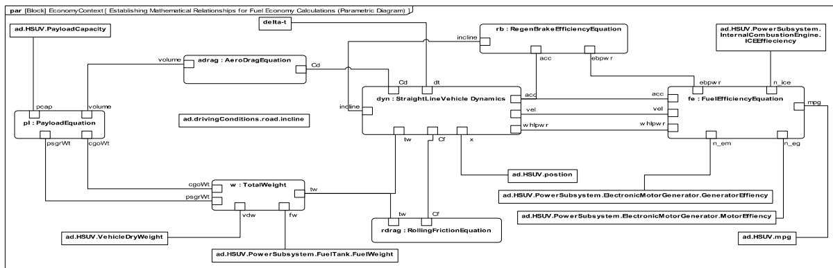
Figure D.32: Establishing Mathematical Relationships for Fuel Economy Calculations (Parametric Diagram)
