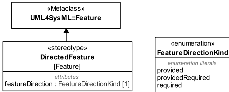
Figure 9.4 - Provided and Required Features
