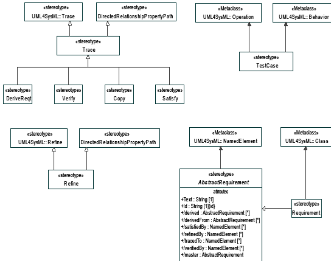
Figure 16.1 - Abstract Syntax for Requirements Stereotypes
