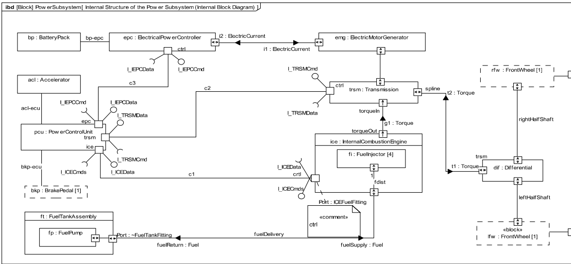
Figure D.19: Internal Structure of the Power Subsystem (Internal Block Diagram)
