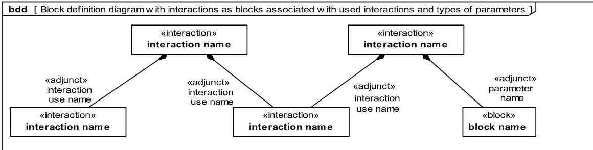
Figure 12.1 - Block definition diagram with interactions as blocks associated with used interactions and types of parameters
