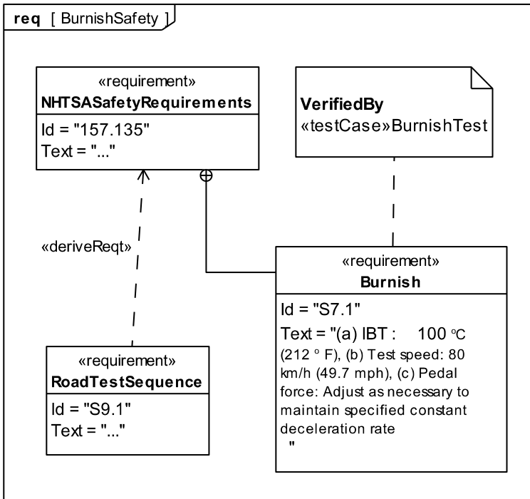
Figure 16.6 - Linkage of a Test Case to a requirement: This figure shows the Requirement Diagram
