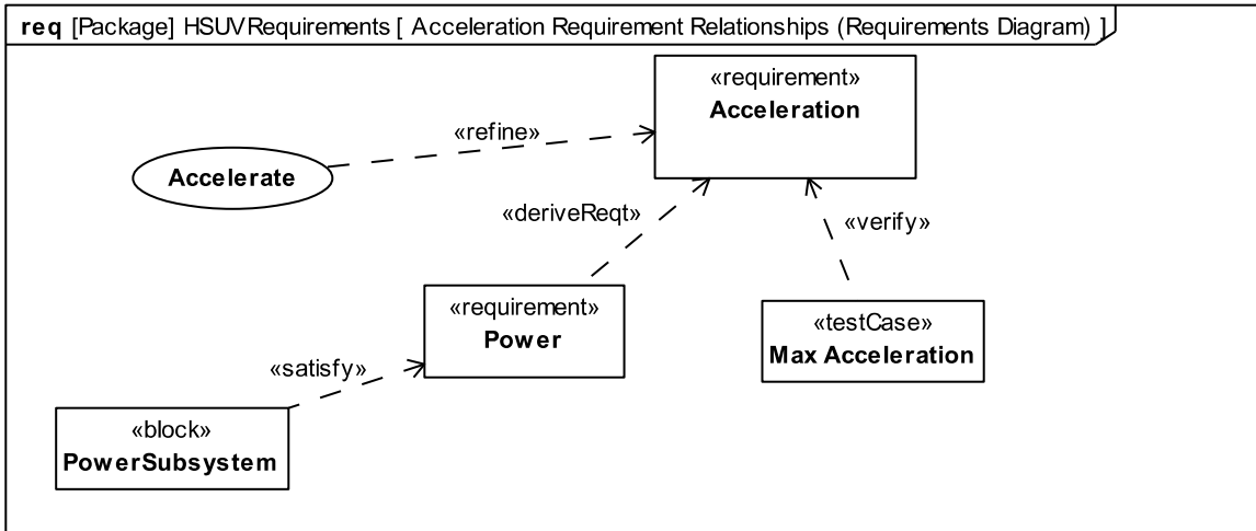
Figure D.13: Acceleration Requirement Relationships (Requirements Diagram)
