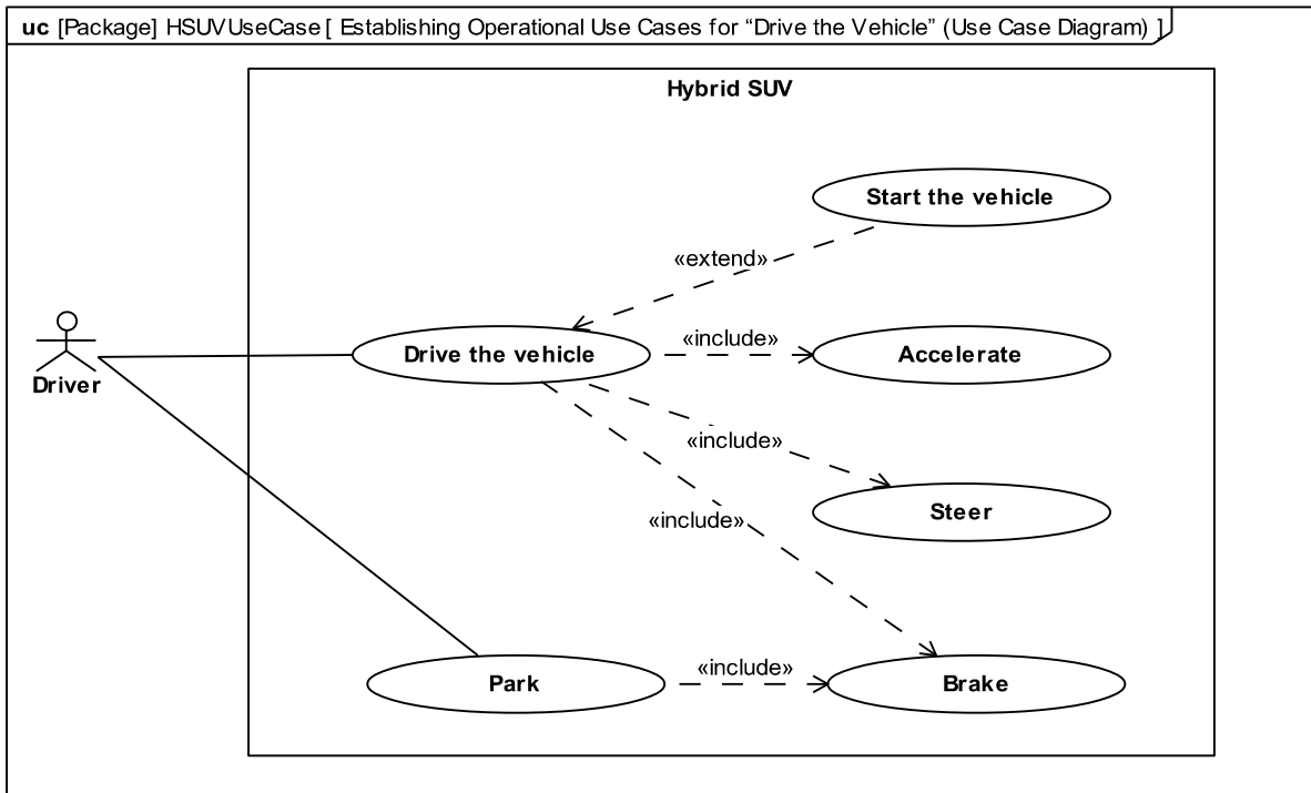
Figure D.6: Establishing Operational Use Cases for “Drive the Vehicle” (Use Case Diagram)
