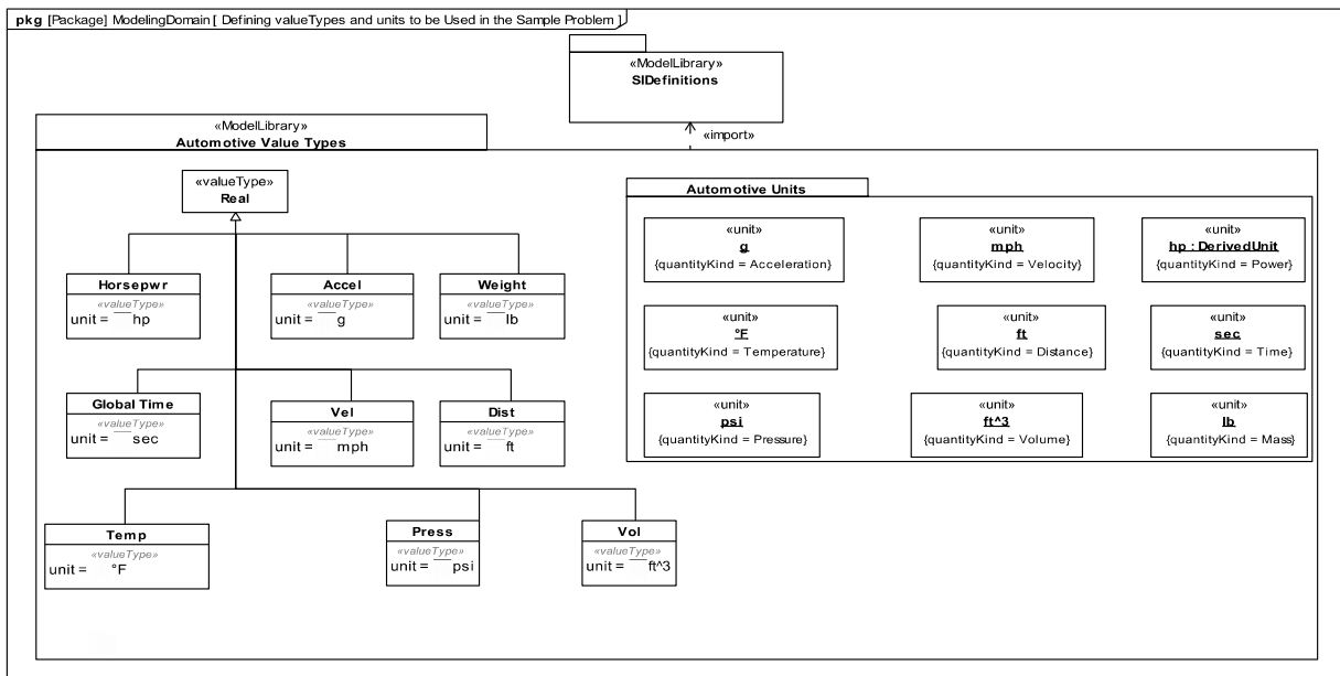
Figure D.2: Defining value Types and units to be used in the Sample Problem
