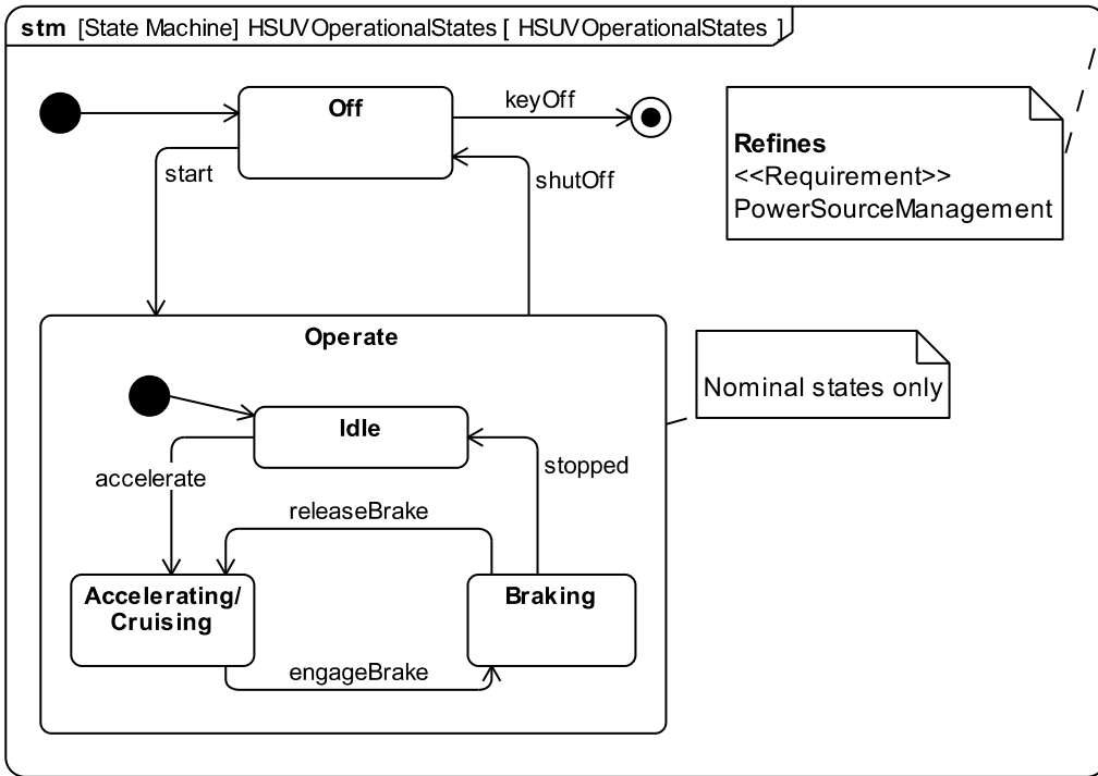
Figure D.8: Finite State Machine Associated with “Drive the Vehicle” (State Machine Diagram)
