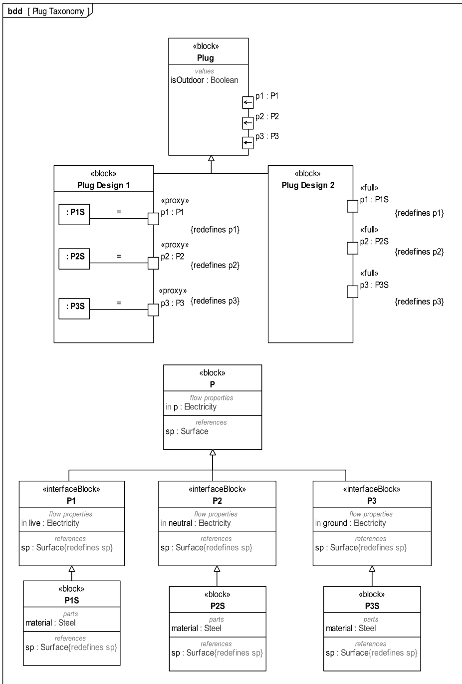
Figure 9.7 - Usage example of proxy and full ports
