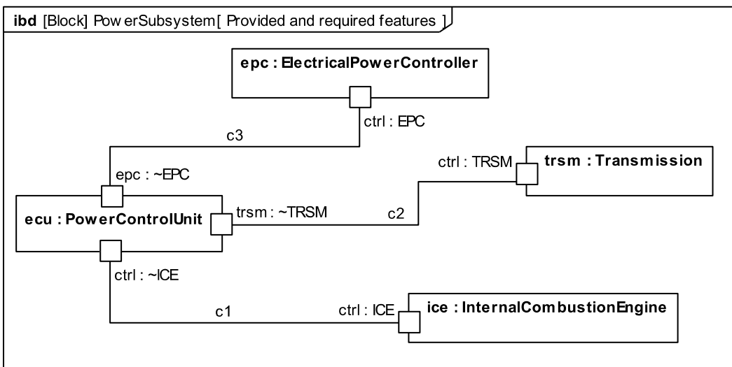
Figure 9.6 - Usage example of ports with provided and required features
