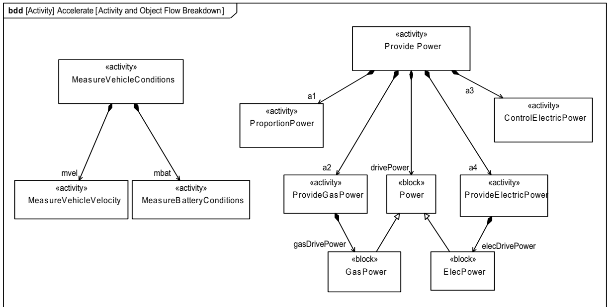
Figure D.37 - Decomposition of “Accelerate” Function (Block Definition diagram)
