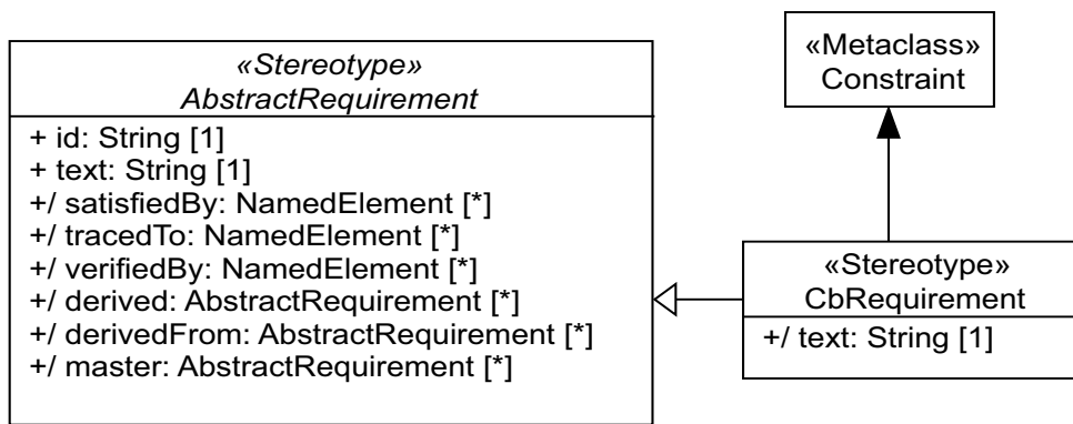
Figure E.27 - Example of a PBR profile based on Constraints
