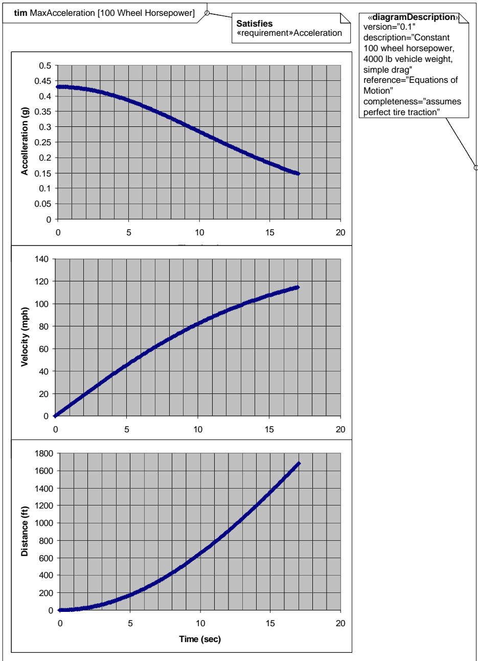
Figure D.35 - Results of Maximum Acceleration Analysis (Timing Diagram)
