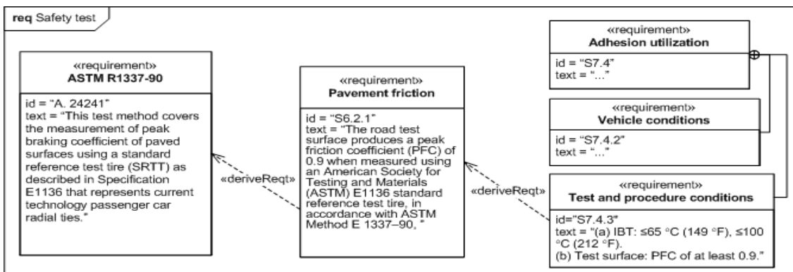
Figure 16.2 - Requirements Derivation
