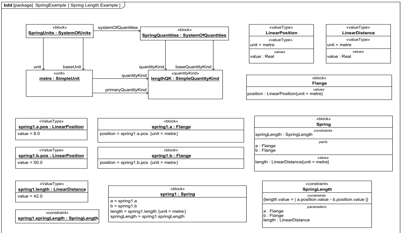
Figure E.10 - Spring Length Example
