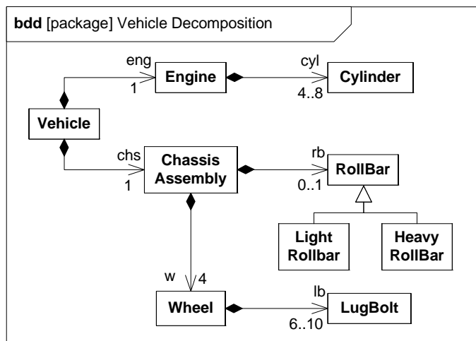
Figure 8.15 - Vehicle decomposition
