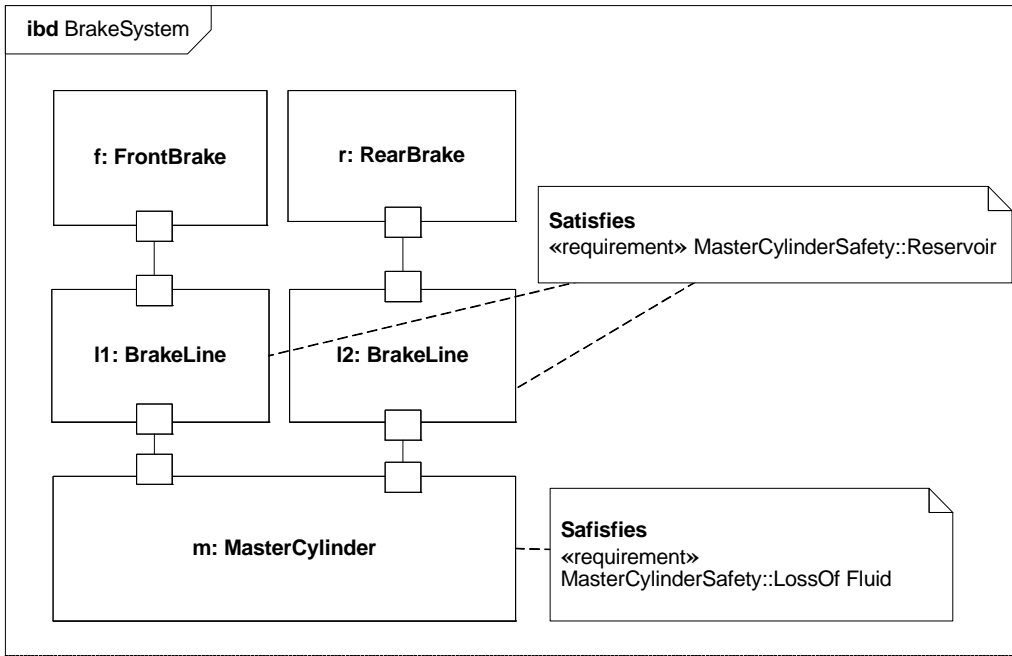
Figure 16.4 - Requirement satisfaction in an internal block diagram
