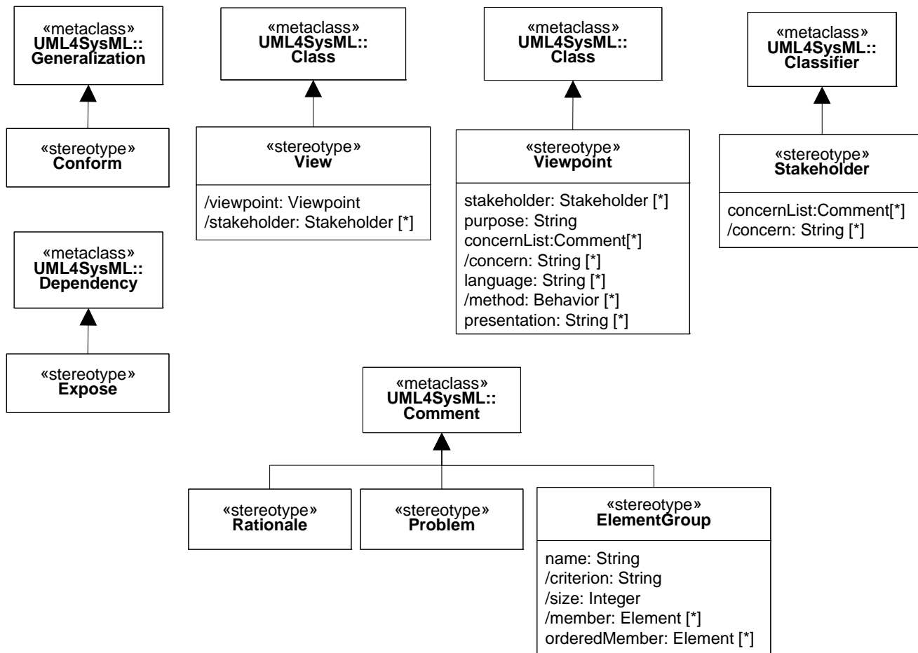
Figure 7.1 - Stereotypes defined in package ModelElements
