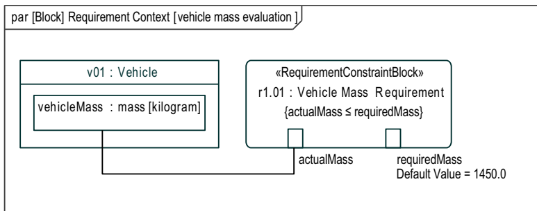
Figure E.26 - Example of Parametric Diagram Using PBR based on Constraint Block
