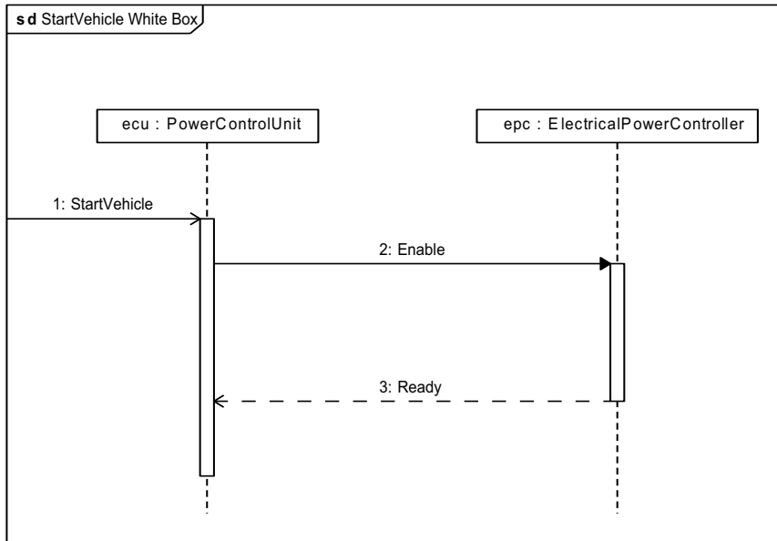
Figure D.10 - White Box Interaction for “StartVehicle” (Sequence Diagram)
