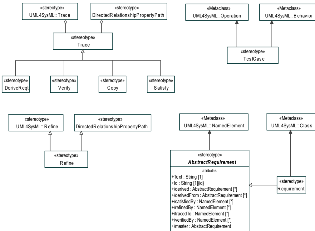
Figure 16.1 - Abstract Syntax for Requirements Stereotypes
