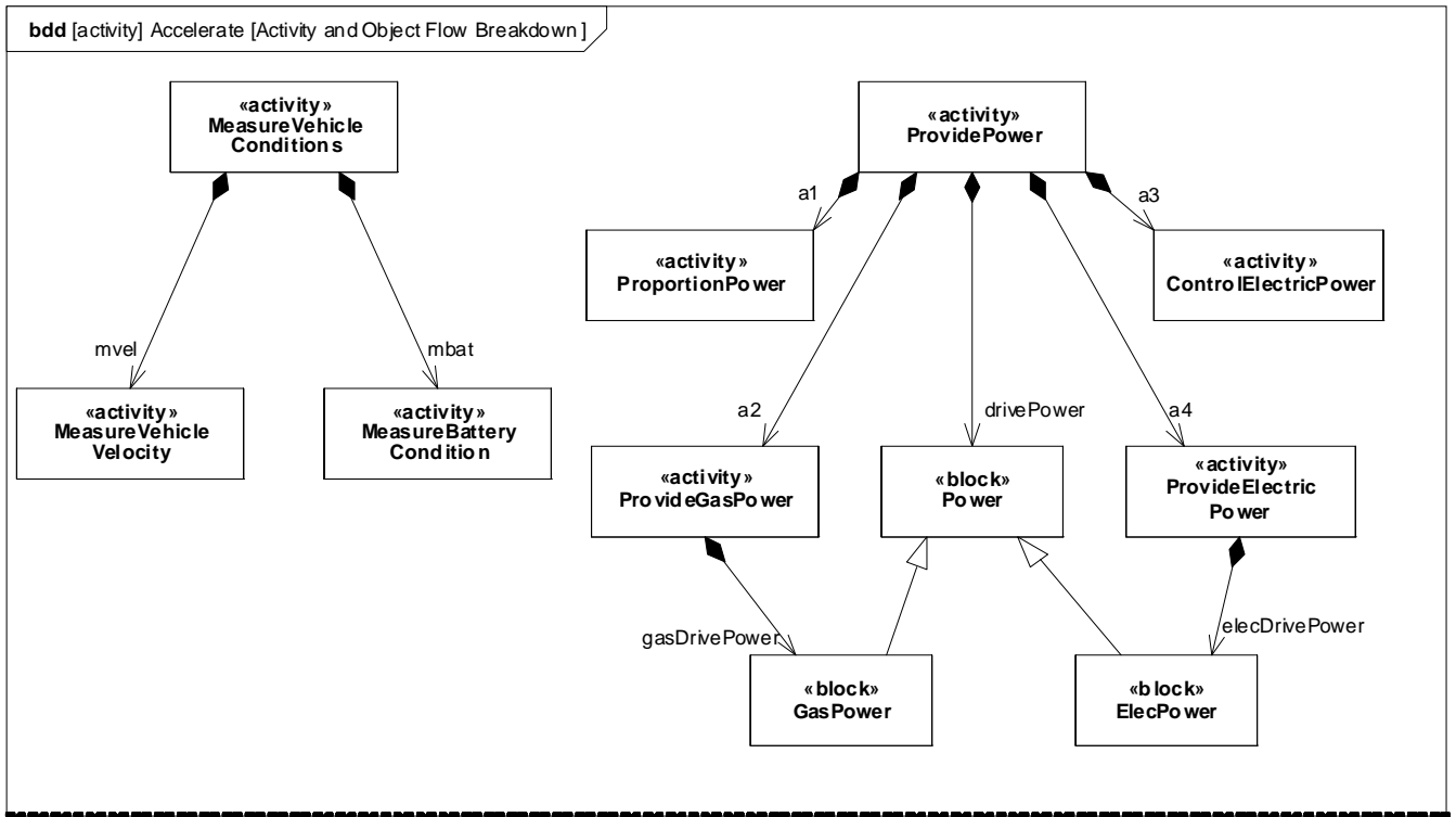
Figure D.37 - Decomposition of “Accelerate” Function (Block Definition diagram)
