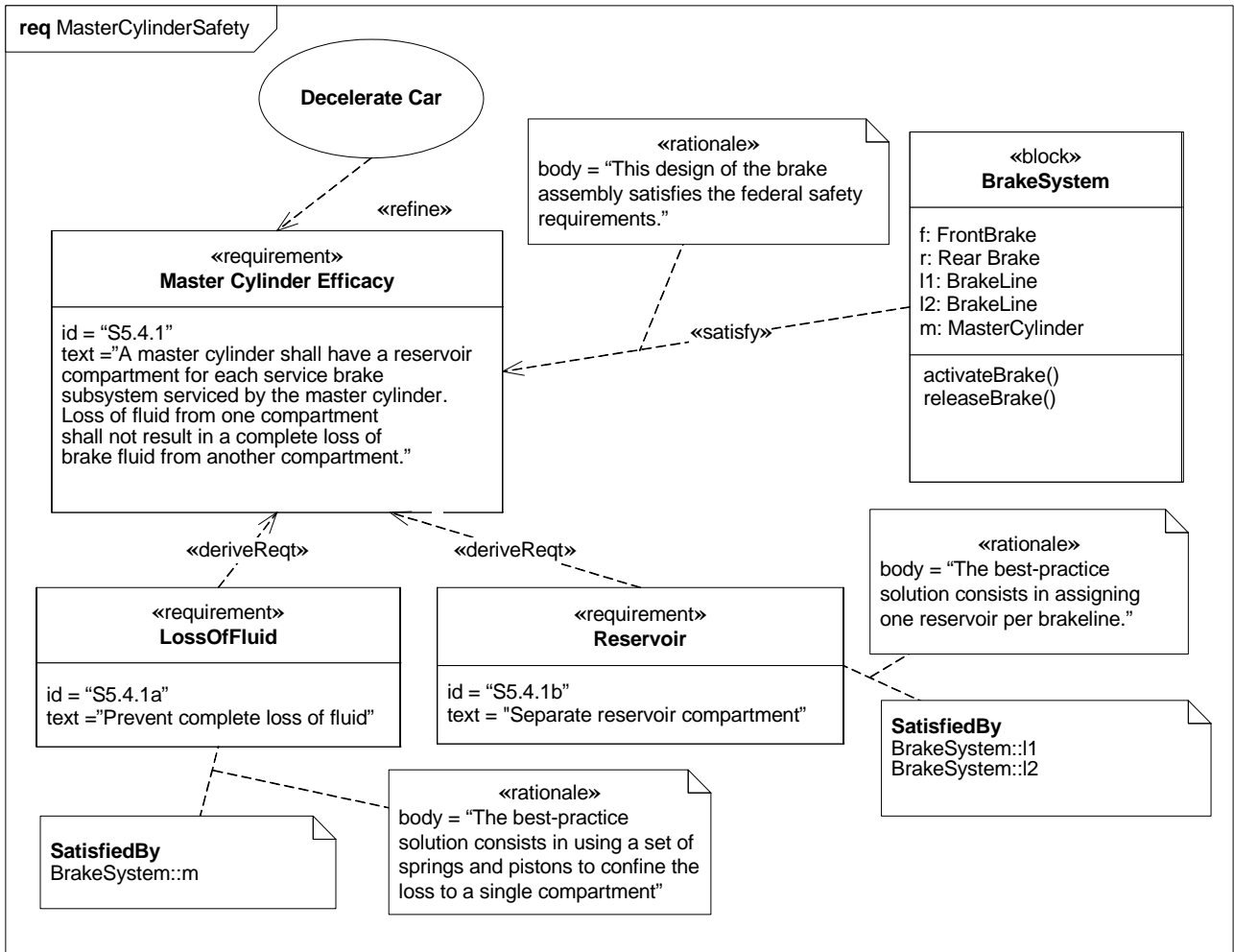
Figure 16.3 - Links between requirements and design
