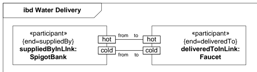
Figure 9.9 - Internal structure of Water Delivery association block
