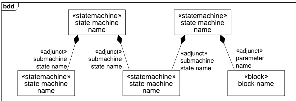
Figure 11.1 - Block definition diagram with state machines as blocks associated with submachines and types of parameters
