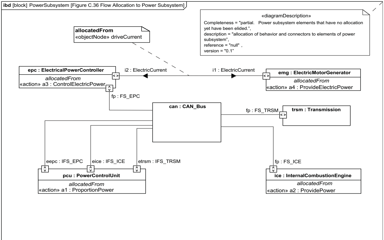
Figure D.39 - Flow Allocation to Power Subsystem (Internal Block Diagram)
