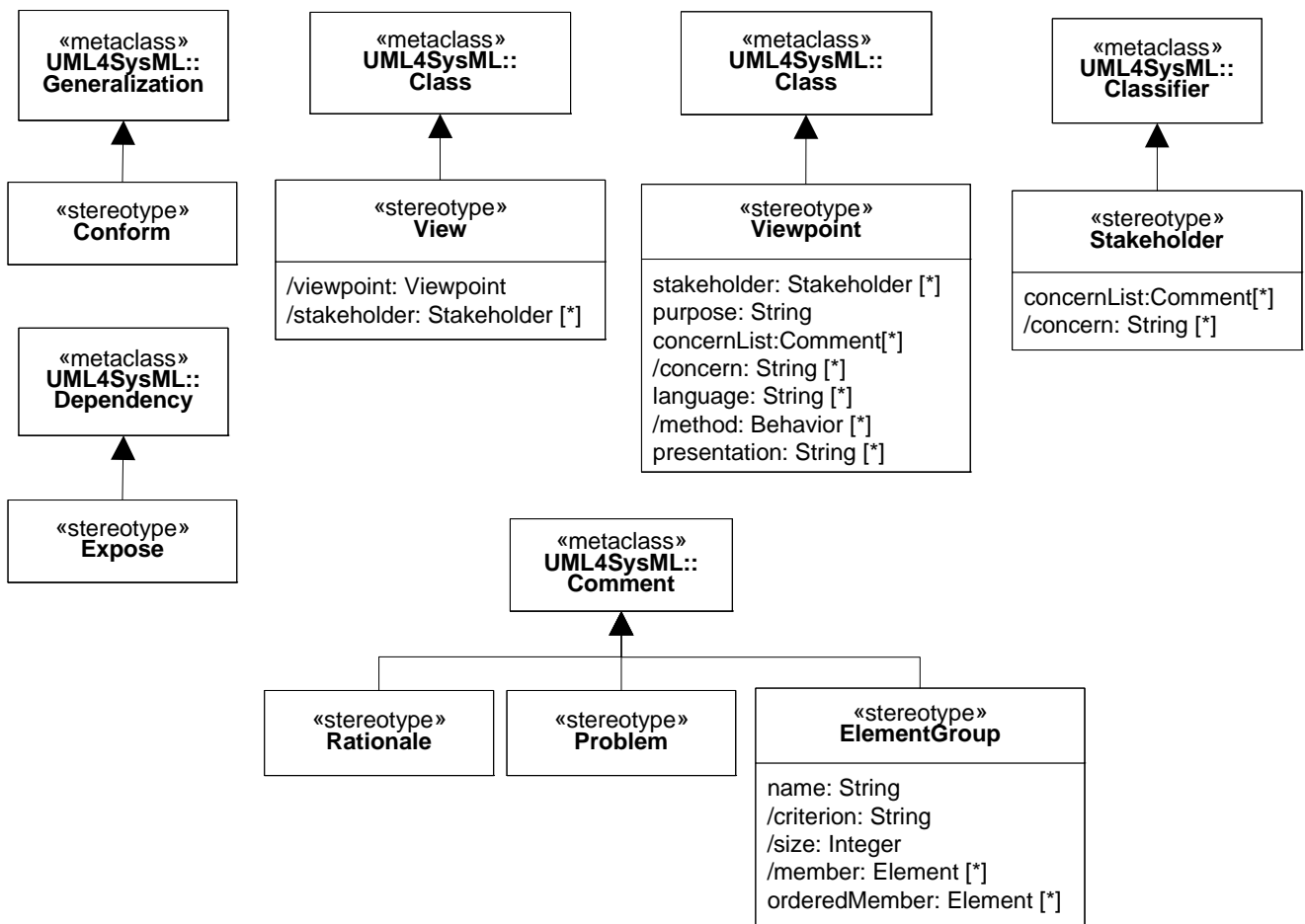
Figure 8.1 - Stereotypes defined in package ModelElements
