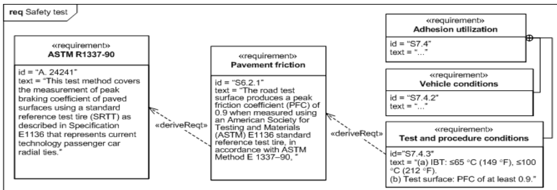
Figure 16.2 - Requirements Derivation
