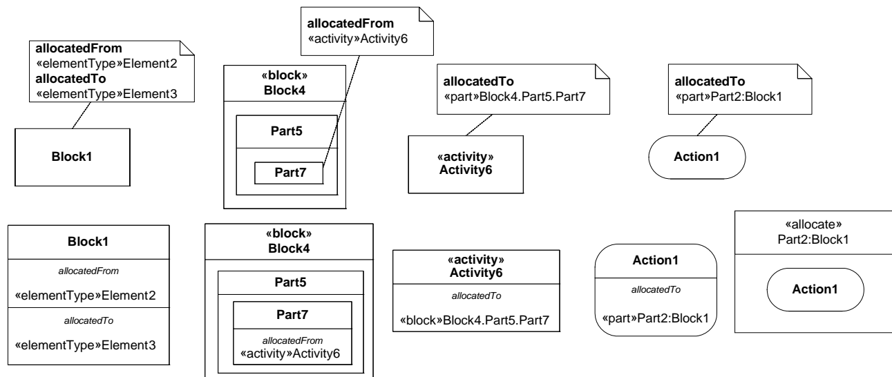
Figure 15.4 - Behavior allocation
