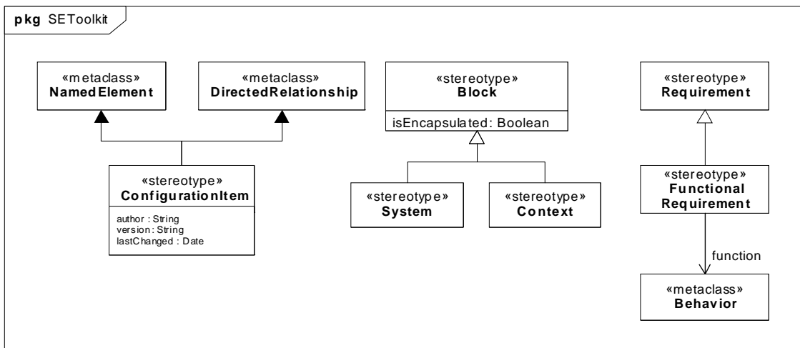
Figure 17.5 - Profile Contents
