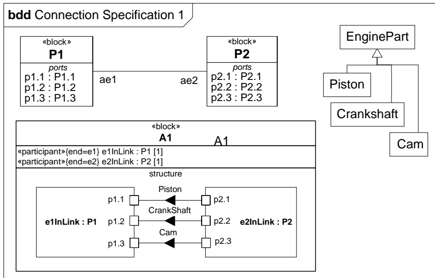
Figure 9.16 - Usage example of item flow decomposition
