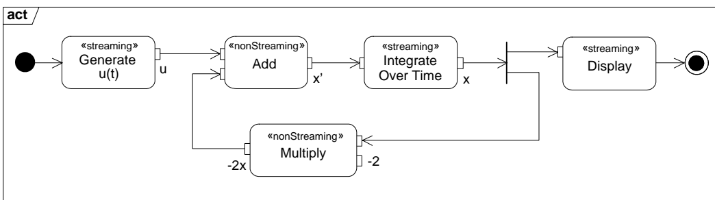
Figure C.2- Example activity with «streaming» and «nonStreaming» stereotypes applied to subactivities
