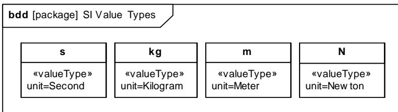
Figure 8.10 - Defining Value Types with units of measure from the International System of Units (SI)
