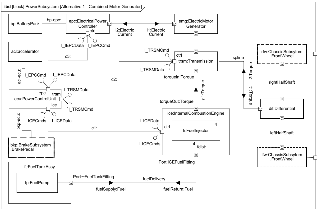
Figure B.19 - Internal Structure of the Power Subsystem (Internal Block Diagram)
