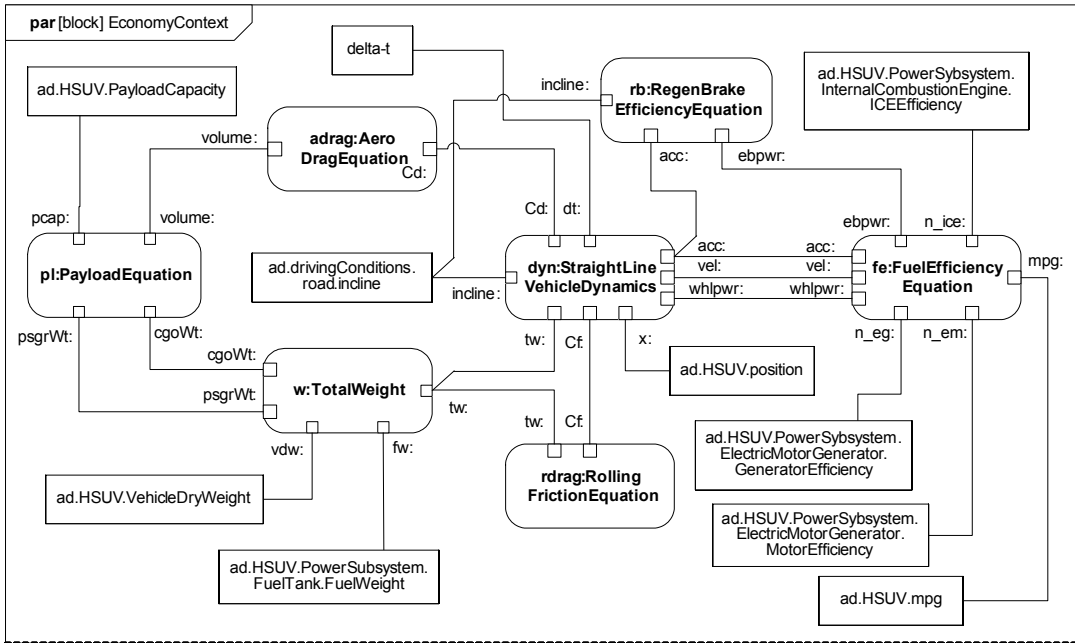
Figure 10.3 -Usage of constraint blocks on a parametric diagram
