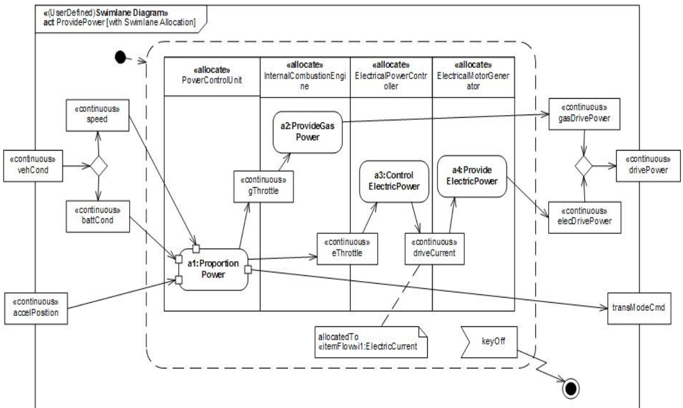
Figure 15.9 - AllocateActivityPartitions (Swimlanes) for HybridSUV Accelerate Example
