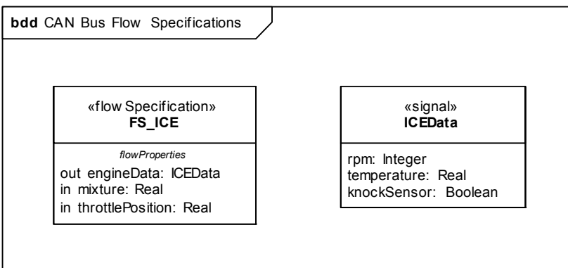
Figure 9.7 - Flow specification for the InternalCombustionEngine flow port to allow its connection over the CAN bus
