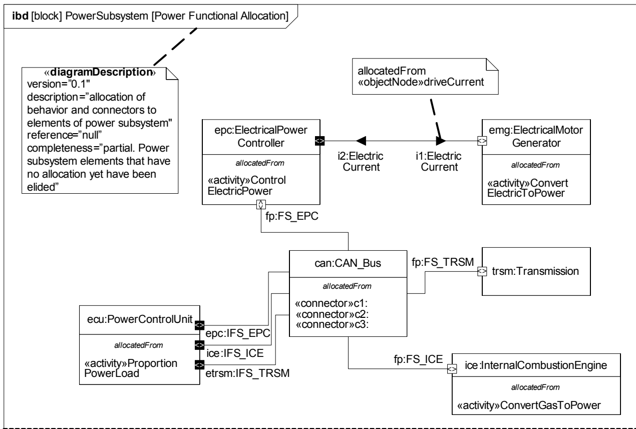
Figure B.36 - Flow Allocation to Power Subsystem (Internal Block Diagram)
