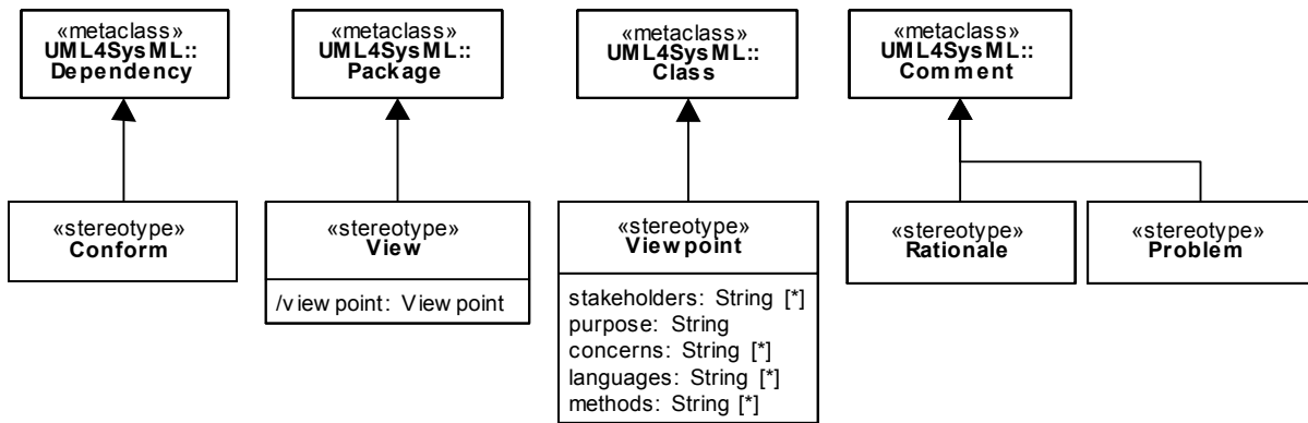
Figure 7.2 - Stereotypes defined in package ModelElements
