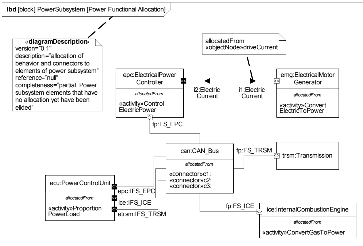
Figure 15.10 - Internal Block Diagram Showing Allocation for HybridSUV Accelerate Example
