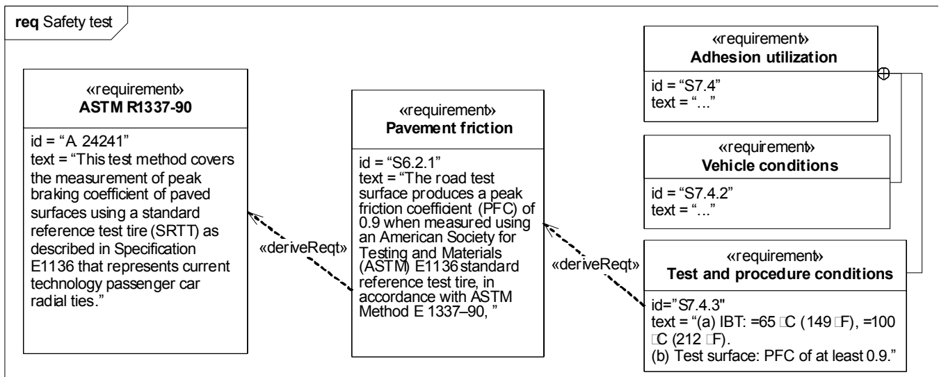
Figure 16.3 - Requirements Derivation
