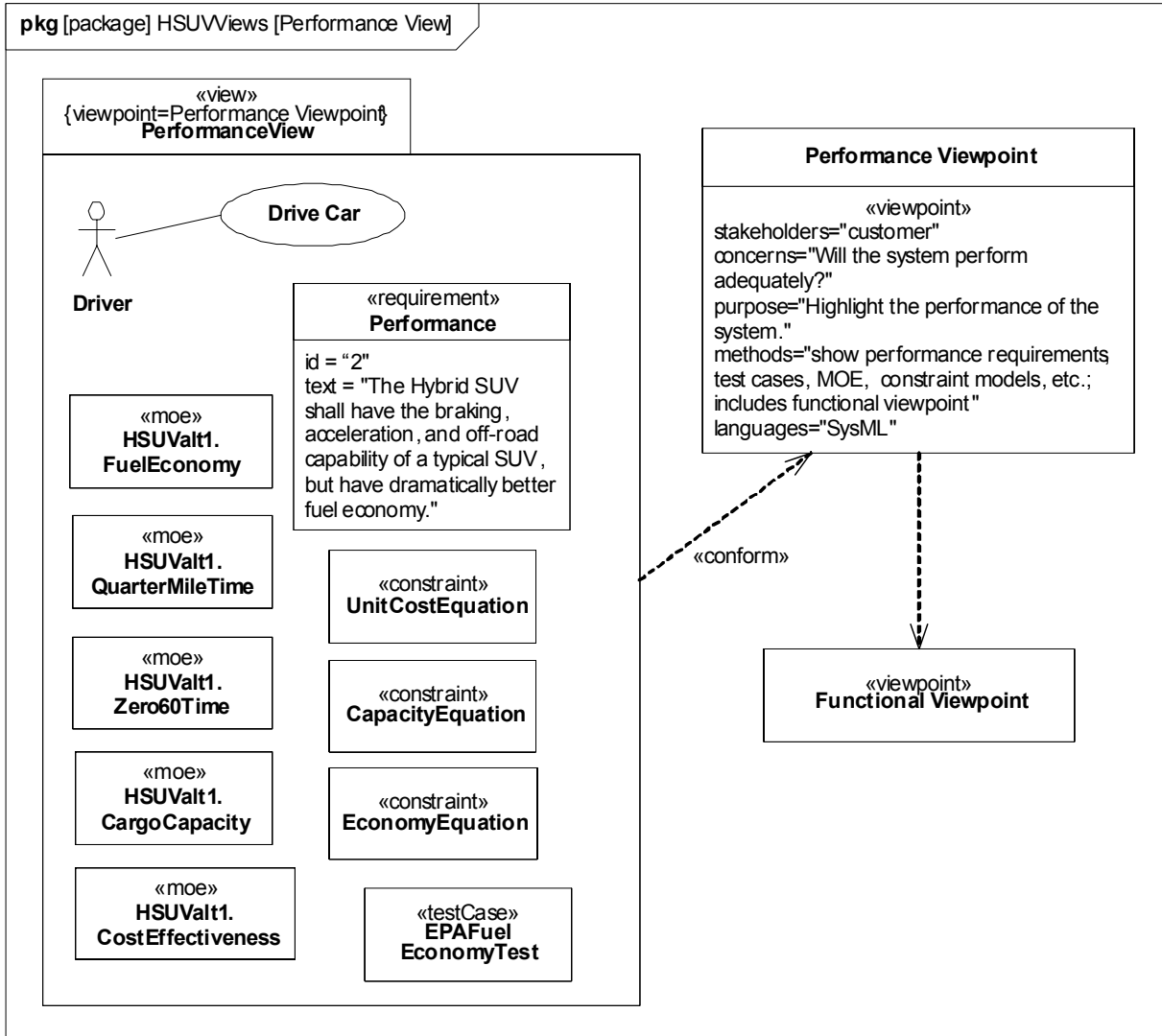
Figure 7.3 - View/Viewpoint example
