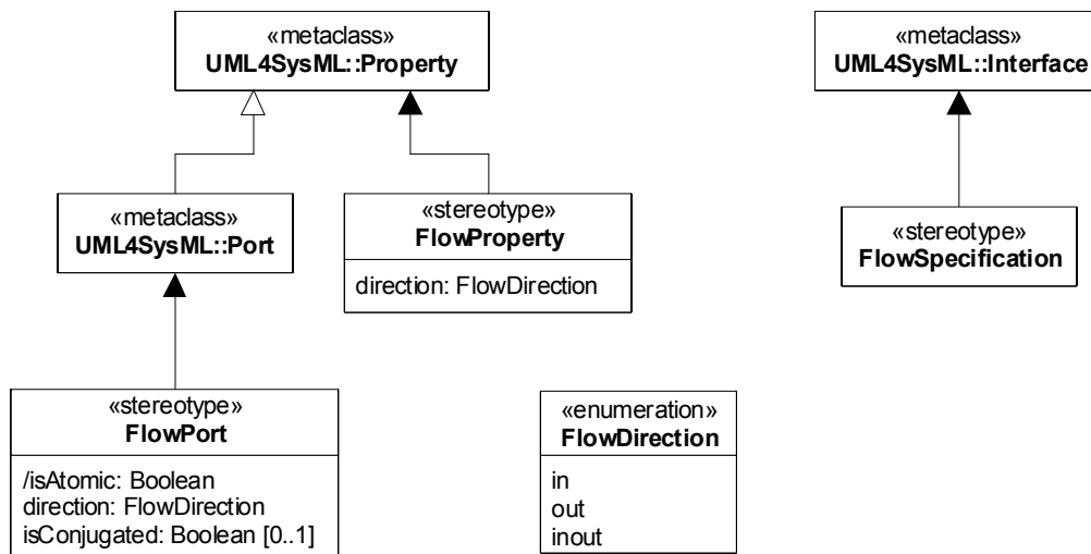
Figure 9.1 - Port Stereotypes
