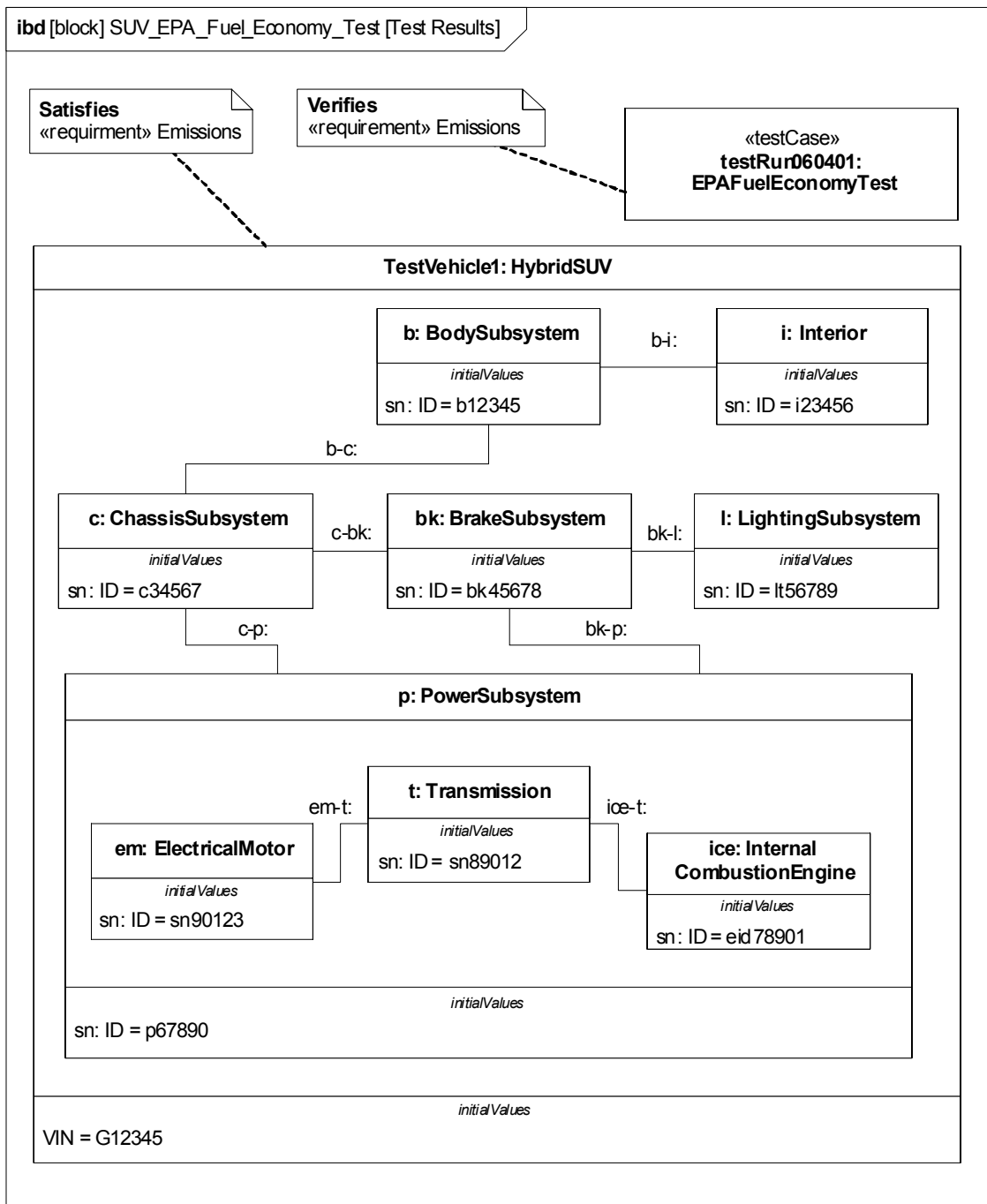
Figure 8.11 - SUV EPA Fuel Economy Test
