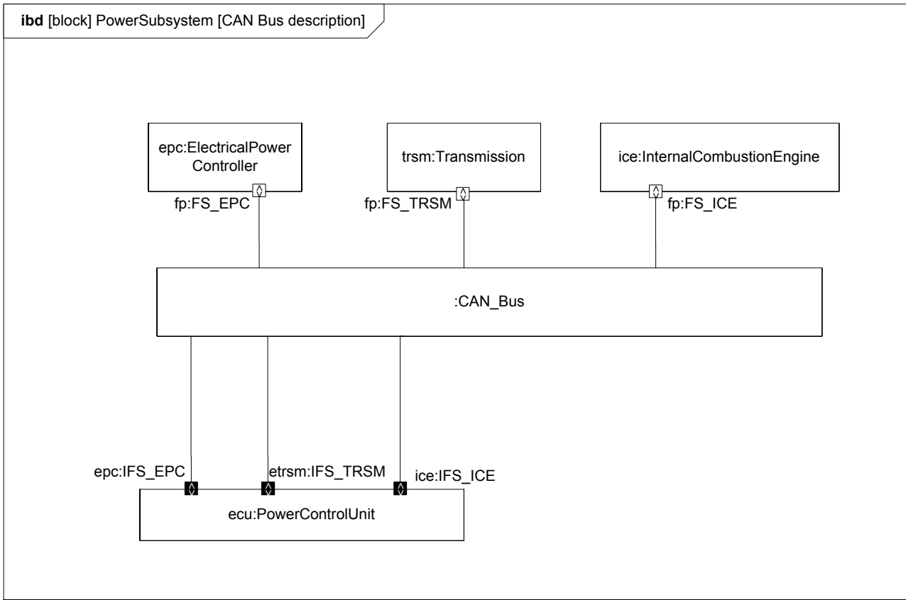
Figure 9.6 - Using flow ports to connect the PowerControlUnit to the ElectricalPowerController, Transmission, and InternalCombustionEngine over a CAN bus
