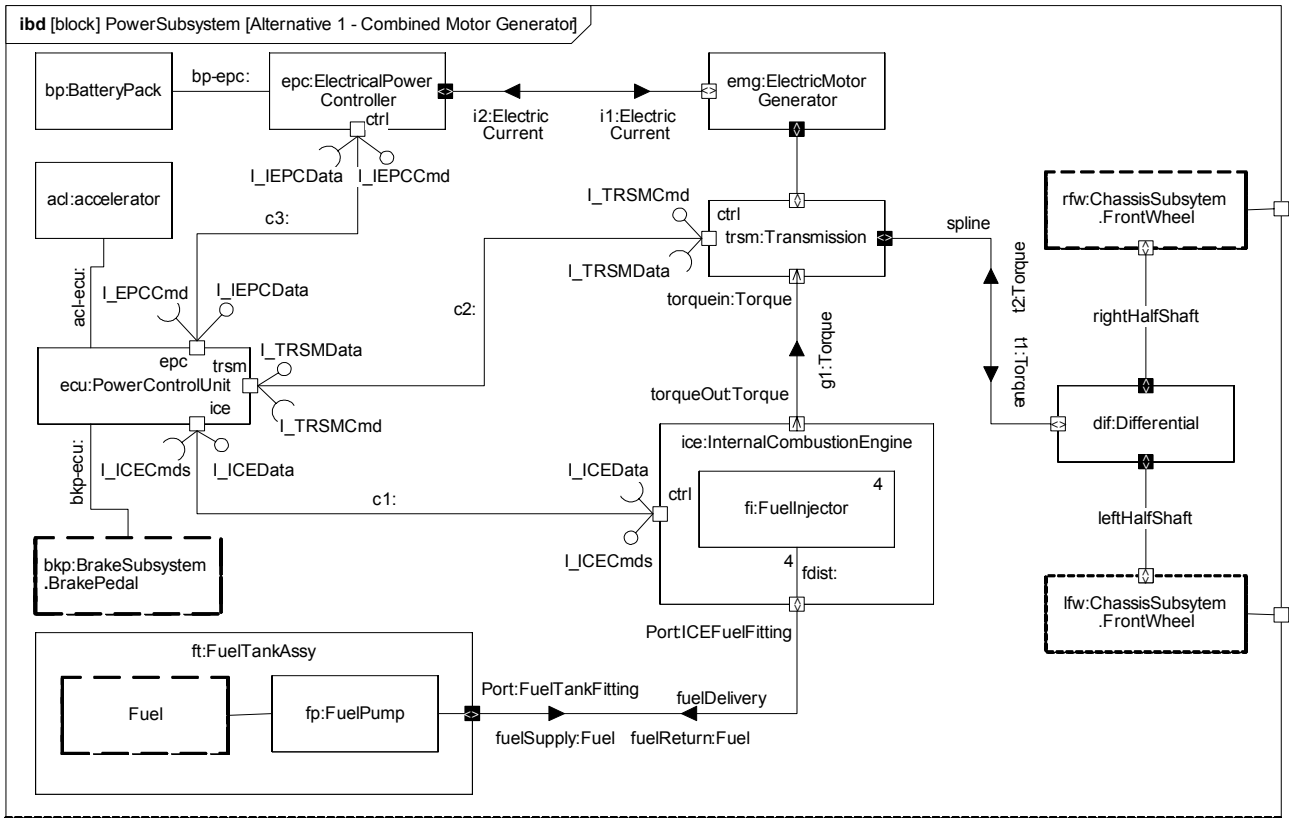
Figure B.19 - Internal Structure of the Power Subsystem (Internal Block Diagram)
