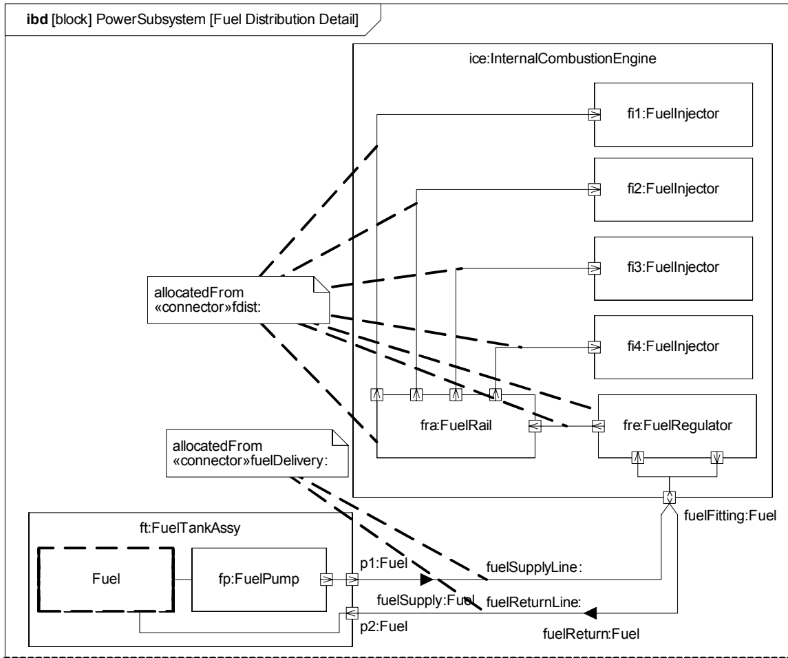
Figure B.25 - Detailed Internal Structure of Fuel Delivery Subsystem (Internal Block Diagram)
