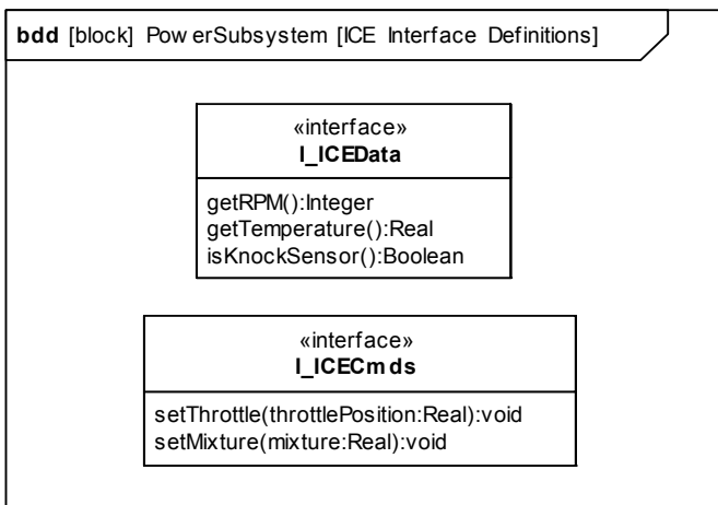
Figure B.20 - Interfaces Typing StandardPorts Internal to the Power Subsystem (Block Definition Diagram)
