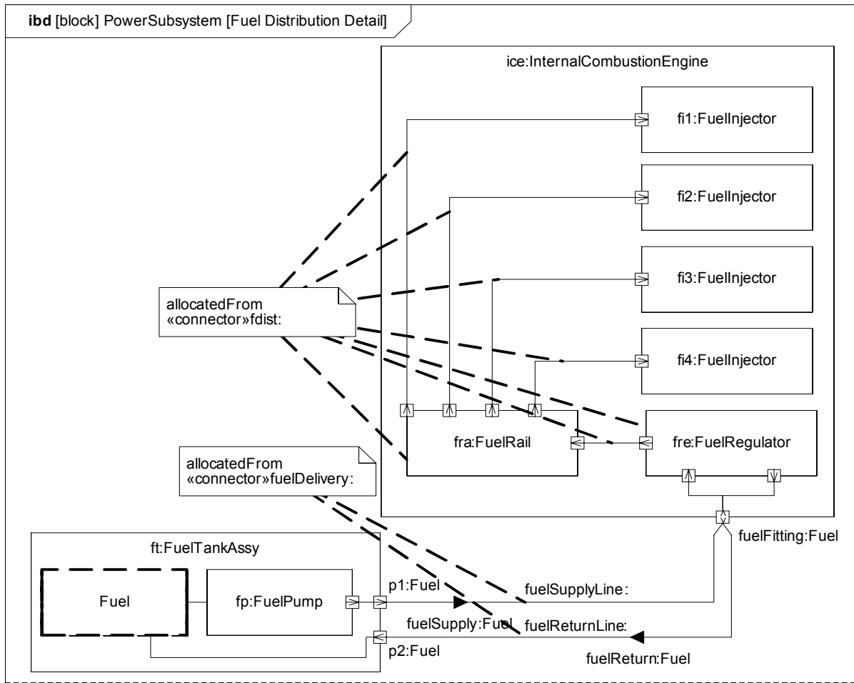
Figure 9.5 - Usage of atomic flow ports in the HybridSUV Sample - ibd:FuelDist diagram
