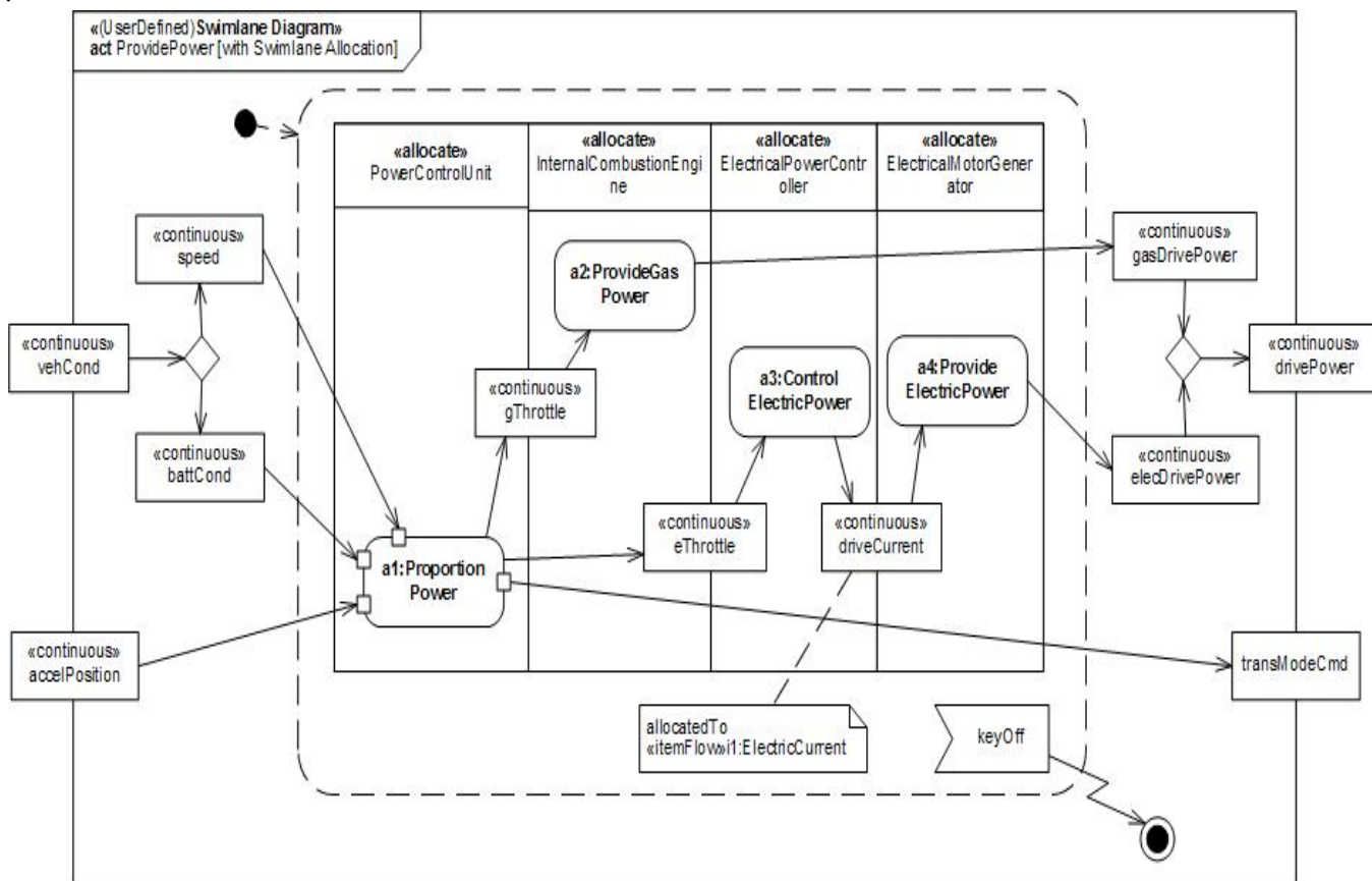
Figure B.35 - Detailed Behavior Model for “Provide Power” (Activity Diagram) Note hierarchical consistency with Figure B.33.
