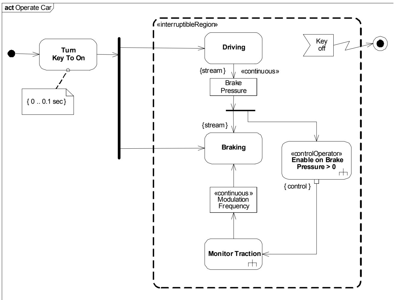
Figure 11.10 - Continuous system example 1
