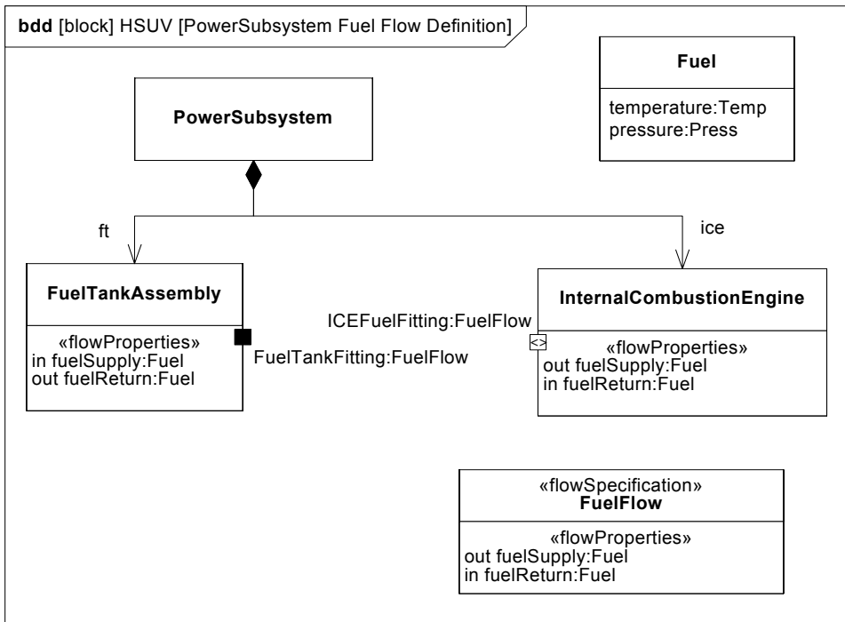
Figure B.23 - Elaborating Definition of Fuel Flow. (Block Definition Diagram)
