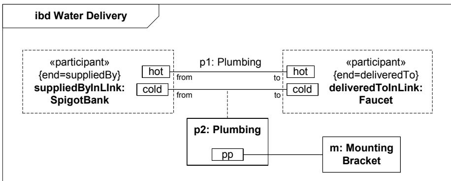
Figure 8.18 - Water Delivery association block with internal Plumbing connector
