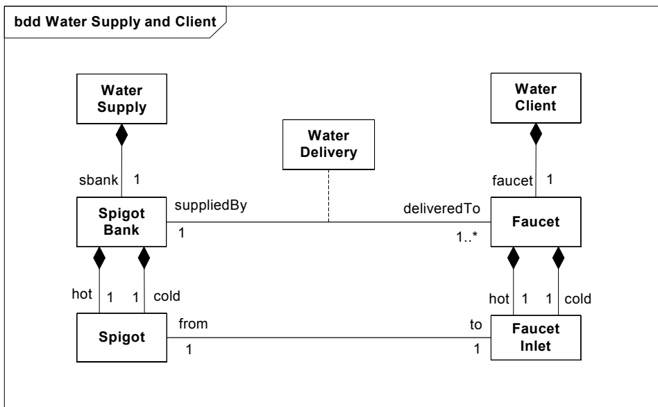
Figure 8.12 Water Delivery association block
