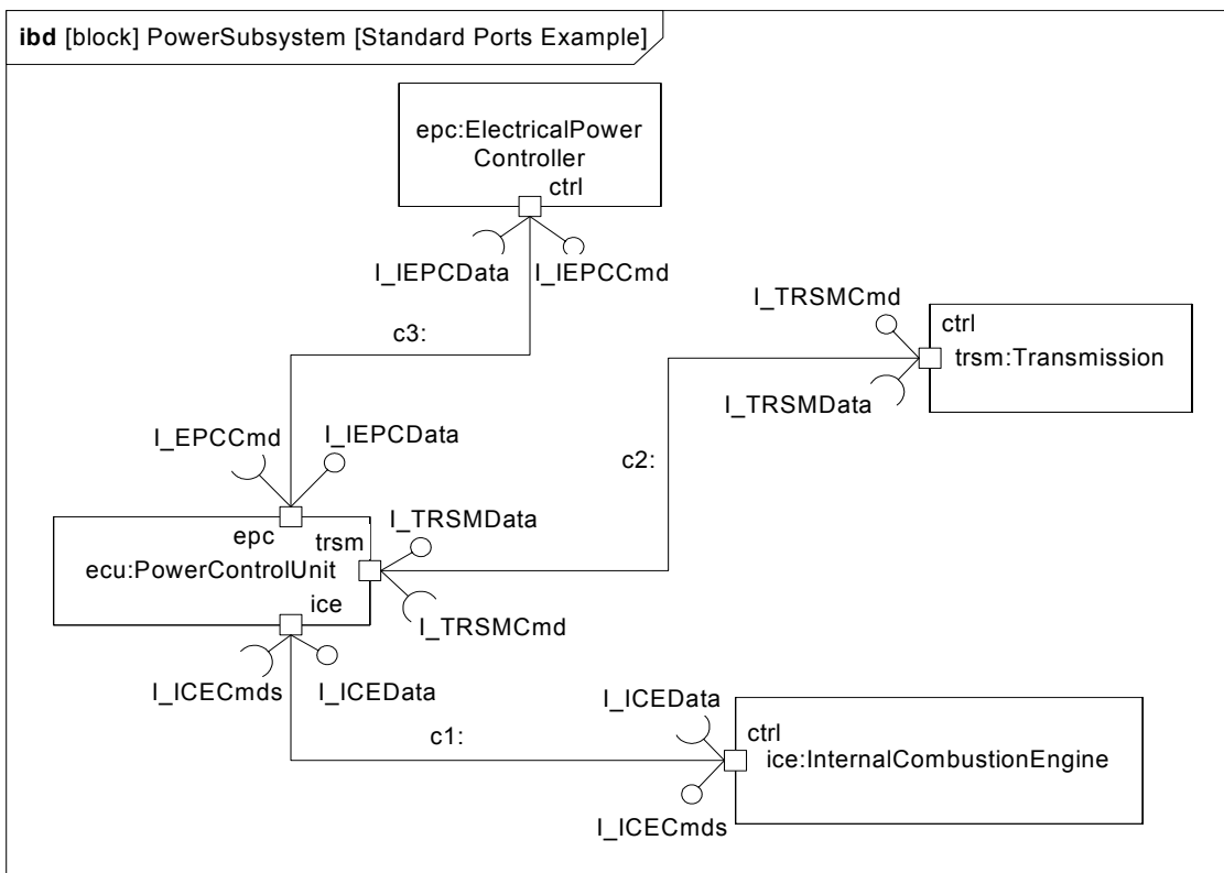
Figure 9.3 - Usage example of standard ports
