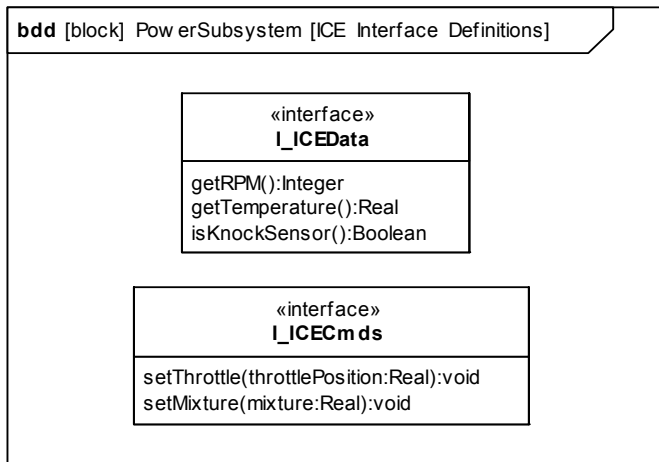
Figure 9.4 - Interfaces “ctrl” standard port of InternalCombustionEngine
