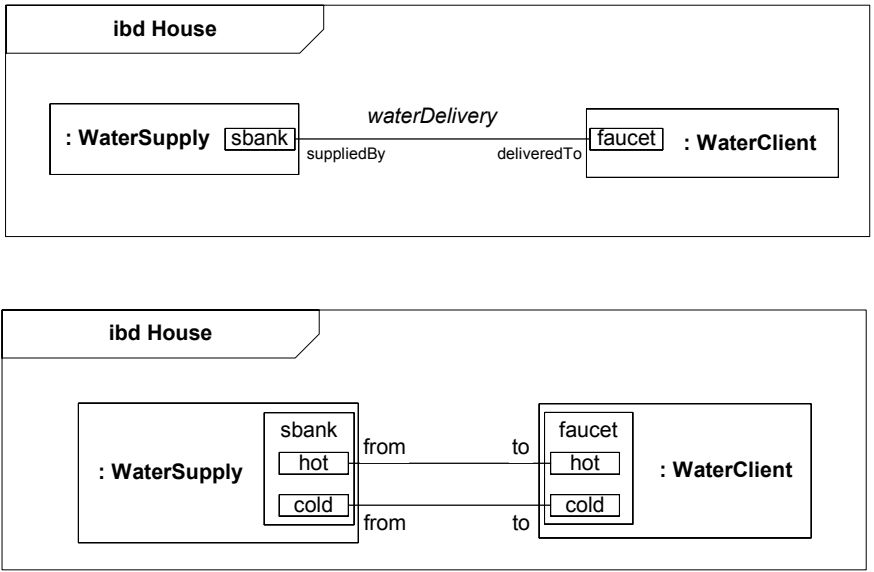
Figure 8.14 - Two views of Water Delivery connector within House block
