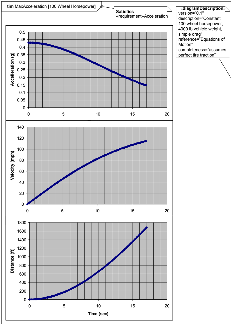
Figure B.32 - Results of Maximum Acceleration Analysis (Timing Diagram)
