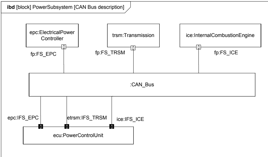
Figure B.22 - Consolidating Interfaces into the CAN Bus. (Internal Block Diagram)
