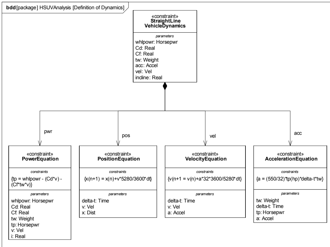
Figure 10.2 Definition of constraint blocks on a block definition diagram
