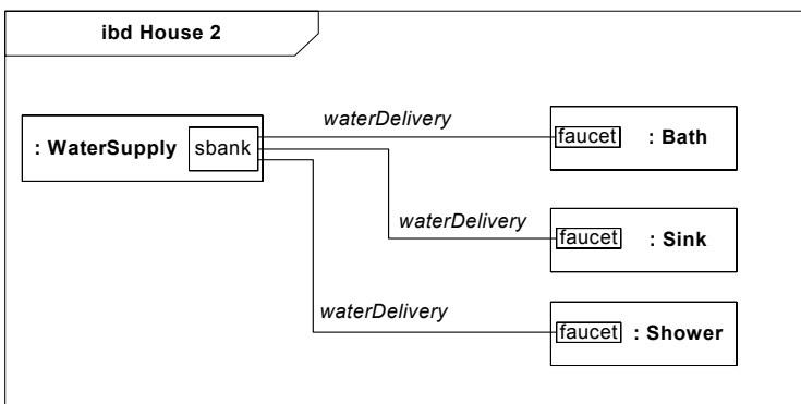
Figure 8.15 - Specializations of Water Client in house example
