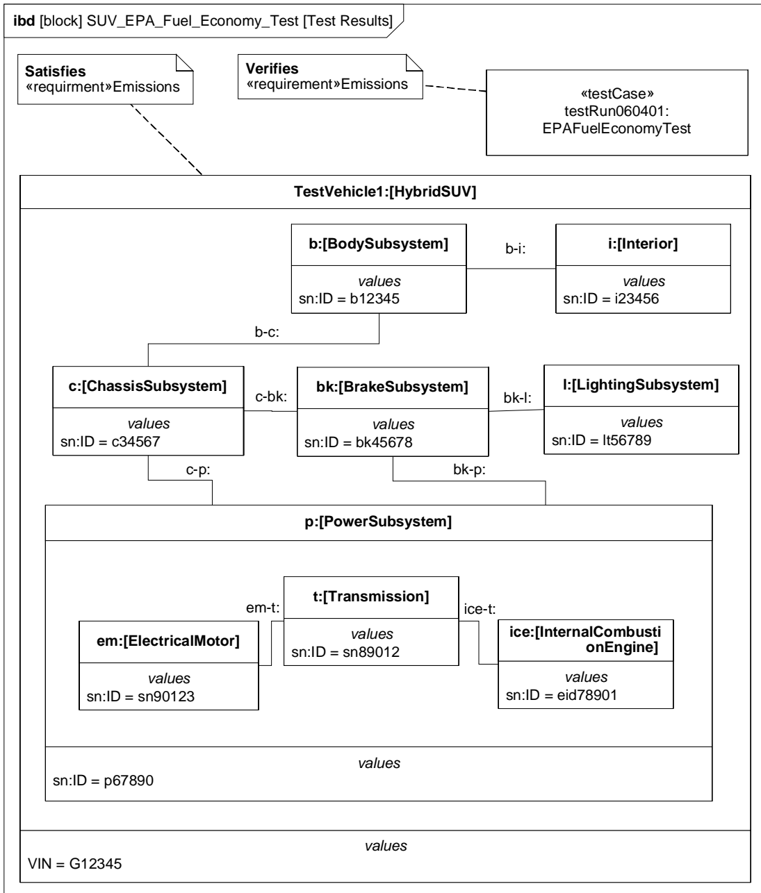
Figure 8.11 - SUV EPA Fuel Economy Test
