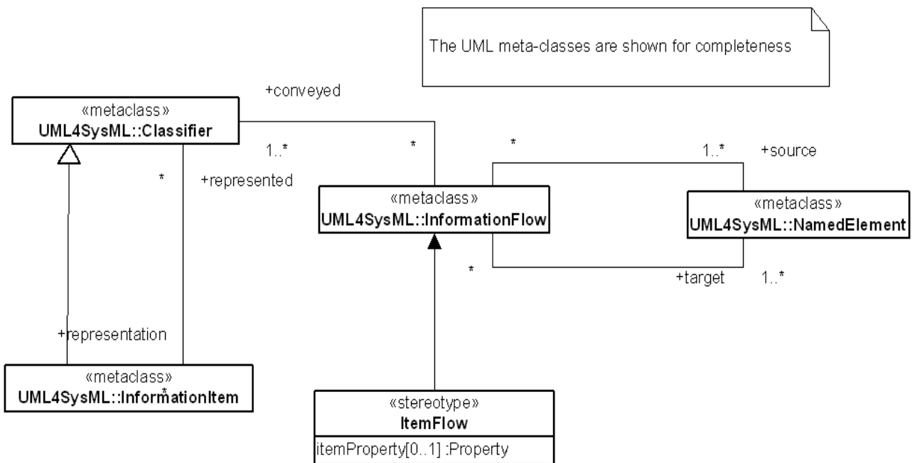
Figure 9.2 - ItemFlow Stereotype
