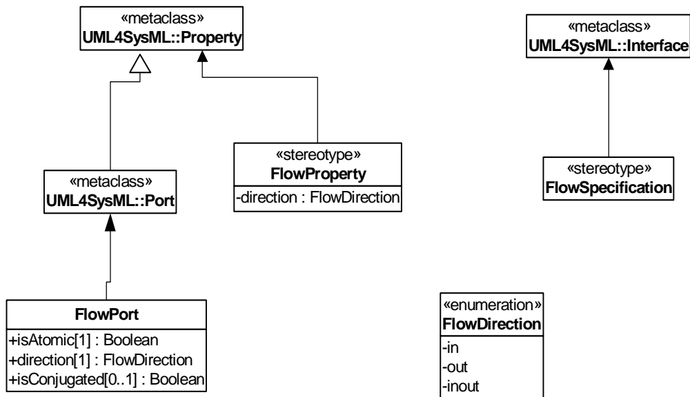
Figure 9.1 - Port Stereotypes
