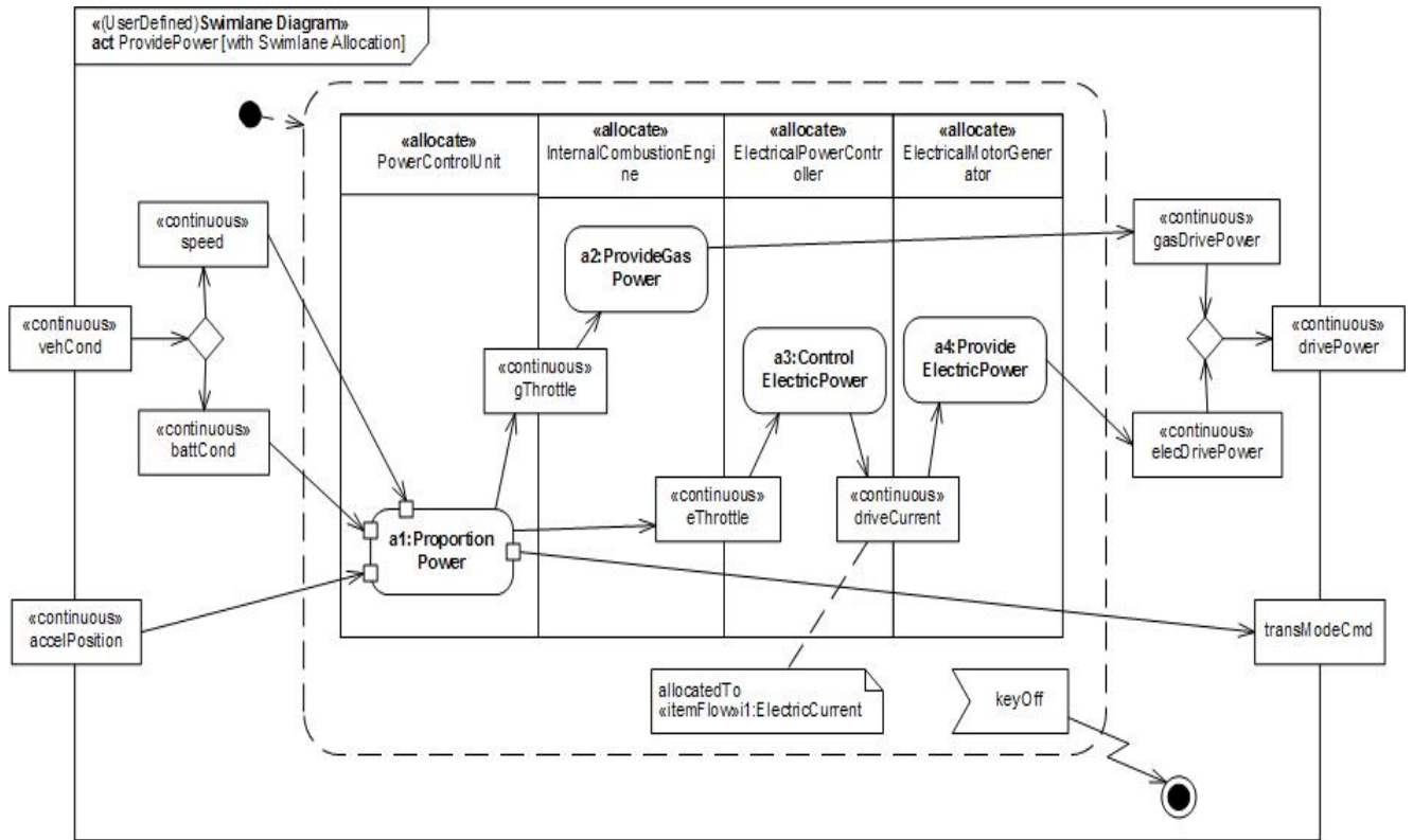
Figure 15.9 - AllocateActivityPartitions (Swimlanes) for HybridSUV Cellarette Example
