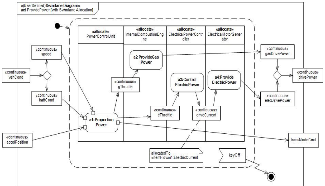
Figure B.35 - Detailed Behavior Model for “Provide Power” (Activity Diagram) Note hierarchical consistency with Figure B.33.
