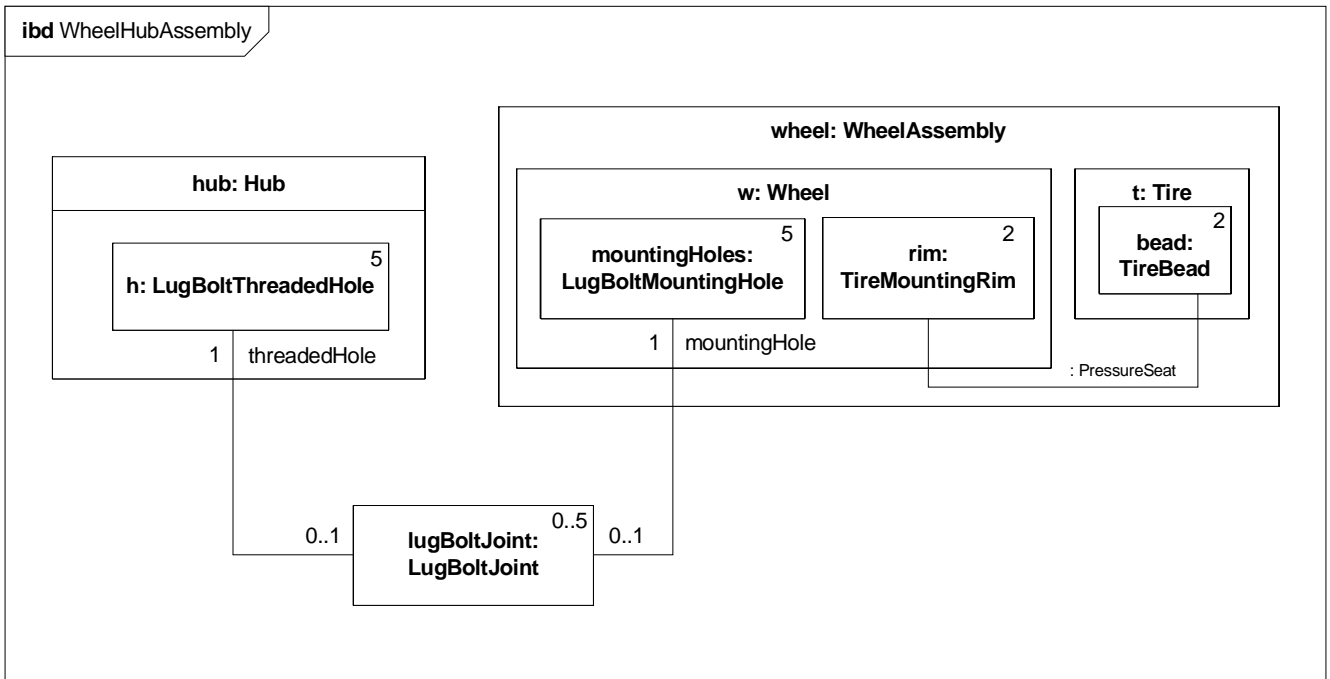
Figure 8.9 - Internal Block Diagram for WheelHubAssembly
