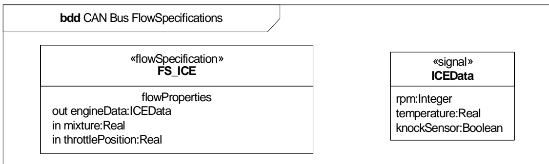
Figure 9.7 - Flow Specification for the InternalCombustionEngine flow port to allow its connection over the CAN bus
