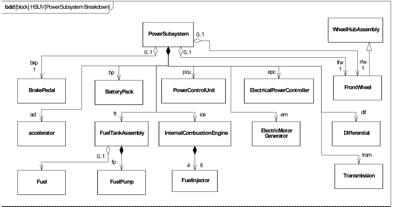
Figure B.18 - Defining Structure of Power Subsystem (Block Definition Diagram)
