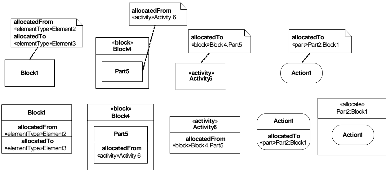
Figure 15.4 - Behavior allocation
