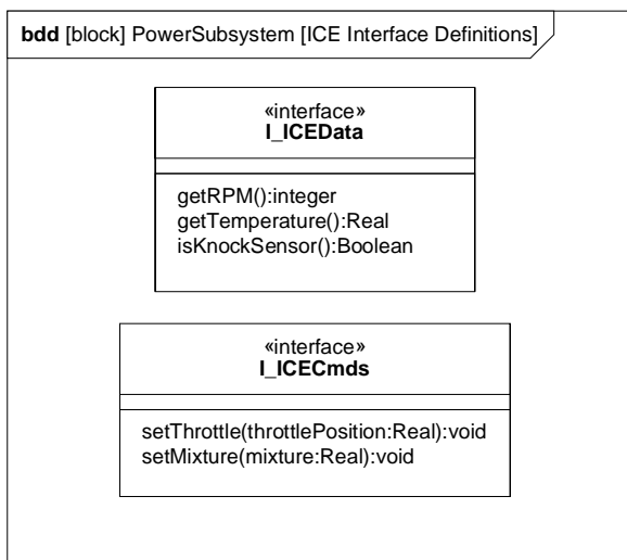
Figure B.20 - Interfaces Typing StandardPorts Internal to the Power Subsystem (Block Definition Diagram)
