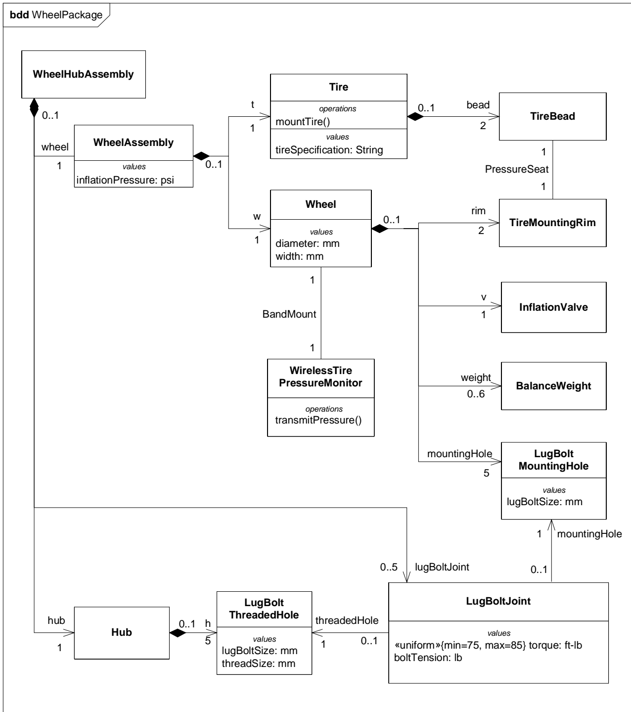
Figure 8.8 - Block diagram for the Wheel Package
