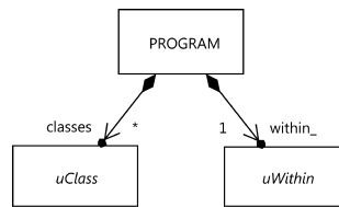
Figure 14: PROGRAM meta-class and relationships
