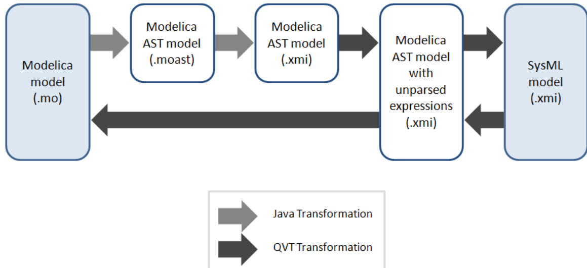
Figure 37: Overview of an implementation of the SysML-Modelica Transformation based on QVT
