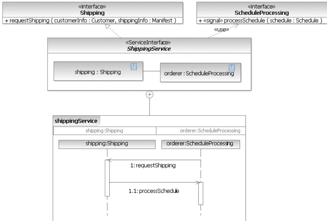
Figure 88: ShippingService Service Interface
