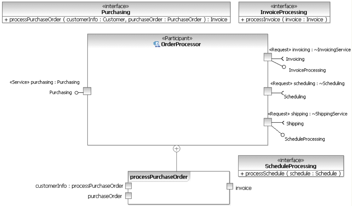
Figure 39: The OrderProcessor Participant
