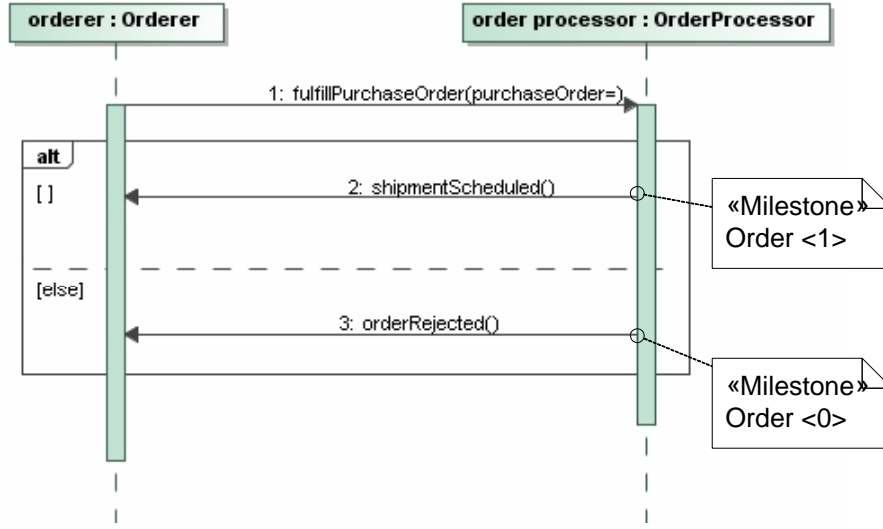
Figure 38: Milestones on Ordering Behavior
