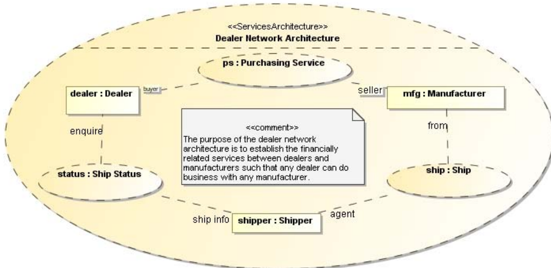
Figure 57: Services architecture involving three participants
