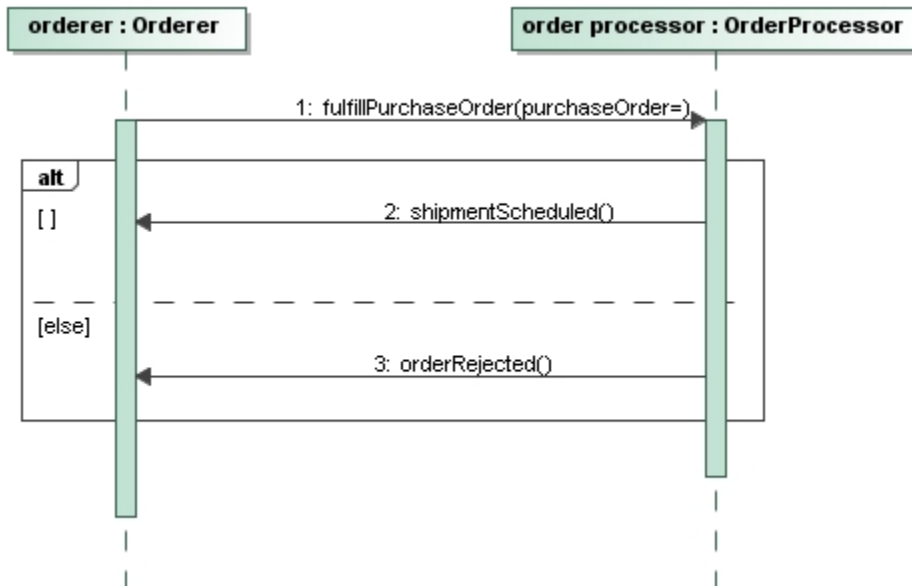
Figure 77: Flow of information
