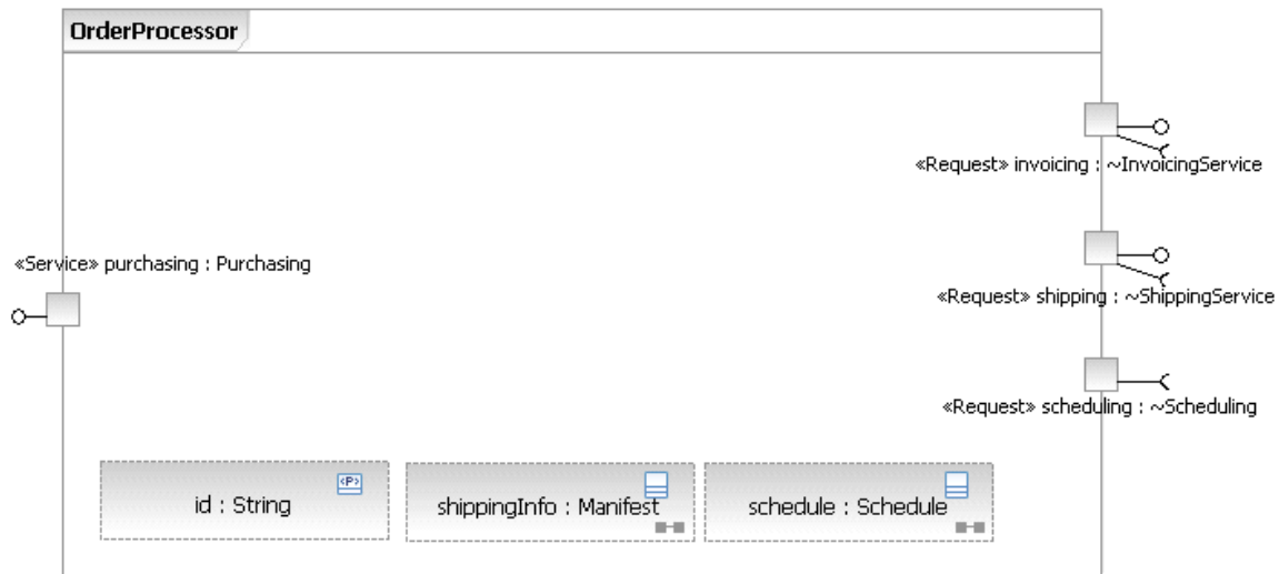
Figure 43: Requests of the OrderProcessor Participant
