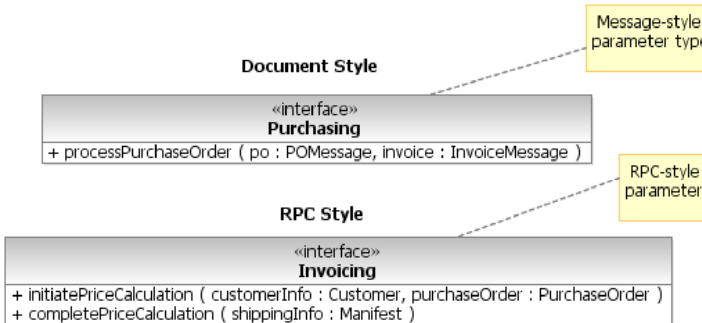
Figure 37: Document and RPC Style service operation parameters
