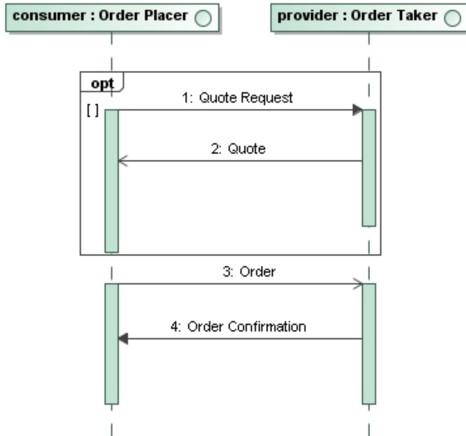
Figure 46: Ordering Service communication protocol
