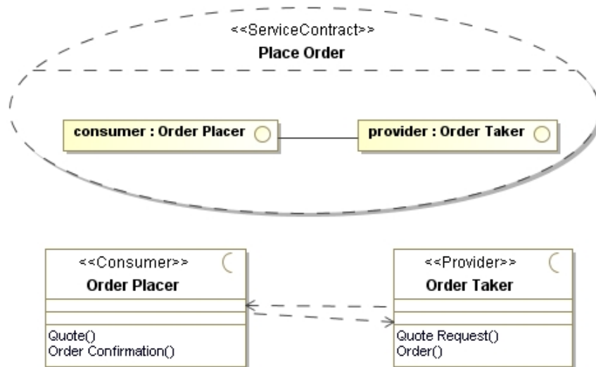
Figure 14 - Service Contract Collaboration and Interfaces
