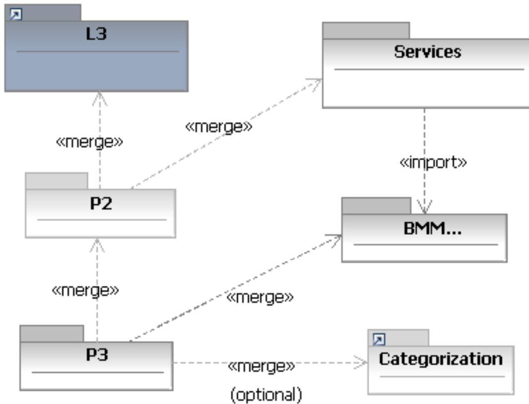
Figure 2: SoaML Compliance point P3
