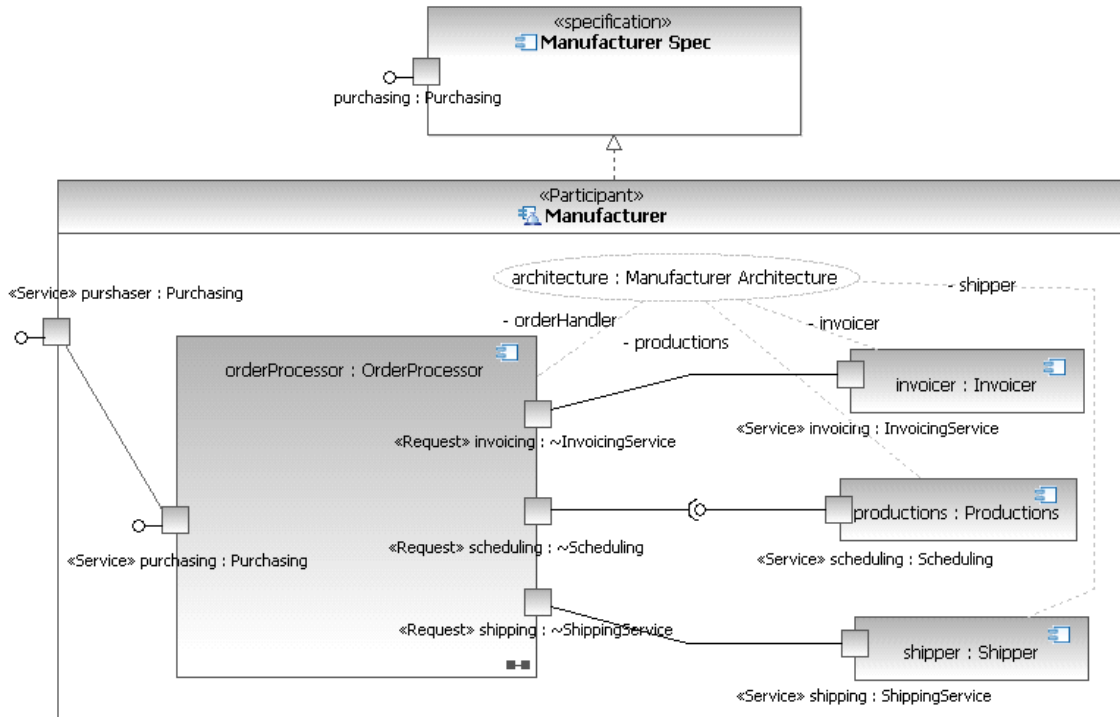
Figure 44: The Manufacturer Participant
