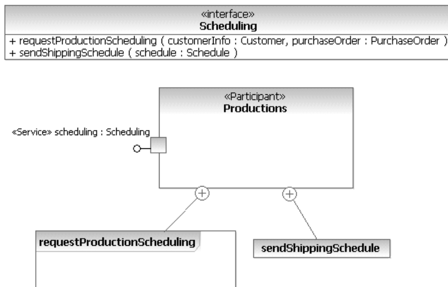
Figure 3: Services and Service Participants
