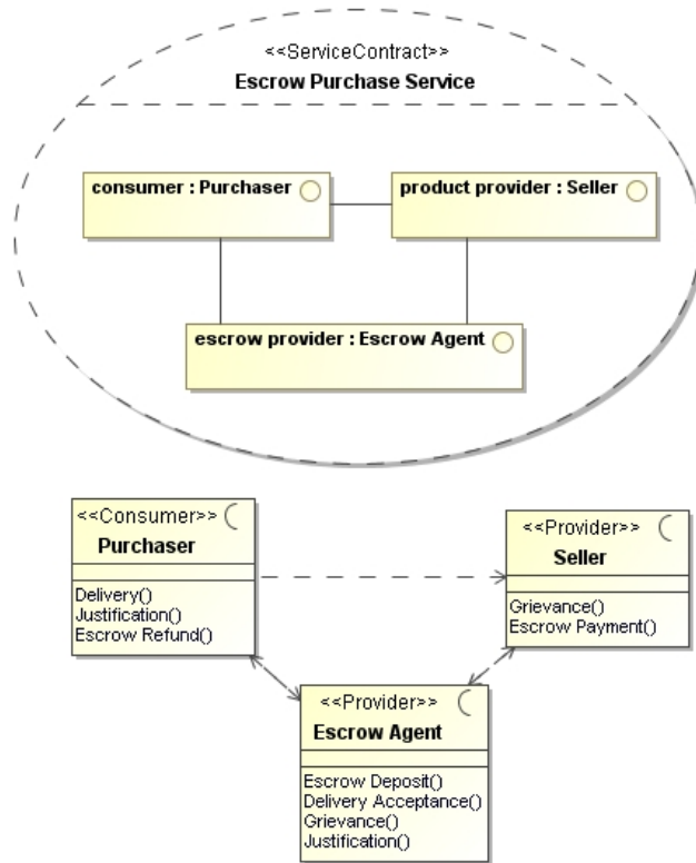
Figure 18 - Multi-party service contract and interfaces
