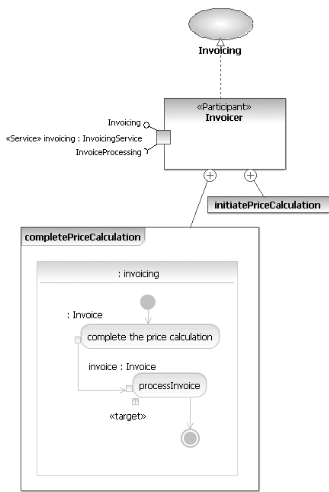
Figure 55: The invoicing Service of the Invoicer Participant
