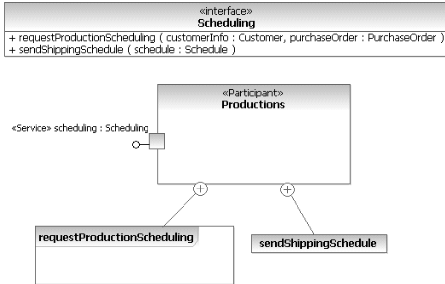
Figure 91: The Productions Service Provider
