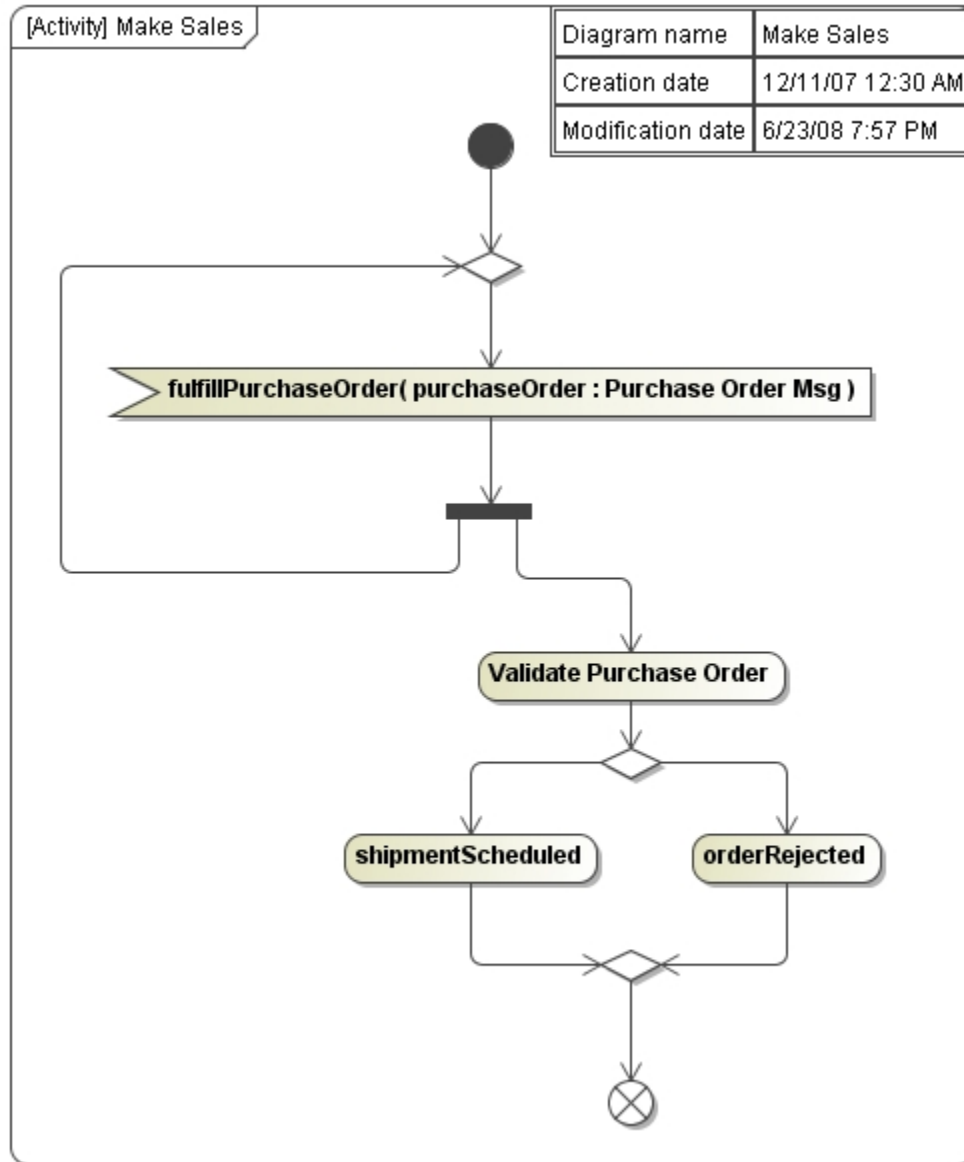
Figure 79: Make sales business process
