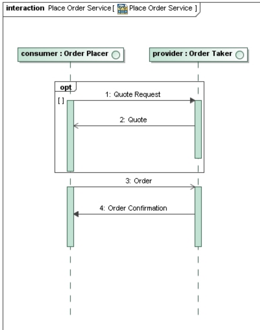
Figure 7 - Place order choreography
