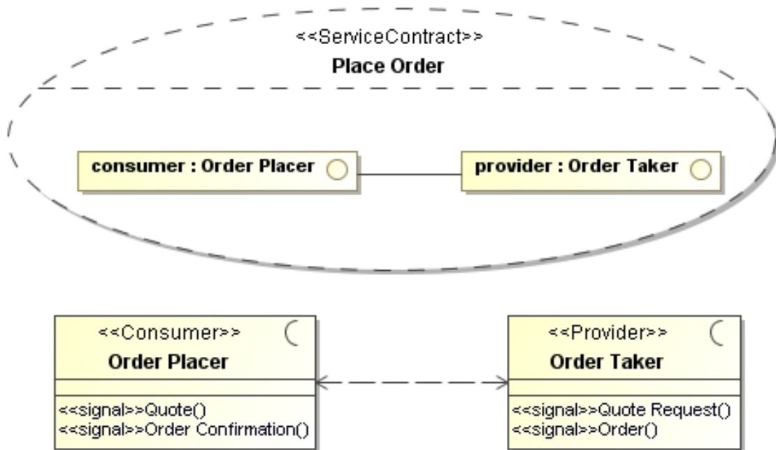
Figure 45: The Ordering Service Contract
