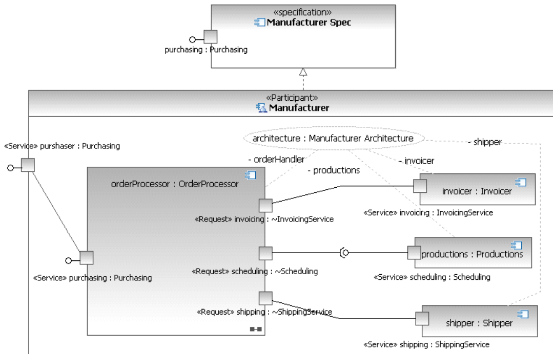
Figure 96: Assembling the Parts into a Deployable Subsystem
