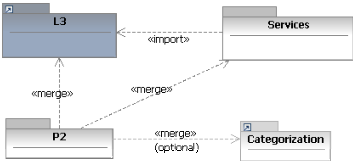
Figure 1: SoaML Compliance point P2
