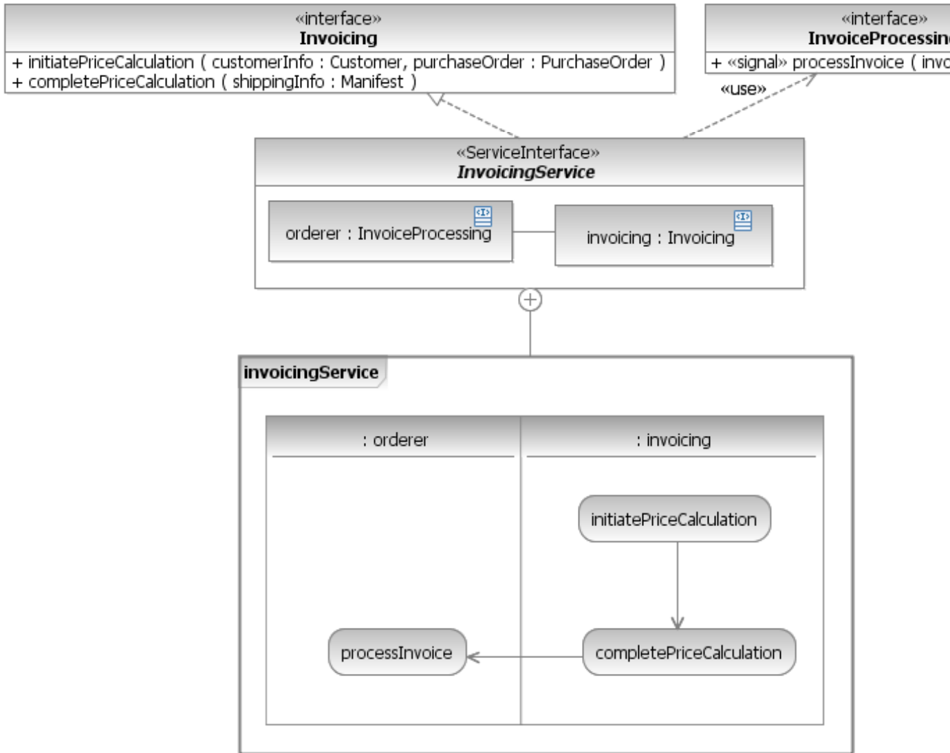
Figure 86: InvoicingService Service Interface
