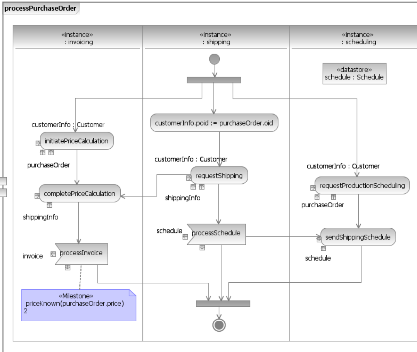
Figure 95: The processPurchaseOrder Service Operation Design
