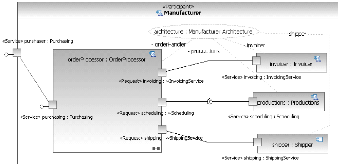
Figure 35: Fulfilling the Process Purchase Order Contract
