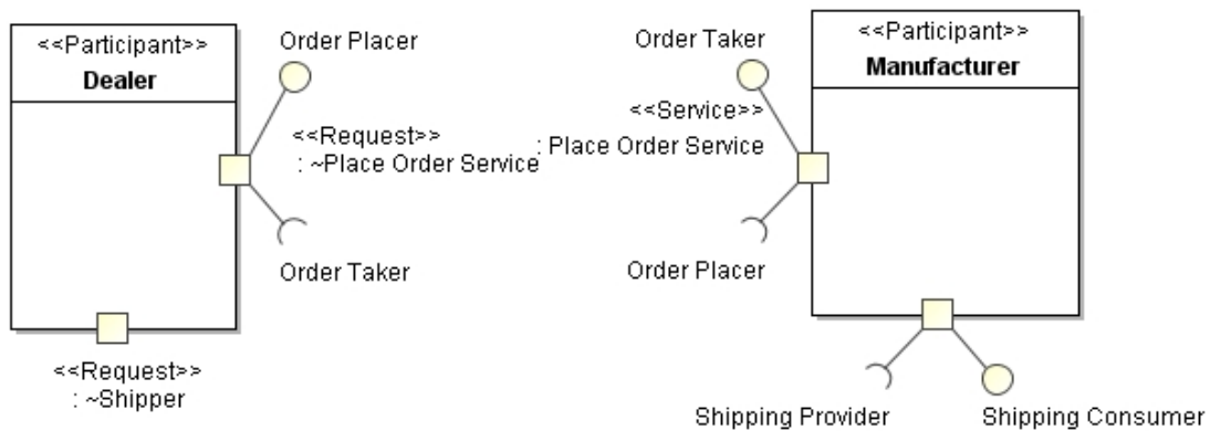
Figure 16 - Use of Request
