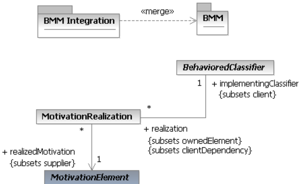
Figure 66: BMM Integration Package
