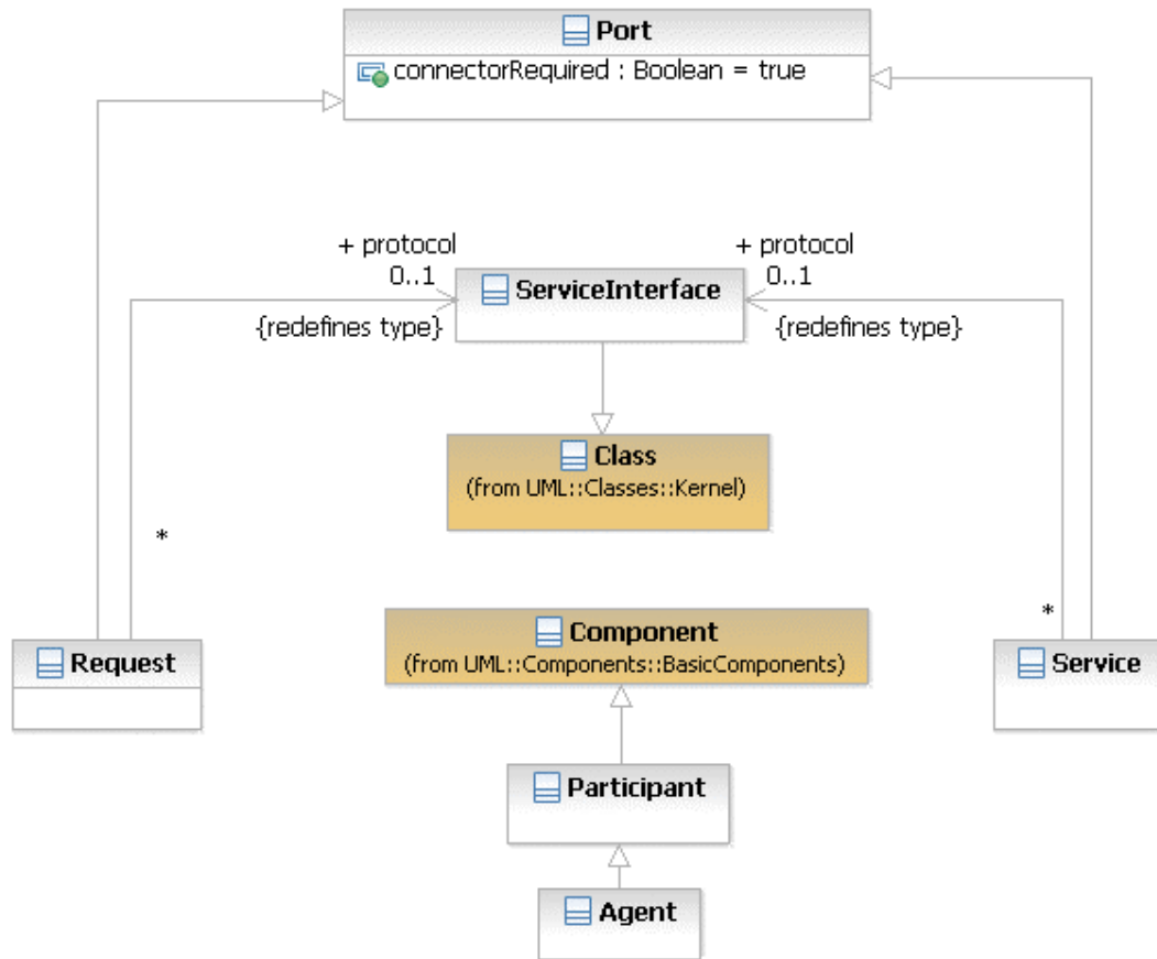
Figure 68: ServiceInterfaces and Participants
