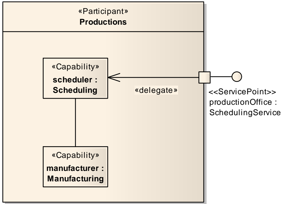
Figure 24: Productions Participant with two parts specified by Capabilities
