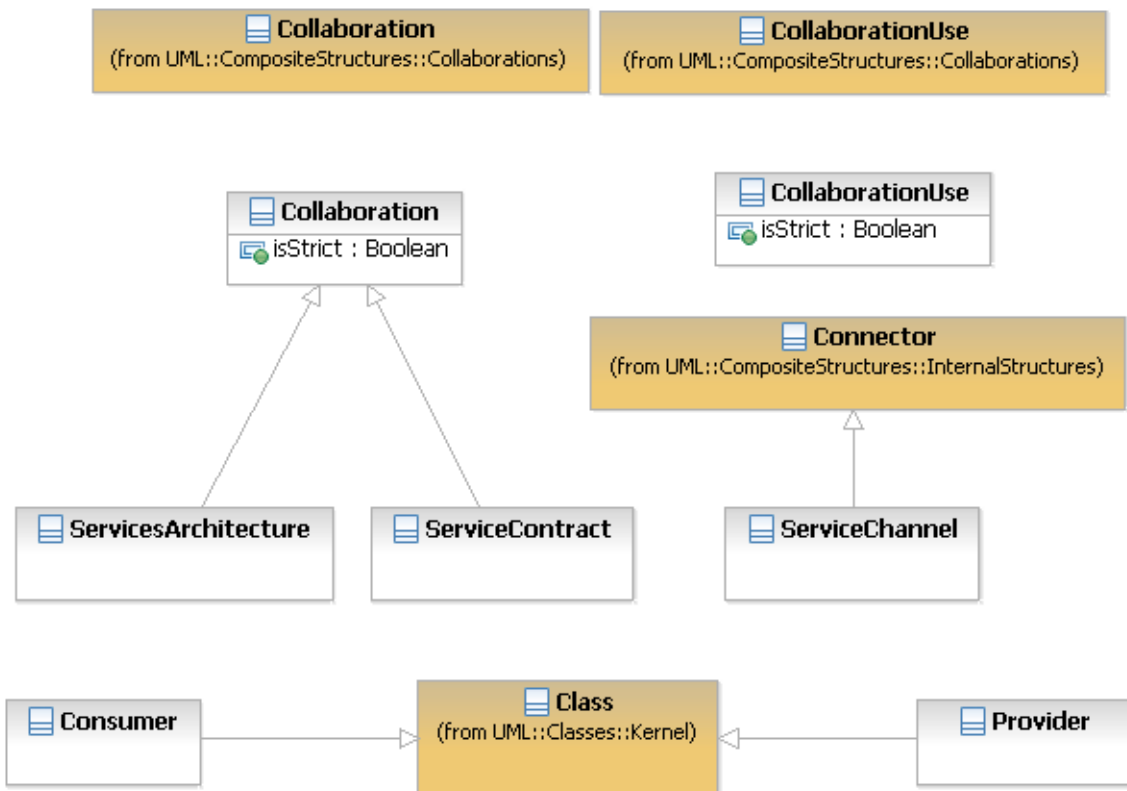
Figure 69: ServiceContracts and ServiceArchitectures
