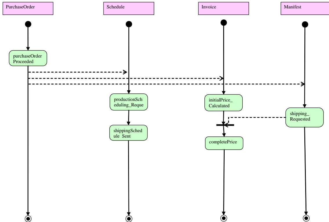
Figure 99: State Machine
