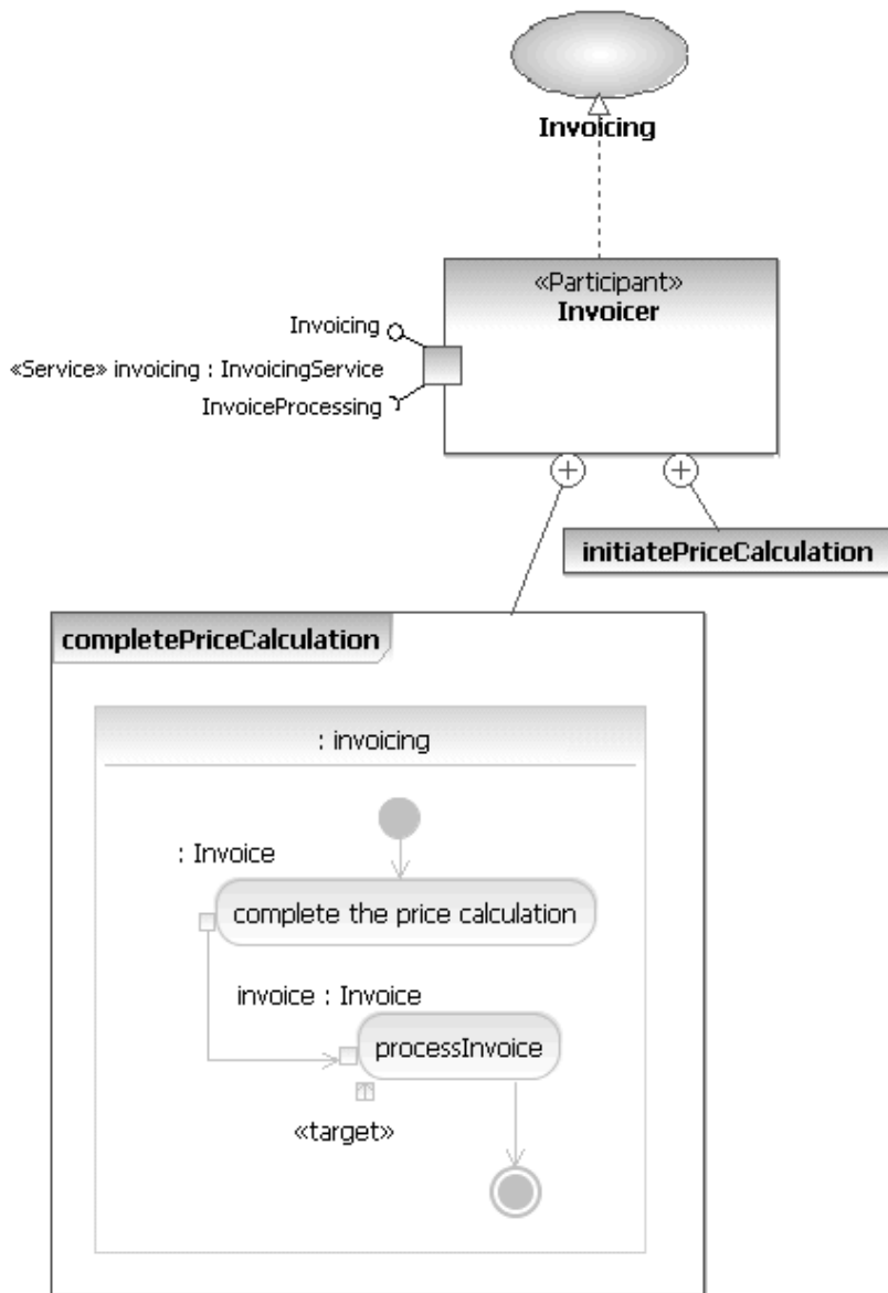
Figure 90: Invoicecer Service Provider providing the invoicing service
