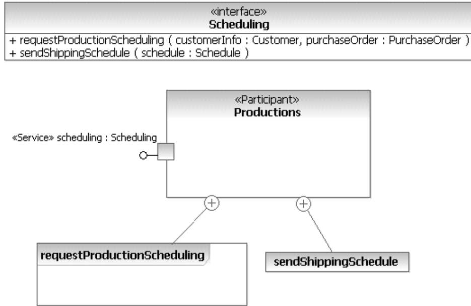
Figure 56: The scheduling Service of the Productions Participant
