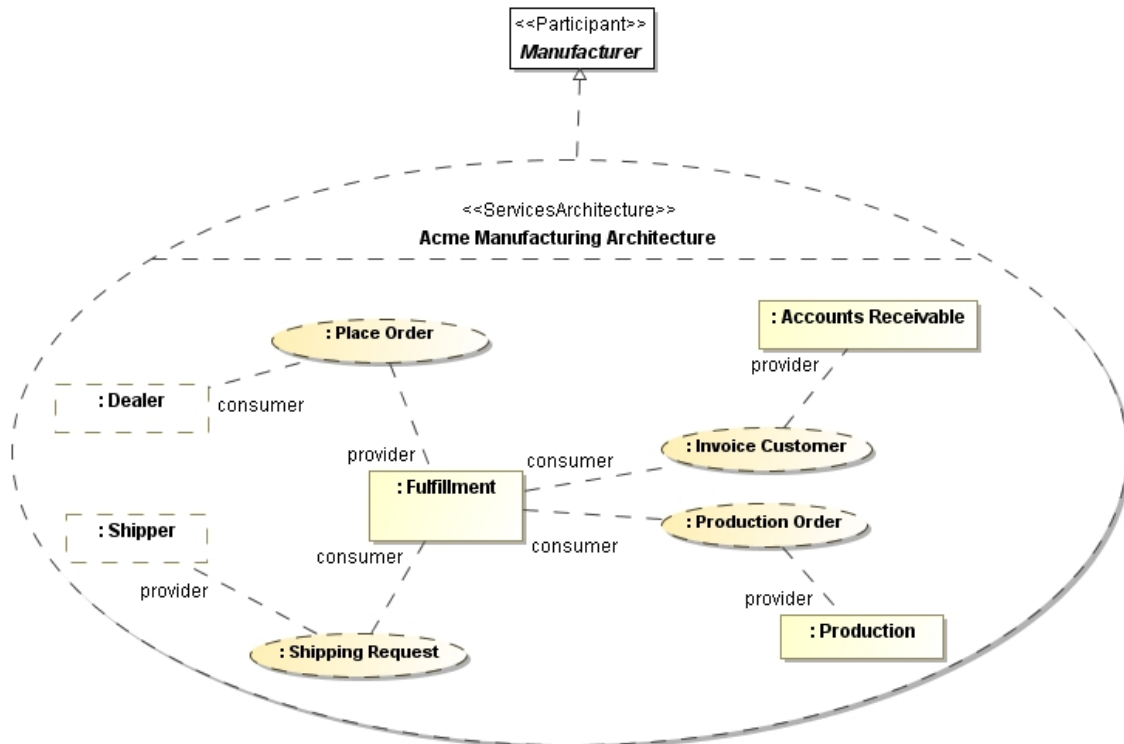
Figure 10: Example Services architecture for a participant
