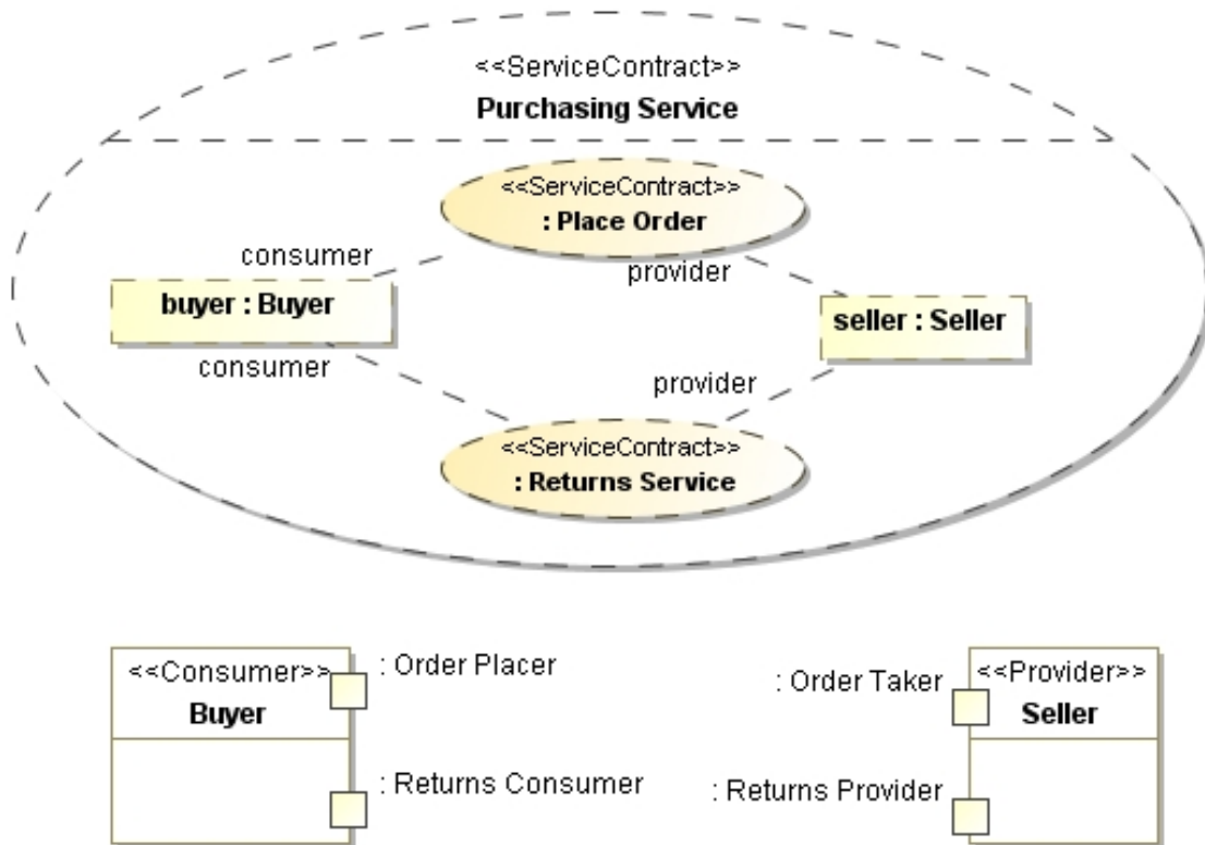
Figure 49: Service Interfaces of a compound service
