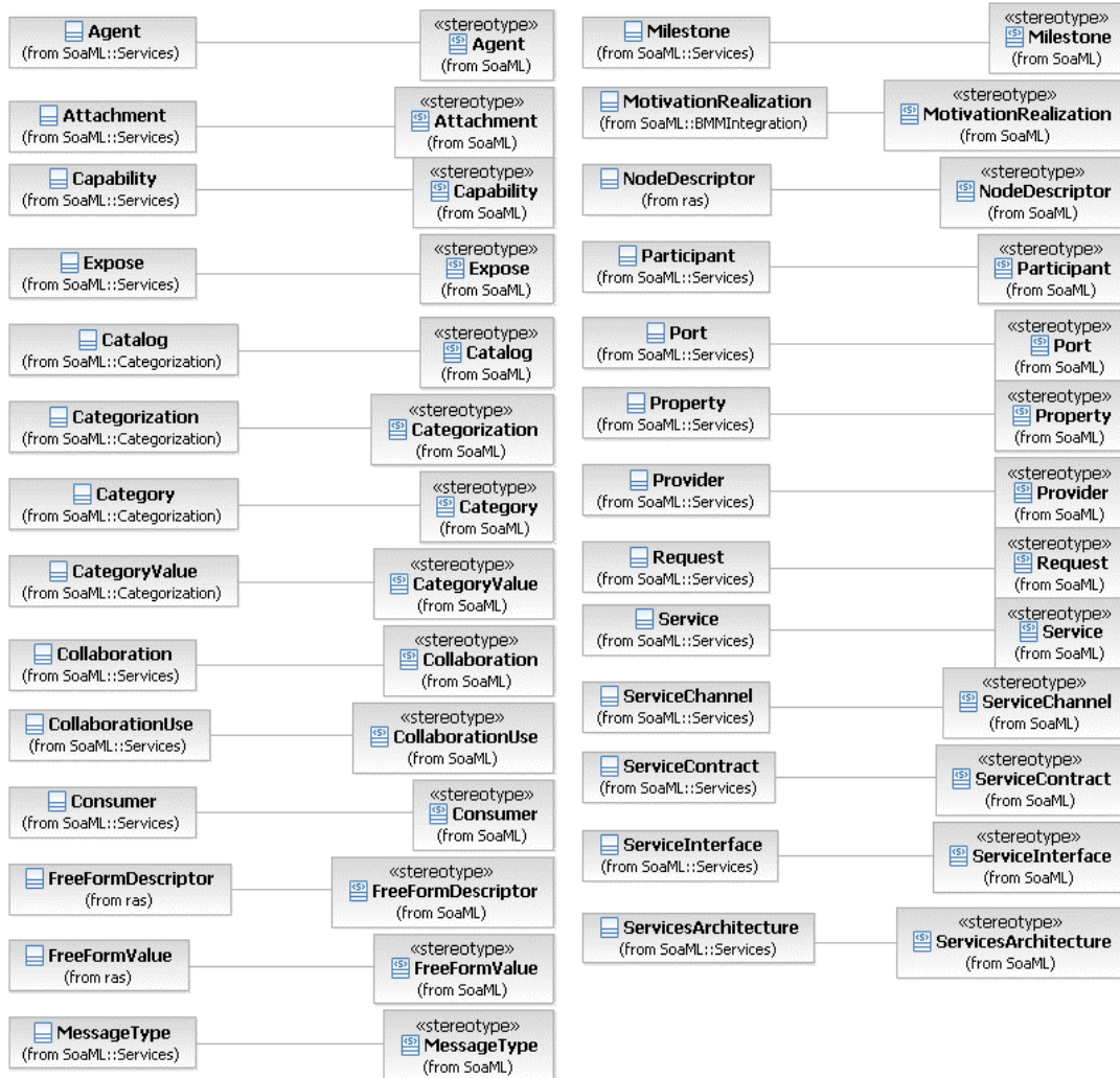
Figure 73: Profile metamodel mapping
