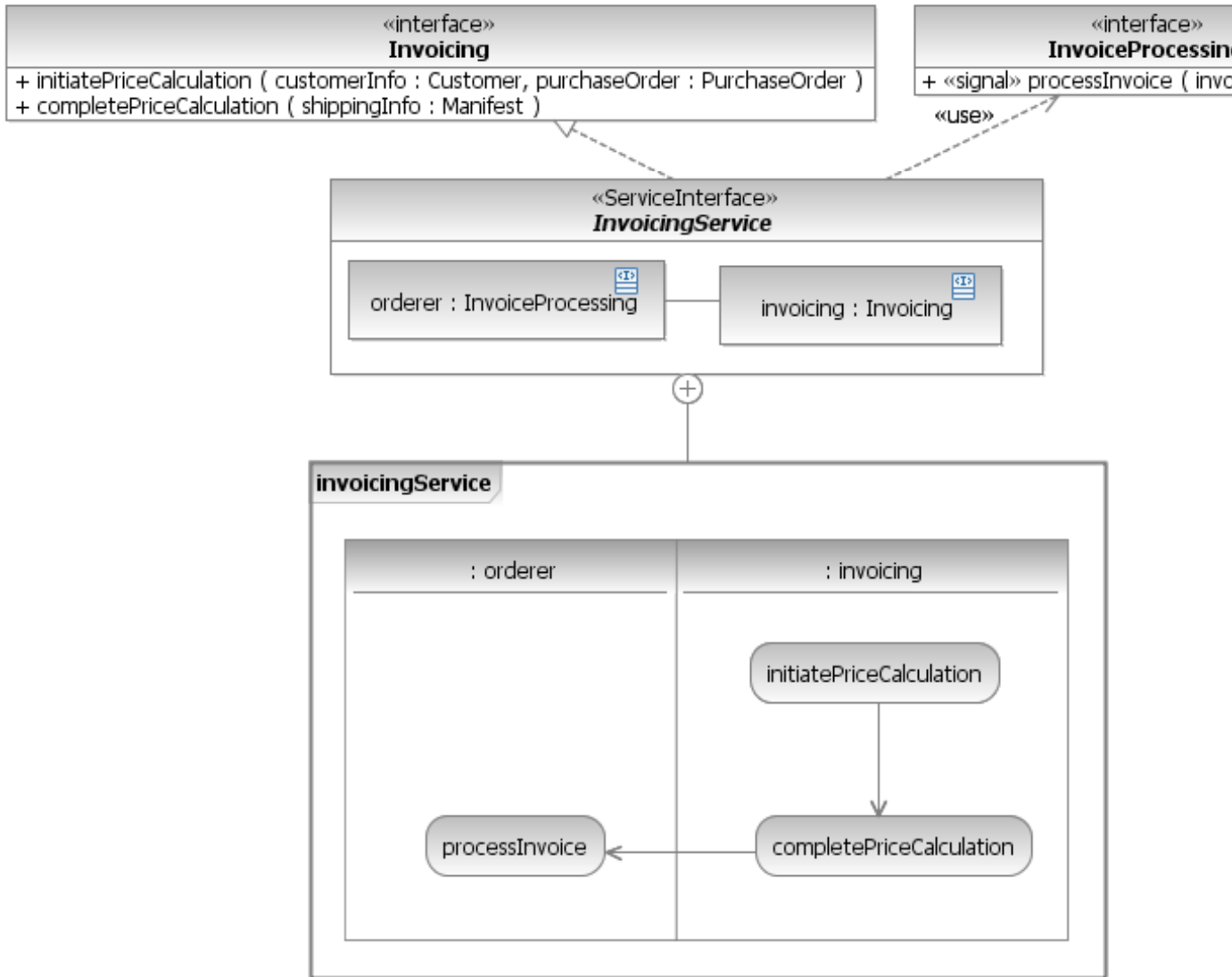
Figure 51: The InvoicingService ServiceInterface
