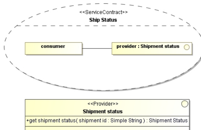
Figure 19 - Simple interface in service contract
