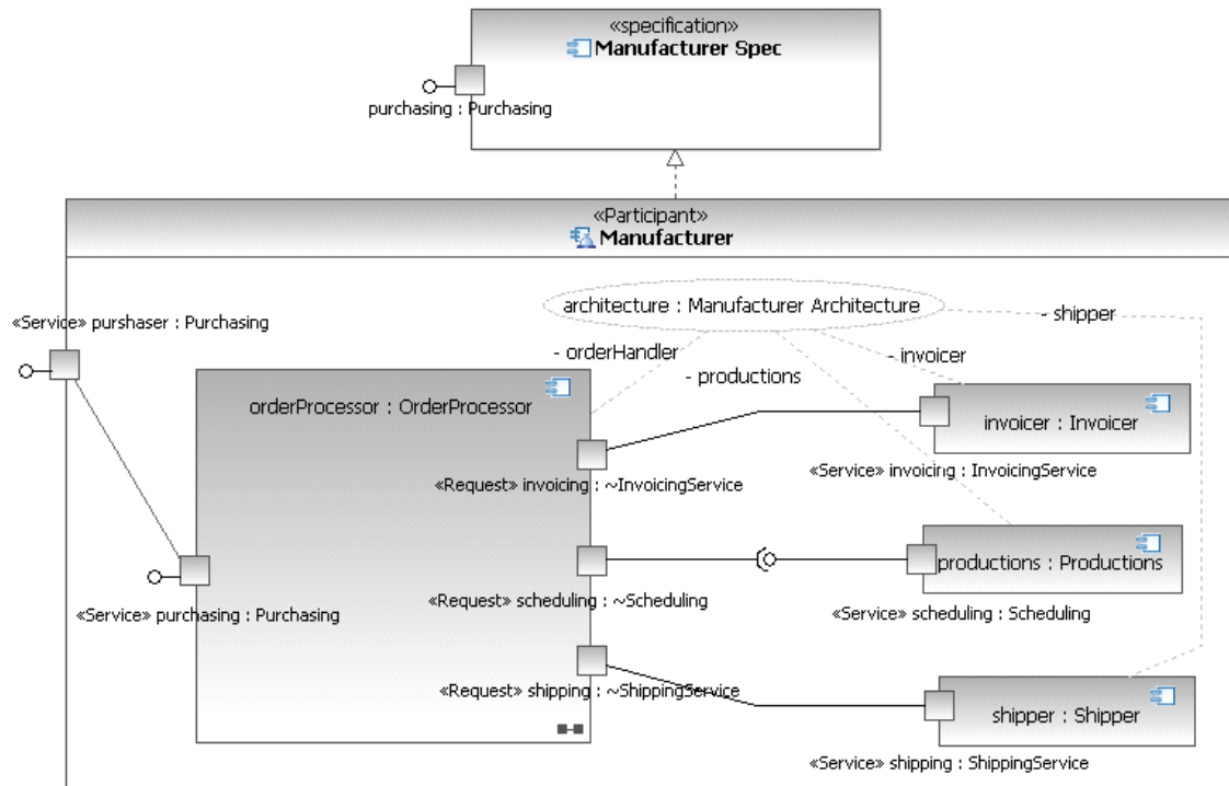
Figure 41: The Manufacturer Participant
