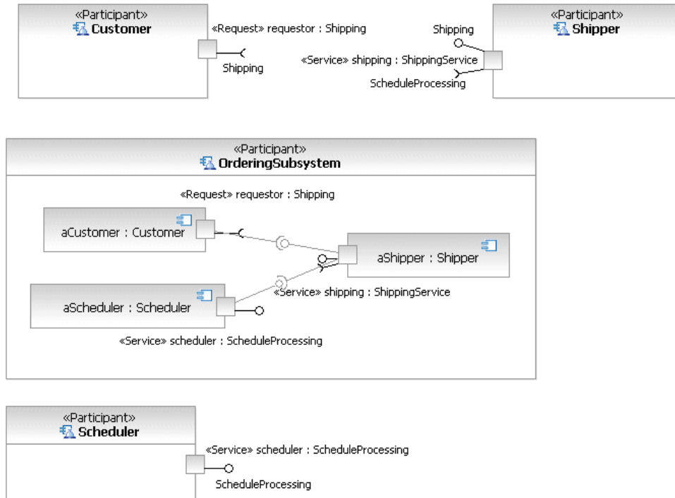
Figure 53: Using the shipping Service with two Consumers
