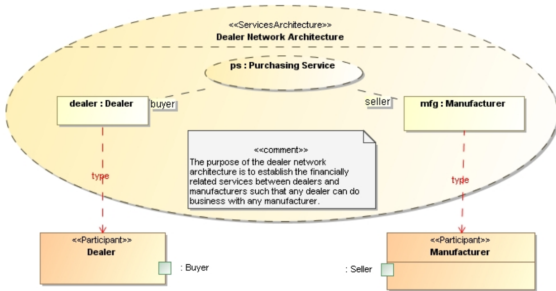
Figure 58: Abbreviated service contract
