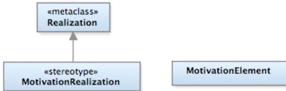
Figure 26: BMM Integration
