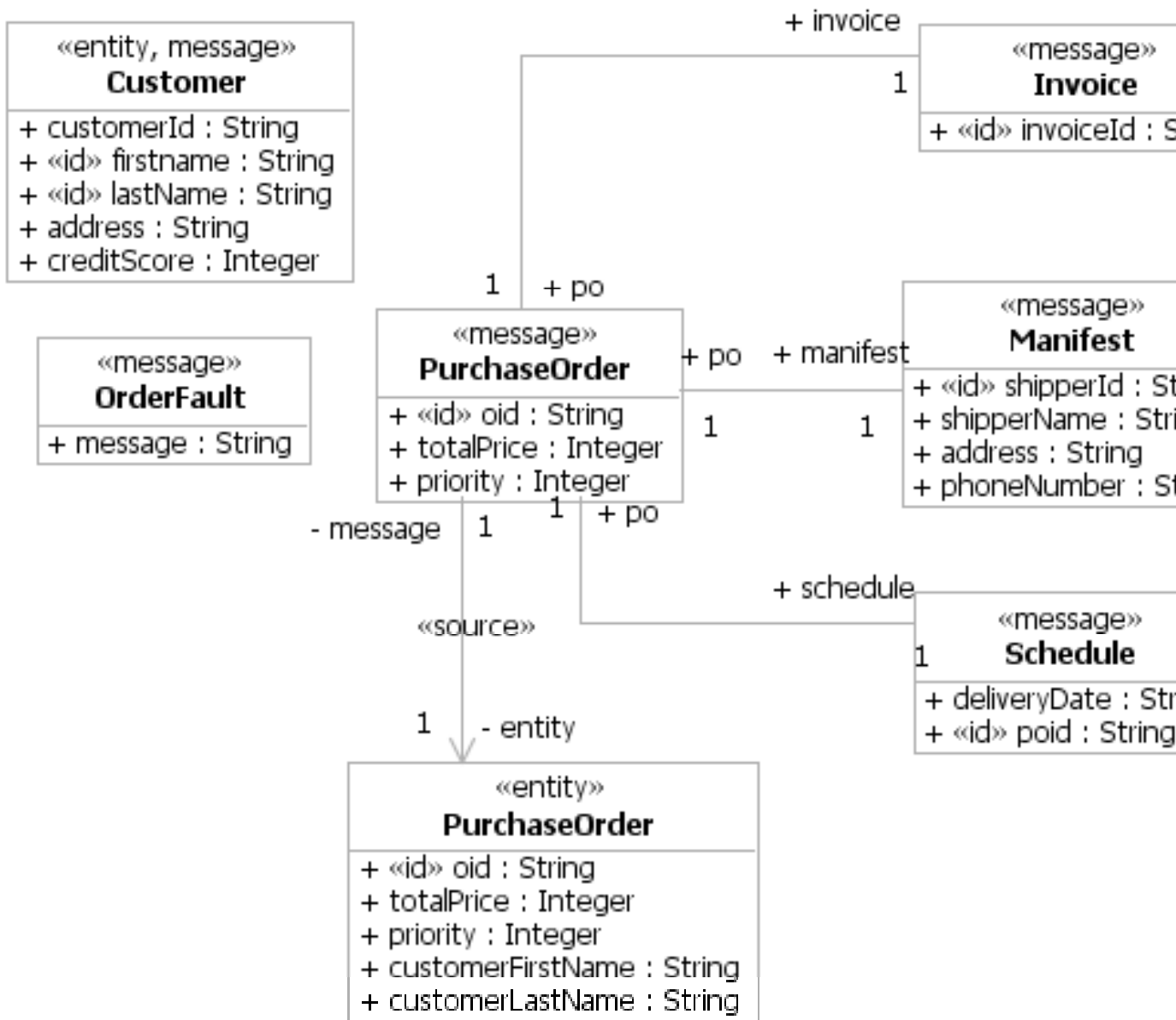
Figure 98: Entity Model (Class diagram)
