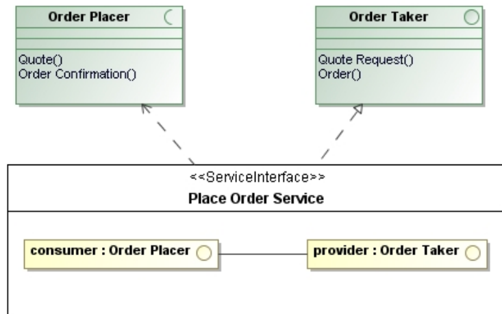
Figure 6 - Service Interface Definition
