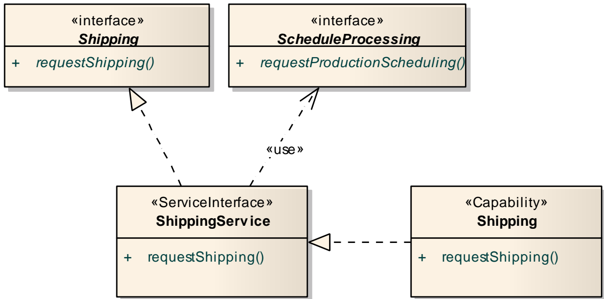
Figure 22: ServiceInterface realized by a Capability
