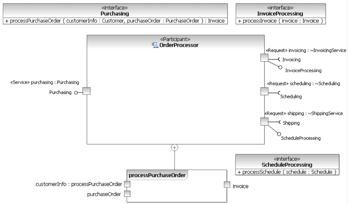
Figure 93: The OrderProcessor Service Provider
