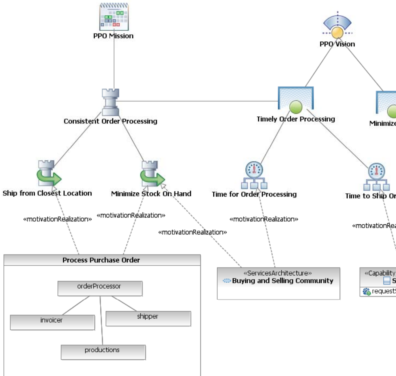
Figure 67: Business Motivation Model for Processing Purchase Orders
