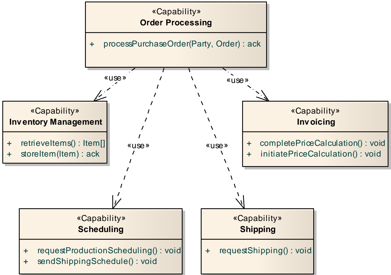
Figure 21: Service Capabilities needed for processing purchase orders
