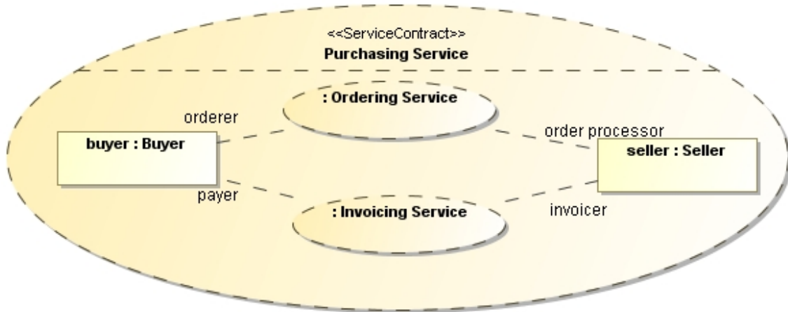
Figure 48: Compound Services
