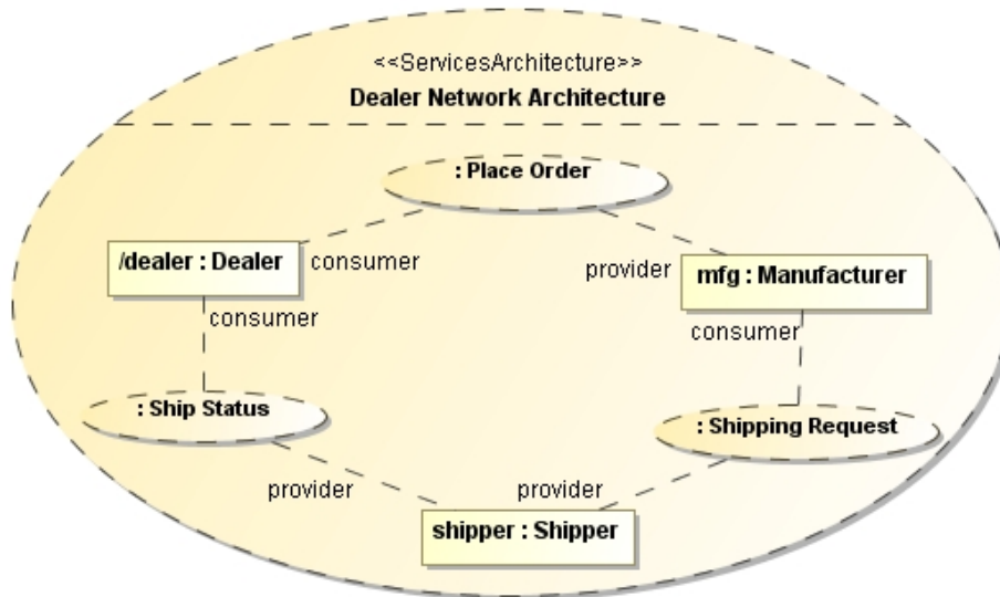
Figure 20 - Services Architecture
