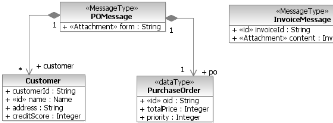
Figure 97: The CRM Data Model
