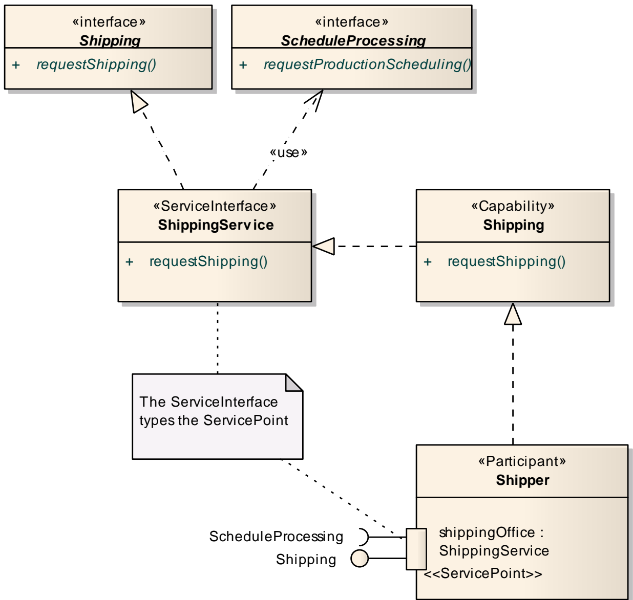
Figure 23: The Shipper Participant realizes the Shipping Capability
