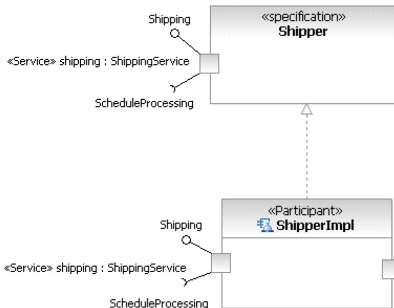
Figure 92: The Shipper Service Provider
