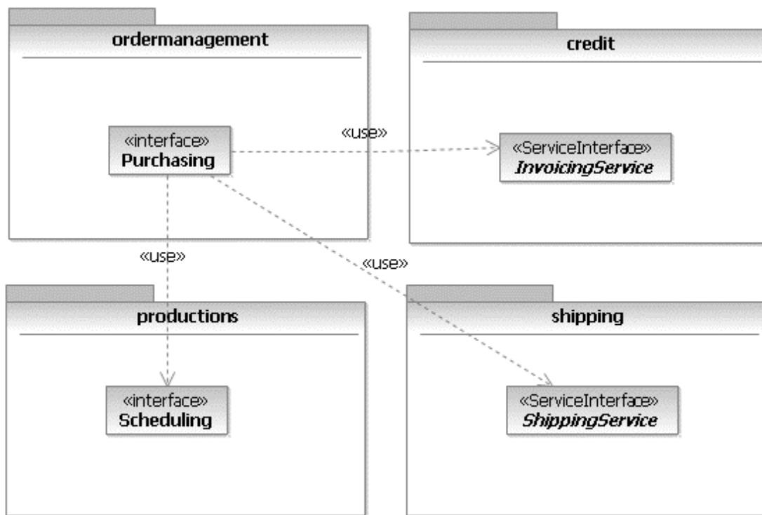
Figure 85: Identified Service Interfaces
