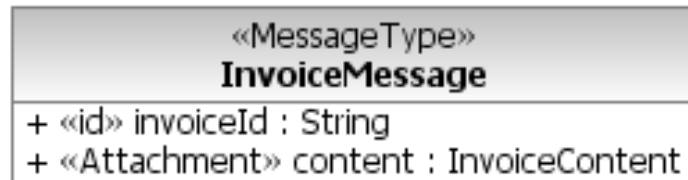
Figure 33: The InvoiceContent Attachment
