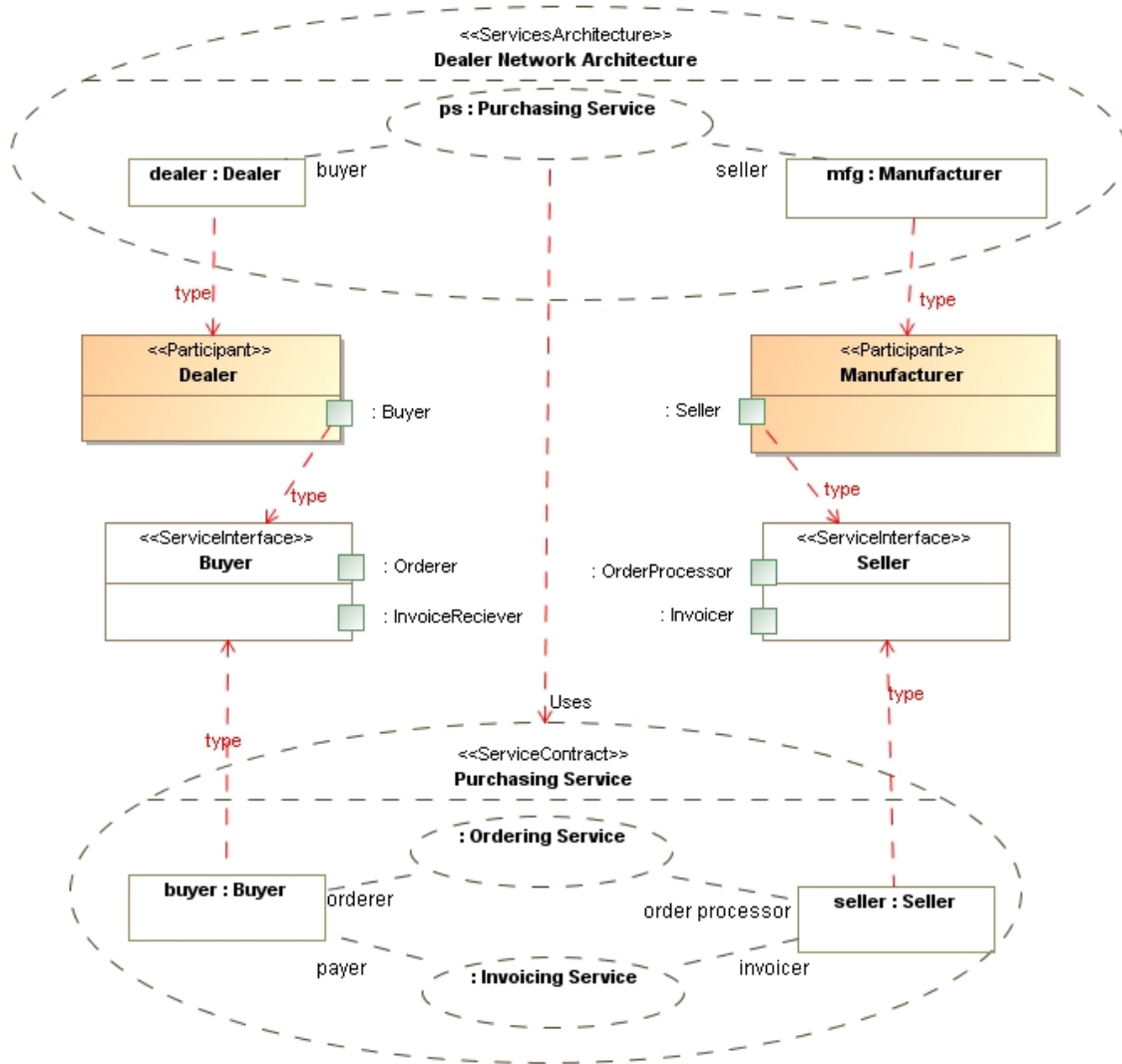
Figure 82: Relating services architecture as service contracts
