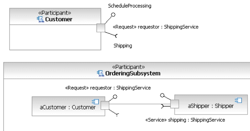
Figure 54: Using the shipping Service with one Consumer
