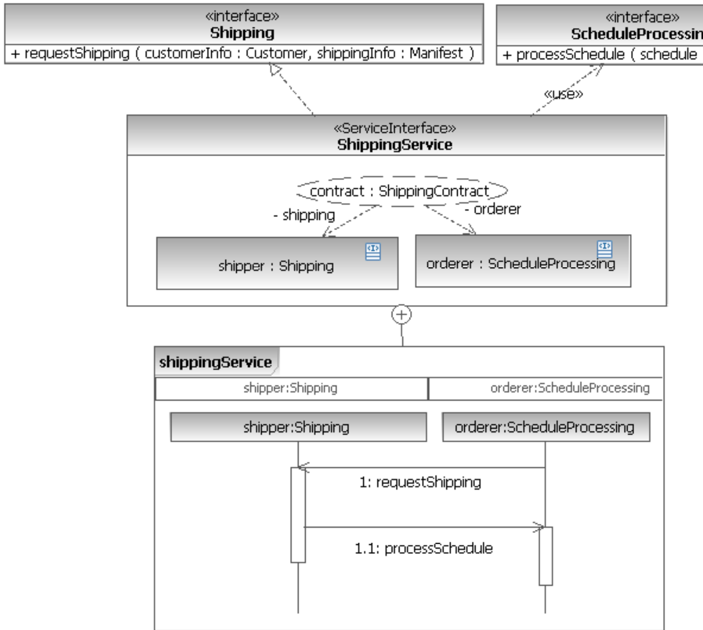
Figure 34: Fulfilling the ShippingContract ServiceContract
