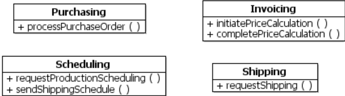
Figure 84: Interfaces Listing Role Responsibilities
