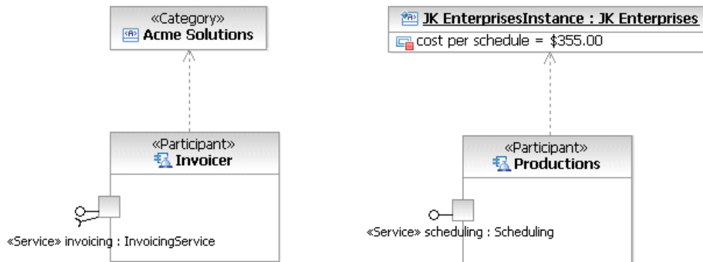
Figure 61: Notation to apply a Category or CategoryValue to a model element
