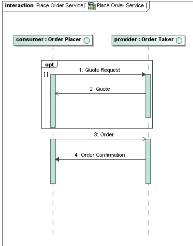
Figure 13 - Place Order Service Contract Choreography
