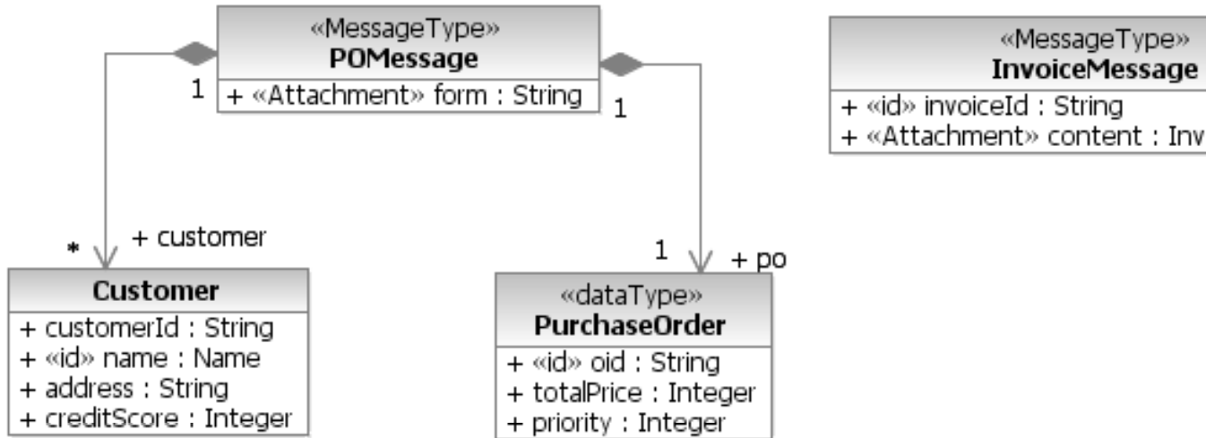
Figure 36: MessageTypes in Purchase Order Processing
