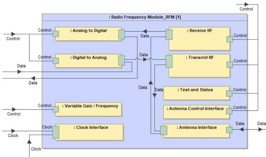
Figure 5: RFM Architecture Details (Detail of Figure 2)
