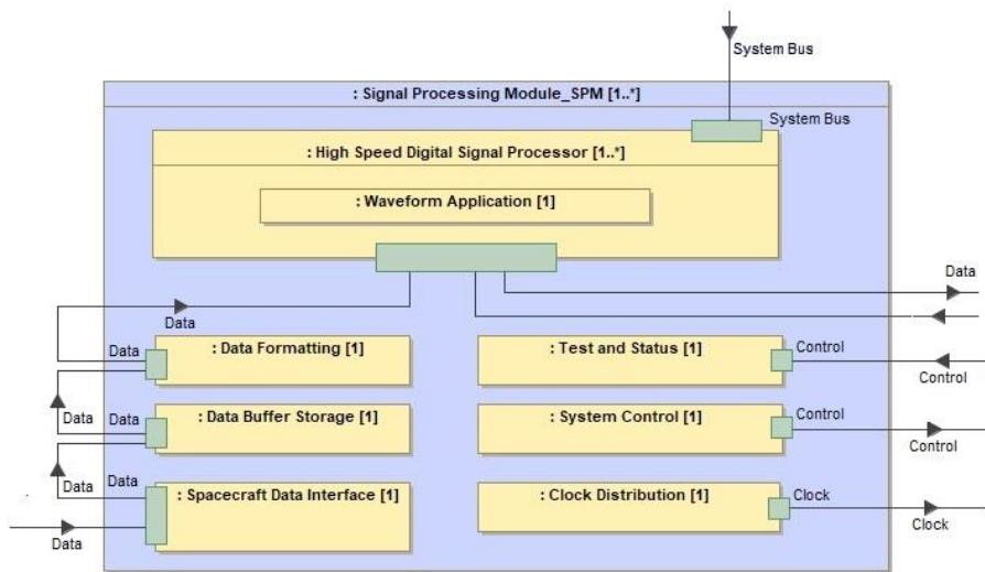
Figure 4: SPM Architecture Details (Detail of Figure 2)
