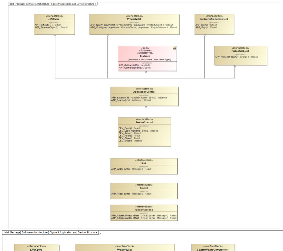
Figure 9 Figure 9, Application and Device Structure, shows a high-level overview of the STI software interface and object definitions.
