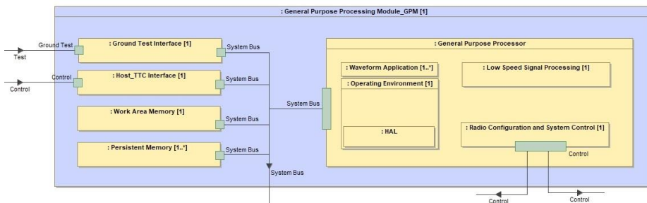
Figure 3: GPM Architecture Details (Detail of Figure 2)
