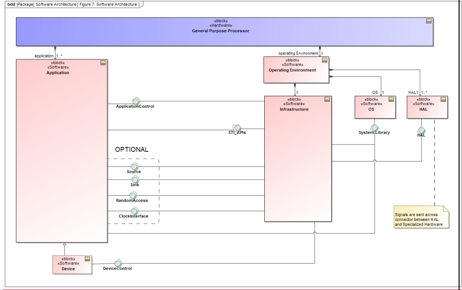
Figure 7: Layered Structure
