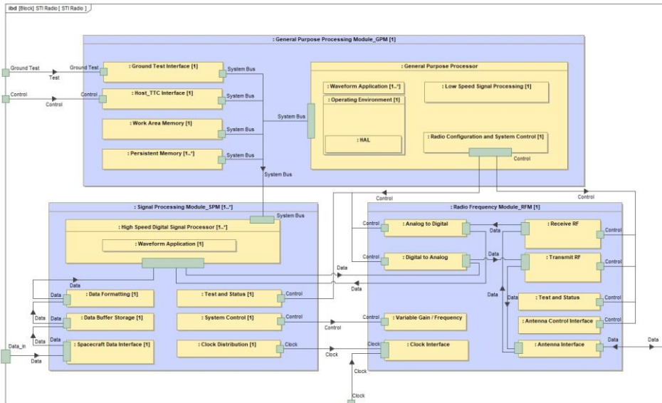
Figure 2: Notional STI Hardware Architecture
