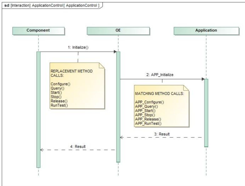
Figure 10: Sequence Diagram for Application Control Component
