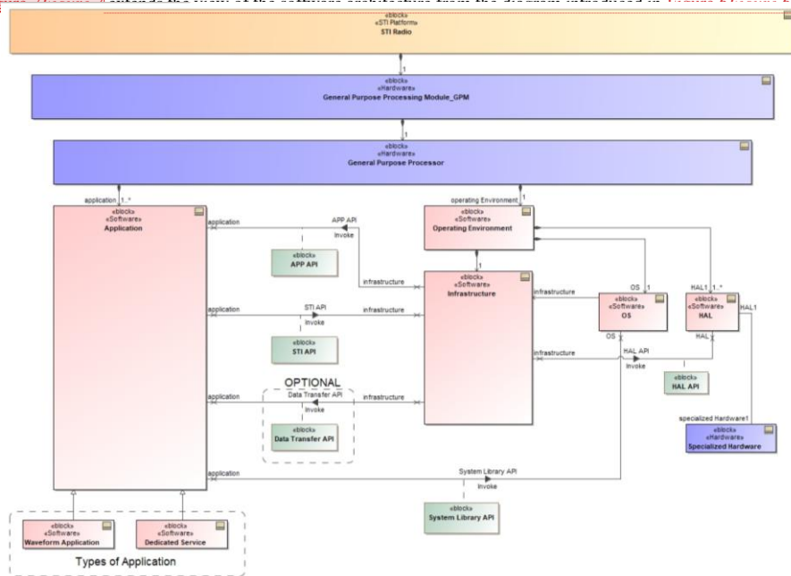
Fig. 7: Layered Structure of Software Architecture from the Diagram introduced in Figure 6
