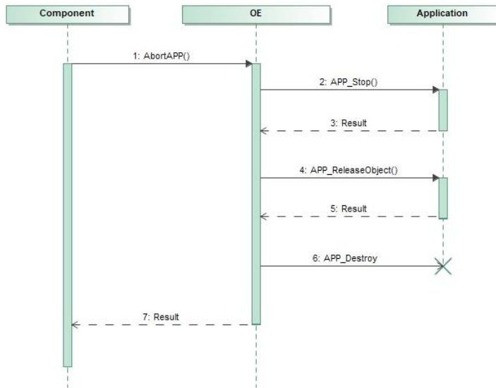
Figure 12: Sequence Diagram for AbortApp
