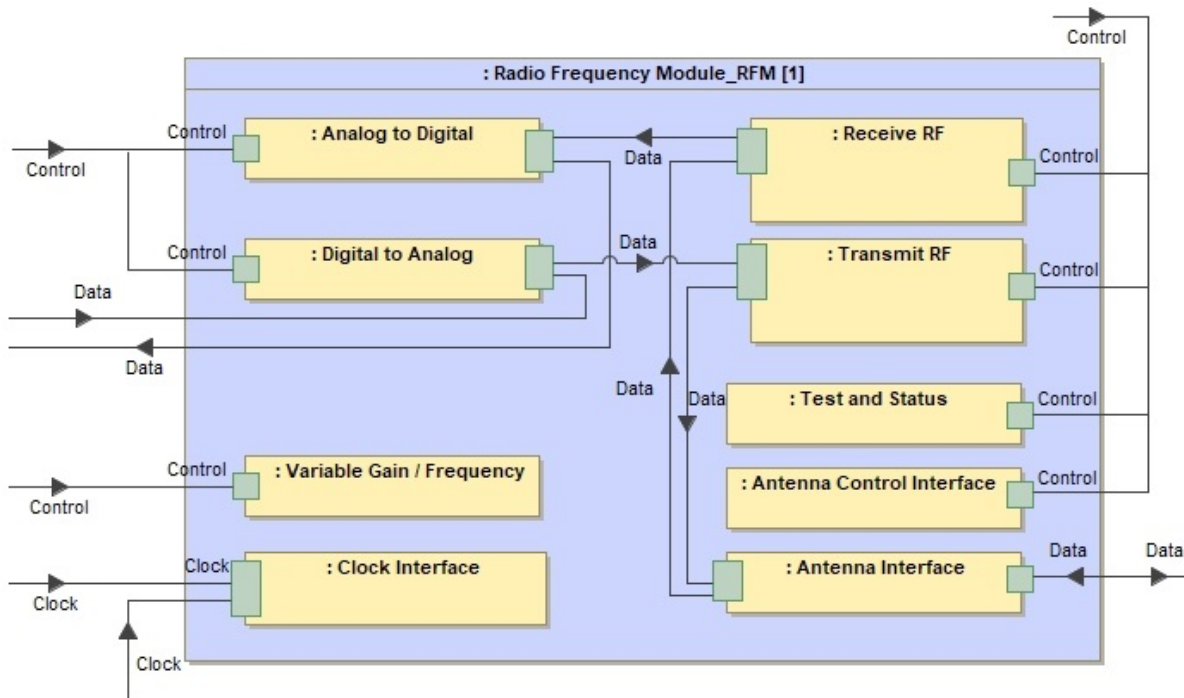
Figure 5: RFM Architecture Details
