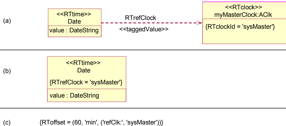
Figure 4-9 Three different ways of denoting references to a specific clock
