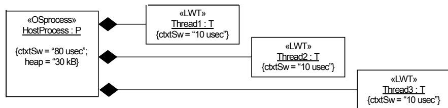
Figure 3-16 Example of a required environment specification
