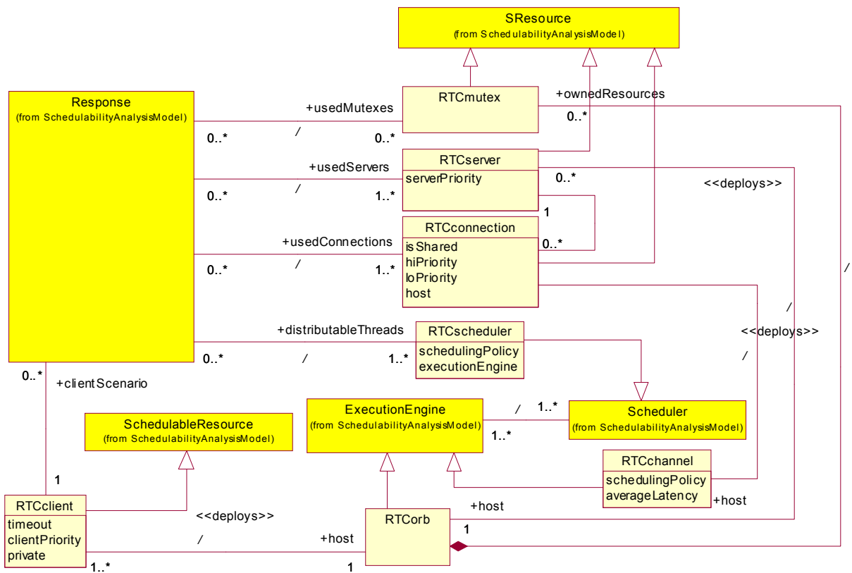
Figure 8-1 The Real-Time CORBA domain model
