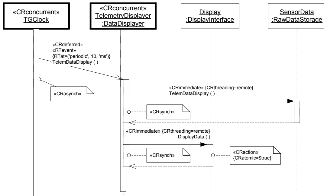
Figure 5-2 Concurrency Model - asynchronous case
