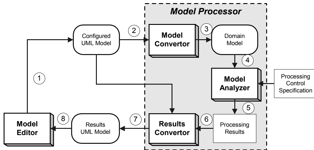
Figure 9-2 A simplified system without a model configurator
