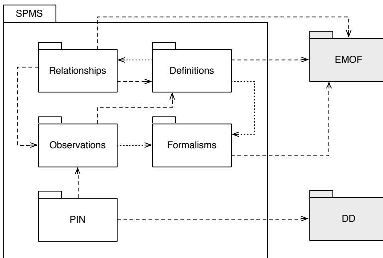
Figure 1: SPMS Metamodels Overview – Normative Packages
