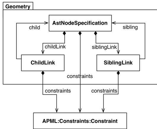
Figure 32: Geometry Package Diagram
