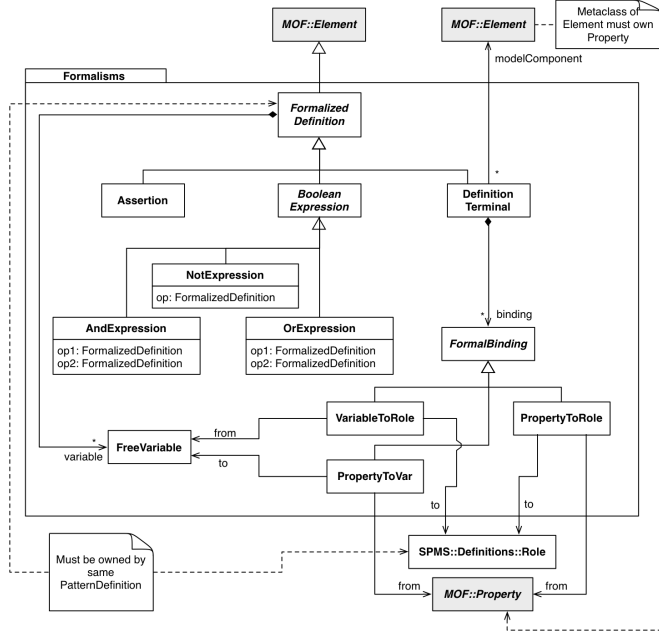
Figure 5: Formalisms package
