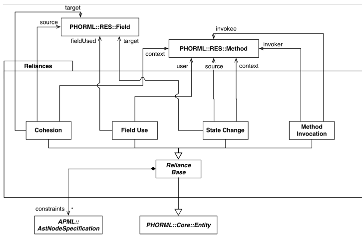
Figure 28: Reliances Package
