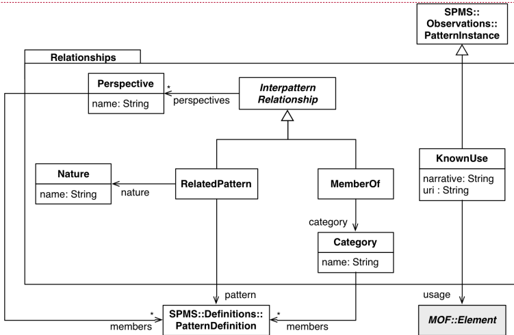
Figure 6: Relationships package
