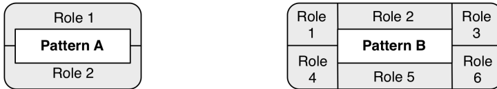
Figure 9: Standard PINbox
