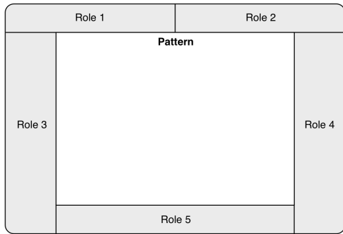
Figure 10: Expanded PINbox
