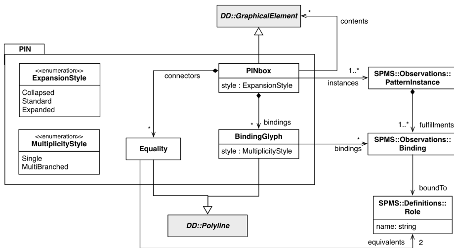
Figure 7: PIN Module
