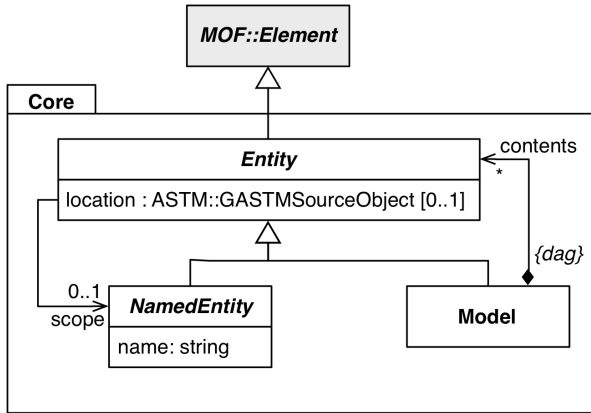
Figure 26: Core Package
