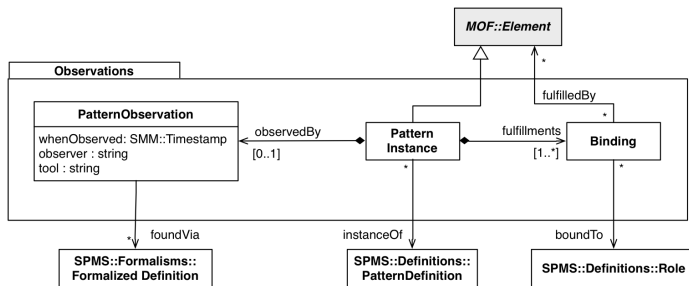
Figure 4: Observations Classes
