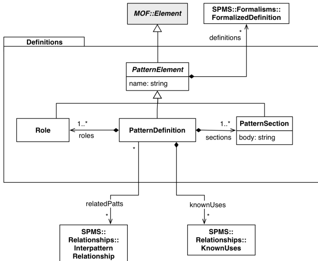
Figure 3: Definitions package
