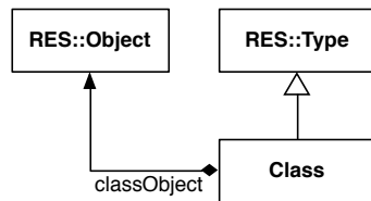
Figure 30: Class Object
