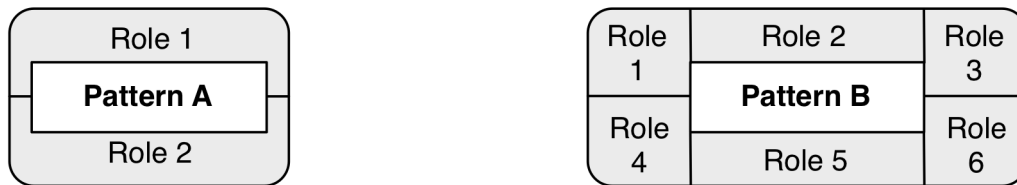
Figure 9: Standard PINbox
