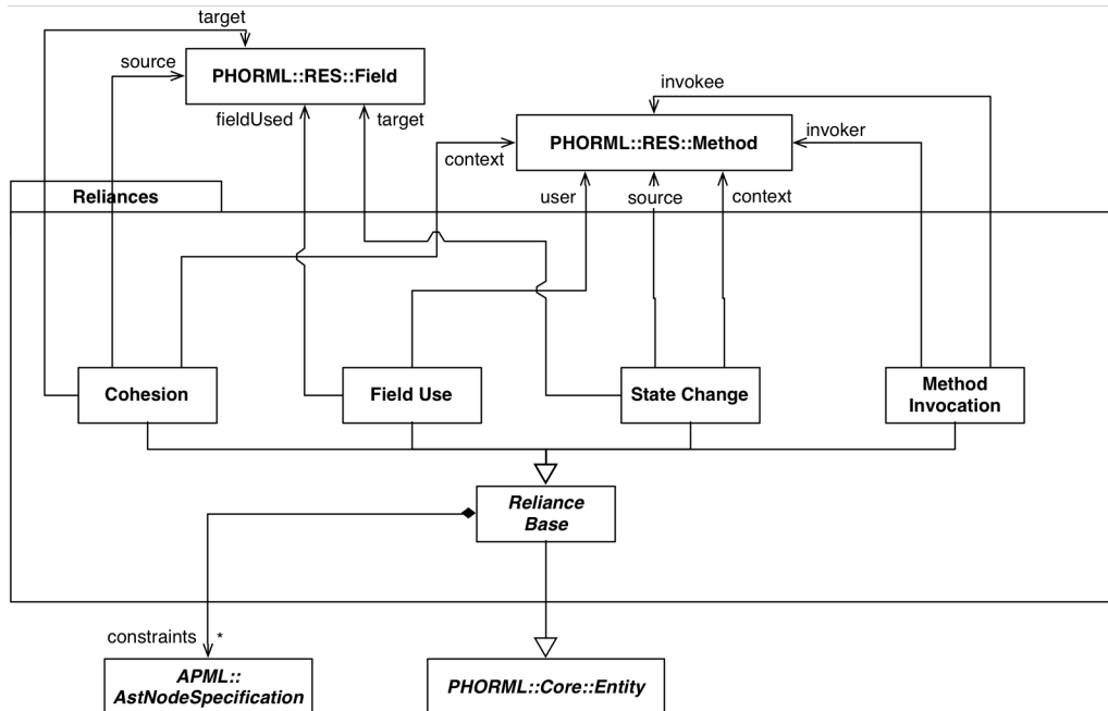
Figure 28: Reliances Package
