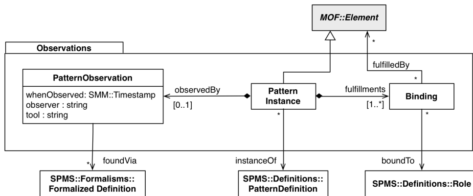
Figure 4: Observations Classes
