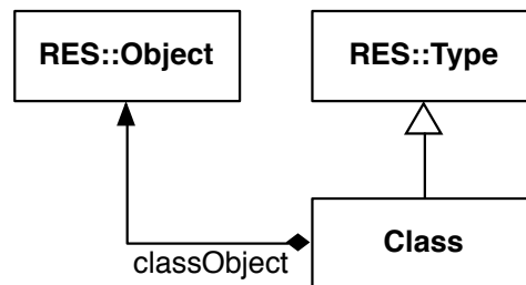
Figure 30: Class Object
