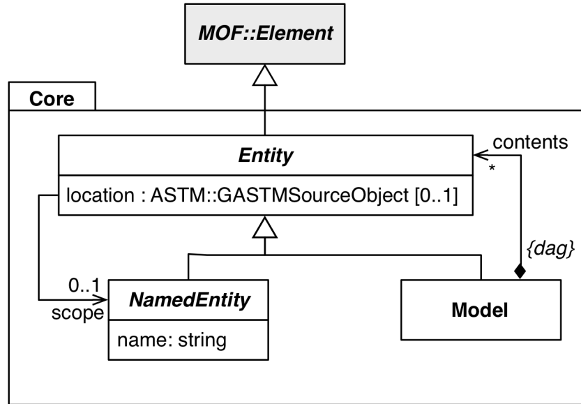
Figure 26: Core Package
