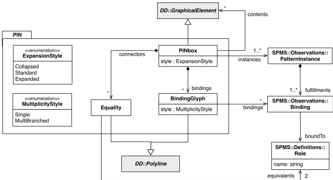
Figure 7: PIN Module
