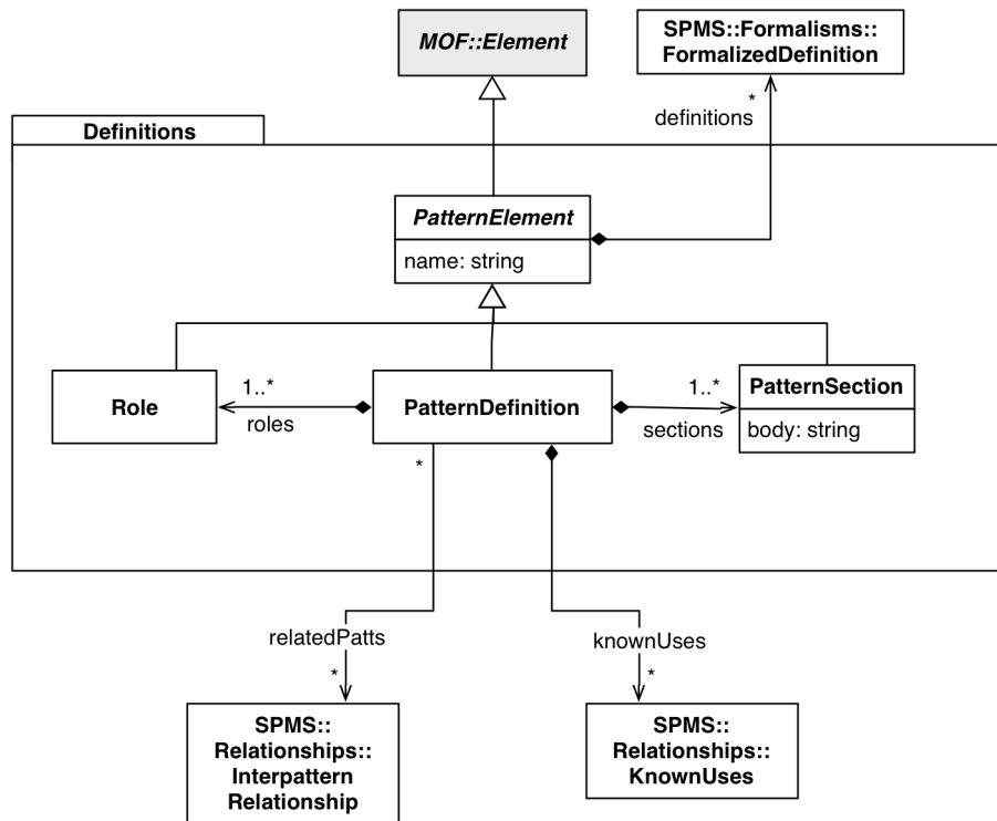
Figure 3: Definitions package
