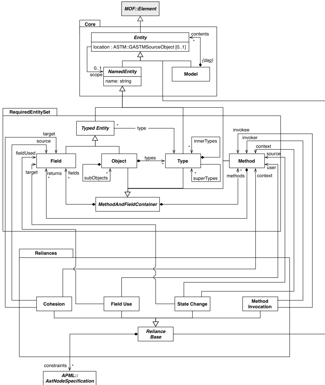
Figure 25: Complete PHORML
