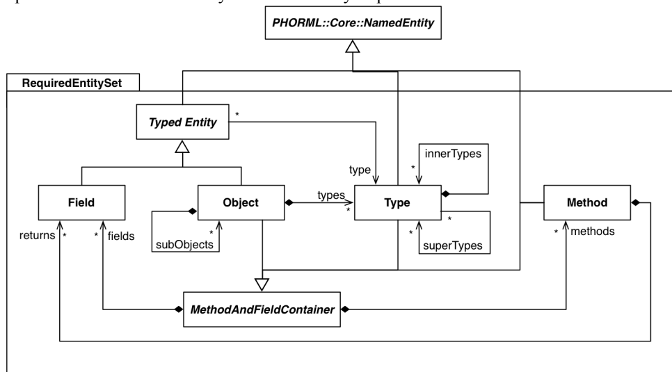
Figure 27: Required Entity Set
