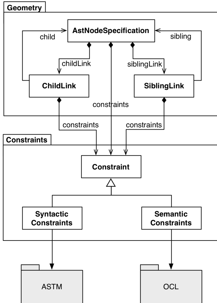
Figure 31: High Level (Composite) Diagram
