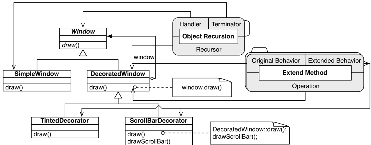
Figure 24: Peeled Decorator instances
