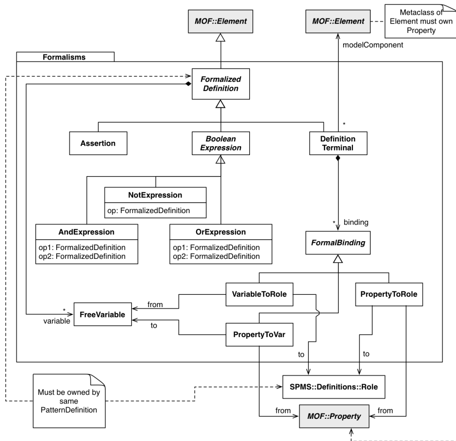
Figure 5: Formalisms package
