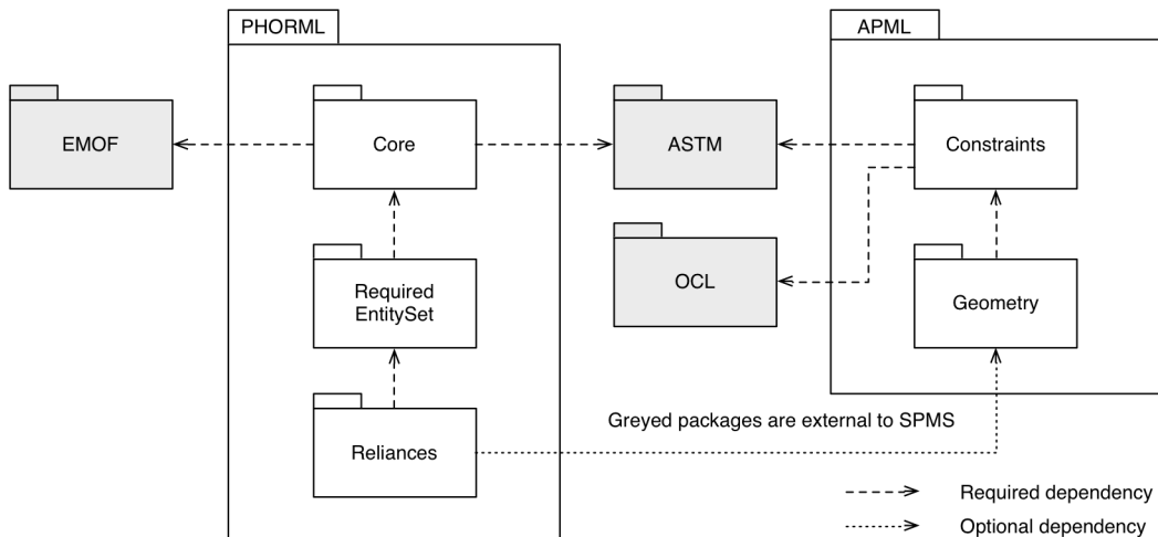
Figure 2: SPMS Metamodels Overview – Non-Normative Packages
