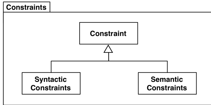
Figure 33: Constraint Package Diagram
