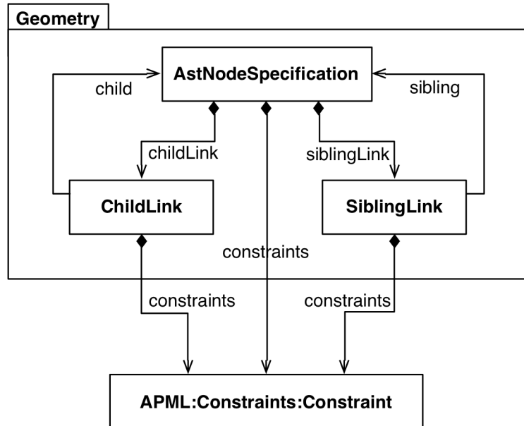
Figure 32: Geometry Package Diagram
