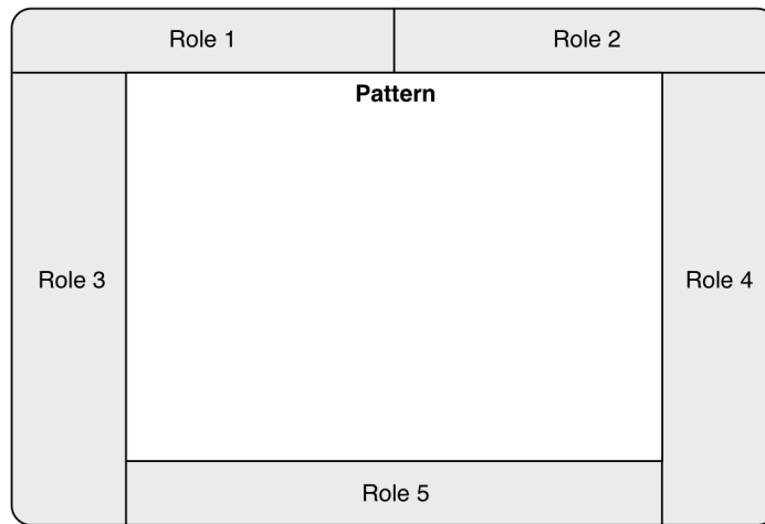
Figure 10: Expanded PINbox
