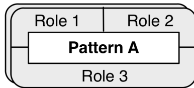
Figure 18: Stacked PINbox
