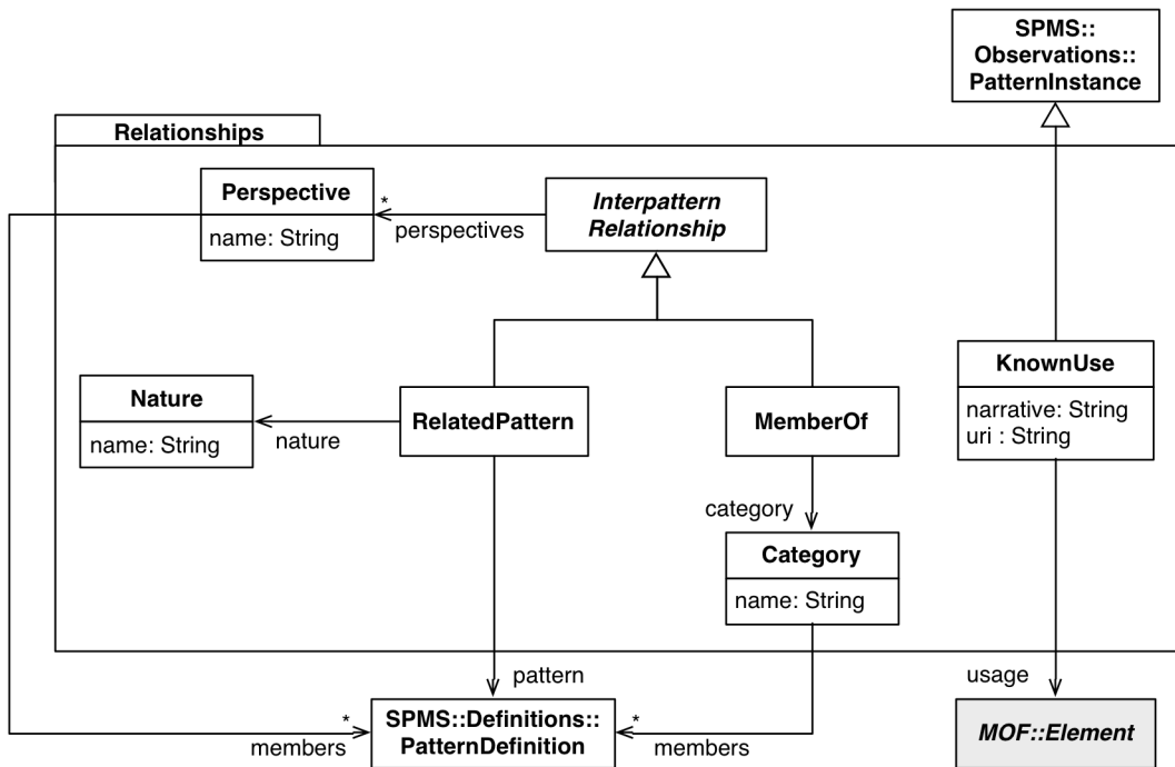
Figure 6: Relationships package
