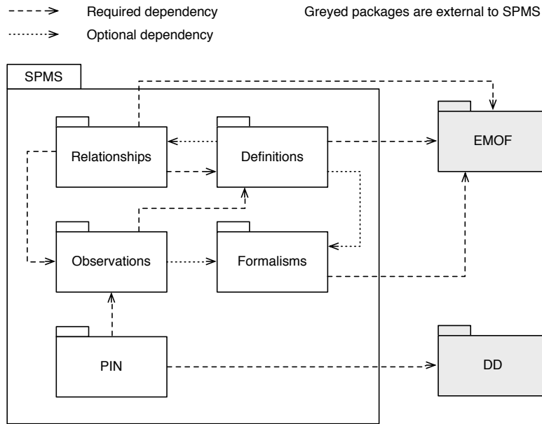
Figure 1: SPMS Metamodels Overview – Normative Packages
