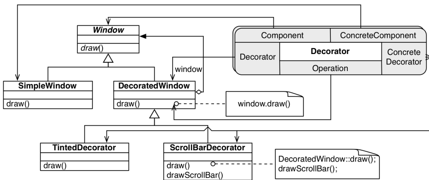
Figure 21: Stacked PINbox of Decorator instances with MultiBranch annotation on Decorator Role
