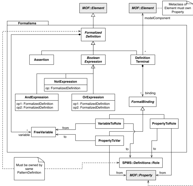
Figure 5: Formalisms package
