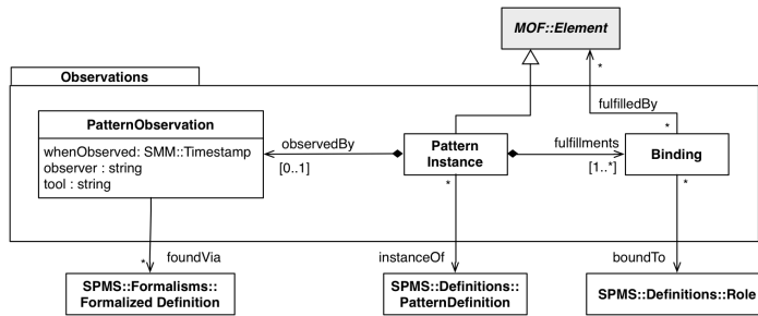
Figure 4: Observations Classes
