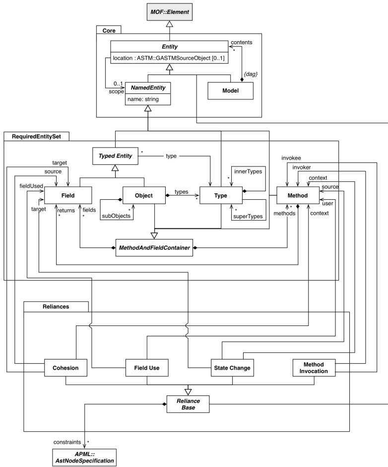
Figure 25: Complete PHORML
