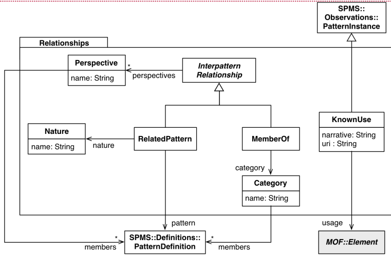
Figure 6: Relationships package
