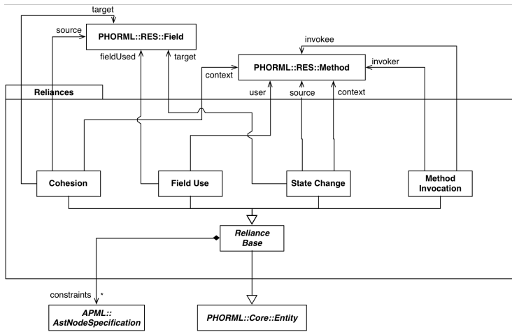
Figure 28: Reliances Package
