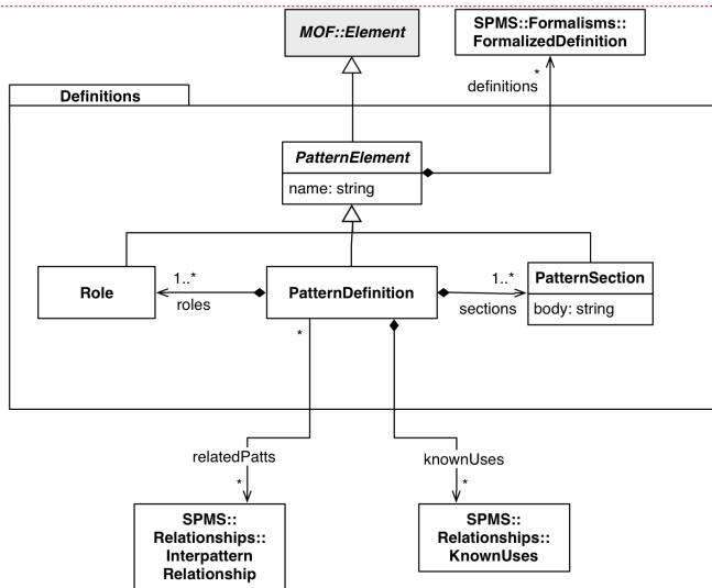
Figure 3: Definitions package
