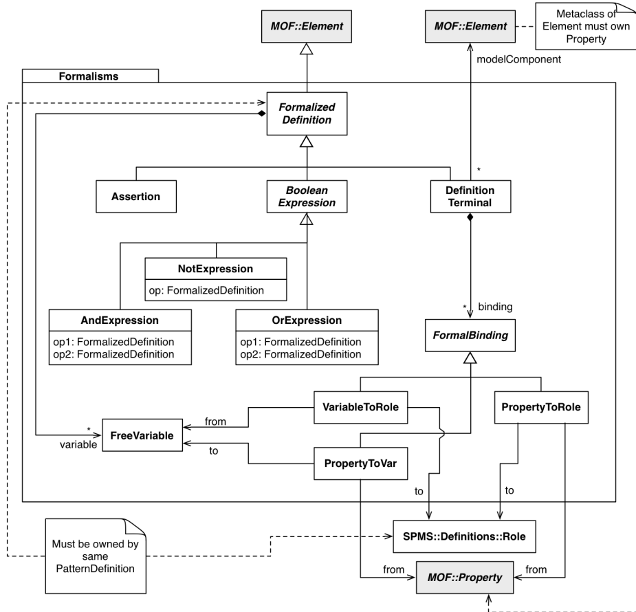
Figure 5: Formalisms package
