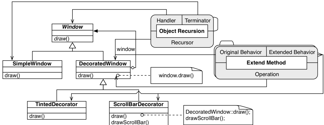
Figure 24: Peeled Decorator instances
