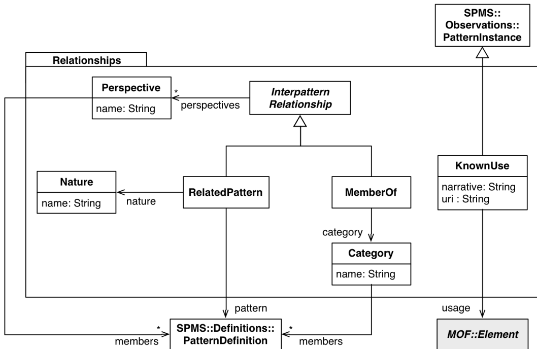
Figure 6: Relationships package
