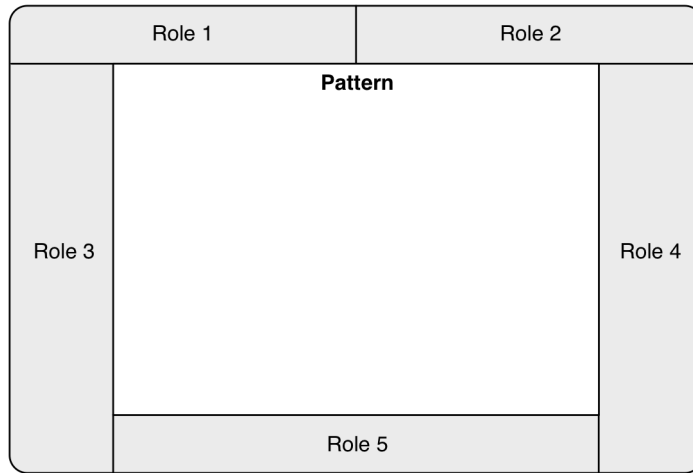
Figure 10: Expanded PINbox
