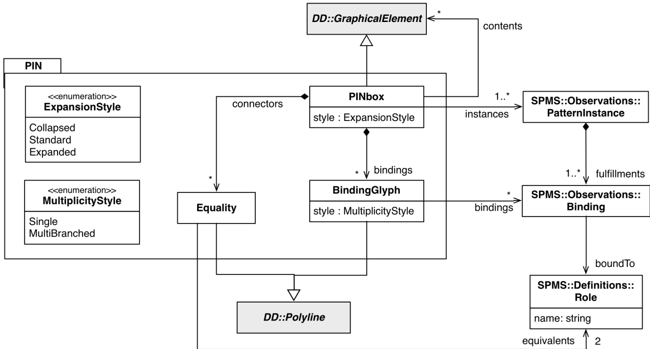
Figure 7: PIN Module
