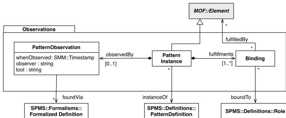
Figure 4: Observations Classes
