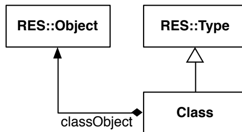
Figure 30: Class Object
