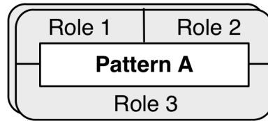
Figure 18: Stacked PINbox
