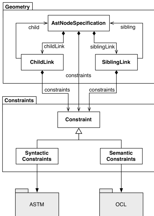
Figure 31: High Level (Composite) Diagram
