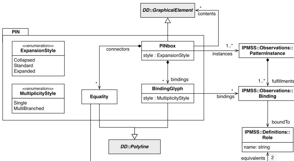
Figure 7: PIN Module
