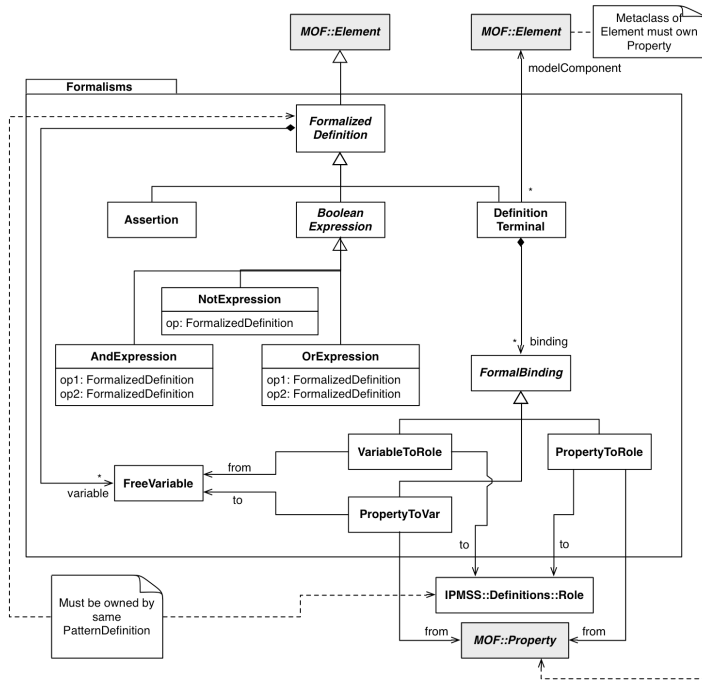
Figure 5: Formalisms package
