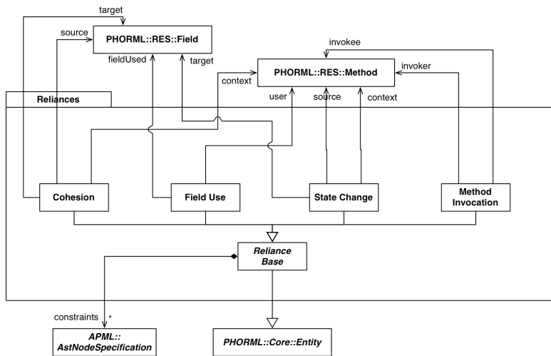
Figure 28: Reliances Package
