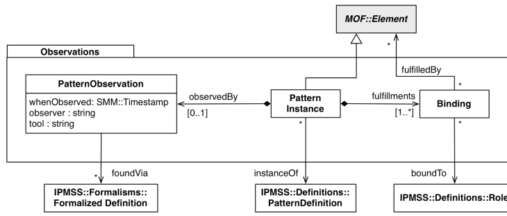
Figure 4: Observations Classes
