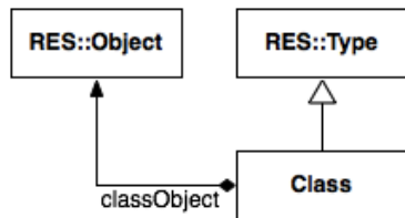
Figure 30: Class Object
