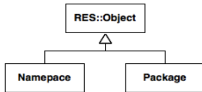
Figure 29: Namespace and Package Object
