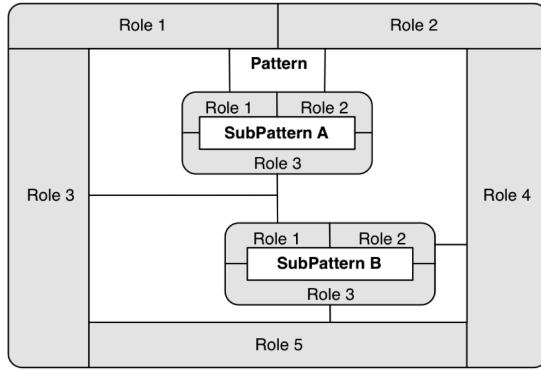
Figure 12: Expanded PINbox illustrating internal PINbox diagram
