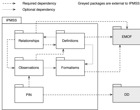
Figure 1: IPMSS Metamodels Overview – Normative Packages
