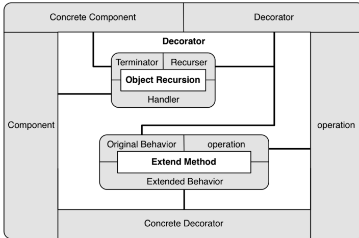
Figure 13: Decorator as an Expanded PINbox with internal PINbox definition
