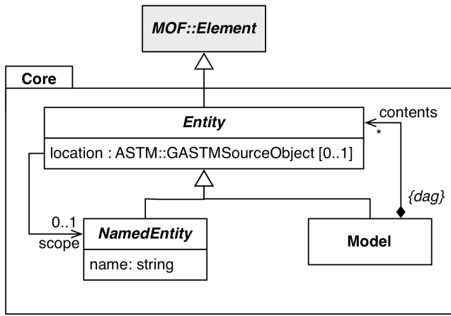
Figure 26: Core Package
