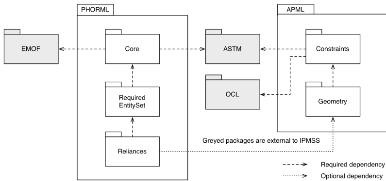
Figure 2: IPMSS Metamodels Overview – Non-Normative Packages
