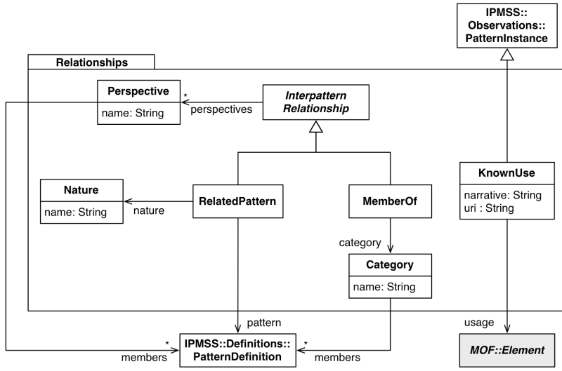
Figure 6: Relationships package
