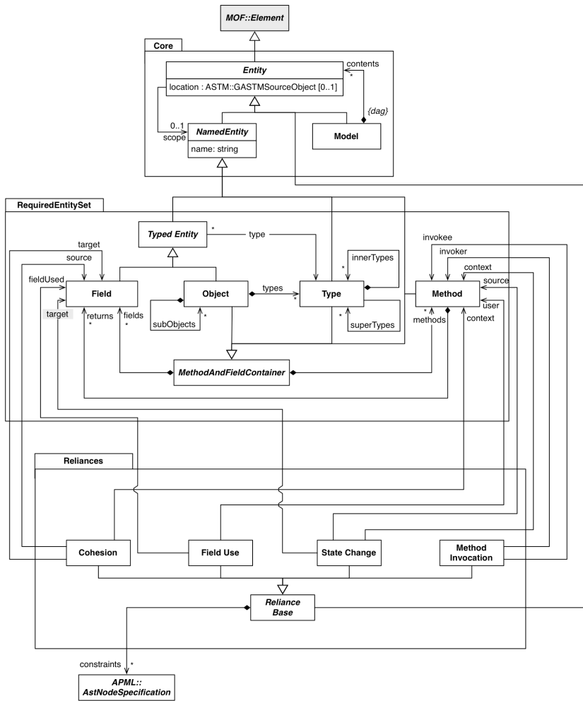
Figure 25: Complete PHORML
