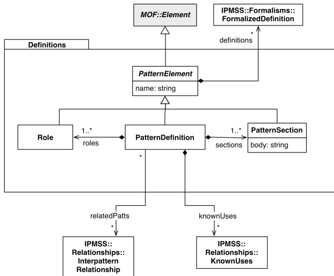
Figure 3: Definitions package
