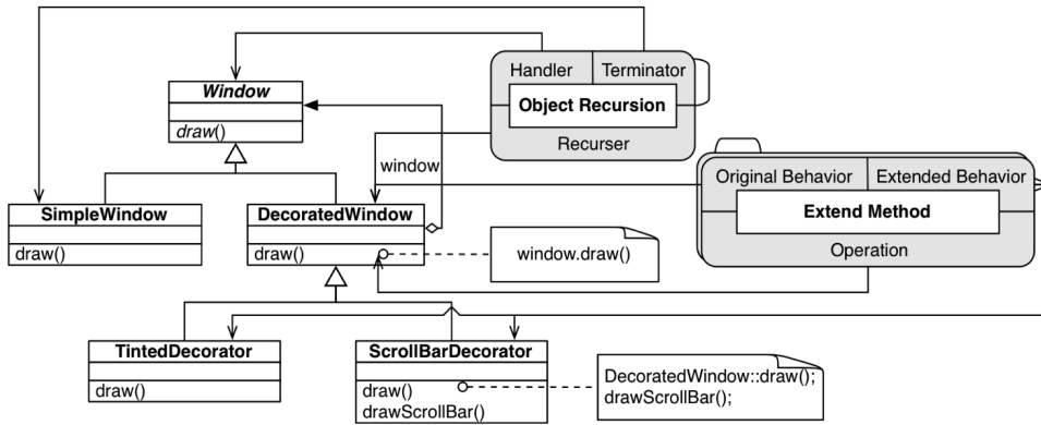
Figure 24: Peeled Decorator instances
