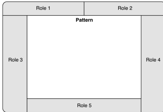
Figure 10: Expanded PINbox
