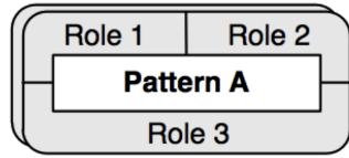
Figure 18: Stacked PINbox
