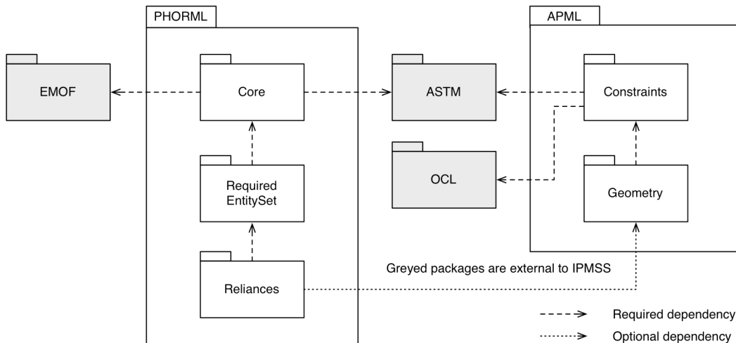
Figure 2: IPMSS Metamodels Overview – Non-Normative Packages
