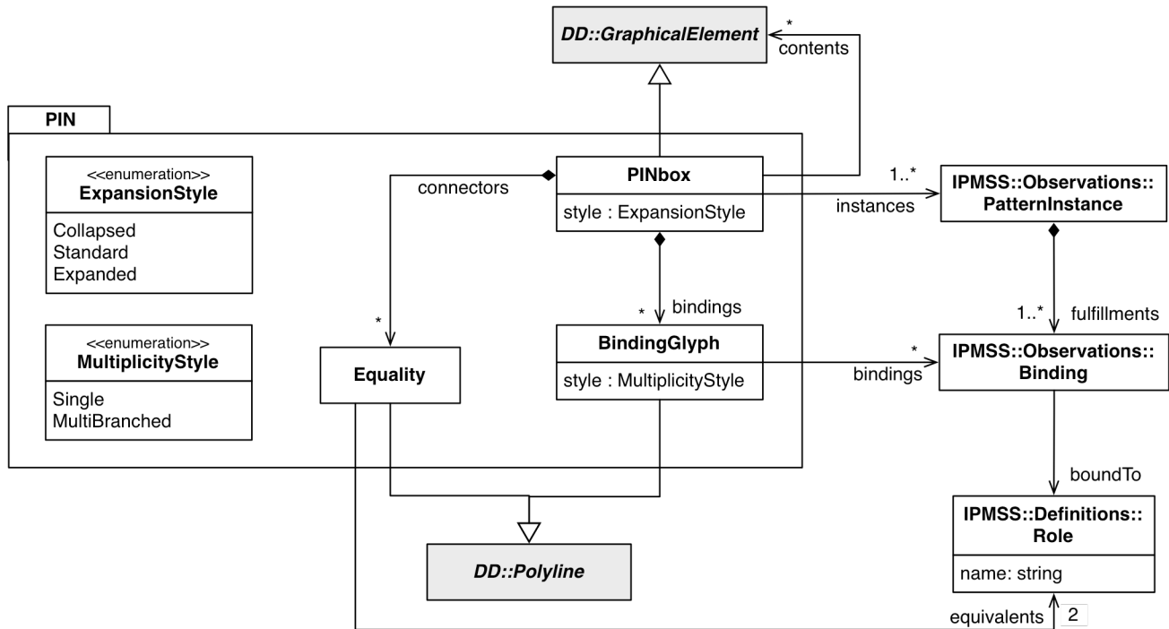
Figure 7: PIN Module
