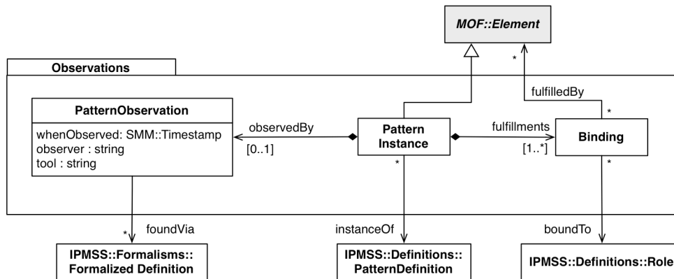
Figure 4: Observations Classes
