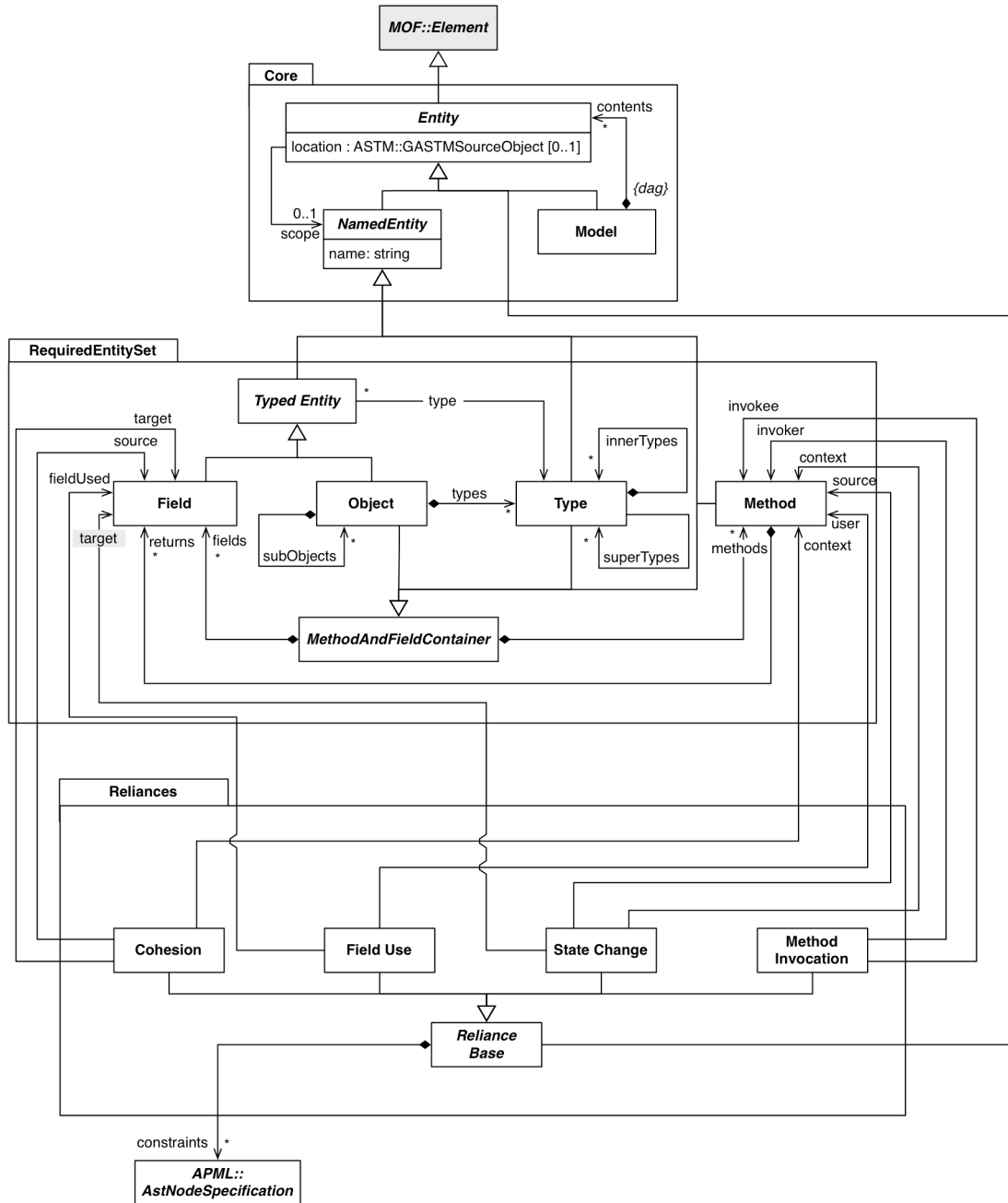
Figure 25: Complete PHORML
