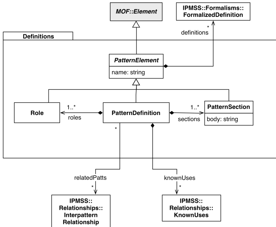
Figure 3: Definitions package
