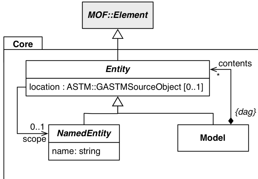
Figure 26: Core Package
