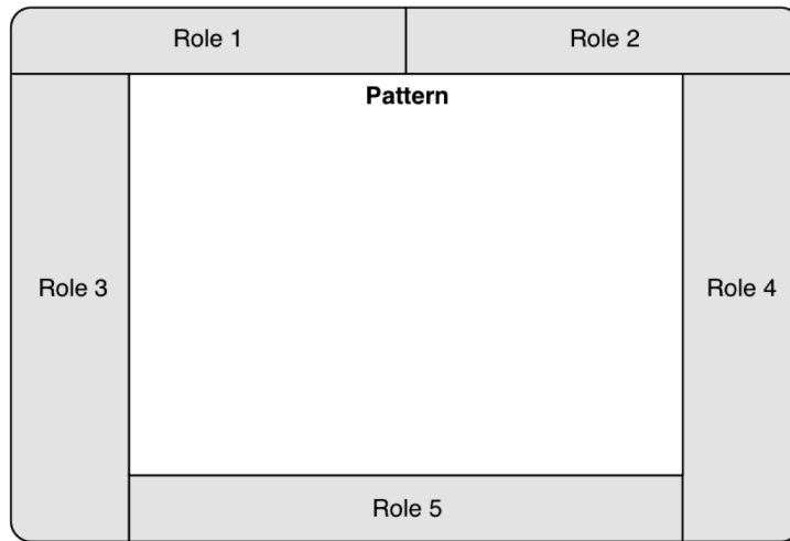
Figure 10: Expanded PINbox
