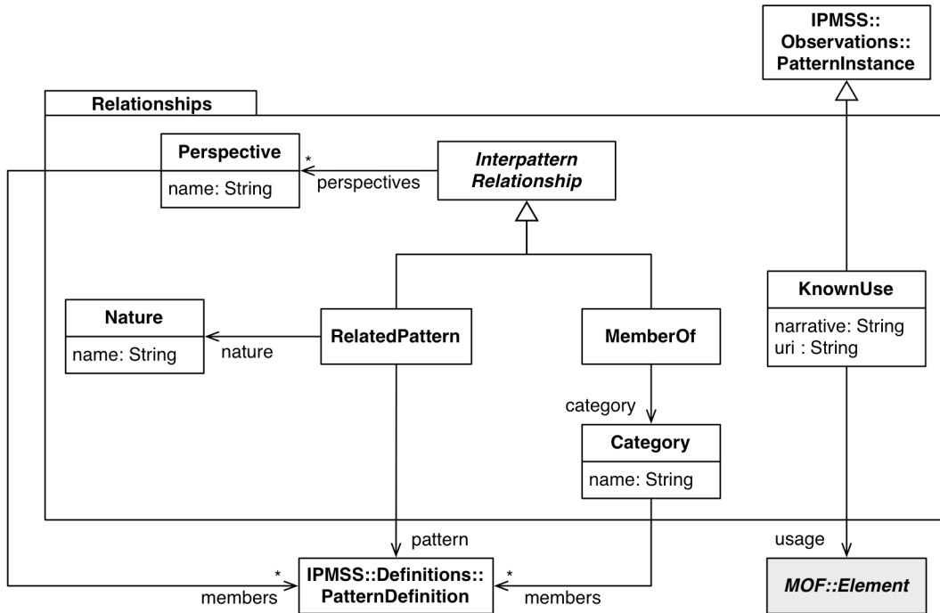
Figure 6: Relationships package
