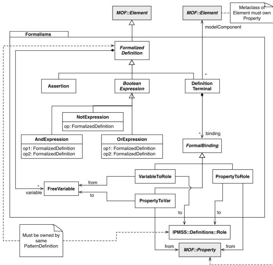
Figure 5: Formalisms package
