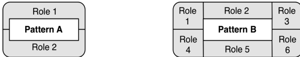
Figure 9: Standard PINbox
