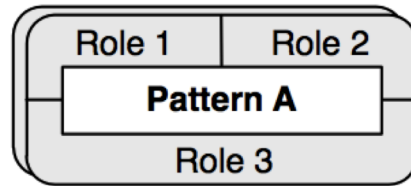
Figure 18: Stacked PINbox
