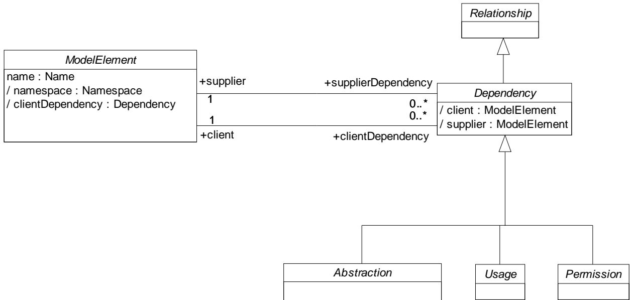
Figure 2-6 Foundation Core Package — Dependencies
