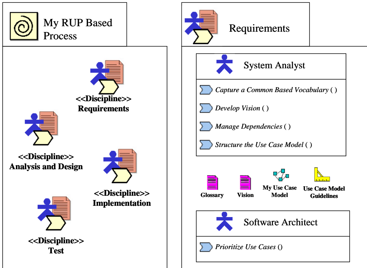
Figure 12-2 Example of Package Diagram
