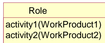
Figure 3-1 Conceptual Model
