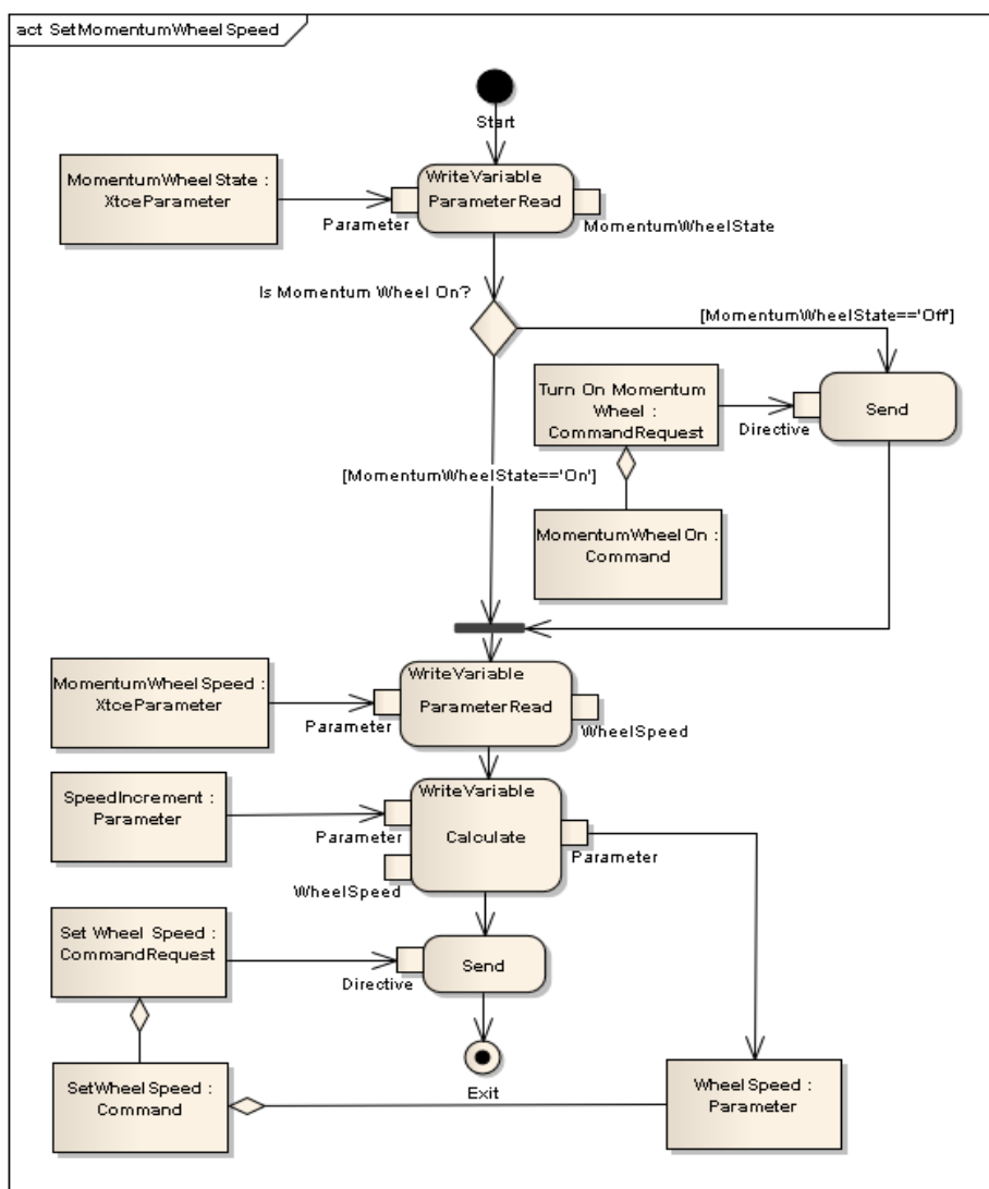
Figure 4 - Notional SOLM Procedure Activity Diagram (Non-Normative)
