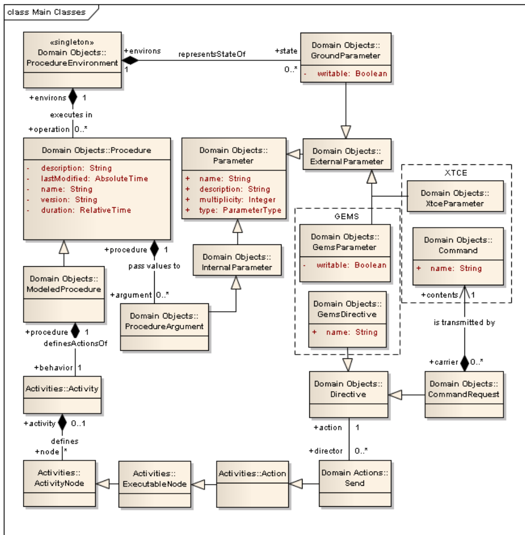
Figure 5 - Key SOLM Classes
