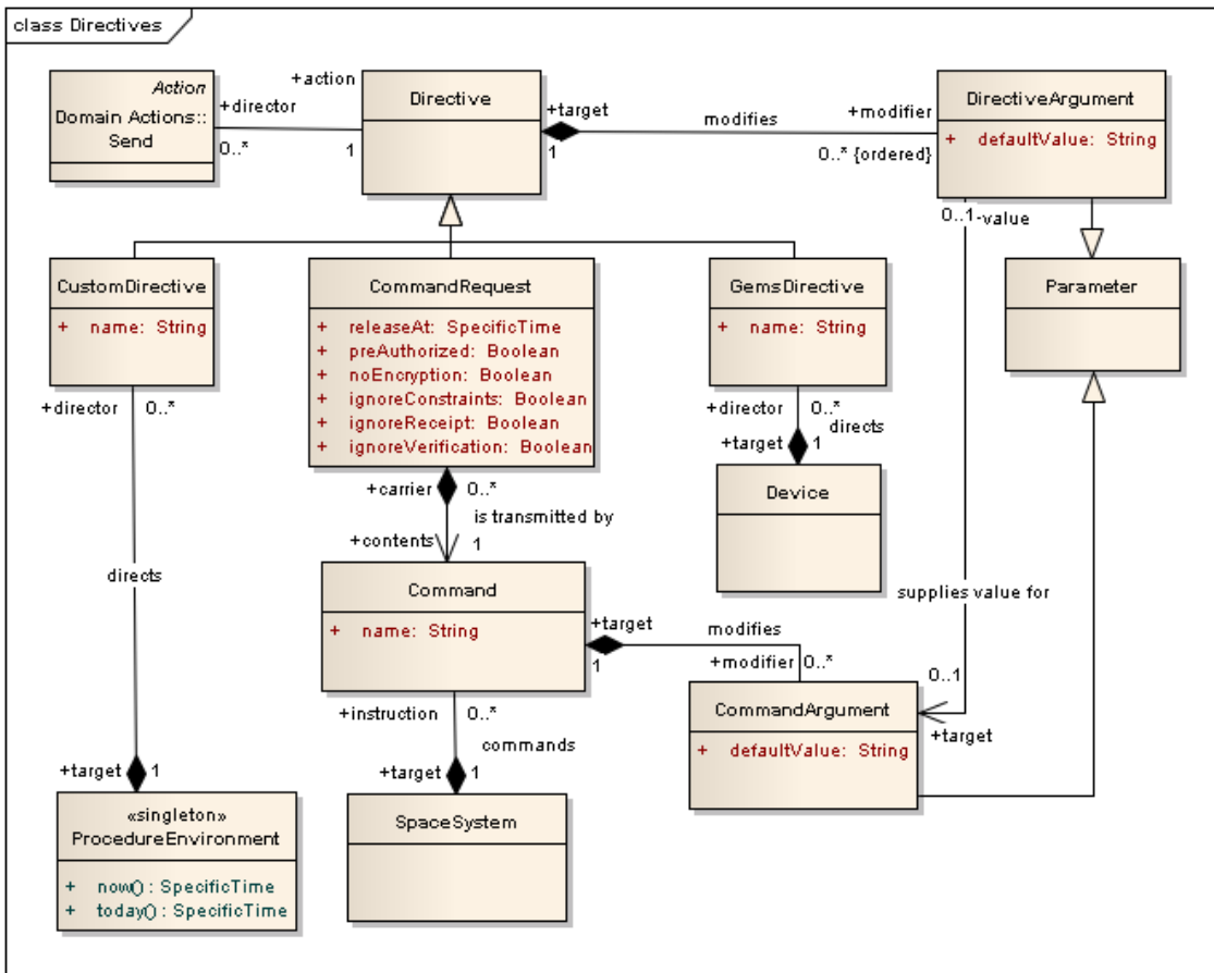
Figure 13 - Directives: CommandRequests and GemsDirectives
