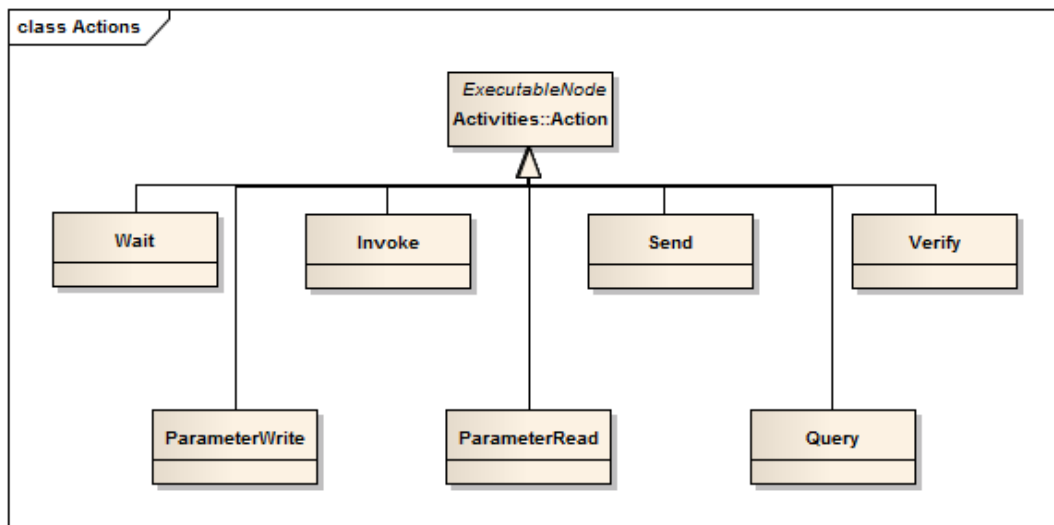
Figure 14 - SOLM Action Nodes for Activity Diagrams
