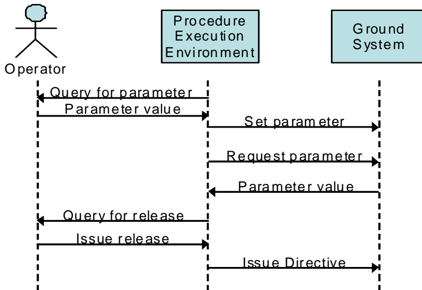
Figure 3 - Notional System Sequence Diagram (Non-Normative)
