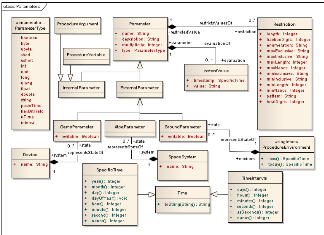
Figure 11 - GEMS and XTCE Parameters
