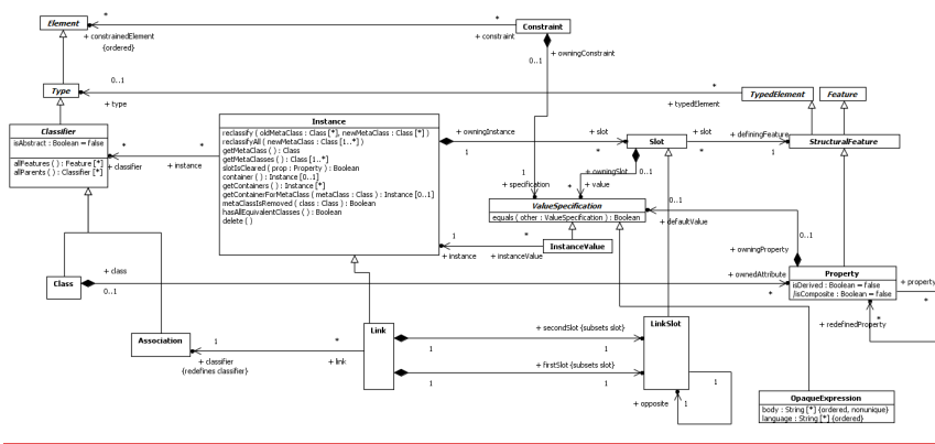
Figure 4 – SMOFAbstractDomainModel package
