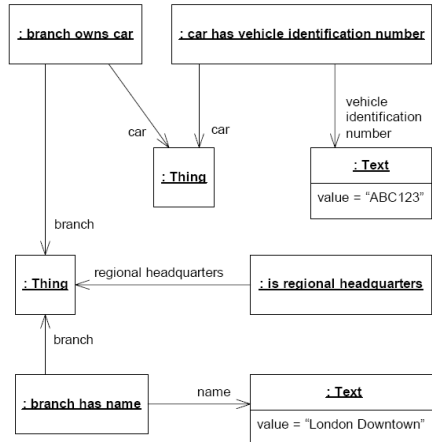
Figure L.2 - Instance diagram of facts expressed using EU-Rent English Vocabulary
