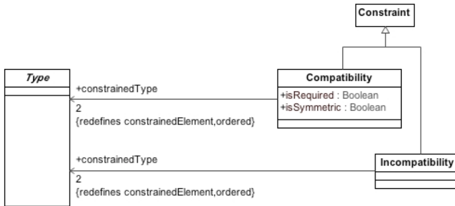
Figure 3 - SMOF Classification Constraints
