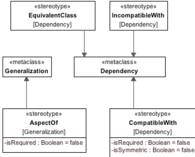
Figure 6.- SMOF Profile
