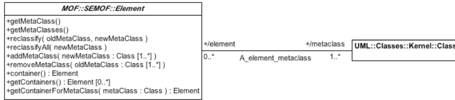
Figure 2 – Reflection, as extended by SMOF
