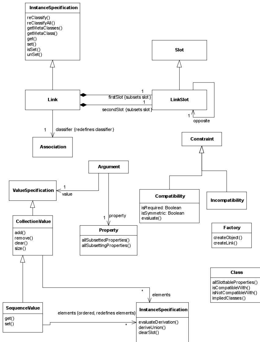
Figure 5 – AbstractDomainModel package
