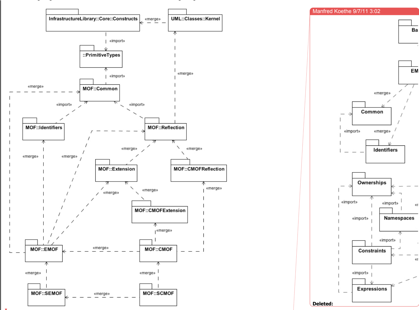
Figure 1 - The SMOF Packages in relation to the EMOF / CMOF Packages
