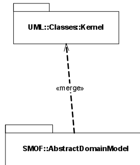
Figure 4 – Semantic Domain Model Package
