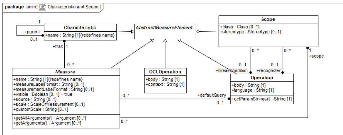
Figure 10.1 - Measurable Characteristic and Scope
