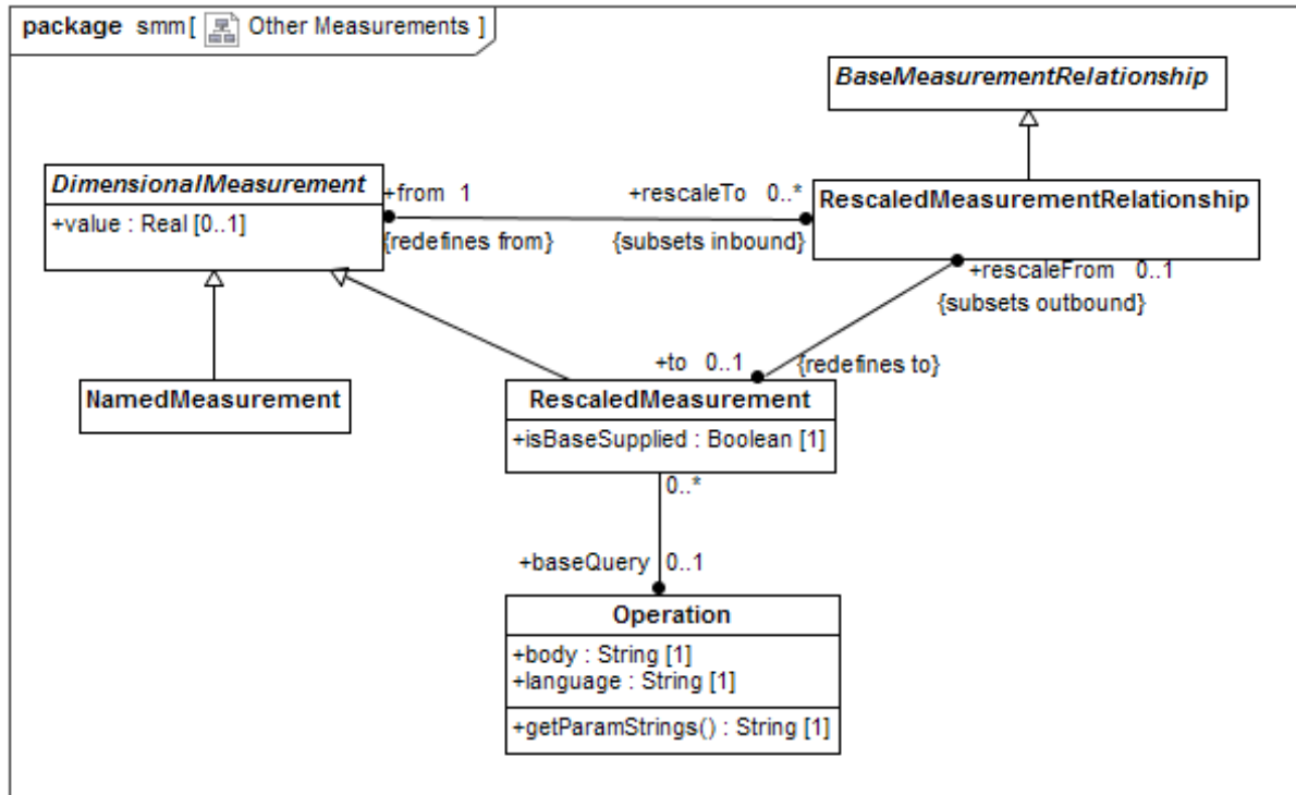
Figure 15.1 - Named and Rescaled Measurements
