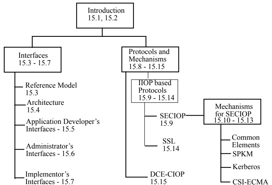
Figure 15-1 Structure of the Document
