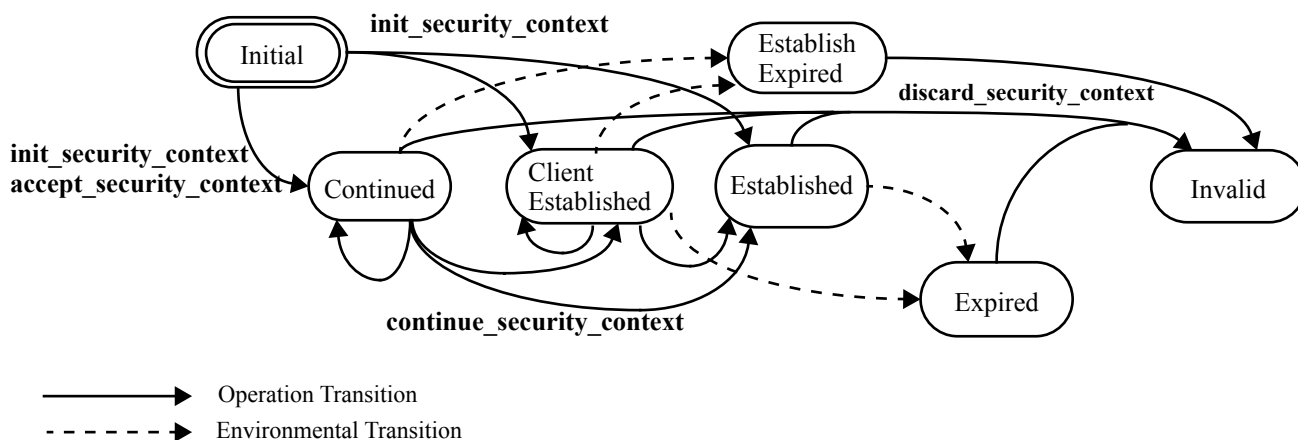
Figure 15-55 Security Context State Transition Diagram
