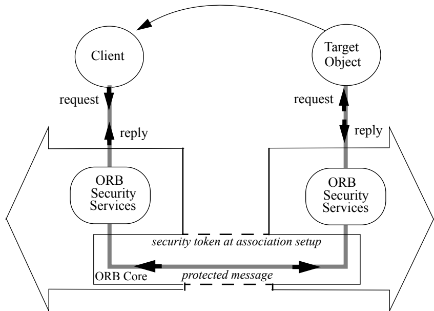
Figure 15-55 Model for Secure Interoperability
