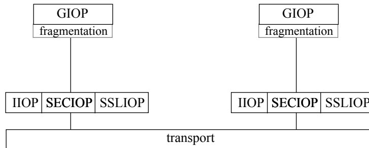
Figure 15-58 Position of SECIOP Protocol
