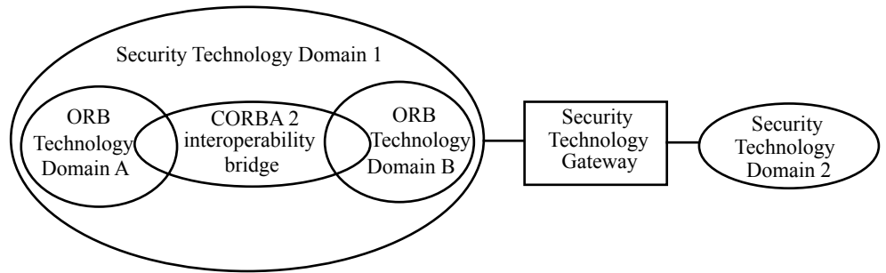
Figure 15-23 Framework of Domains
