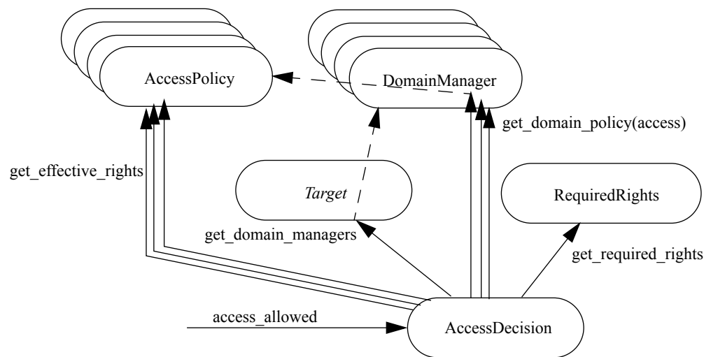
Figure 15-69 Supporting Overlapping Access Policy Domains
