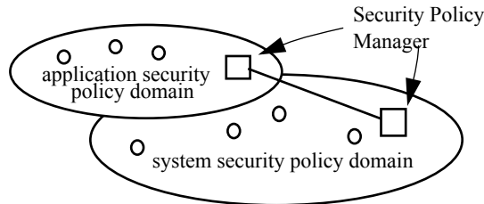
Figure 15-21 System- and Application-enforced Policies
