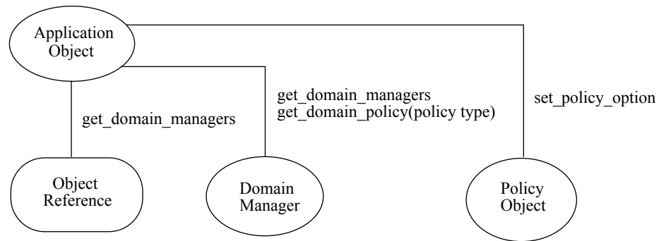
Figure 15-46 Managing Security Policies
