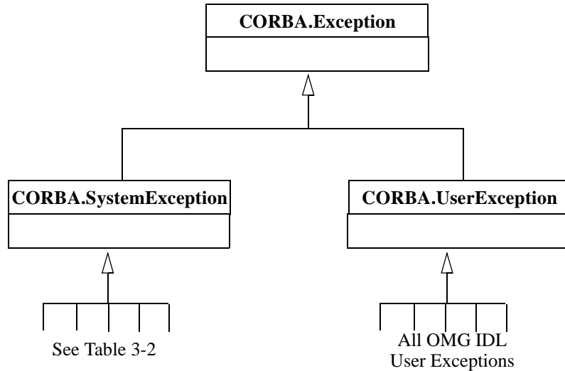
Figure 3-1 The CORBA Exception Type Hierarchy
