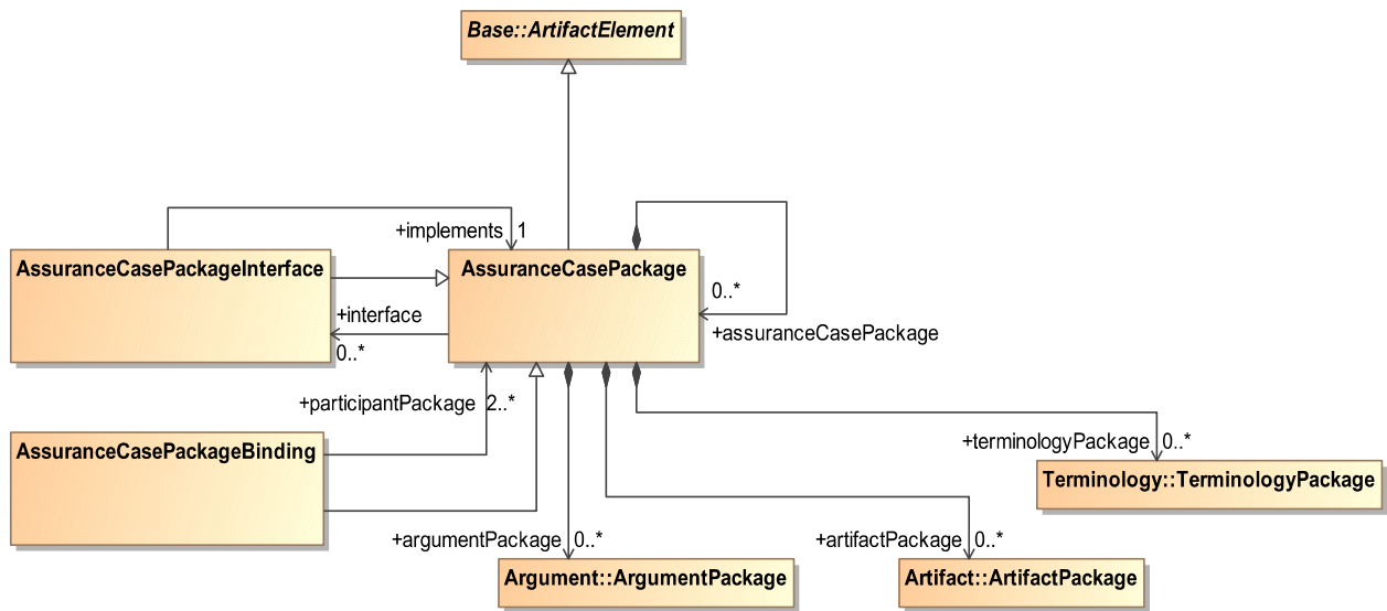
Figure 9.19.1 - Structured Assurance Case Packages Class Diagram
