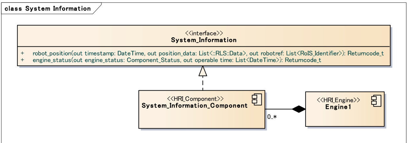
Figure 17 - System Information
