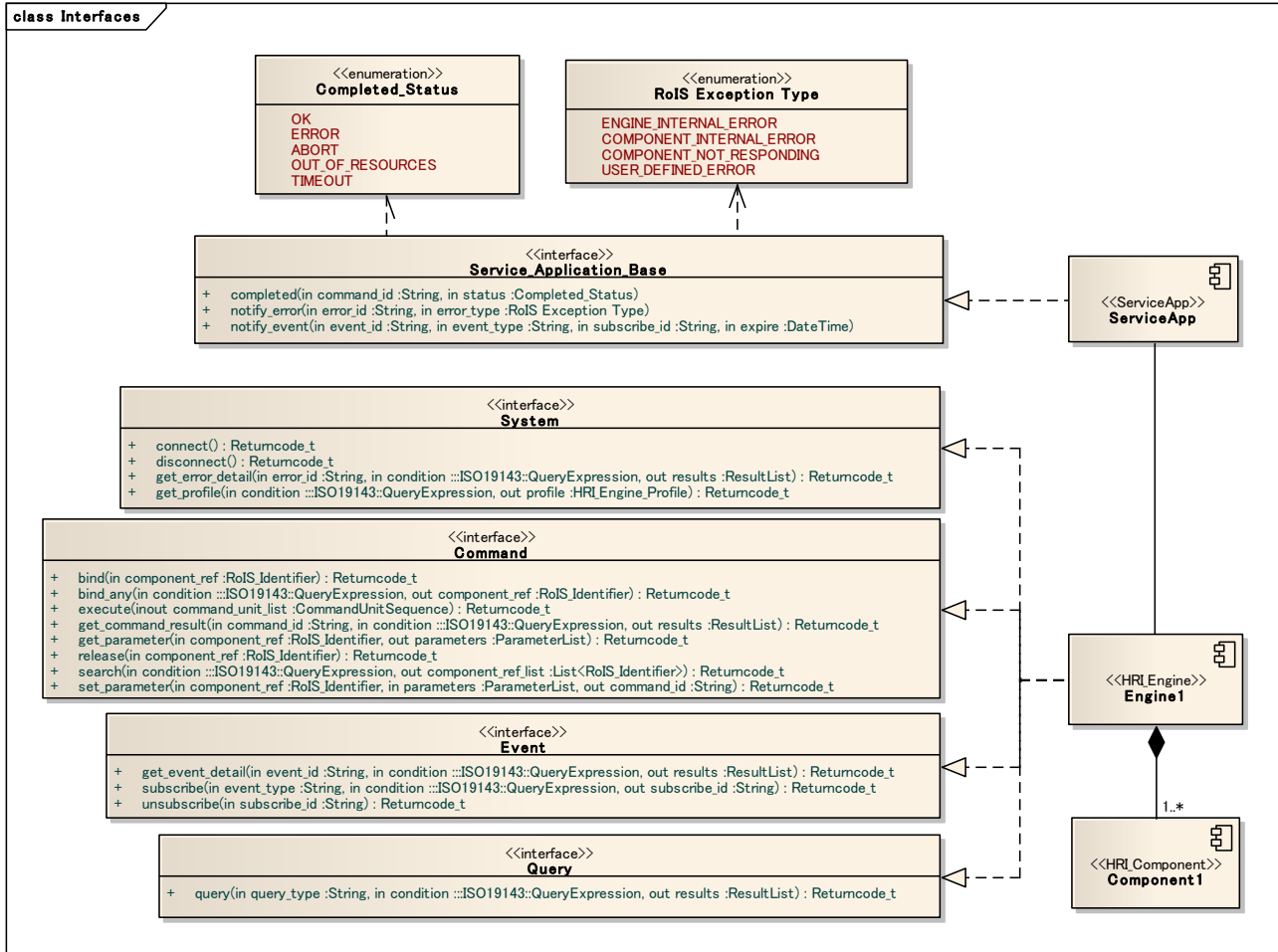
Figure 14 : RoIS Interfaces.
