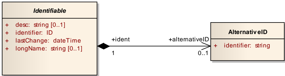
Figure 10.2 – Primary and alternative identifier
