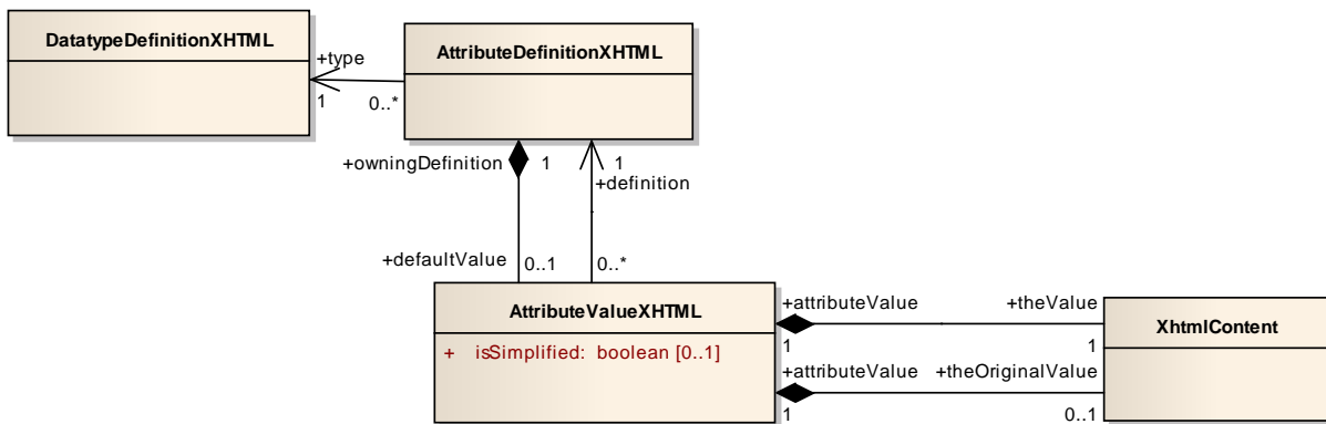
Figure 10.12 - Data types for XHTML content
