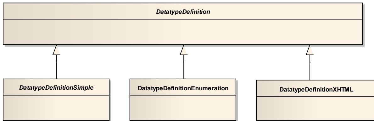
Figure 10.8 - DatatypeDefinition class hierarchy
