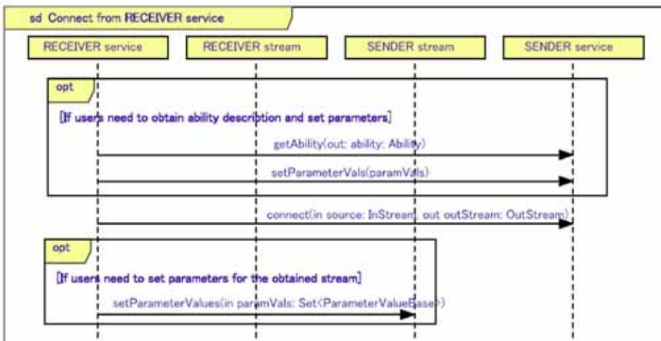
Figure 7.24 - Sequence Diagram of Connection Establishment from RECEIVER Service
