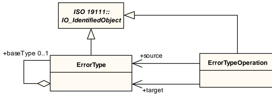
Figure 7.9 - RoLo Error Types
