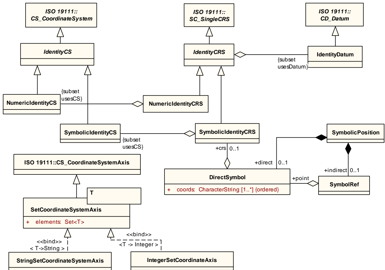
Figure 7.7 - Identity Information
