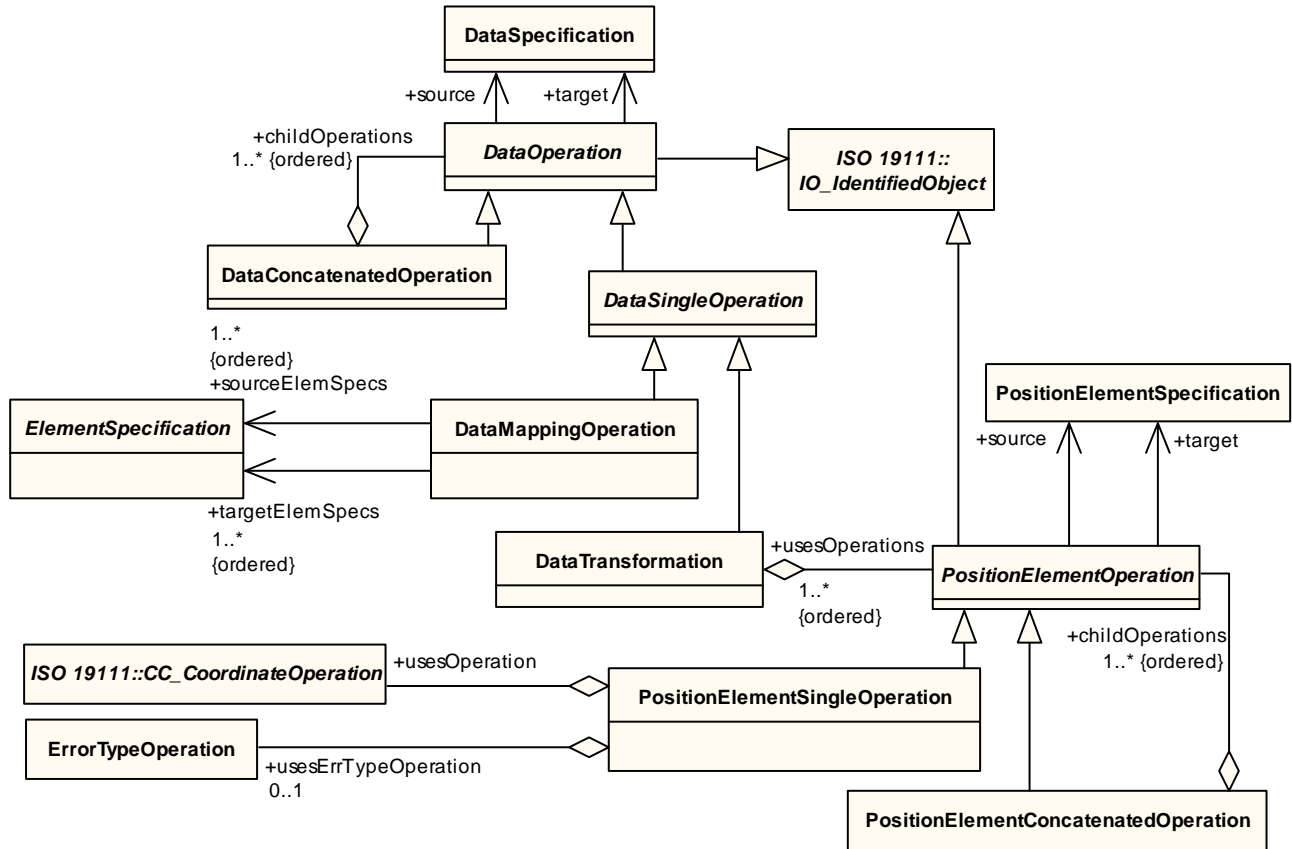
Figure 7.14 - RoLo Data Operation
