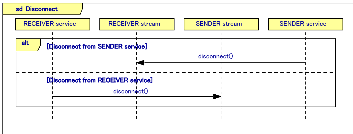
Figure 7.26 - Sequence Diagram of Disconnecting Connection
