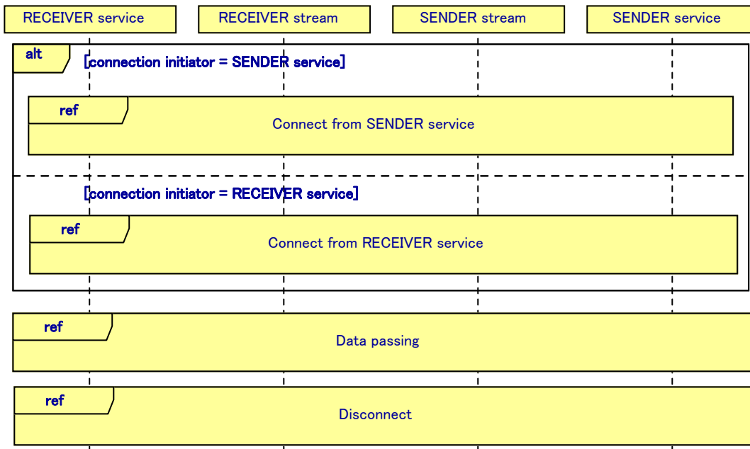
Figure 7.22 - Sequence diagram of typical RoLo service usage
