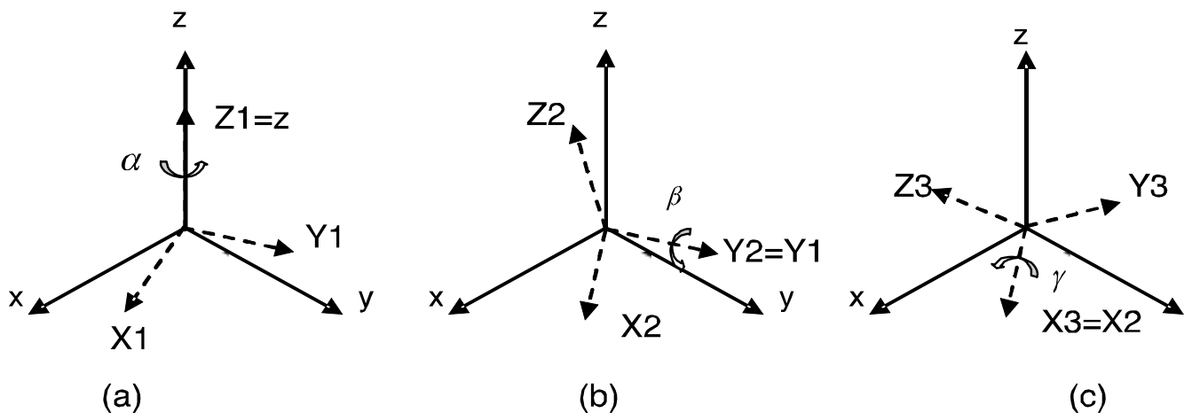
Figure 7.4 - Three sequential rotations for the PT_Euler_zY1X2 pose representation
