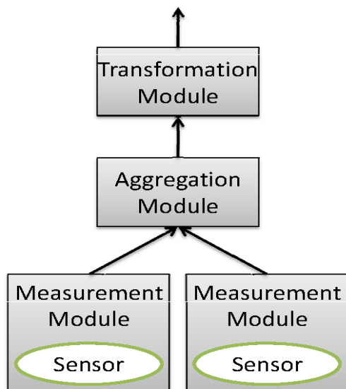
Figure 7.19 - Example of a cascading module connection
