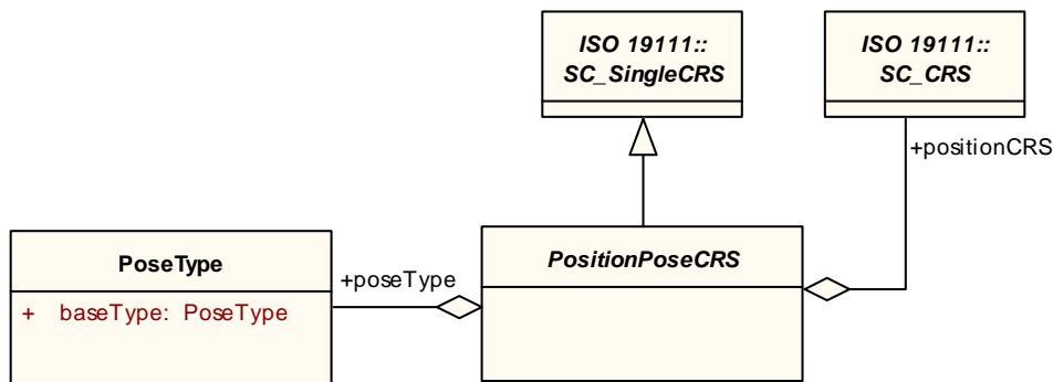
Figure 7.1 - Pose information
