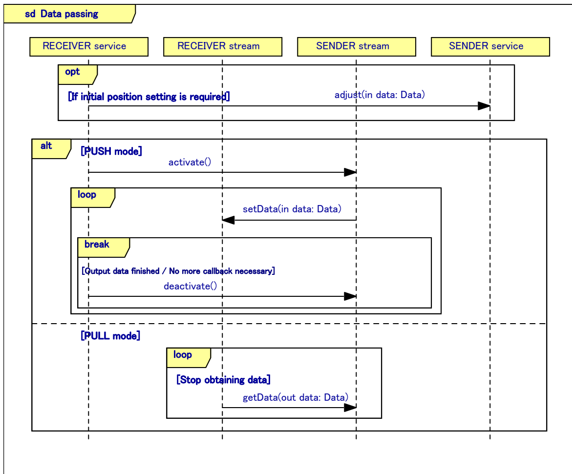
Figure 7.25 - Sequence Diagram of Data Passing
