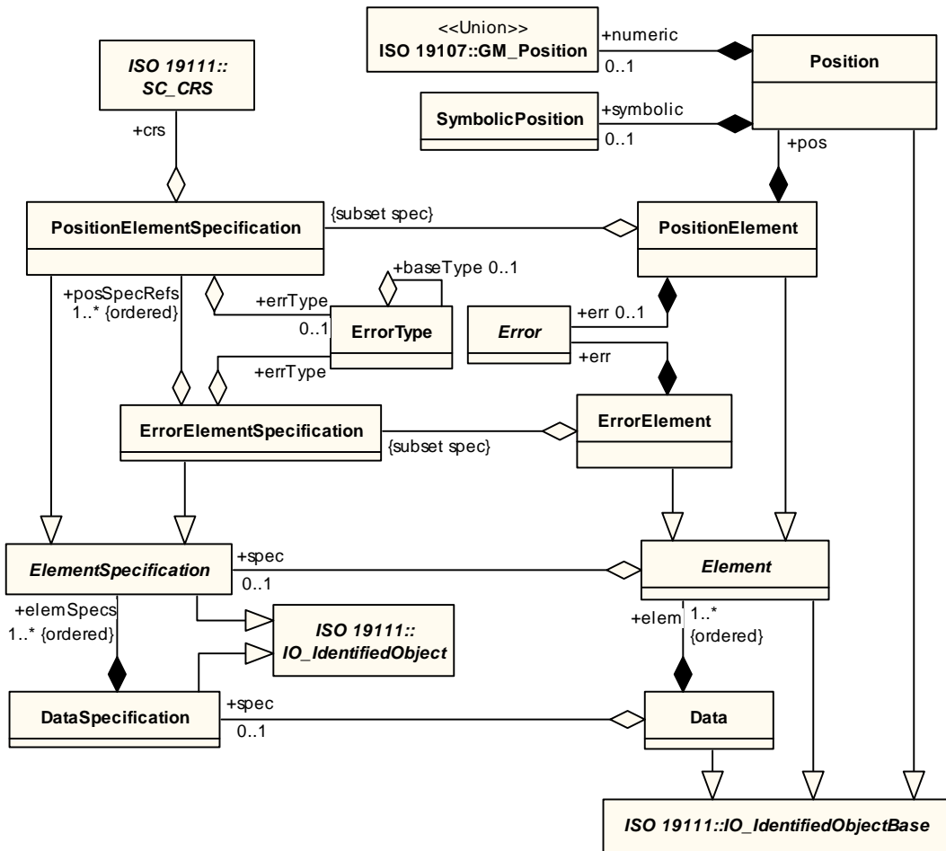
Figure 7.12 - RoLo Architecture
