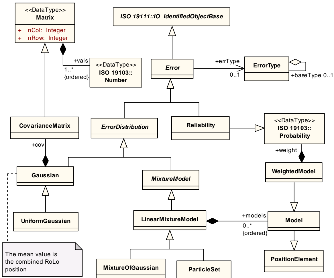
Figure 7.10 - RoLo Error
