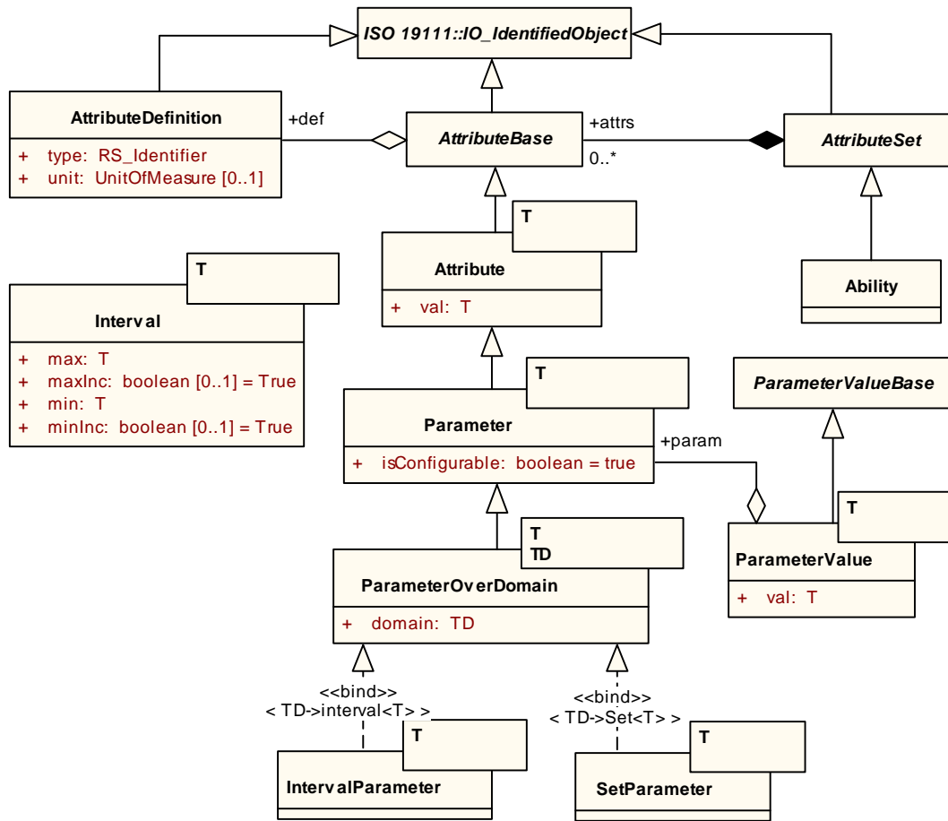
Figure 7.20 - RoLo Ability
