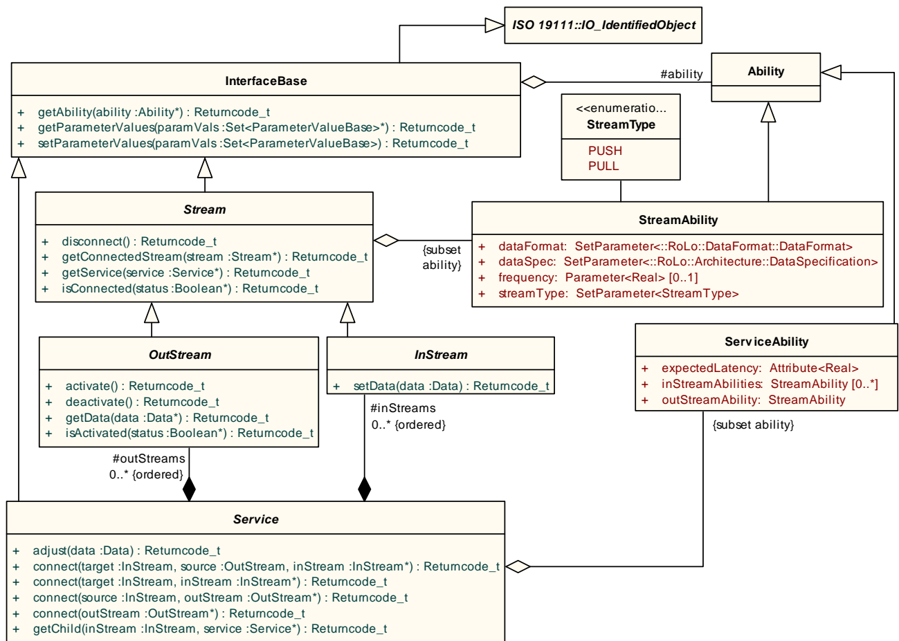
Figure 7.21 - RoLo Service
