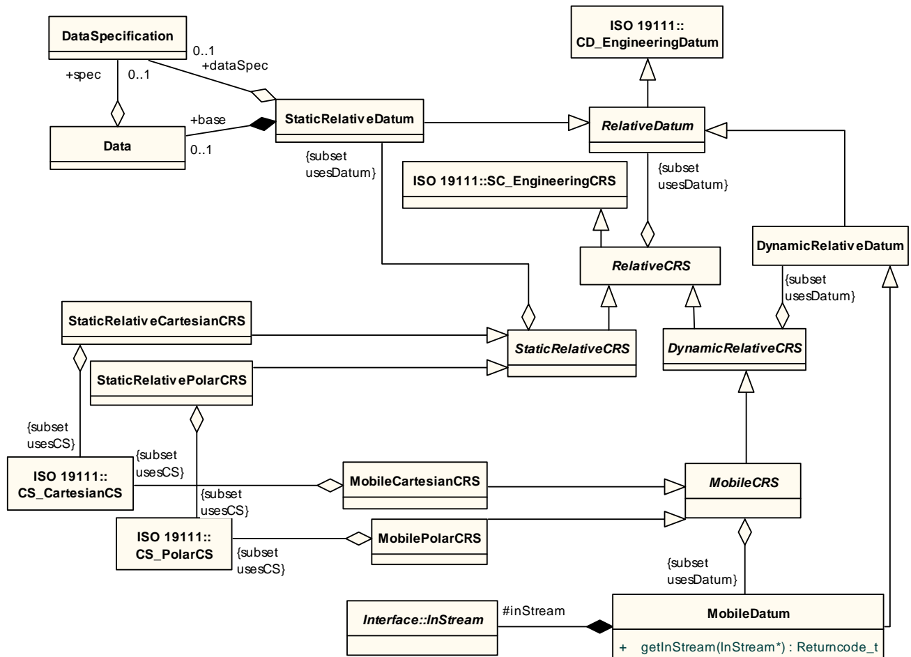
Figure 7.5 - Relative and Mobile coordinate reference system
