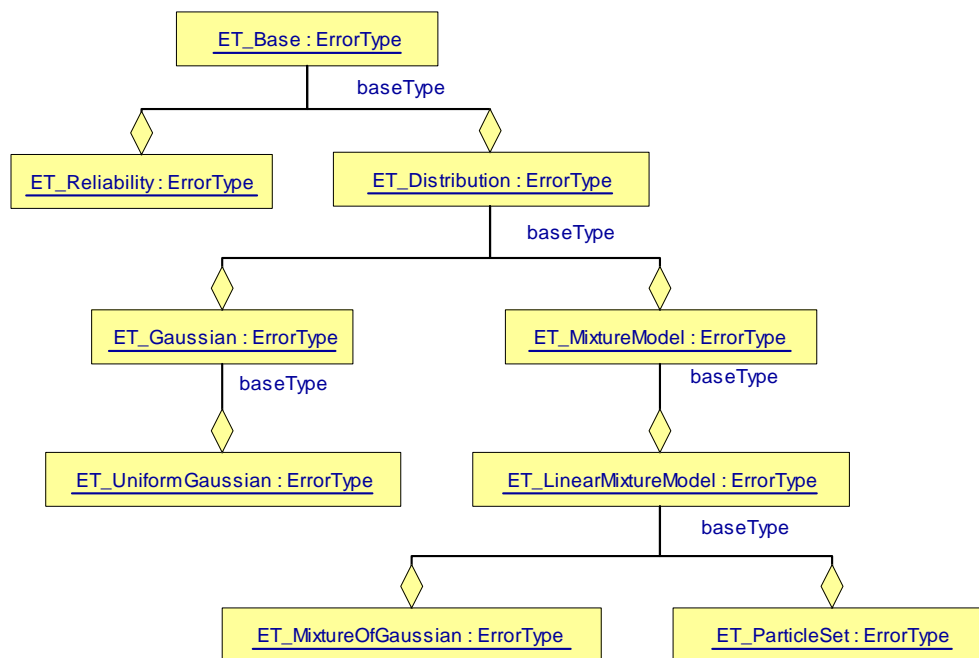
Figure 7.8 - Hierarchy of RoLo Error Types
