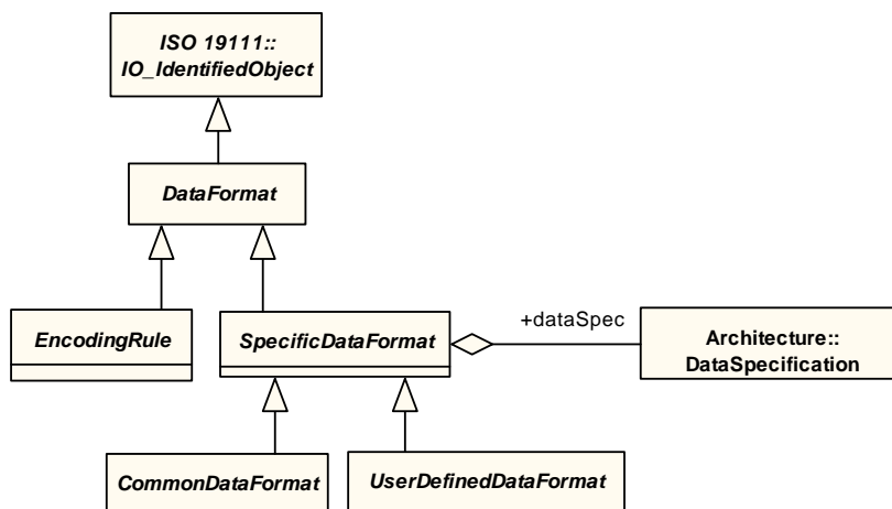
Figure 7.15 - RoLo Data Format
