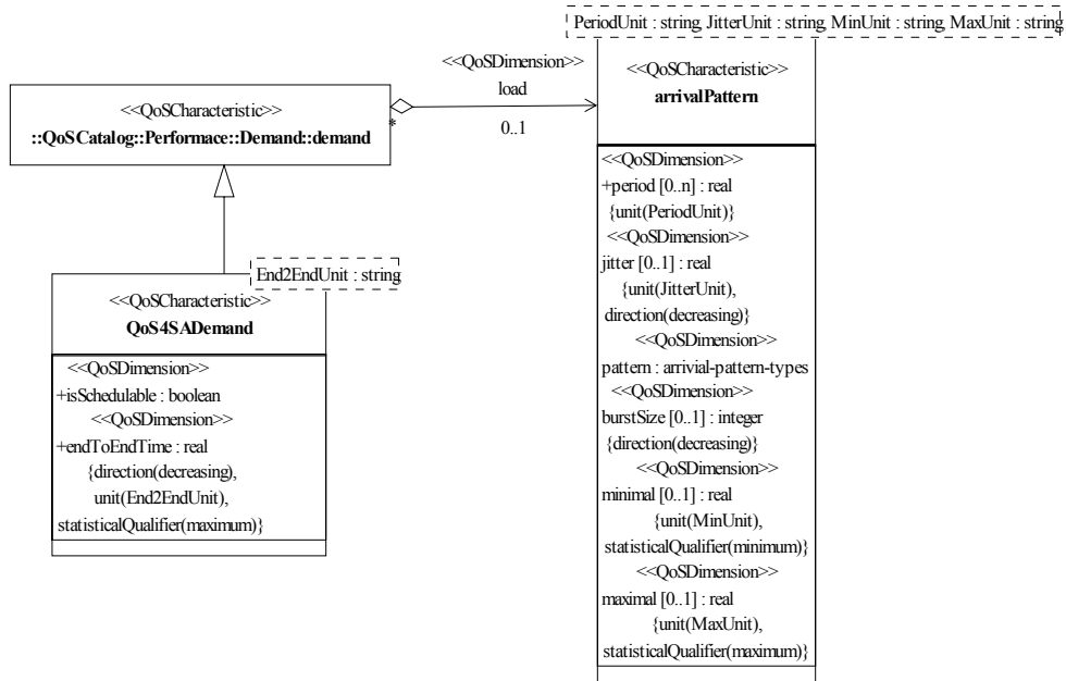
Figure B-1 Demand Characteristic for Scheduling Analysis
