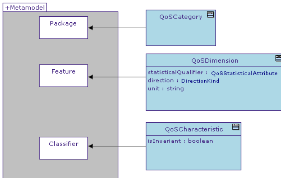
Figure 9-2 QoS Characteristics stereotypes
