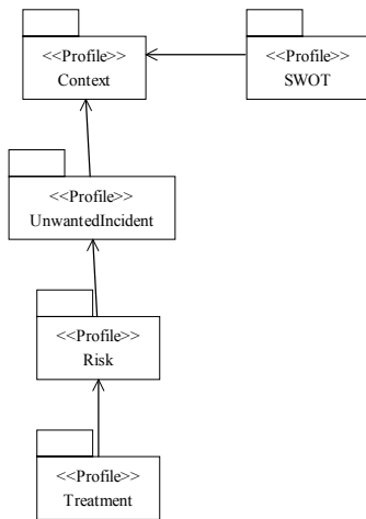
Figure 11-7 Subprofiles in the Risk Assessment profile
