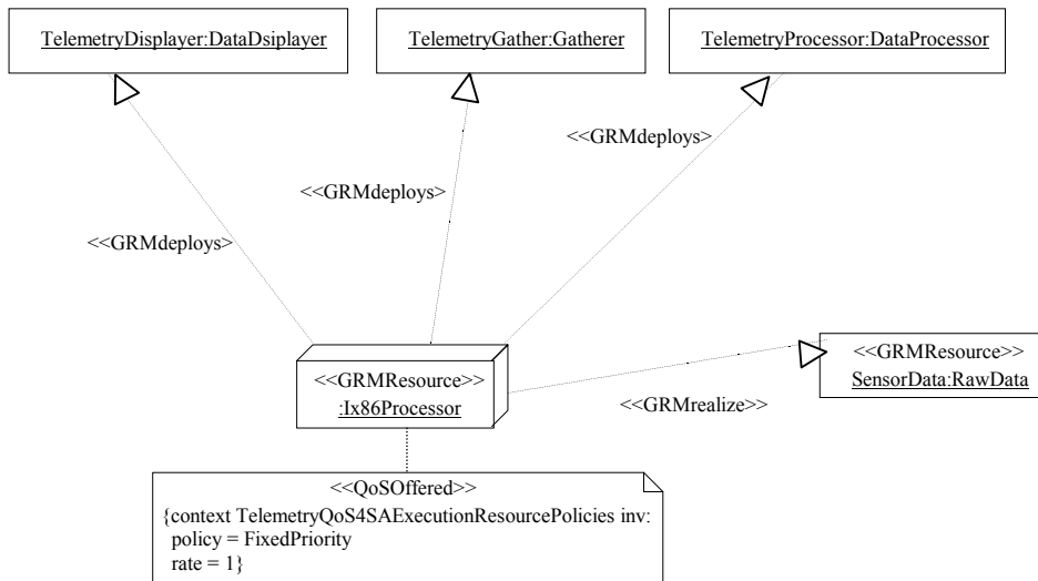
Figure B-8 Execution Engine Policies
