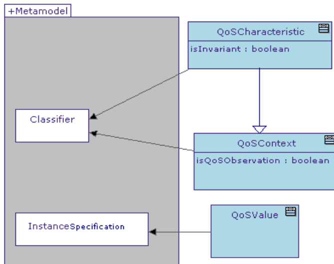
Figure 9-3 QoS Values stereotypes
