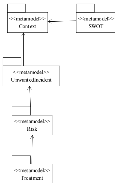
Figure 11-1 Submodels in the Risk Assessment Metamodel
