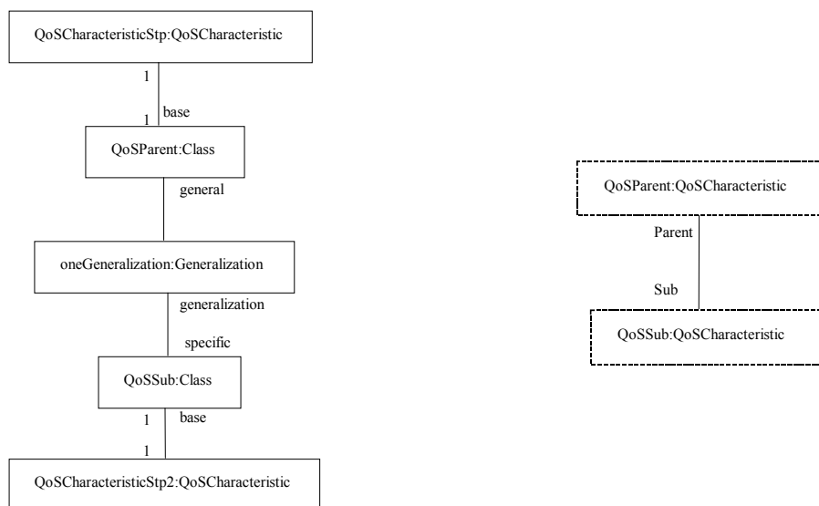
Figure 9-5 (a) QoS Paren-Sub in UML 2.0 (b) QoS Parent-Sub in QoS metamodel
