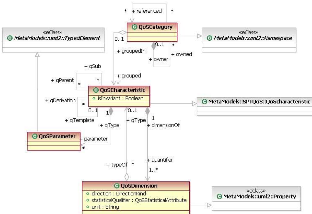
Figure 8-2 QoSCharacteristic Diagram
