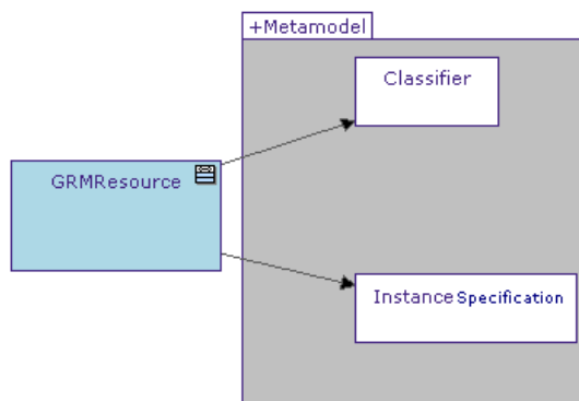
Figure 9-14 Resource Stereotype
