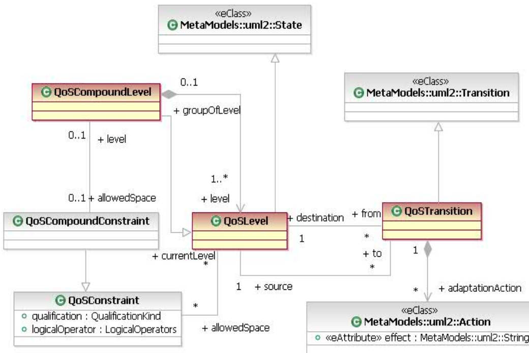
Figure 8-6 QoSLevel Diagram
