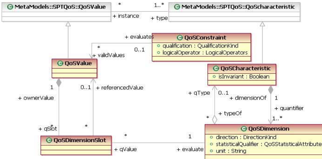
Figure 8-3 QoSValues Diagram
