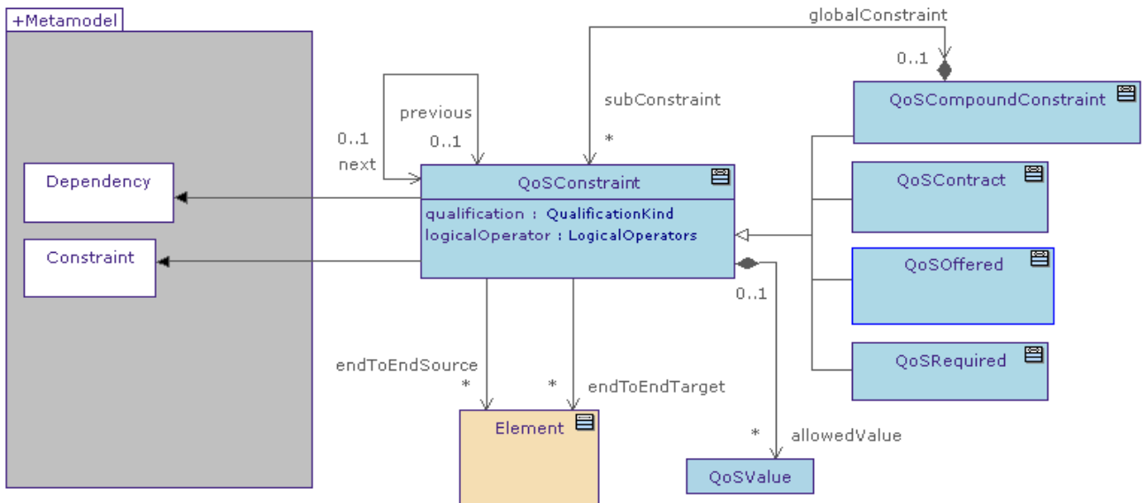
Figure 9-10 QoS Constraints Stereotypes
