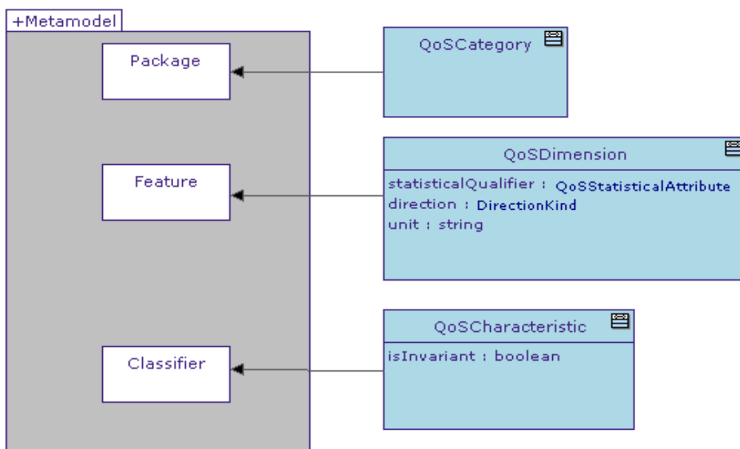
Figure 9-2 QoS Characteristics stereotypes
