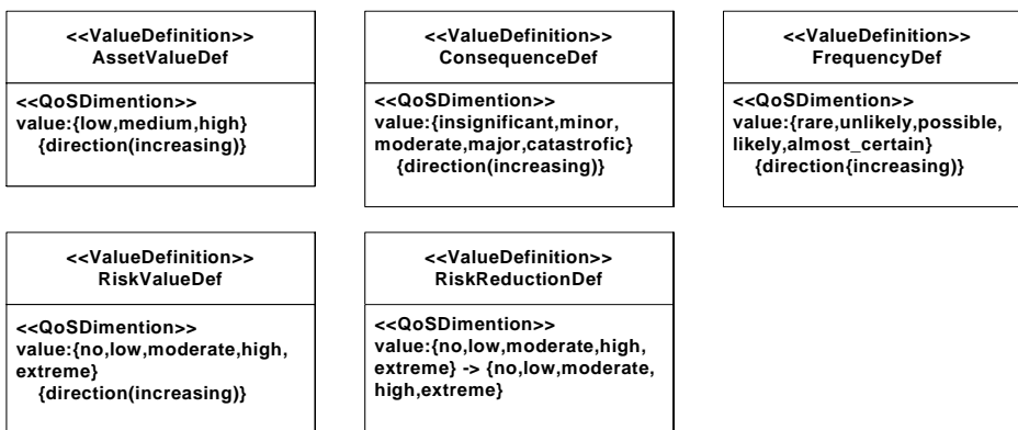
Figure 11-13 Value definitions
