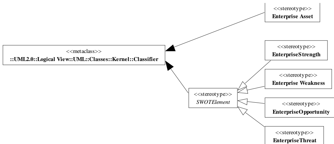
Figure 11-9 SWOT subprofile
