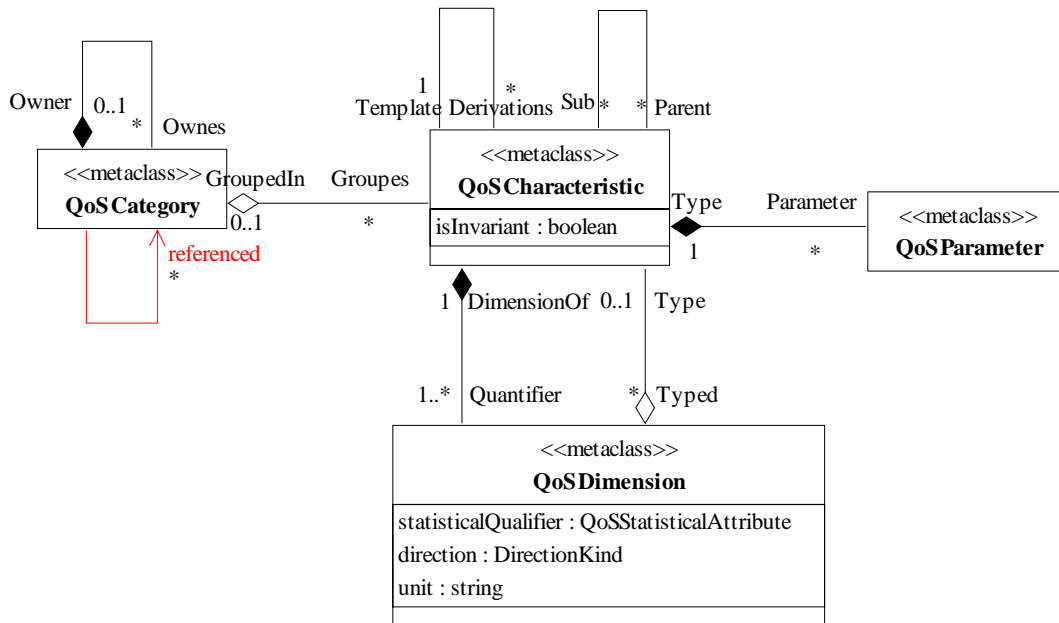
Figure 8-2 QoSCharacteristic Diagram
