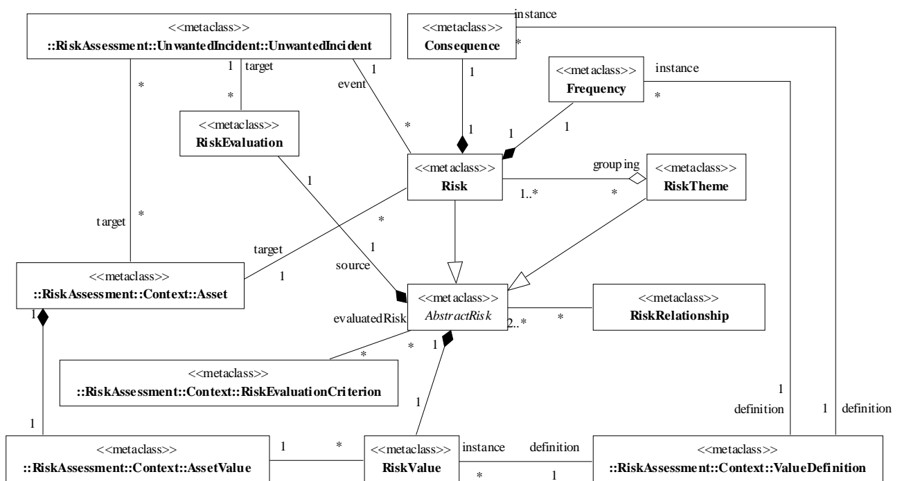
Figure 11-5 Risk submodel
