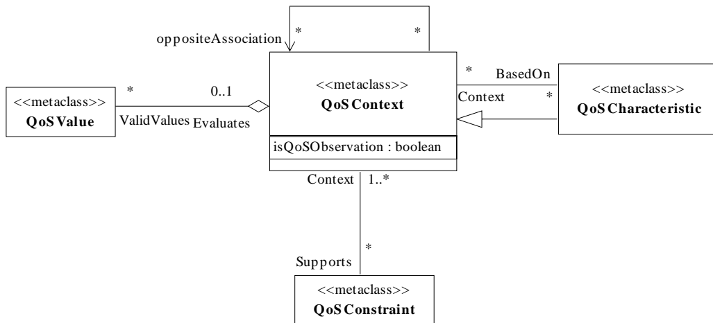
Figure 8-4 QoSContext Diagram
