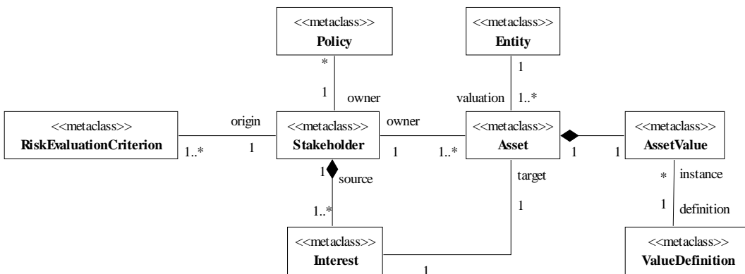
Figure 11-2 Context submodel
