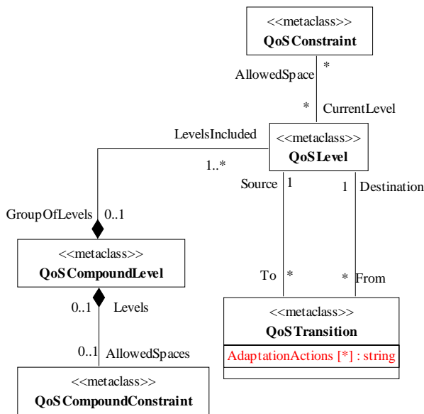
Figure 8-6 QoSLevel Diagram
