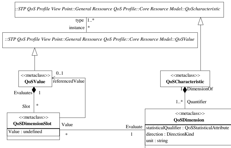
Figure 8-3 QoSValues Diagram
