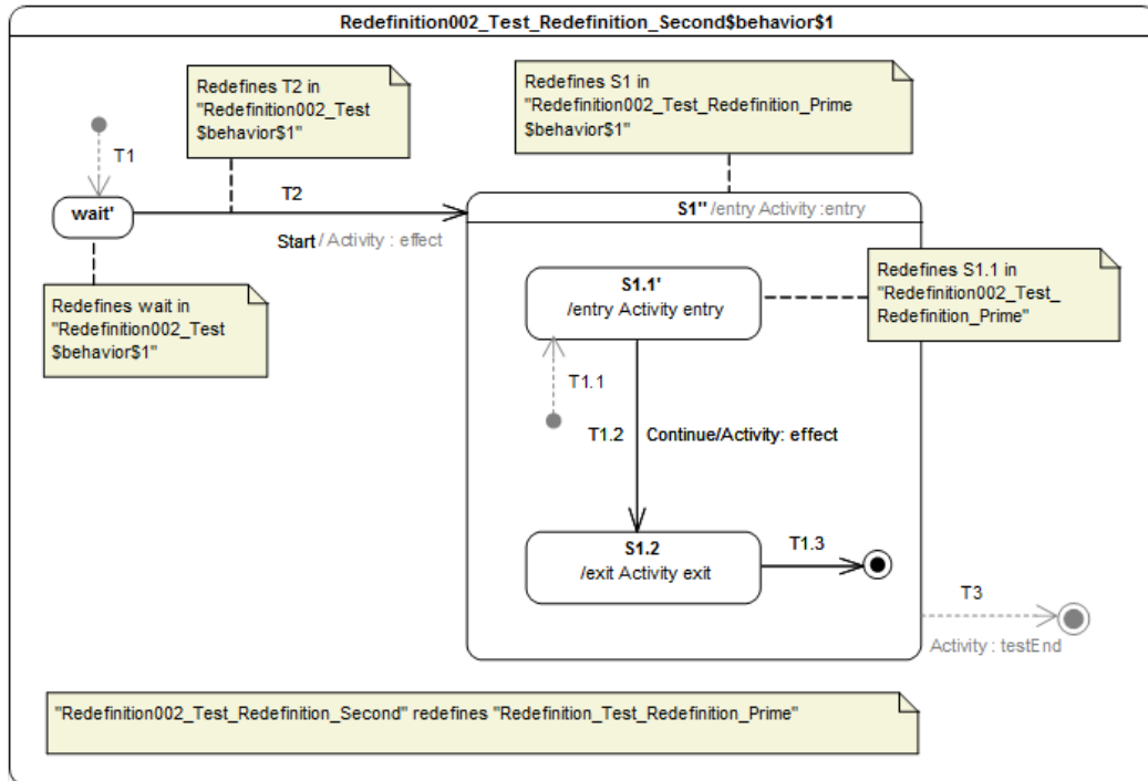
Figure 9.106 - Redefinition 002 Test Classifier Behavior – Runtime State Machine
