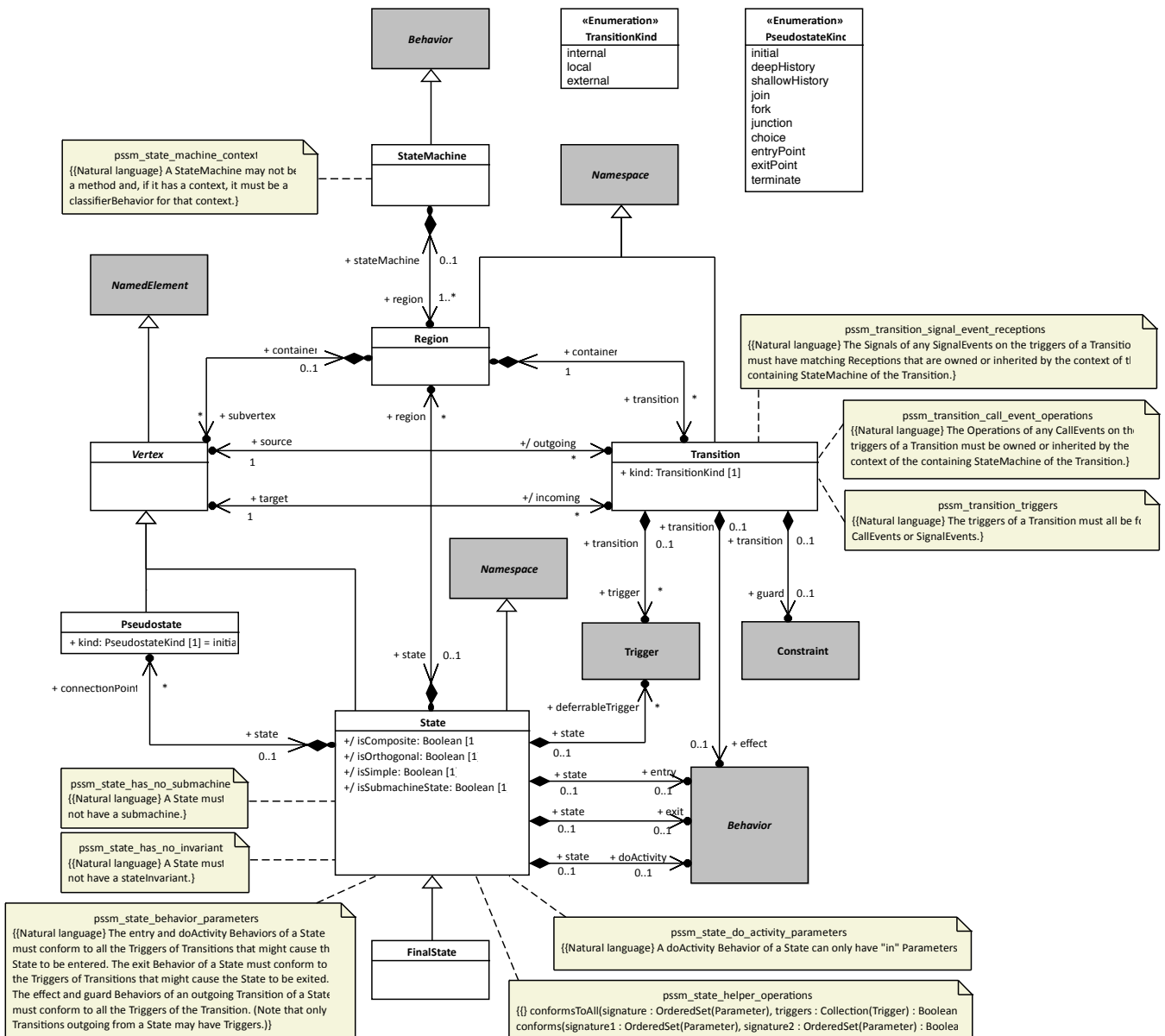
Figure 7.6 - Behavior StateMachines
