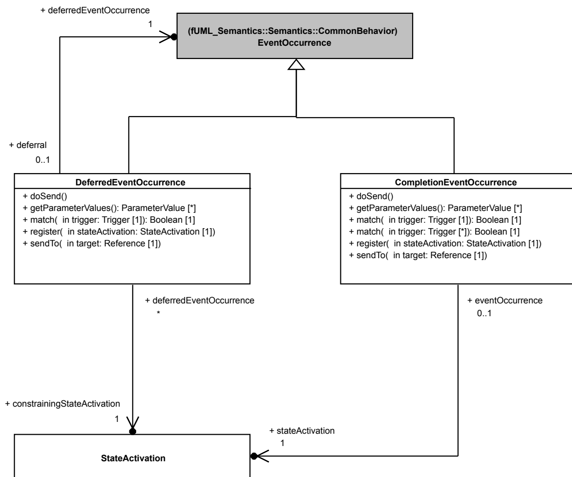
Figure 8.15 – Event Occurrences
