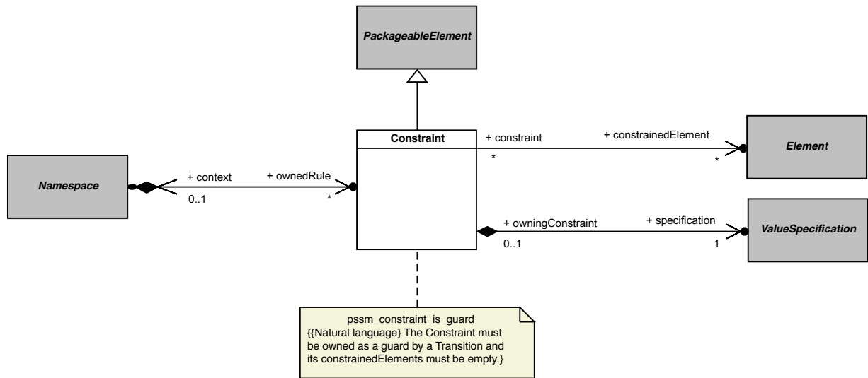
Figure 7.3 - Constraints
