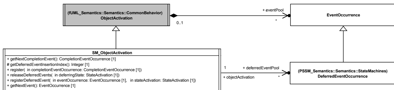
Figure 8.4 - CommonBehavior Extension
