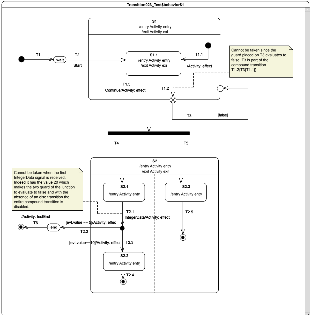
Figure 9.25: Transition 023 Test Classifier Behavior
