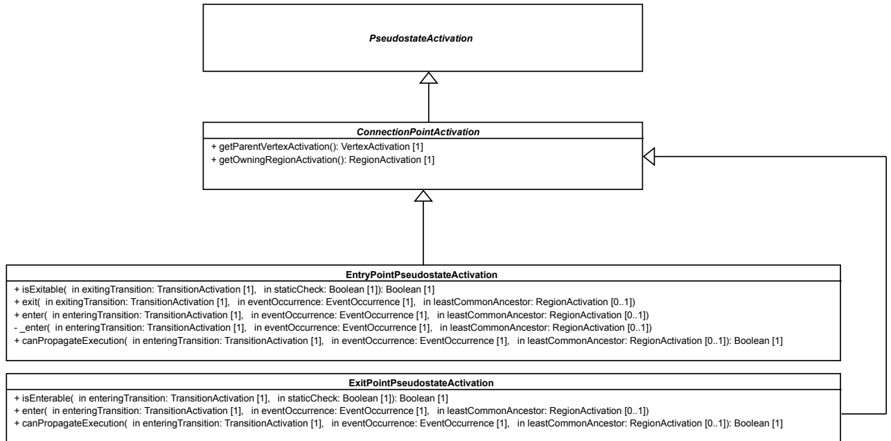
Figure 8.11 - EntryPointActivation and ExitPointActivation
