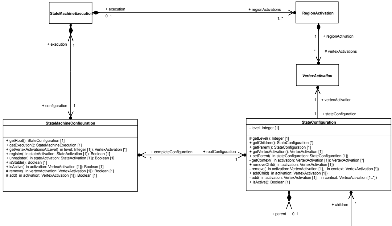
Figure 8.7 - StateMachineConfiguration
