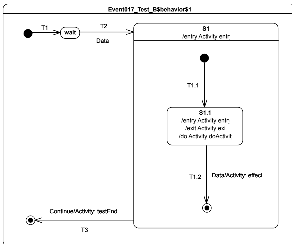
Figure 9.35 - Event 017 - B Test Classifier Behavior
