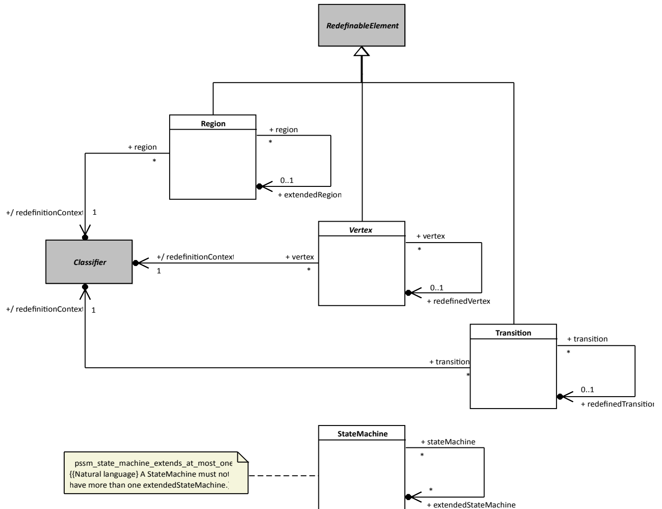
Figure 7.7 - StateMachine Redefinition
