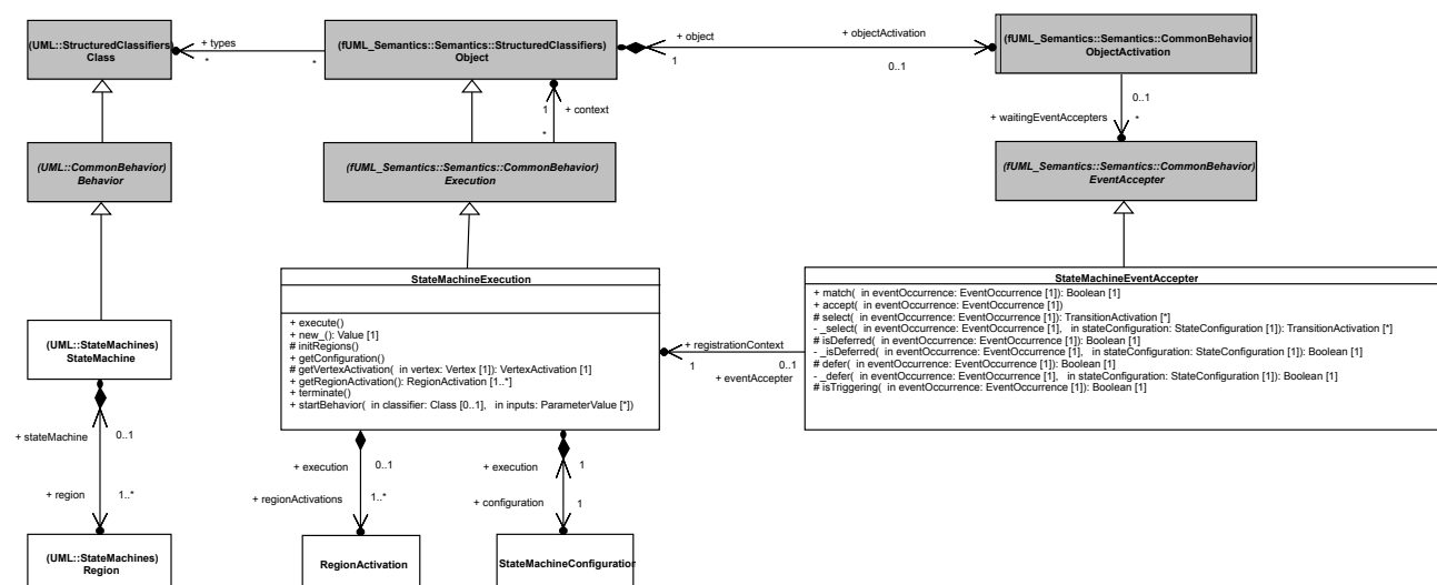
Figure 8.5 - StateMachineExecution
