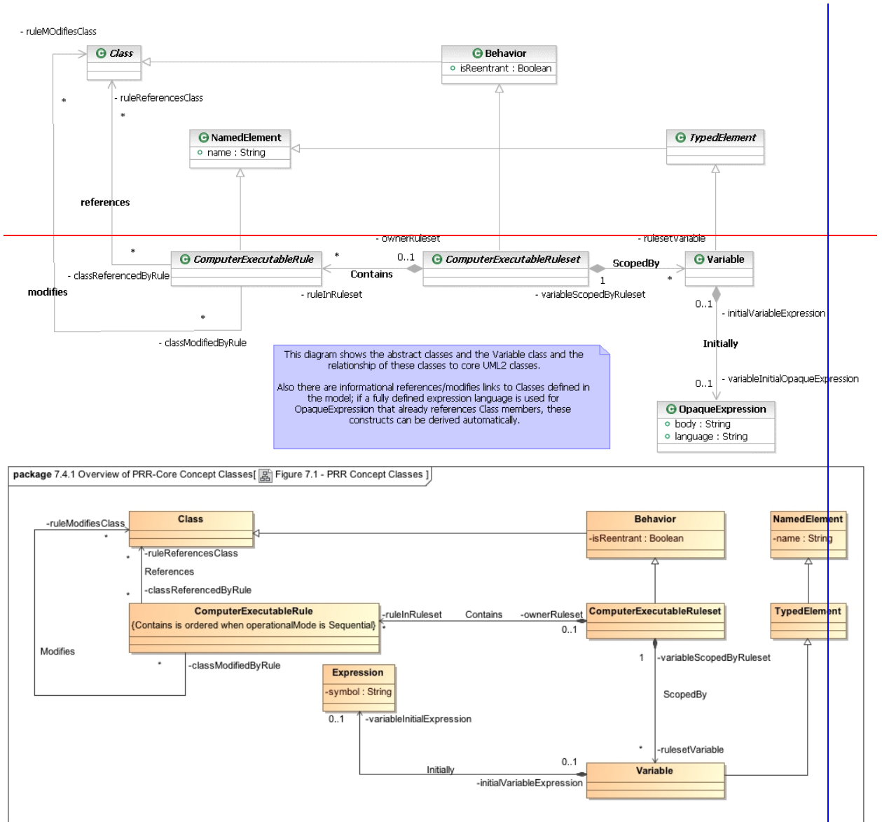
Figure 1: PRR Concept Classes
