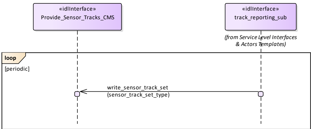
Figure 7.171 Basic Flow - Sensor Track Reporting (Individual) (Interaction diagram)
