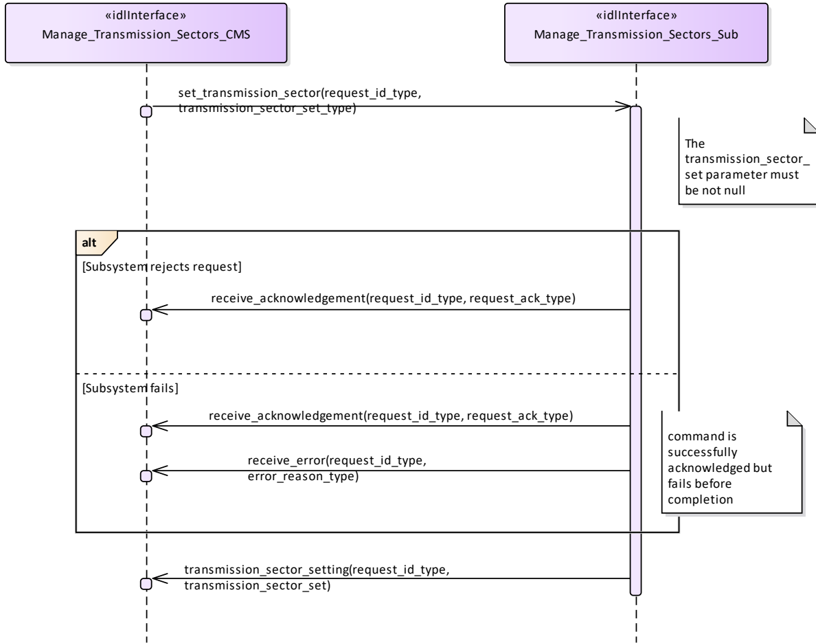
Figure 7.153 Alternative Flow - Manage Transmission Sectors - Enable/Disable - loss of mastership (Interaction diagram)
