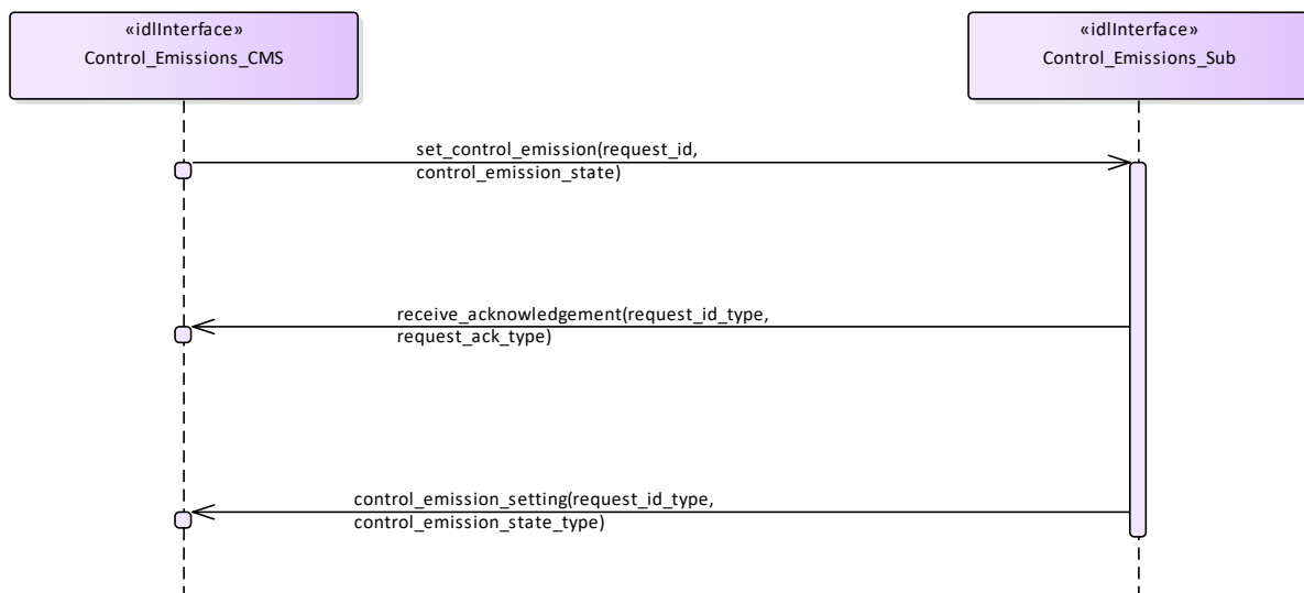
Figure 7.154 Basic Flow - Control Emissions - On/Off (Interaction diagram)
