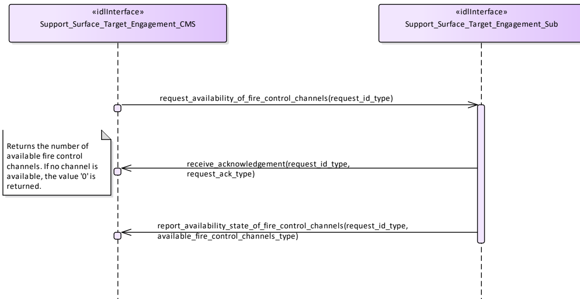
Figure 7.186 Support surface target engagement - Check availability (Interaction diagram)
