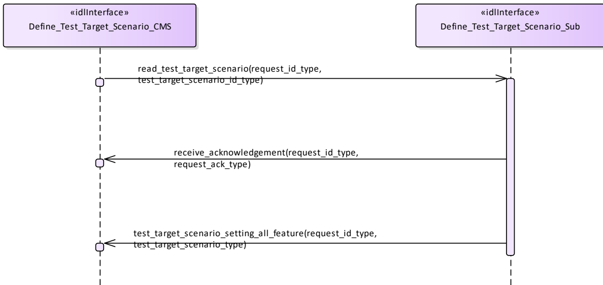
Figure 7.158 Basic Flow - Inspect a Test Target Scenario (Interaction diagram)
