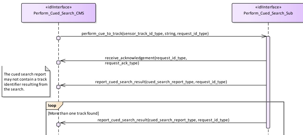
Figure 7.125 Alternative Flow - Sensor does not Perform Cued To Track (Interaction diagram)
