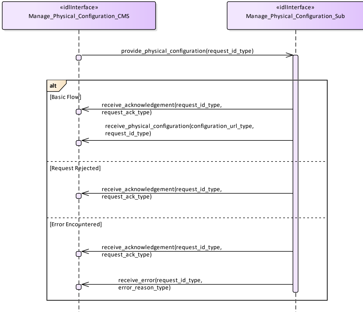
Figure 7.69 Manage Physical Configuration - Request (Interaction diagram)
