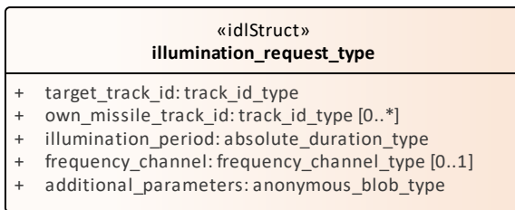
Figure 7.62 Illumination (Class diagram)
