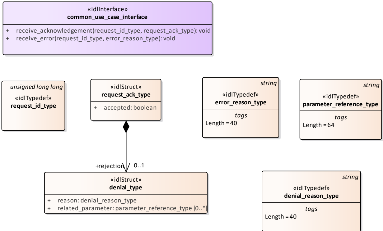
Figure 7.31 Domain Model (Class diagram)
