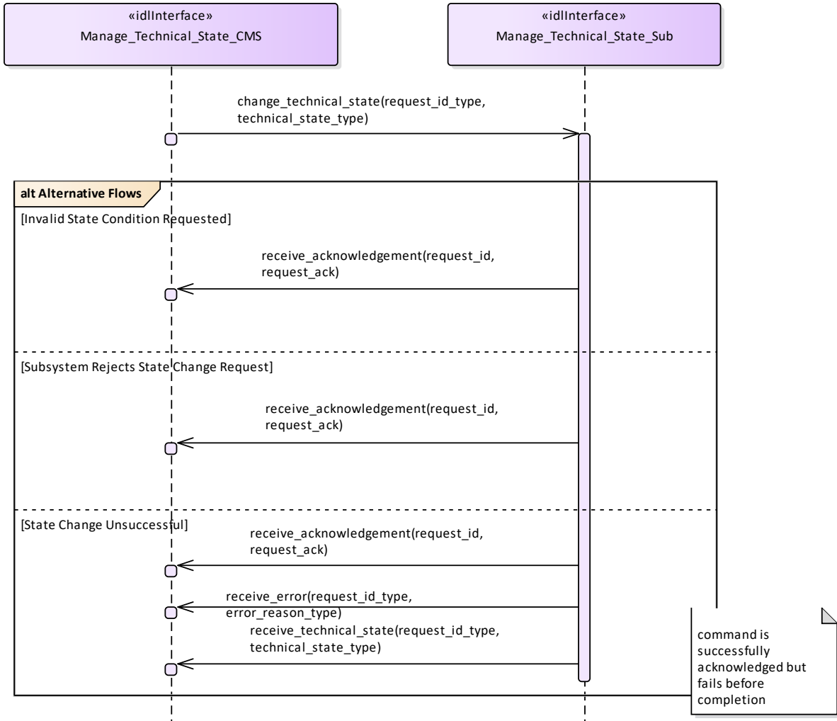
Figure 7.90 Alternative Flow - Manage Technical State - Change (Interaction diagram) Alternate flow depicting rejection and error cases for a CMS requesting the subsystem to change its Technical State.
