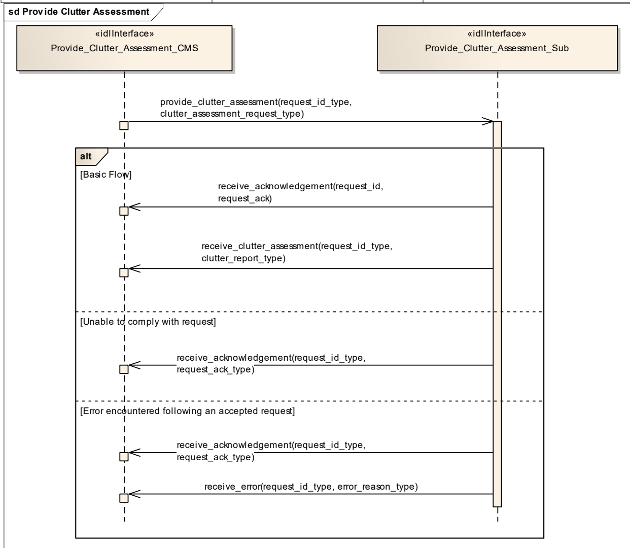
Figure 7.100 Provide Clutter Assessment (Sequence diagram)
