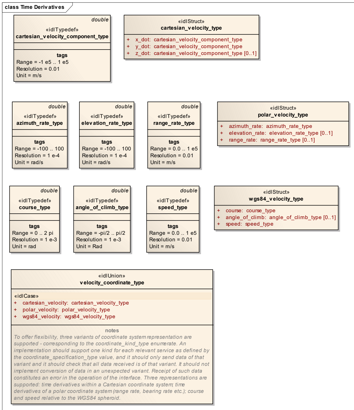
Figure 7.26 Time Derivatives (Logical diagram)
