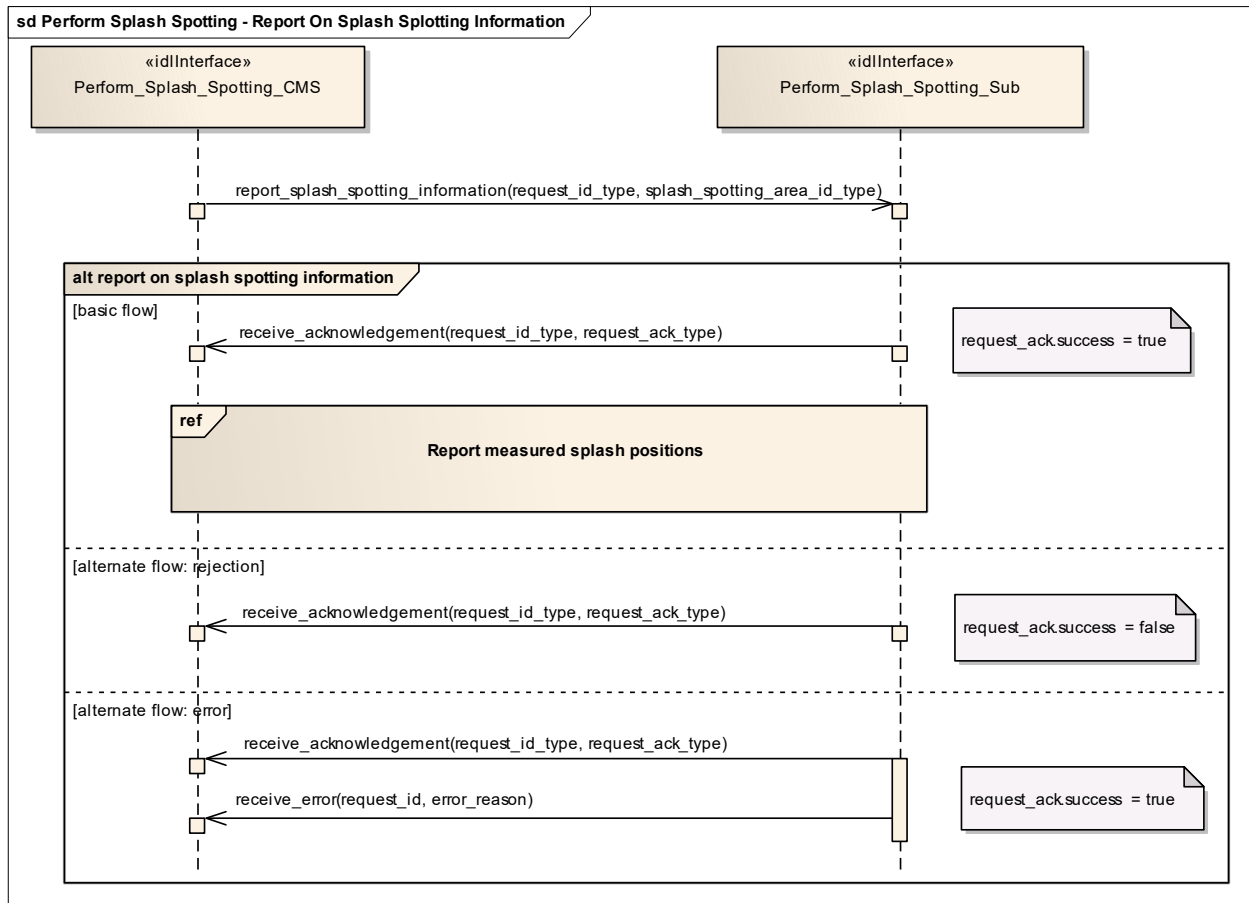
Figure 7.157 Perform Splash Spotting - Report On Splash Spotting Information (Sequence diagram)
