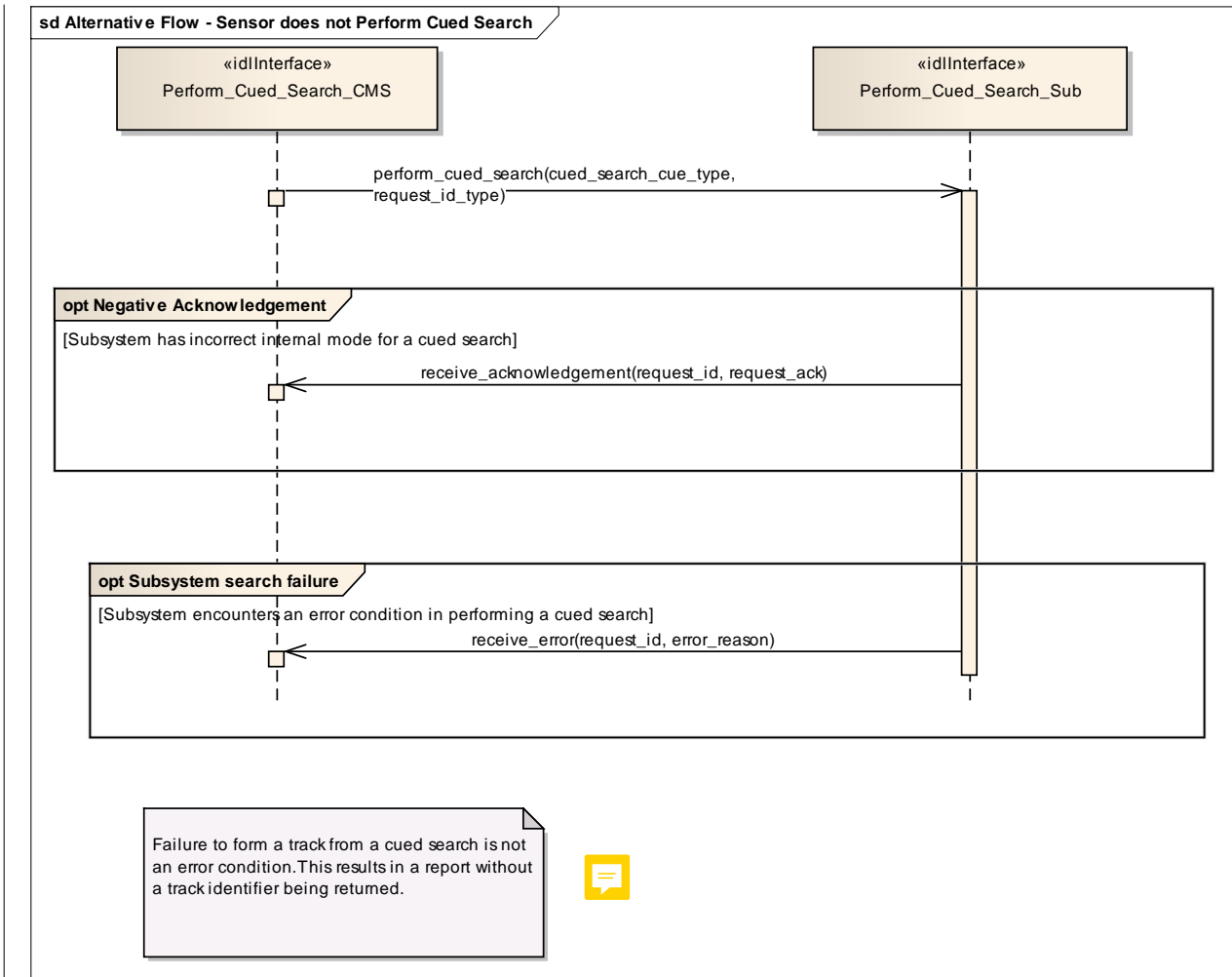
Figure 7.149 Alternative Flow - Sensor does not Perform Cued Search (Sequence diagram)
