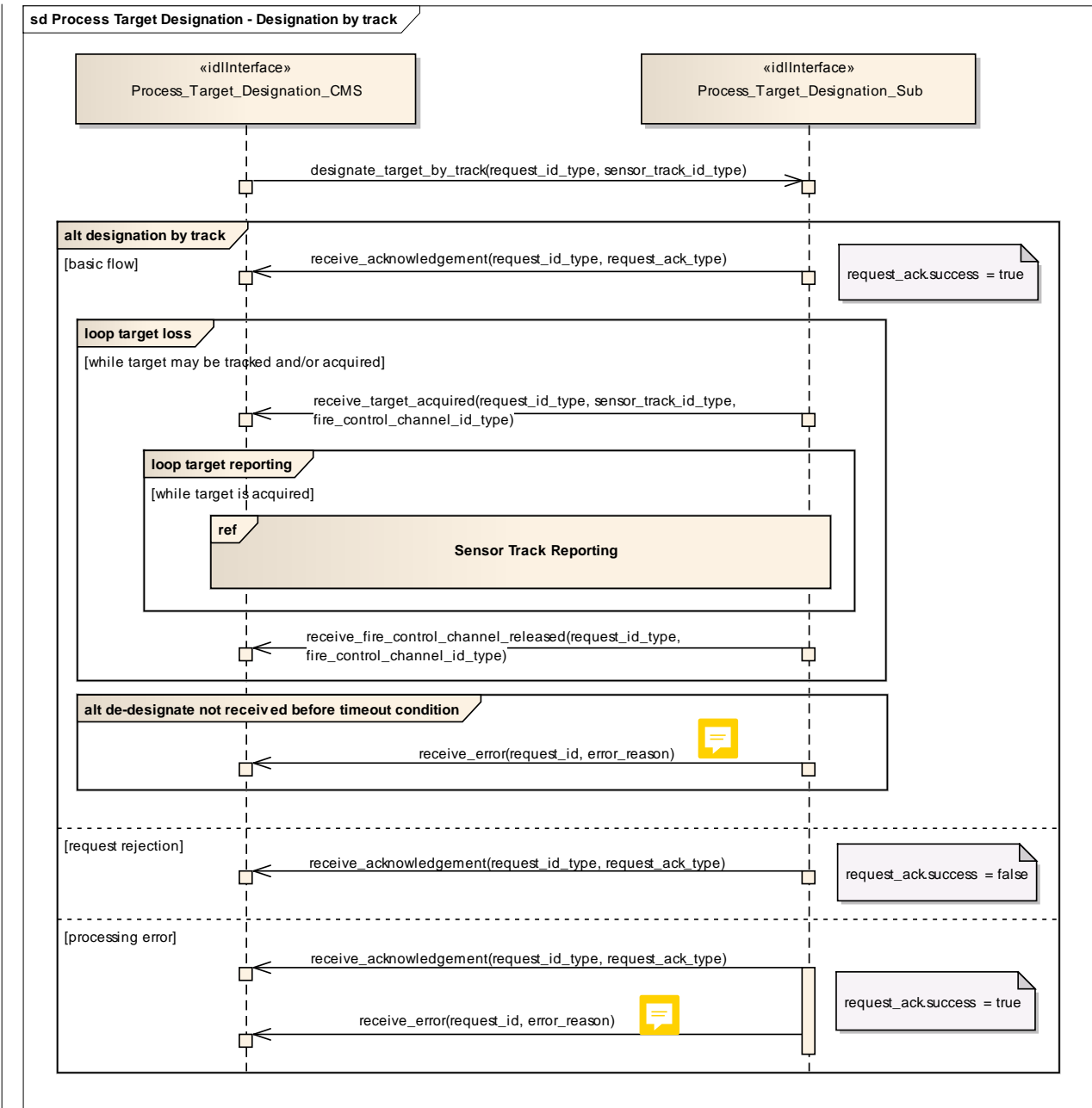
Figure 7.139 Process Target Designation - Designation by track (Sequence diagram)
