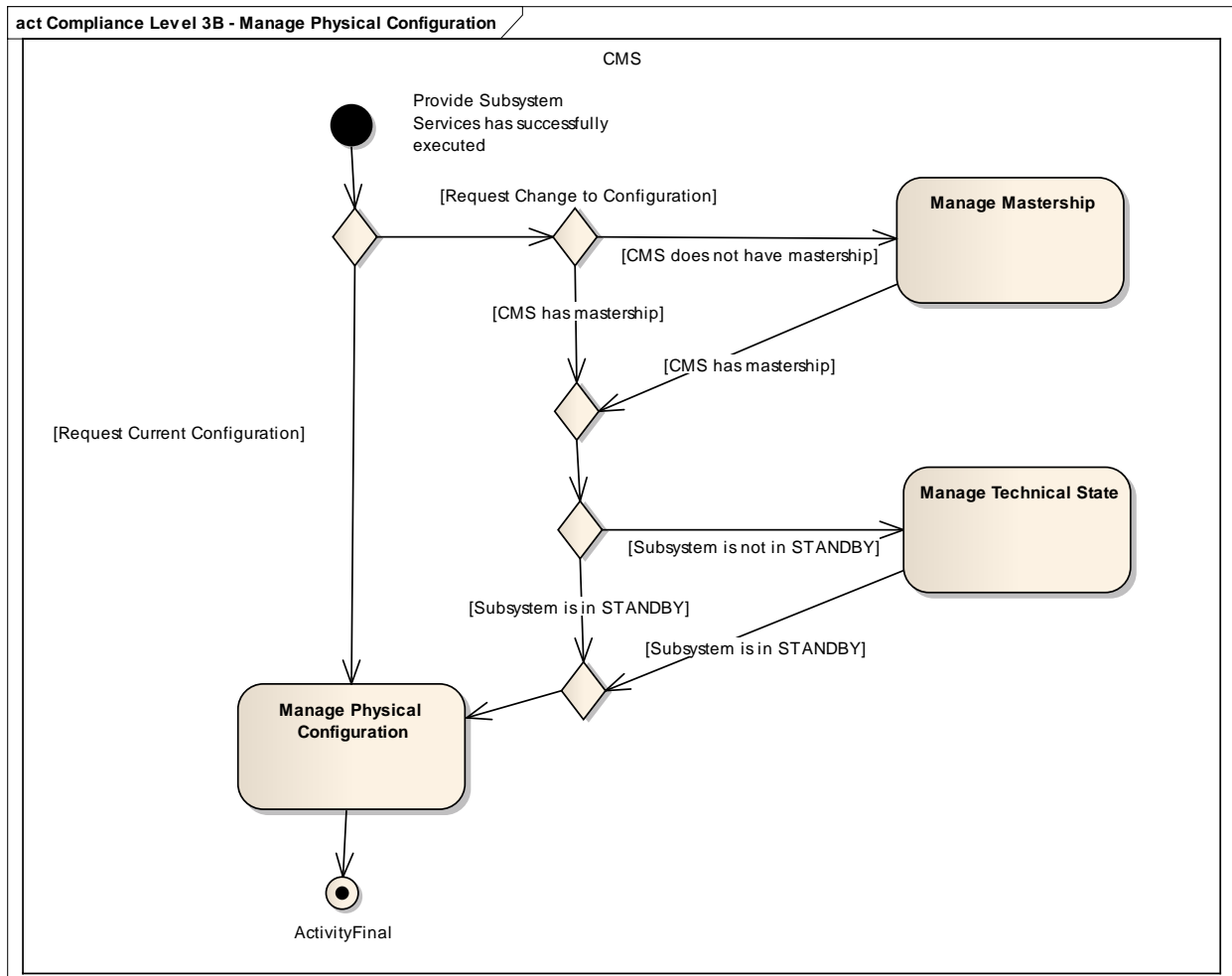
Figure 7.10 Compliance Level 3B - Manage Physical Configuration (Activity diagram) These interfaces support more detailed control of the subsystem configuration.
