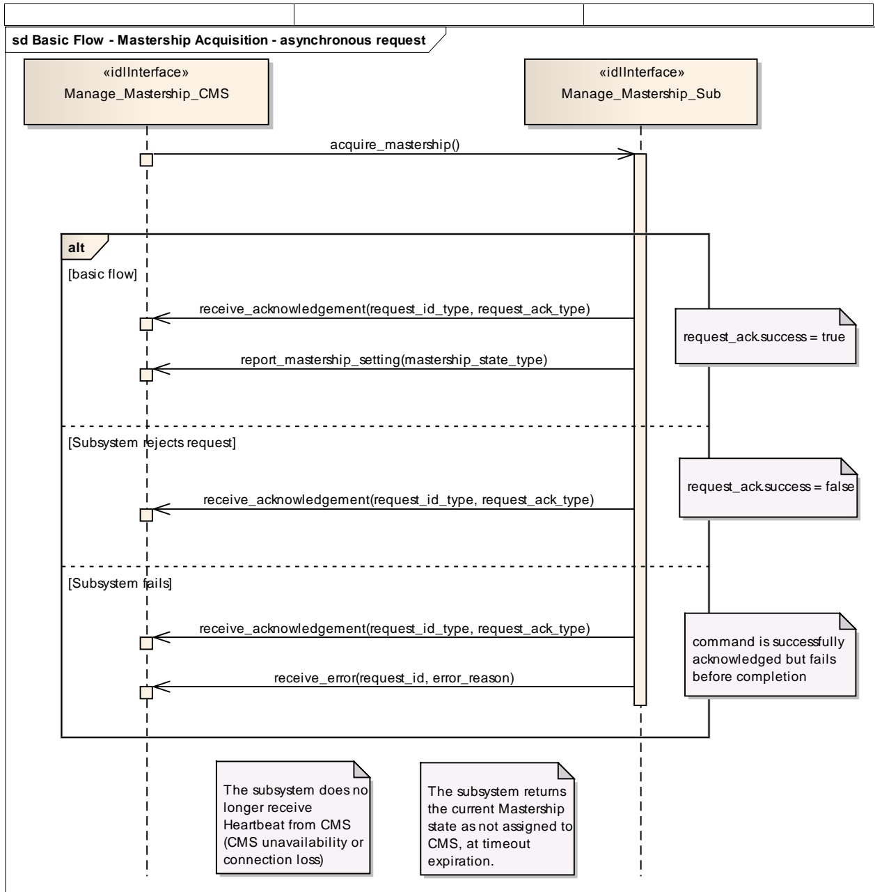
Figure 7.93 Basic Flow - Mastership Acquisition - asynchronous request (Sequence diagram)
