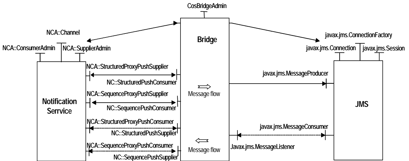
Figure 2-1 General Architecture of the Bridge
