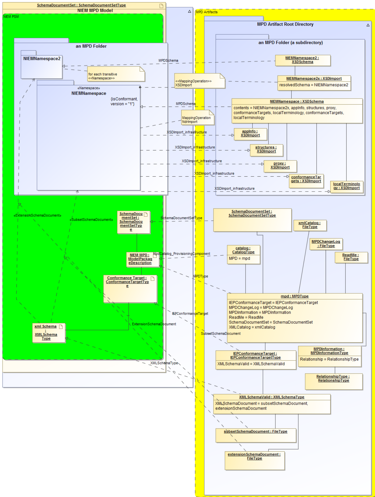
Figure 9-23 NIEM MPD Model to NIEM MPD Artifact Mapping Overview
