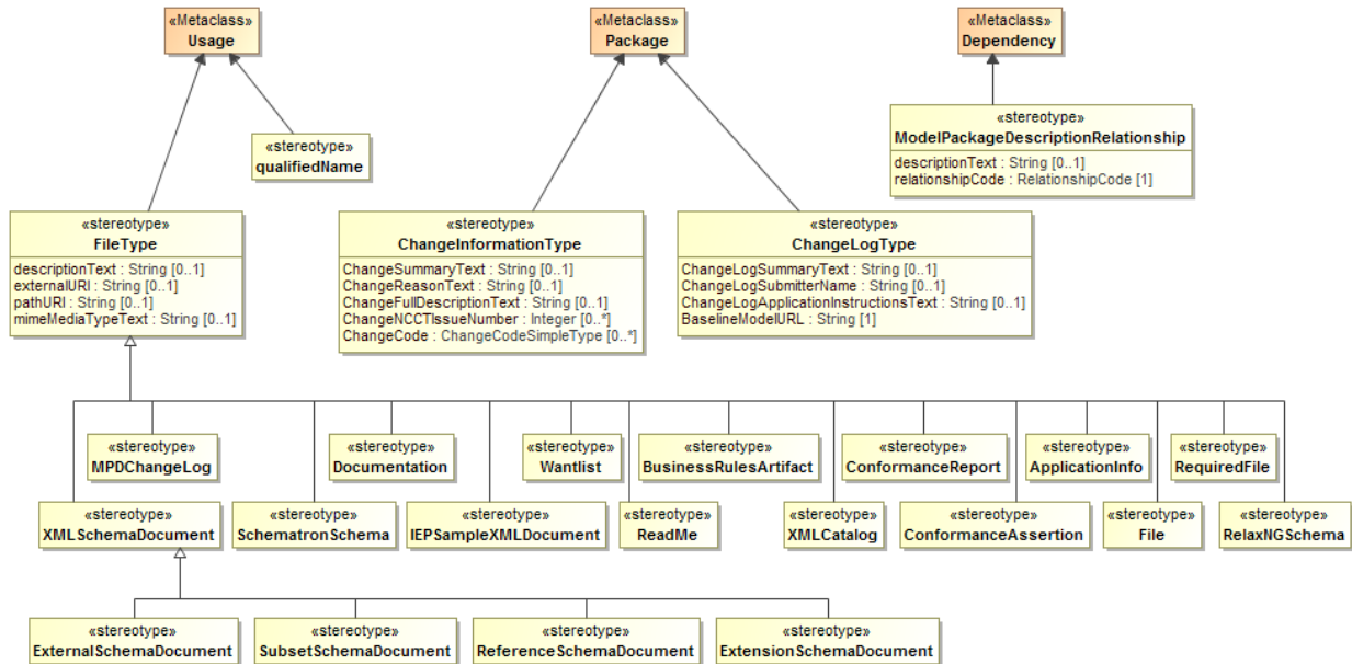
Figure 8-5 Model Package Description profile stereotypes
