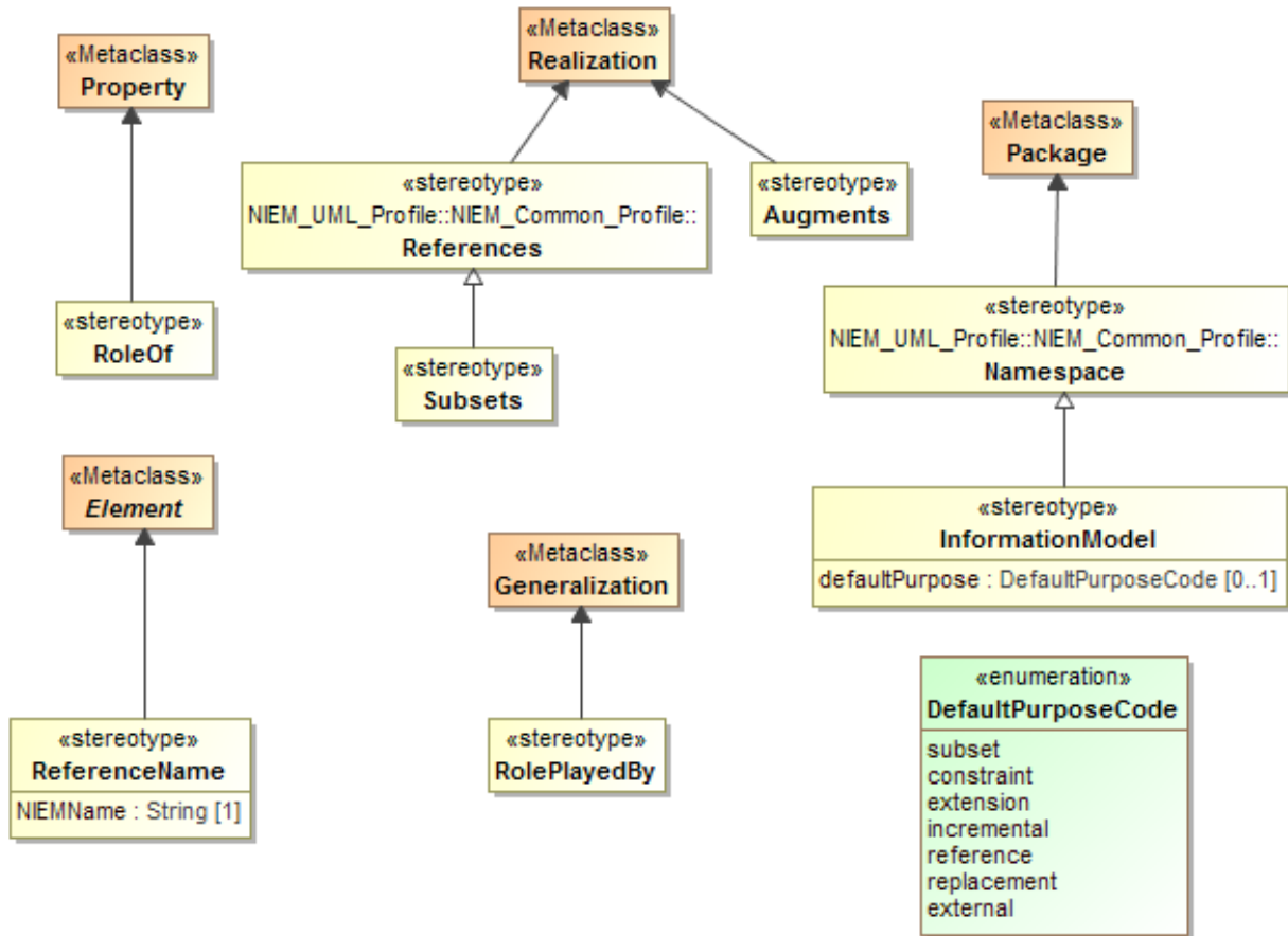
Figure 8-3 NIEM PIM Profile
