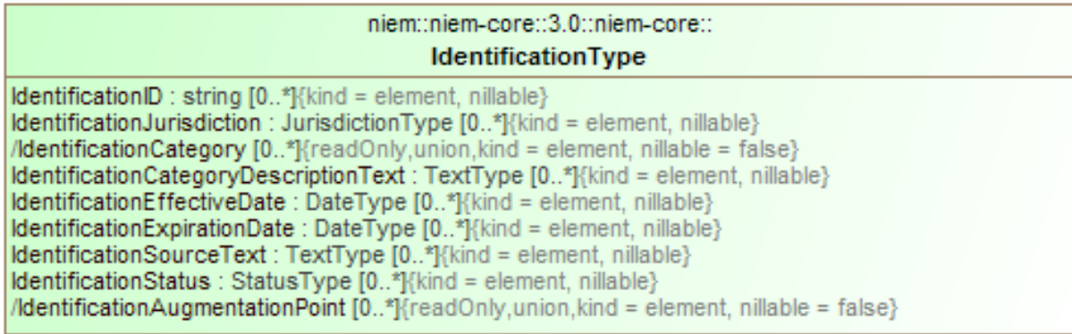
Figure 10-9 Identification Class Contents
