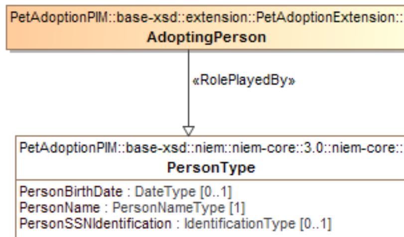
Figure 10-13 Role of Person
