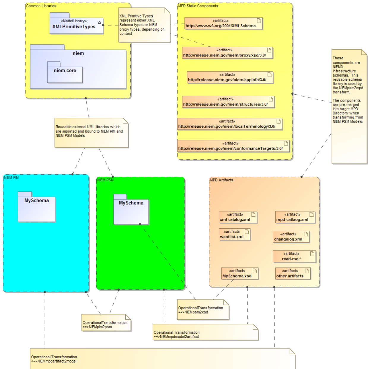
Figure 9-1 NIEM Provisioning Context
