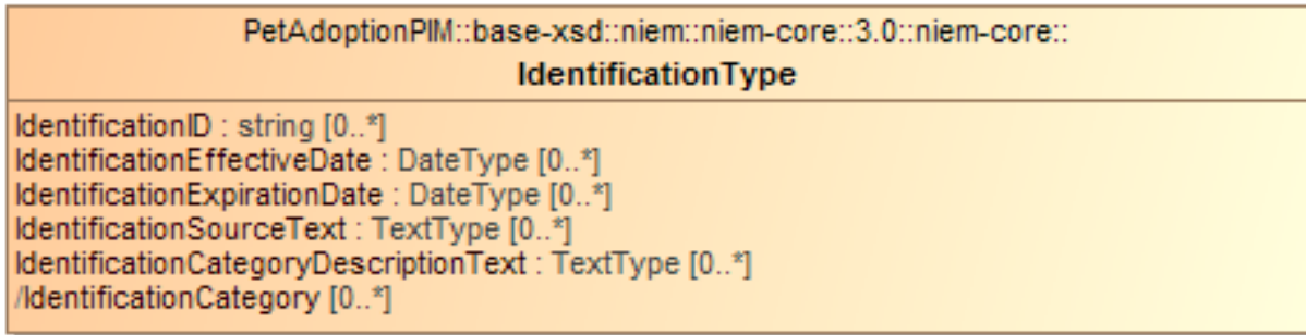
Figure 10-6 Properties Using Identification Class
