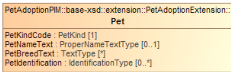
Figure 10-5 Properties of Pet
