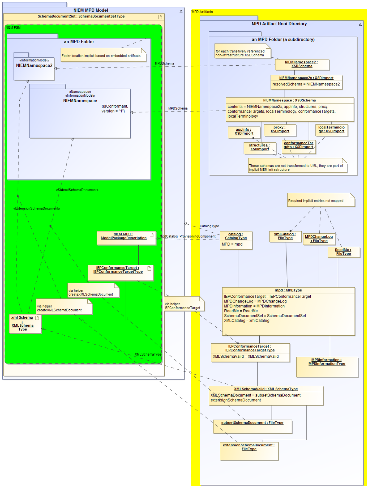
Figure 9-24 NIEM MPD Artifact to NIEM MPD Model - Overview
