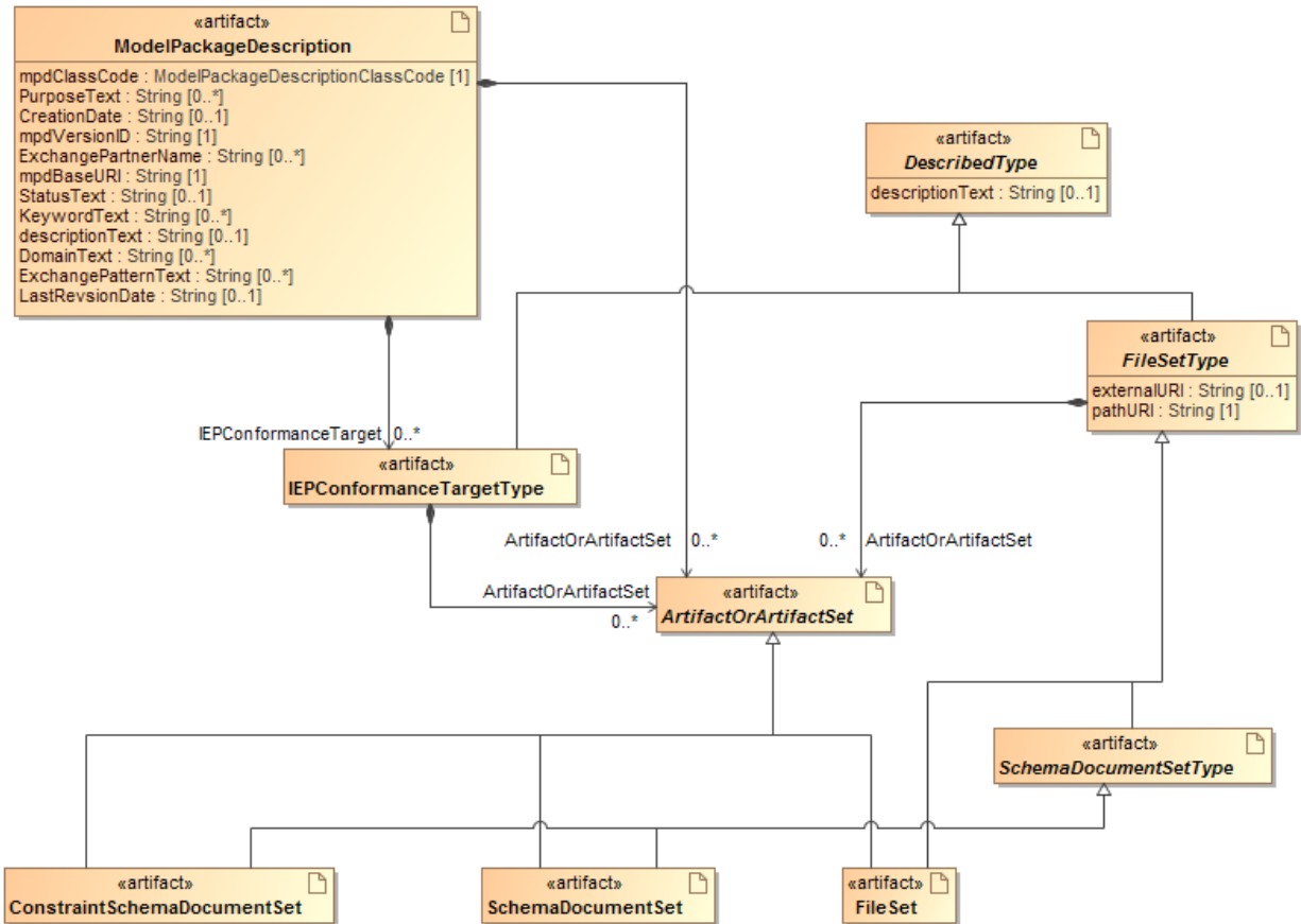
Figure 8-9 MPD Profile Artifacts for files and documents
