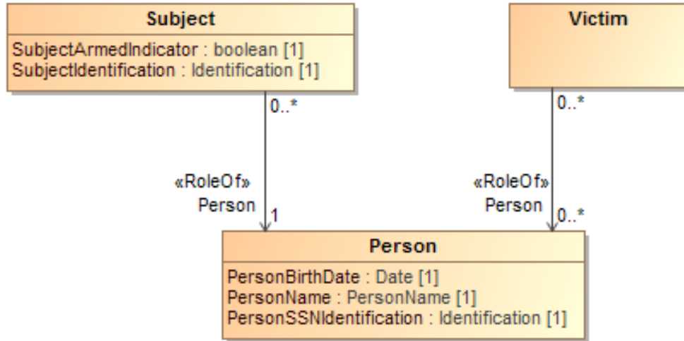
Figure 7-7 Representation of role types using role-of properties in a PIM
