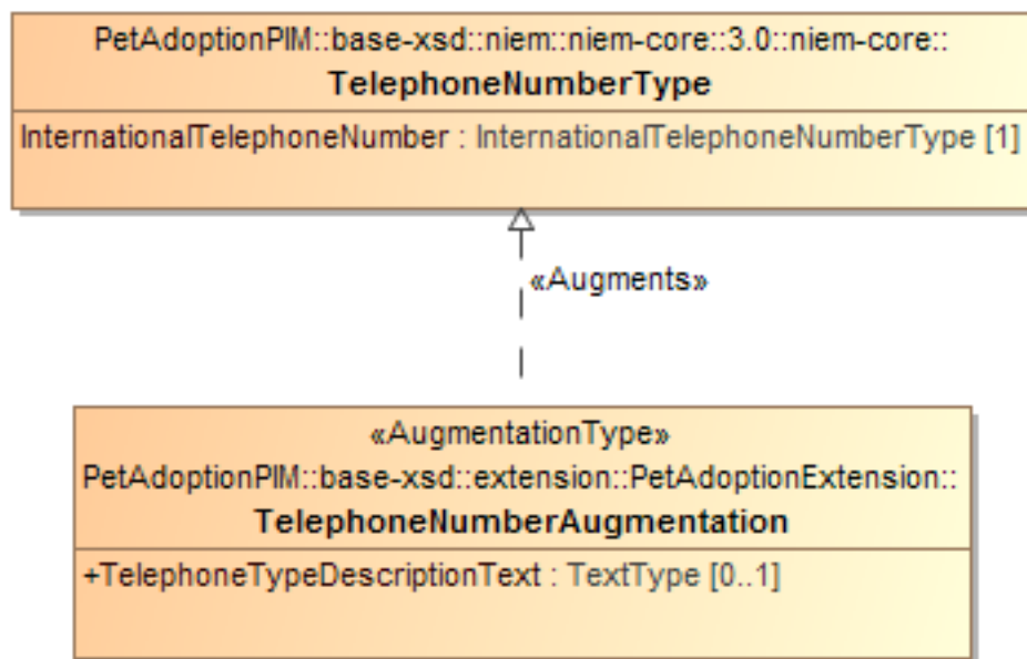
Figure 10-18 Augmenting Telephone Number
