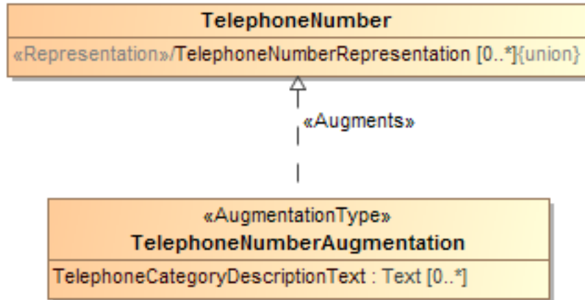
Figure 7-16 Representation of augmentation in a PIM
