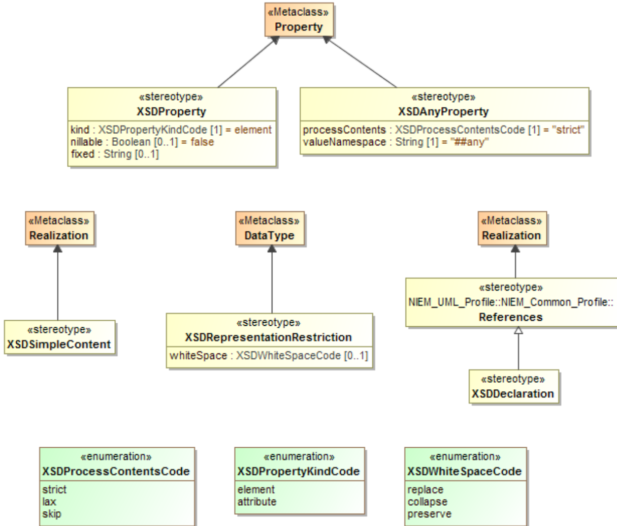
Figure 8-4 NIEM PSM Profile
