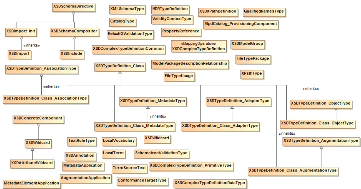
Figure 9-34 NIEM MPD Artifact to NIEM MPD Model - Inheritance NIEM Type Mapping
