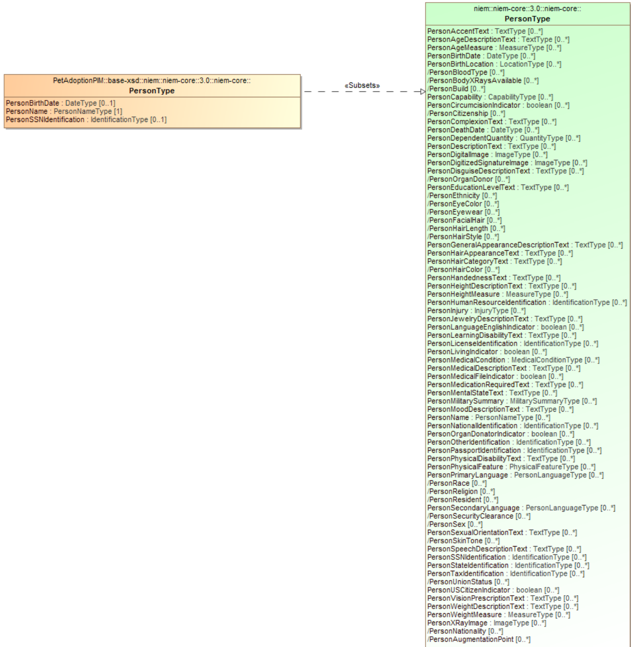
Figure 10-14 Reuse of Person Class
