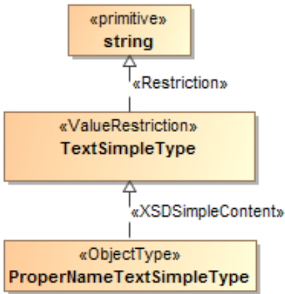
Figure 7-21 Representation of primitive types in a PSM
