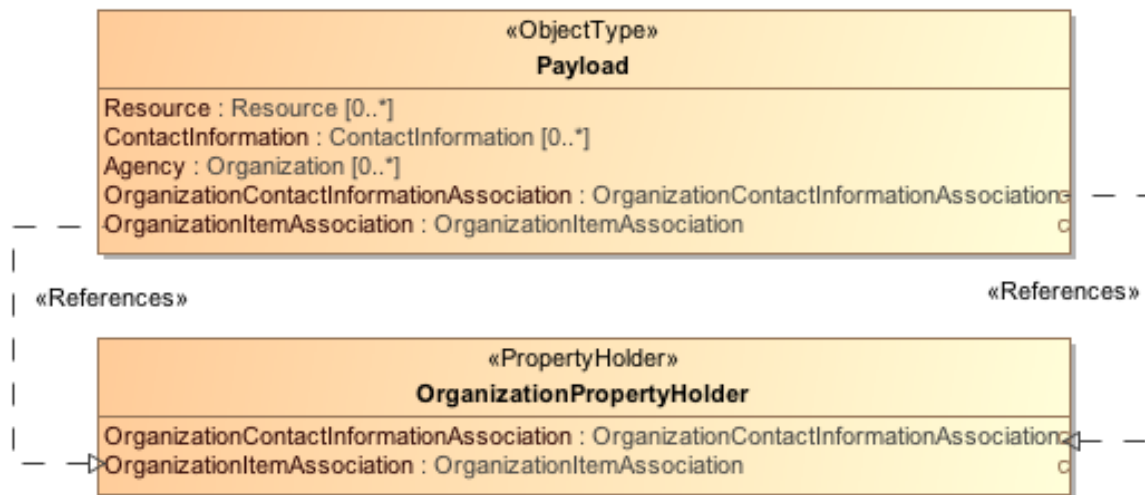
Figure 7-31 Representation of property references using «References» realizations
