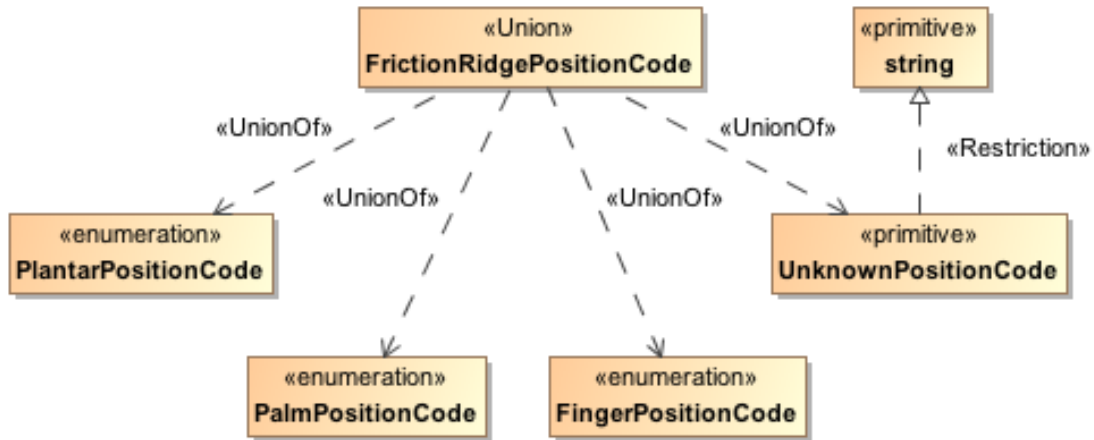
Figure 7-25 Representation of a union as a UML data type
