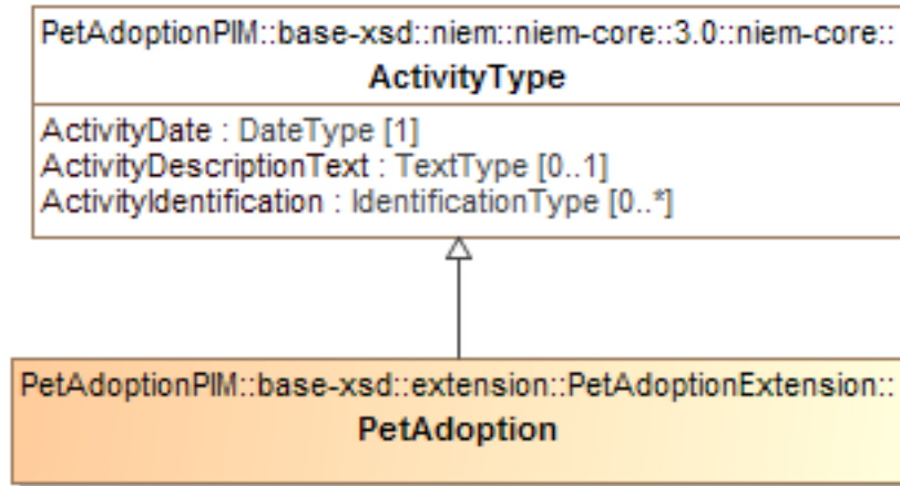
Figure 10-21 PetAdoption as a kind of Activity
