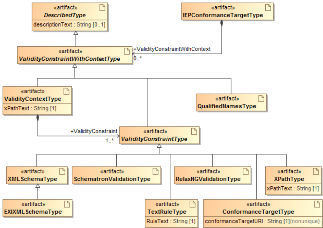
Figure 8-7 MPD Profile Artifacts for validation
