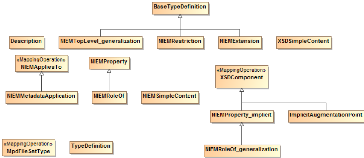
Figure 9-12 NIEM PIM to NIEM PSM Inheritance (2)
