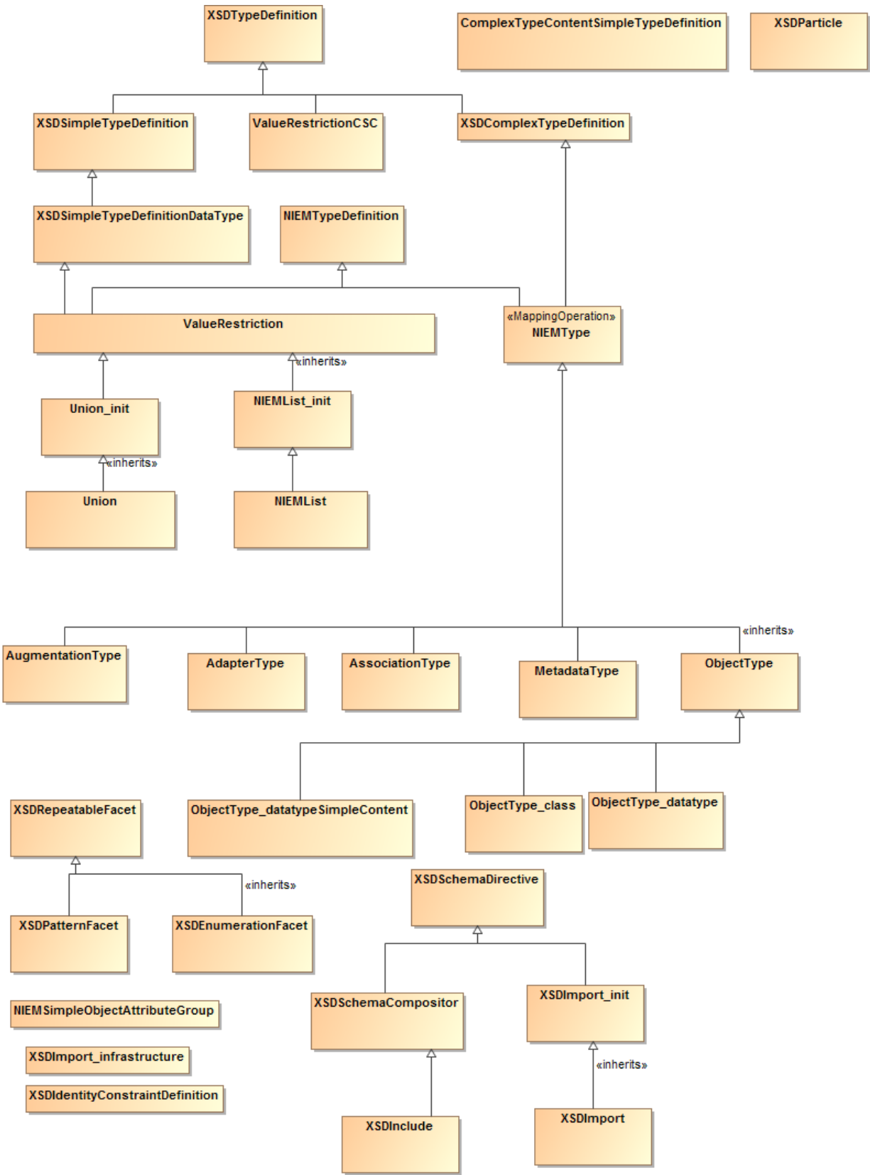
Figure 9-22 NIEM PSM to NIEM-Conforming XML Schema - Inheritance Other
