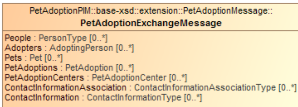
Figure 10-25 Exchange message type
