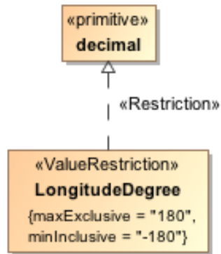
Figure 7-22 Representation of a primitive type with a value restriction in a PSM
