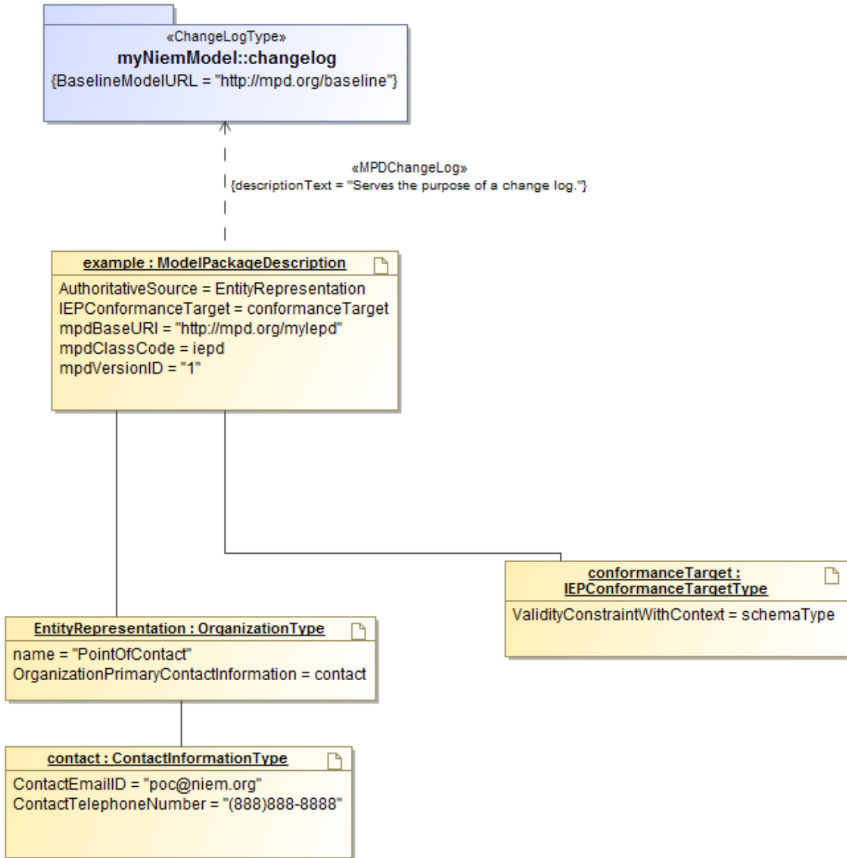
Figure 7-39 Representation of a NIEM MPD
