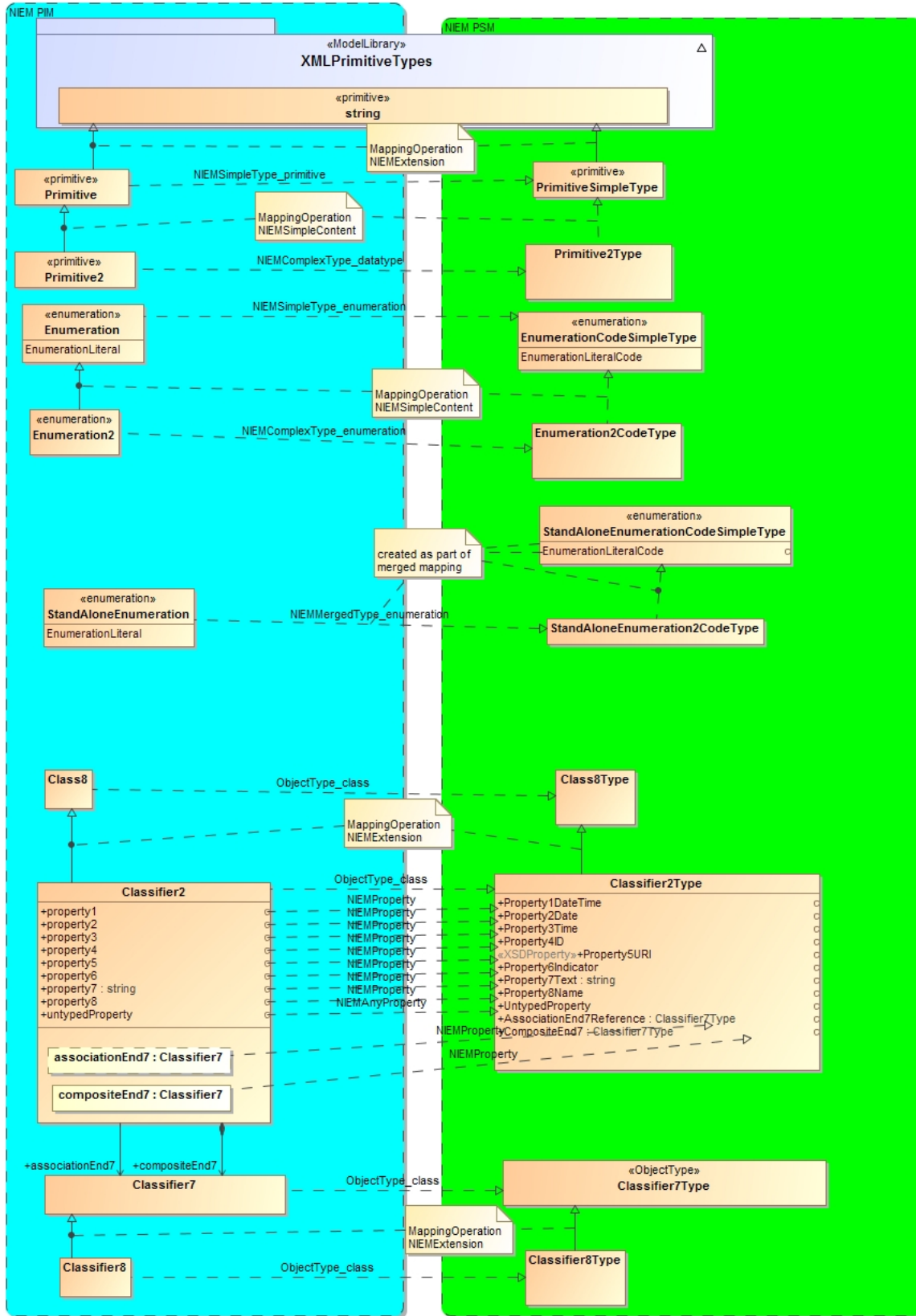
Figure 9-6 NIEM PIM to NIEM PSM - PSM Profile Mapping Overview
