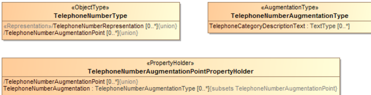
Figure 7-17 Representation of augmentation in a PSM
