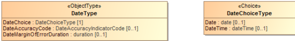
Figure 7-36 Representation of a choice group
