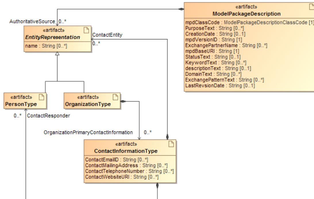
Figure 8-6 MPD Profile Artifacts for contact information
