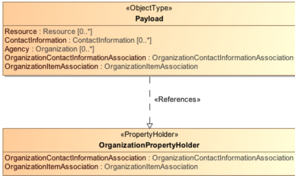
Figure 7-32 Alternative representation using «References» realizations between classes
