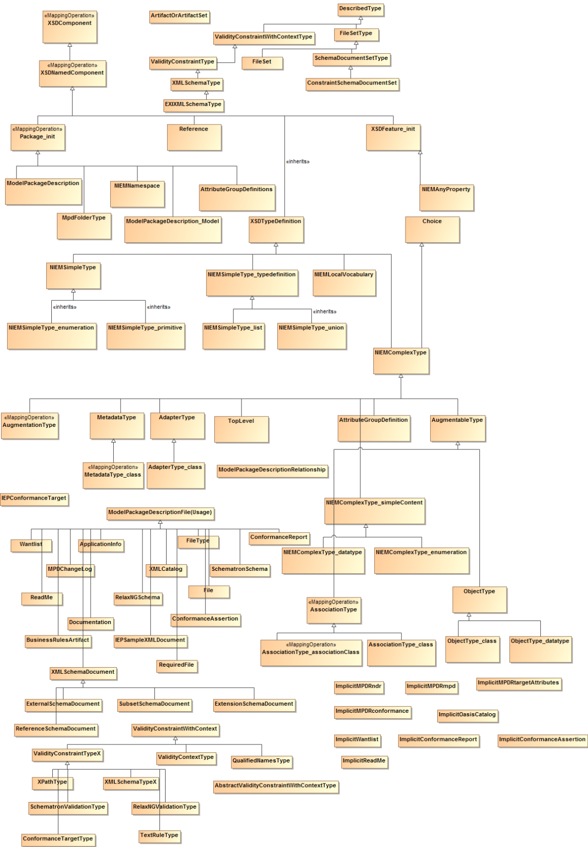
Figure 9-11 NIEM PIM to NIEM PSM Inheritance (1)
