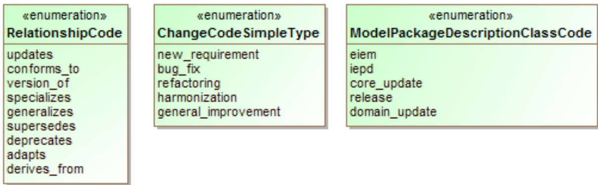
Figure 8-8 MPD Profile Enumerations
