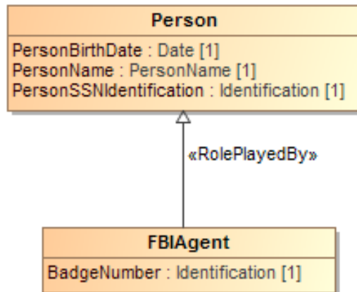
Figure 7-8 Representation of a role type using a generalization in a PIM
