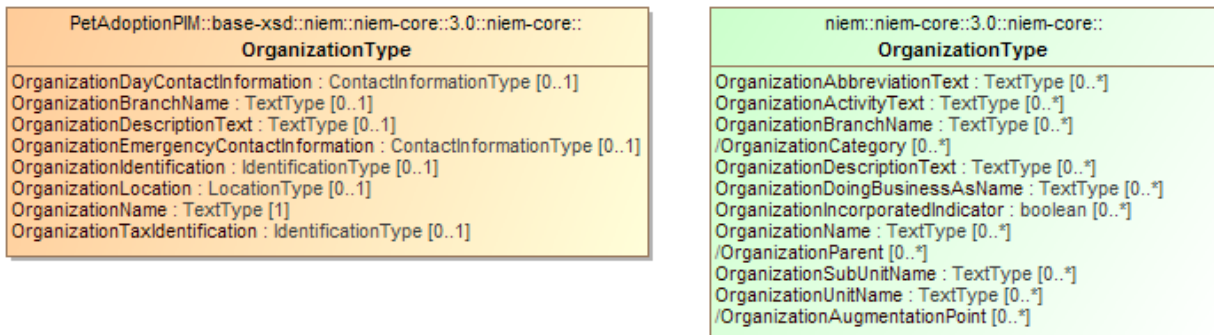
Figure 10-22 Using Organization from Core
