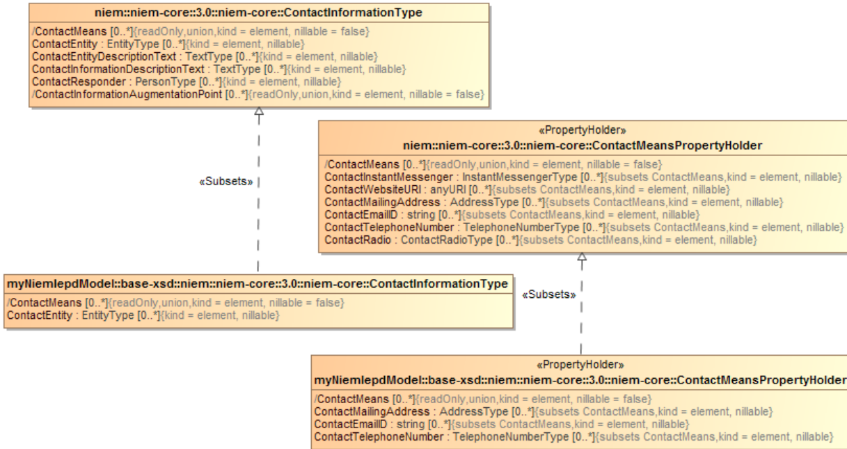
Figure 7-37 Representation of a subset model using «Subsets» realizations between classes
