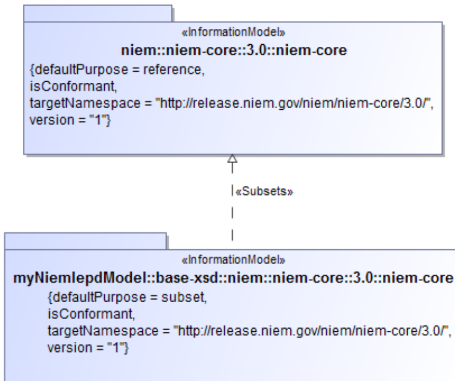
Figure 7-38 Alternative Representation using «Subsets» realization between packages
