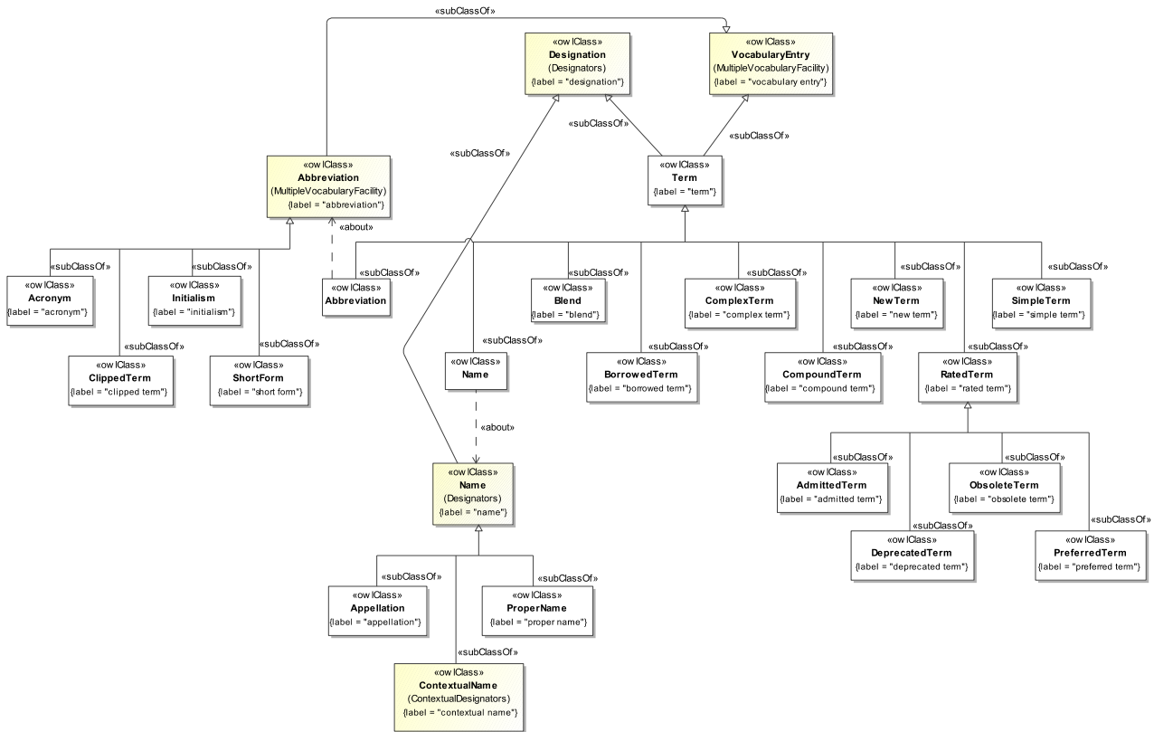
Figure 7: ISO 1087 Term Class Hierarchy
