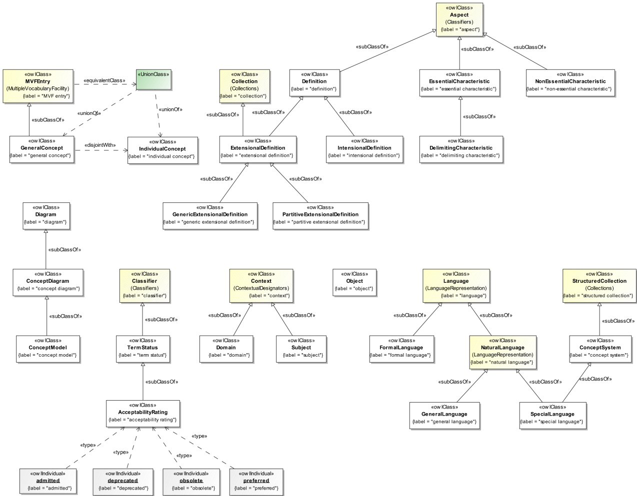
Figure 8: Characteristics, Definitions, Language Extensions, and Term Rating Aspects of the Ontology
