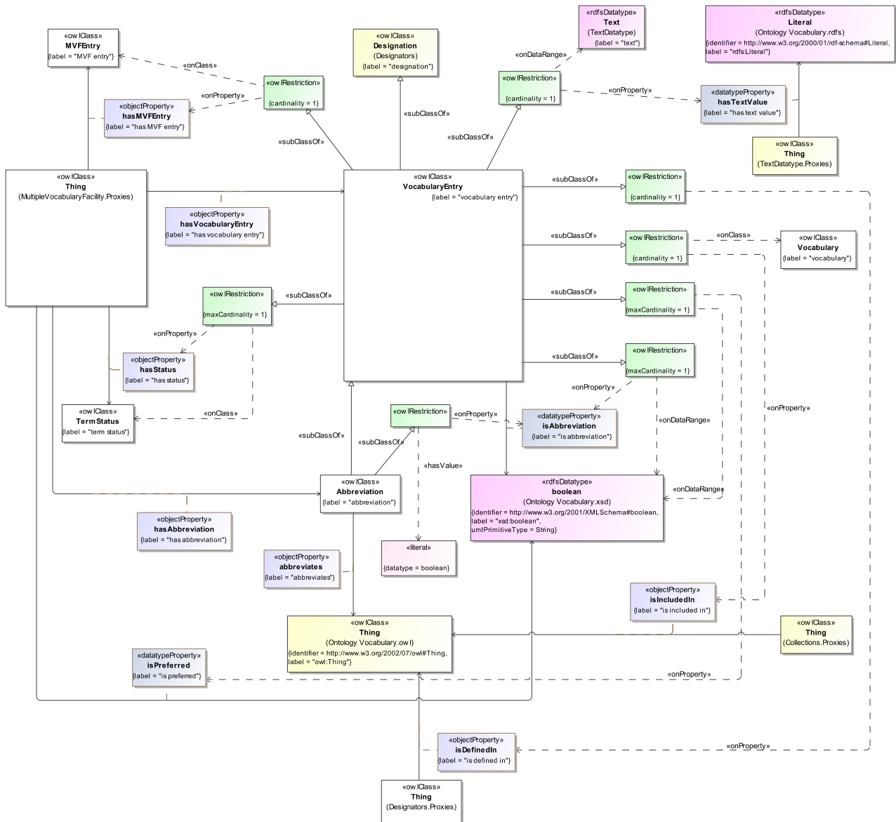
Figure 6: MVF Vocabulary Entry Class Diagram
