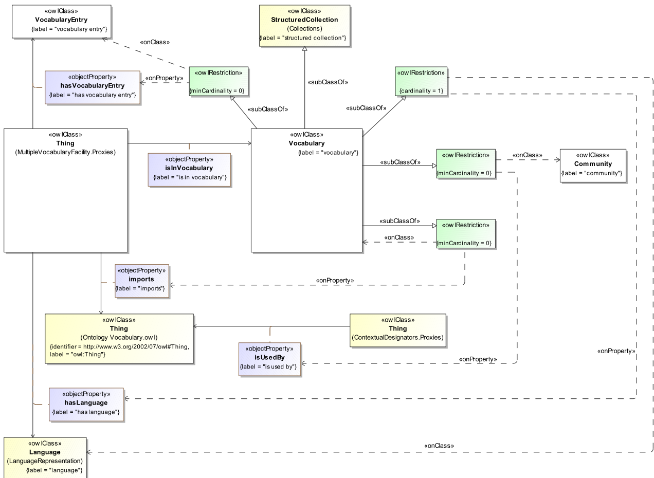
Figure 5: MVF Vocabulary Class Diagram
