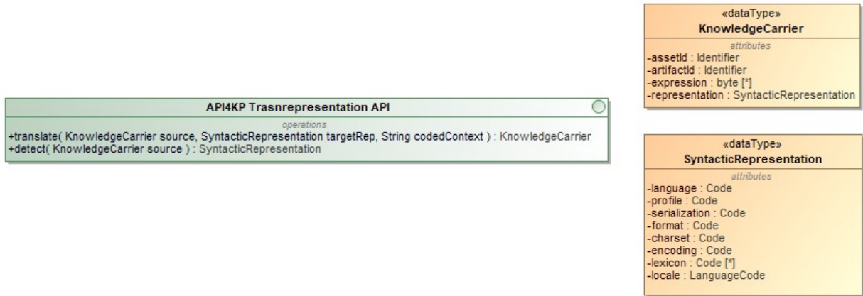
Figure 13: API4KP Translation API
