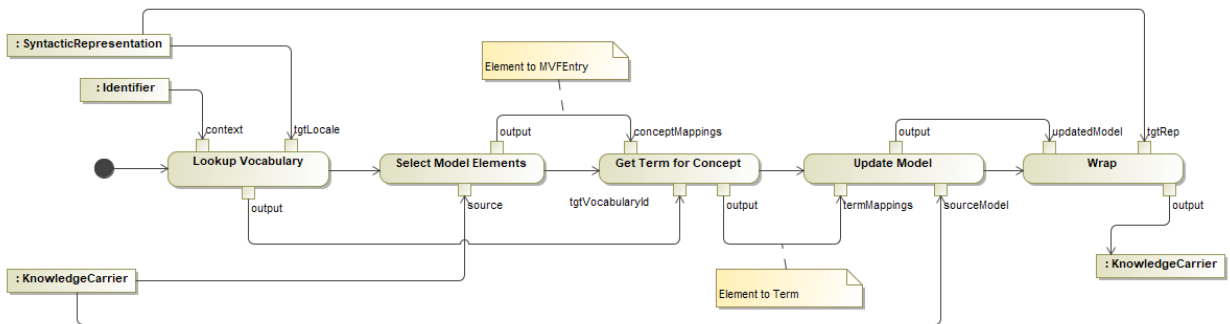
Figure 15: API4KP-based Specification of the MVF-profiled api4kp:translate operation
