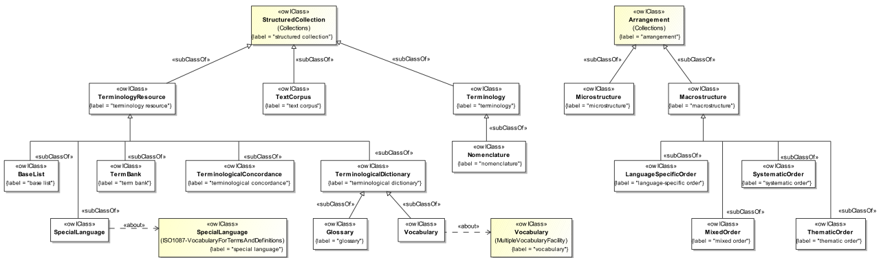
Figure 9: ISO 1087 Terminology Resource Class Hierarchy
