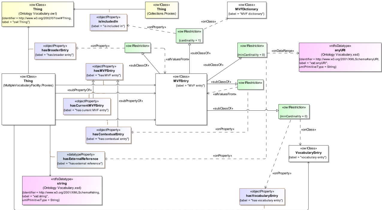
Figure 4: MVF Entry Class Diagram
