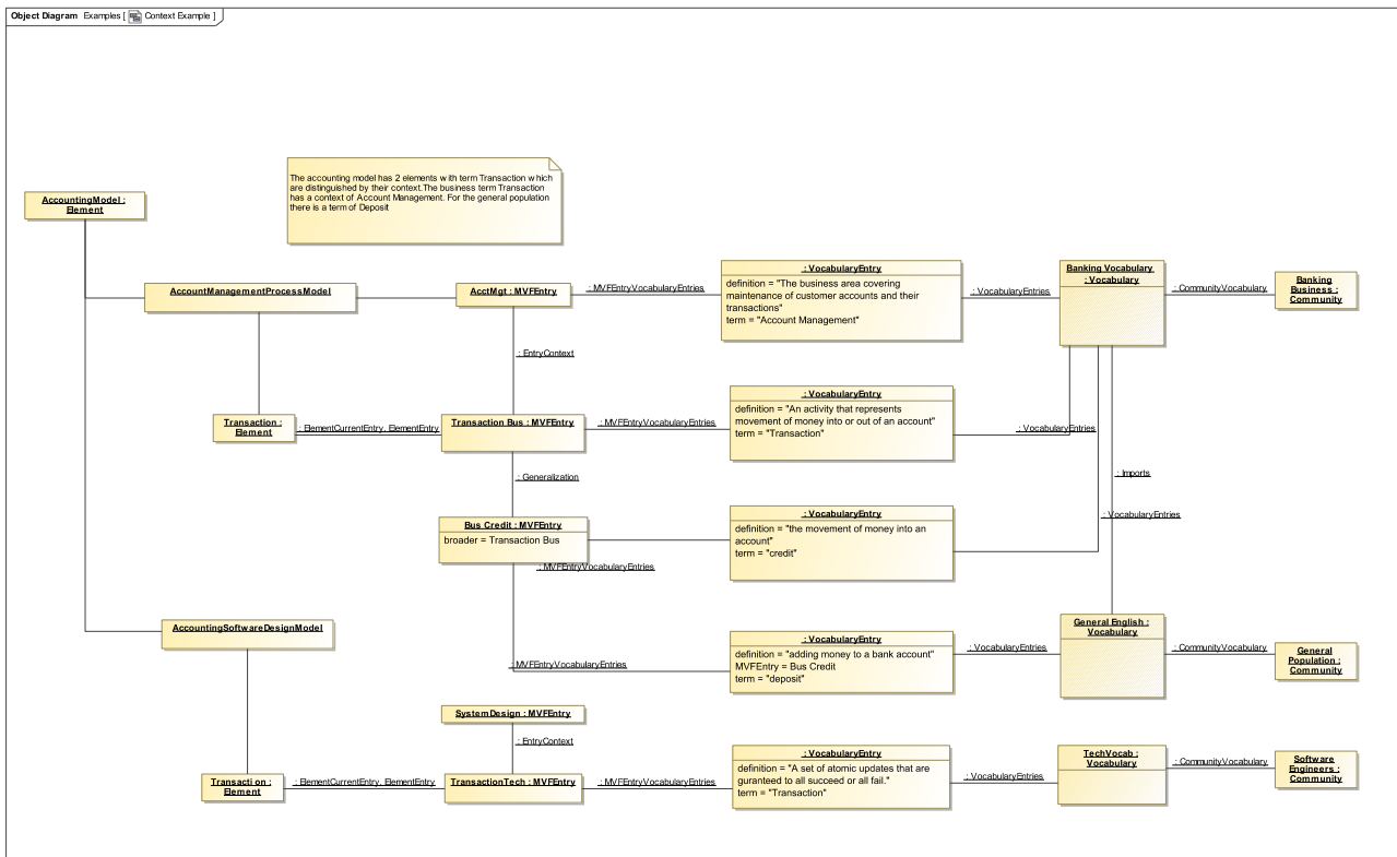
Figure 16: Example showing a mapping from multiple vocabulary elements to the same concept
