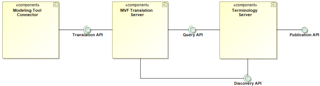
Figure 11: Notional Component / Interface Integration
