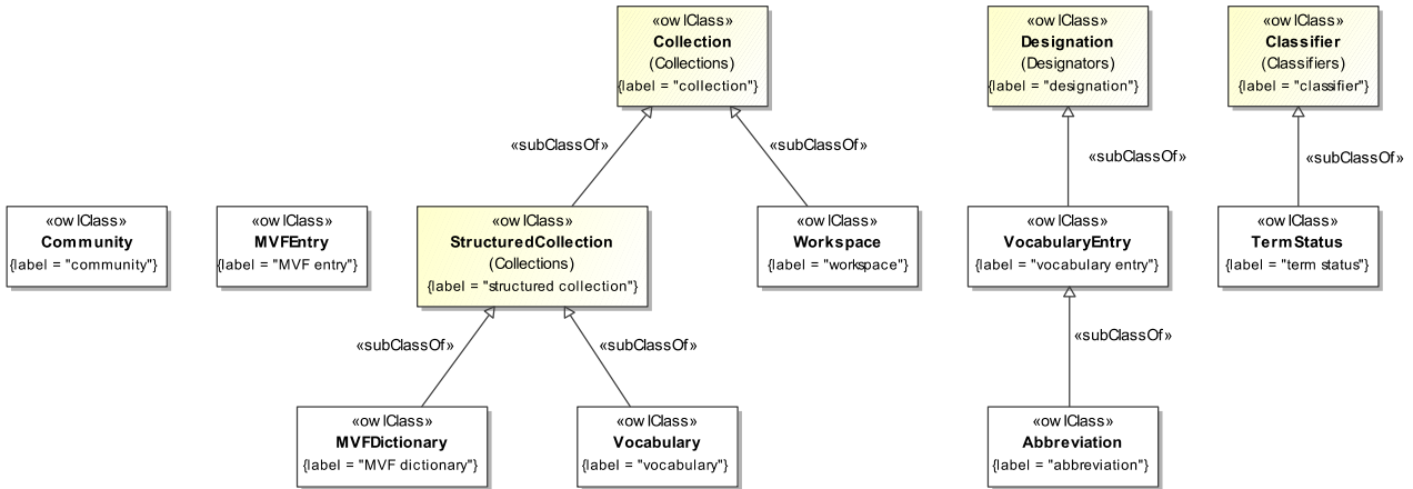
Figure 3: MVF Class Hierarchy
