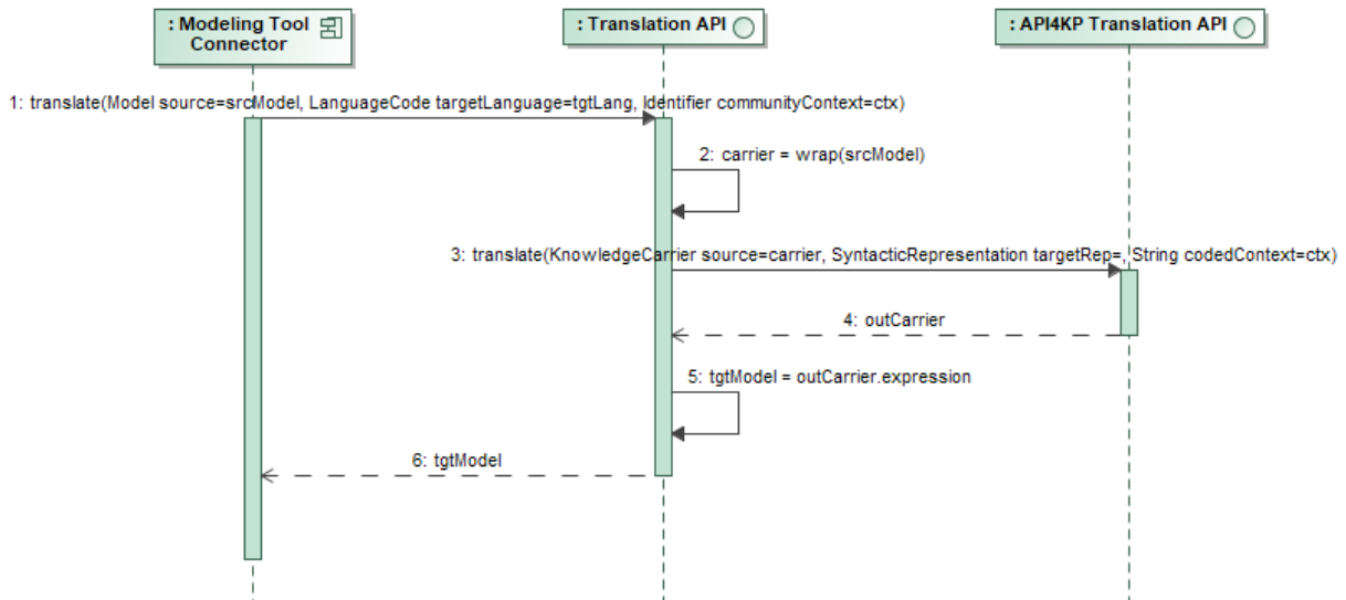
Figure 14: MVF to API4KP Delegation
