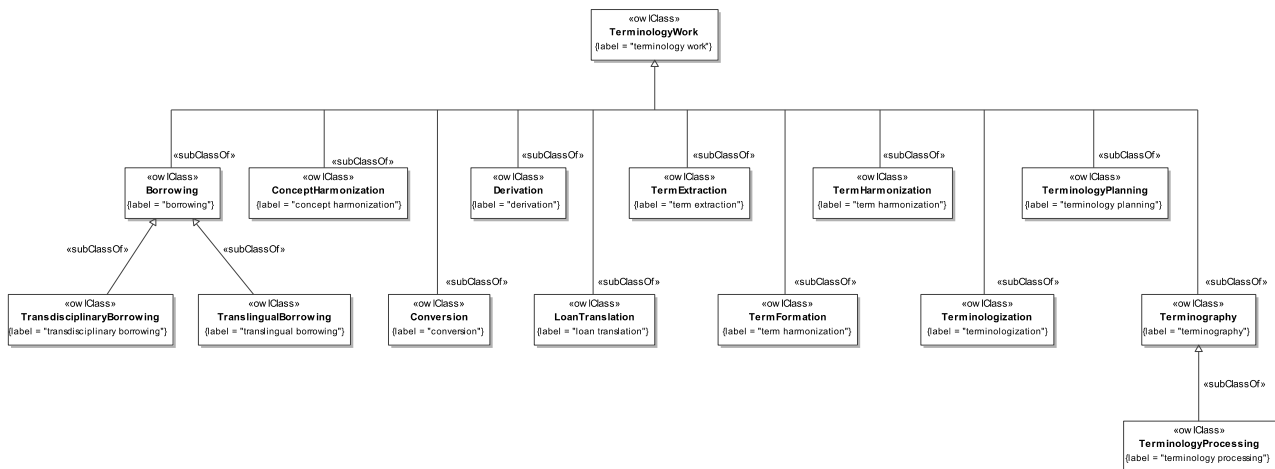
Figure 10: ISO 1087 Terminology Work Class Hierarchy
