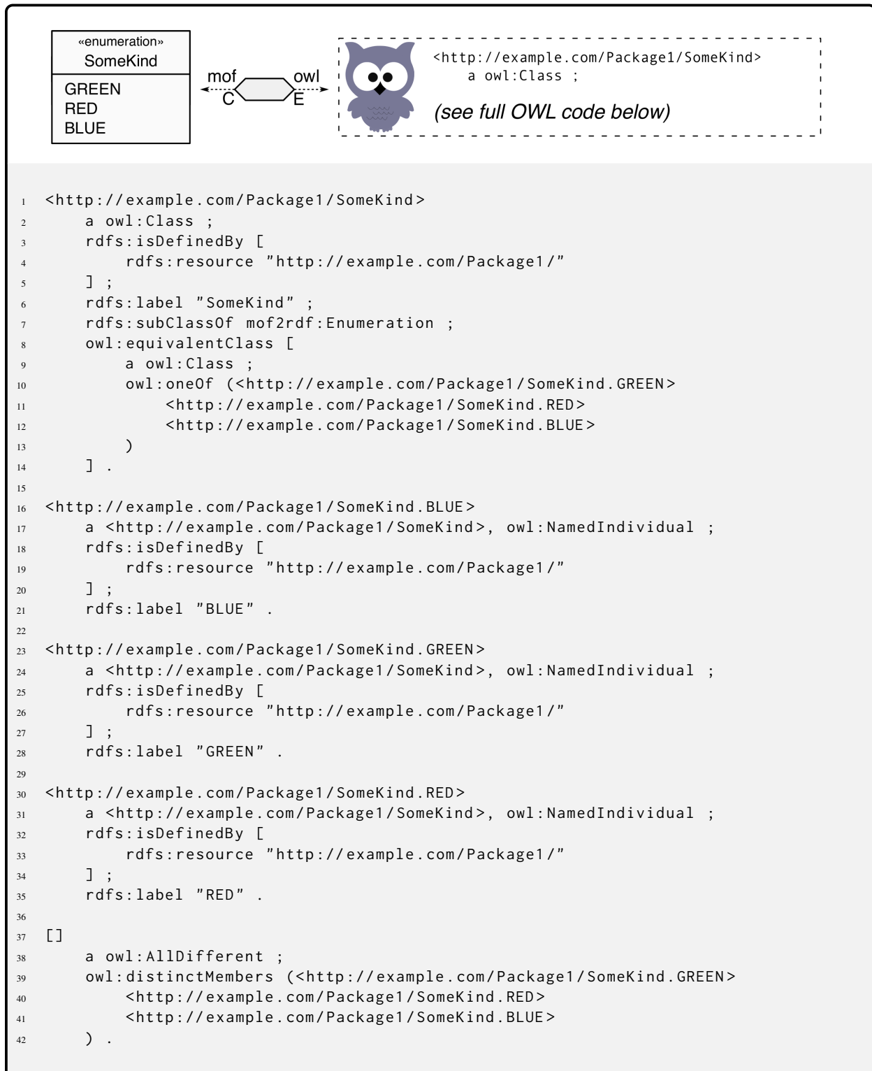
Mapping of Enumeration types
