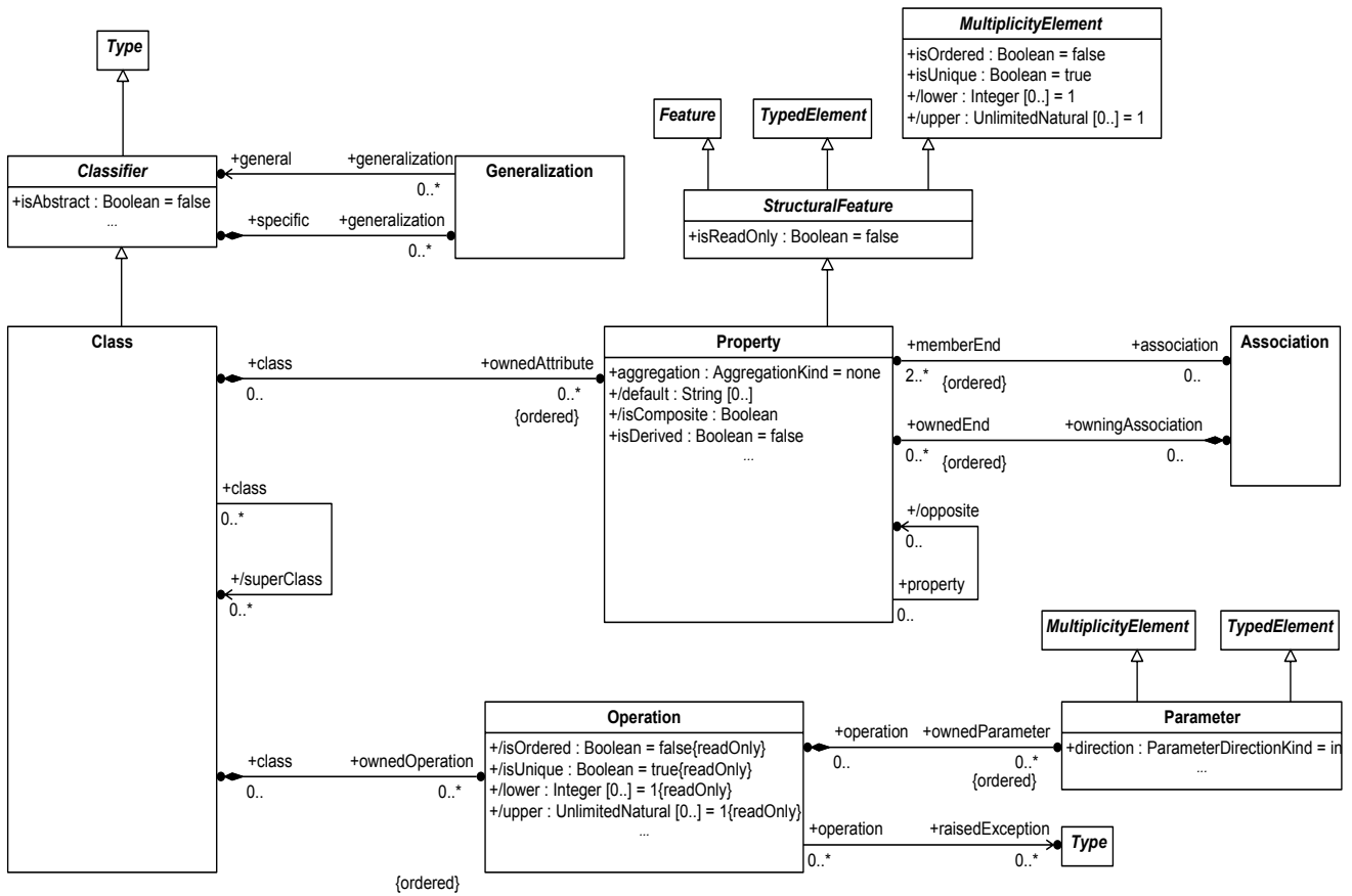
Figure 12.2 - EMOF Classes
